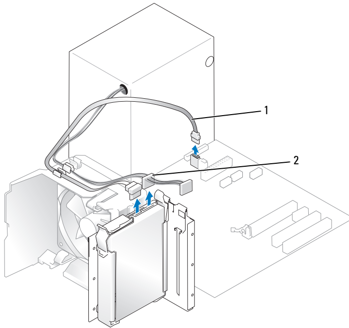
1 serial ATA data cable 2 power cable
