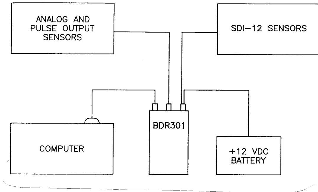
FIGURE 1-2. System Block Diagram
