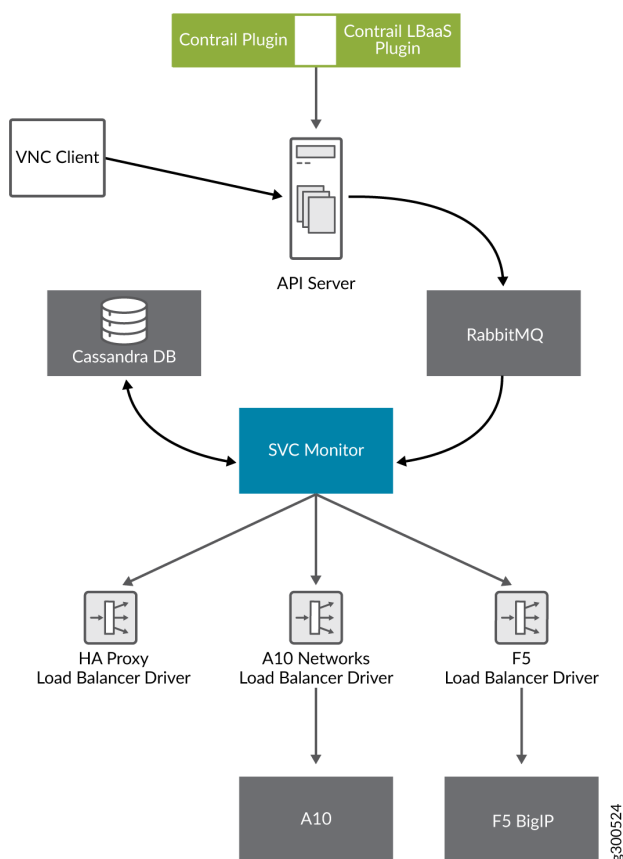
Figure 64: Contrail LBaaS components with neutron-lbaas
