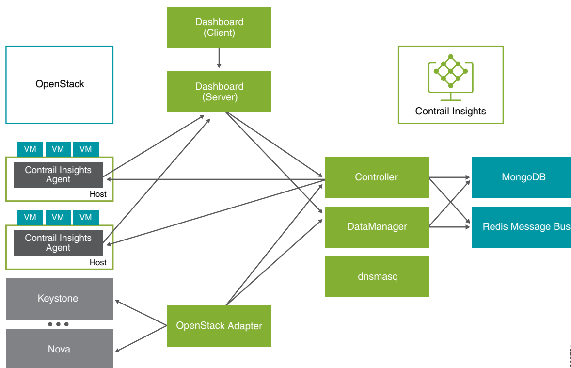
Figure 75: Contrail Insights Architecture with OpenStack
