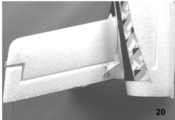
Fig. 20 - The photo shows the finished view.
