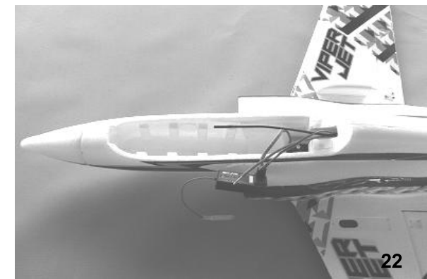
Fig. 22 - Connect the electronic speed controller and servos to the receiver. Refer to the radio instructions for the correct channel sockets and servo lead polarity.
