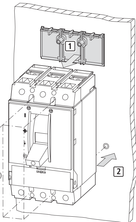
Connector Type NZM2-XKA
