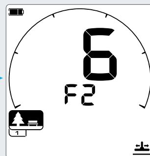
Press Accept/Reject to advance to adjusting the Iron Bias F2 setting.
