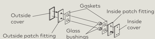
Bottom bolt patch fitting assembly, mounting Screws provided with patch fitting.
