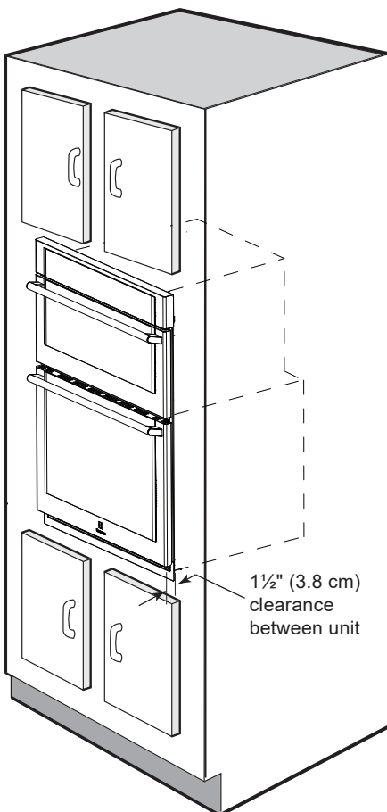
Figure 6: Cabinet Installation
