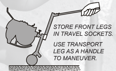
Figure 8 Maneuvering
