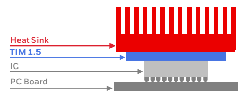
Figure 2. A: Schematic of thermal interface materials used in a flip-chip package. TIM 1 is placed between the chip (or die) and the integrated heat spreader. TIM 2 is placed between the IHS and the heat sink; B: TIM 1.5 is placed between the chip and the heat sink.
