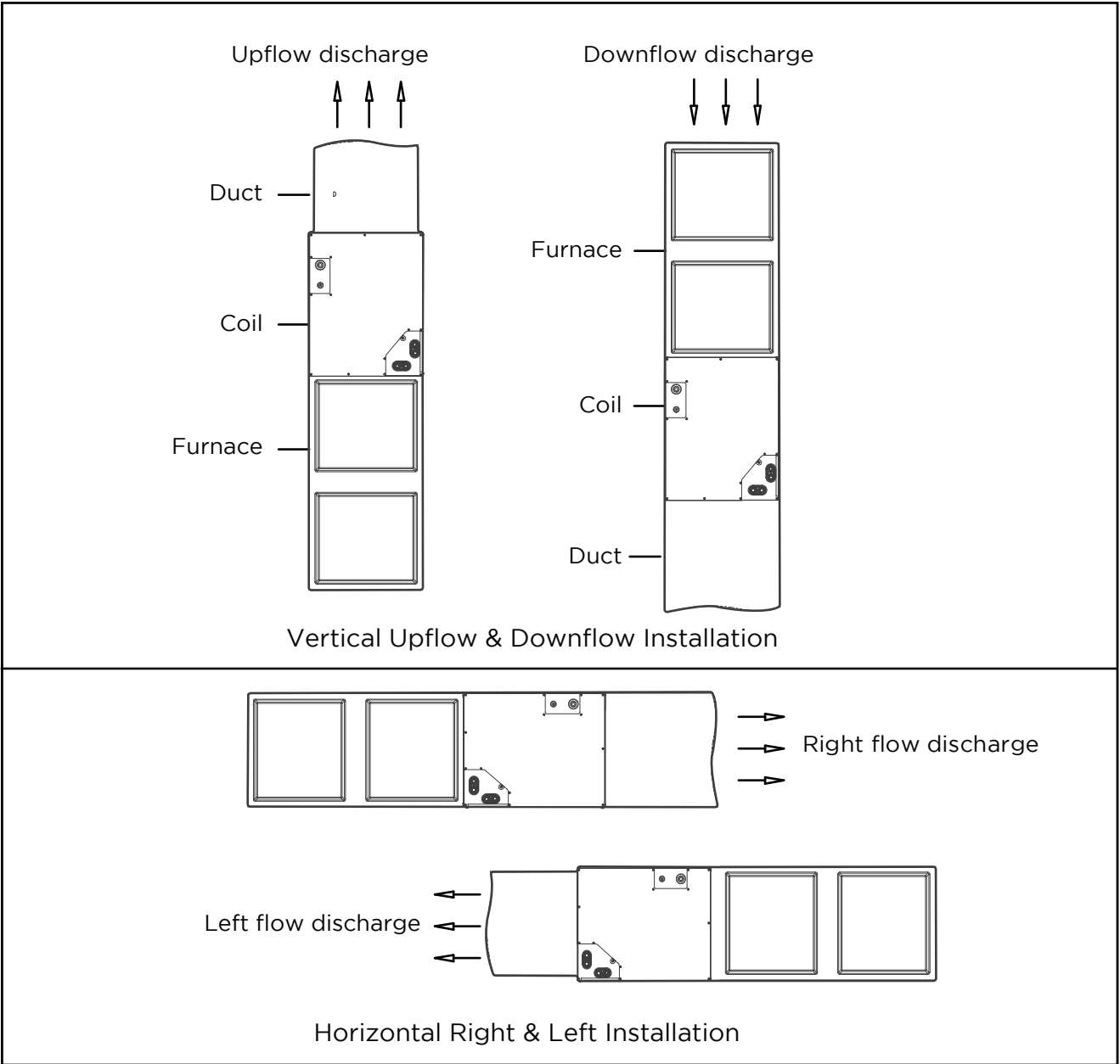
Installation type 2: Model MMC60H2128B coil installation on furnace
