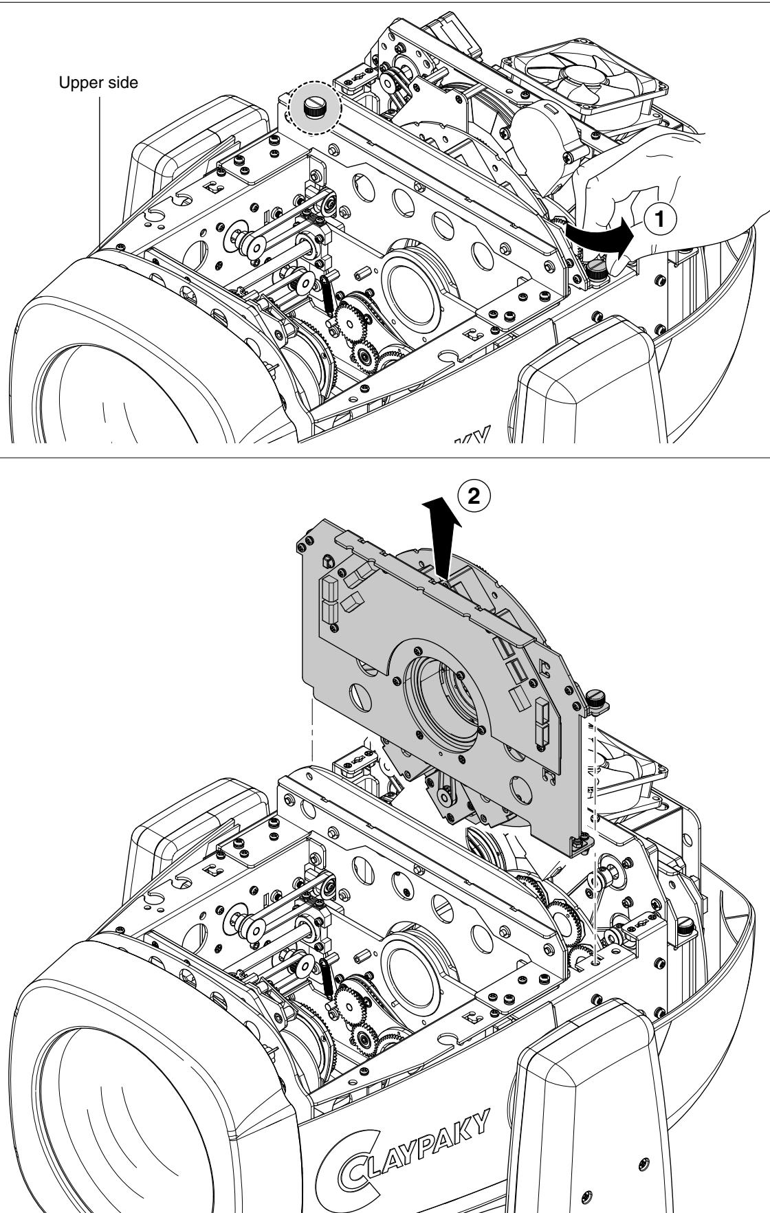
Extraction of the effect modules - Fig. 14.
