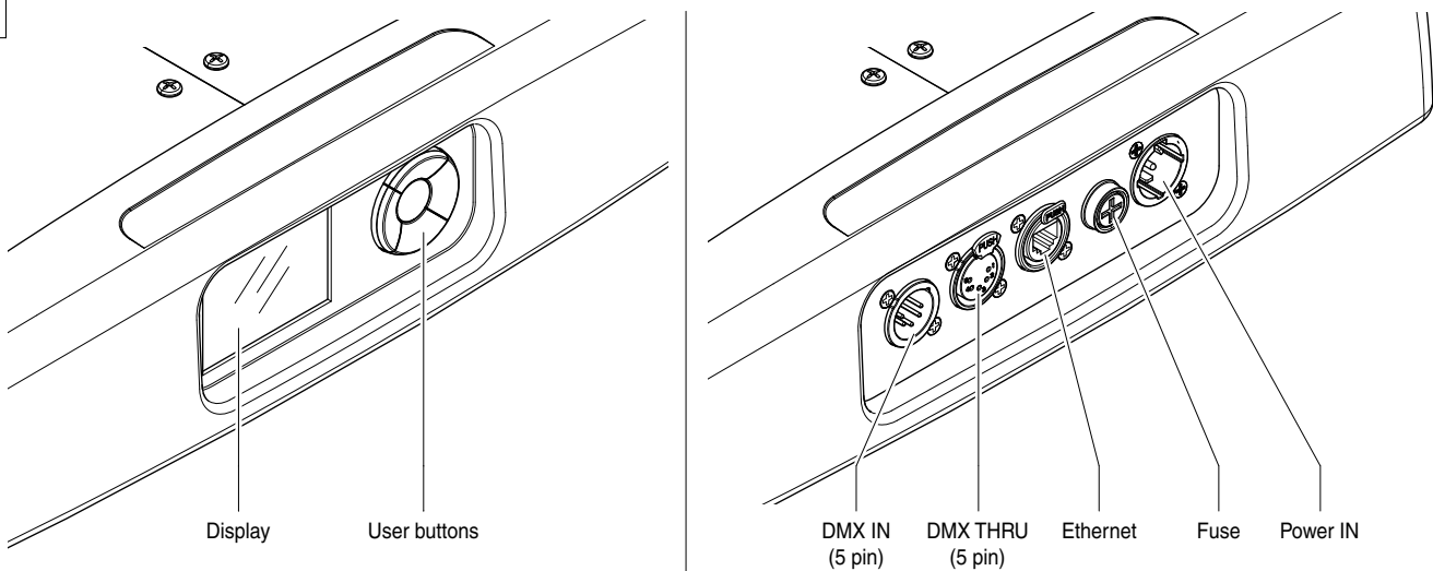
Control panel - Fig. 5
