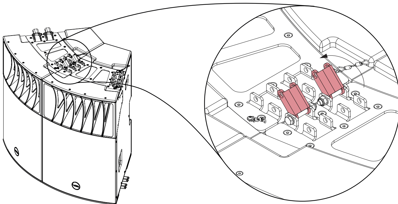
Figure 5.6: Links
