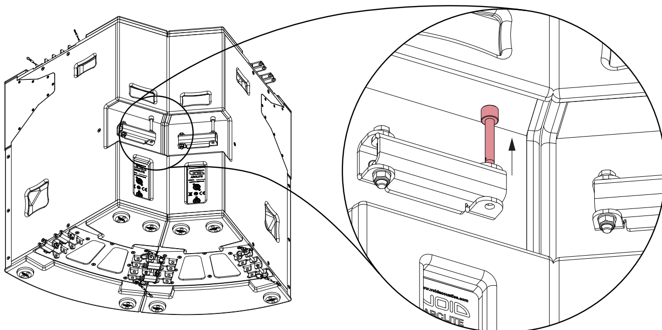
Figure 5.10: Remove pin
