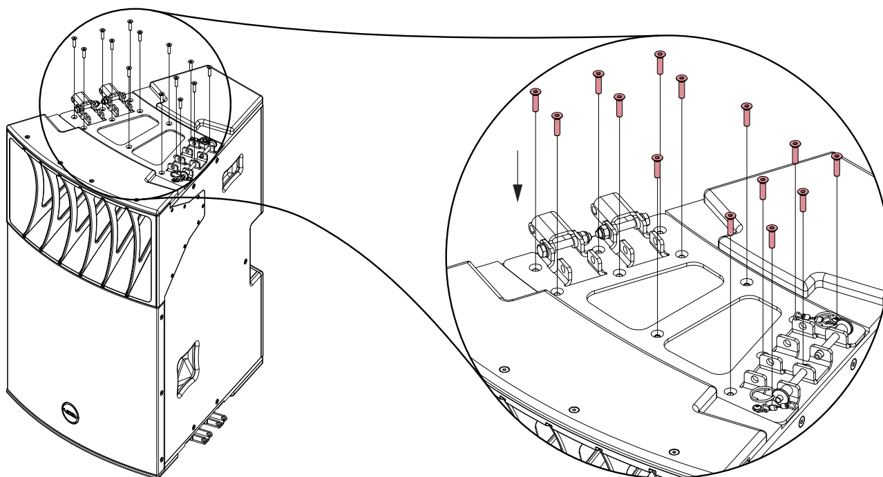
Figure 5.4: Plate fixing
