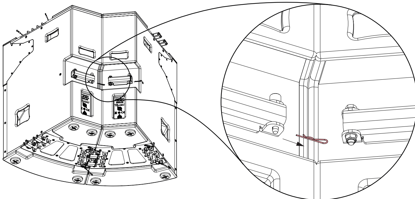
Figure 5.9: R-clip release
