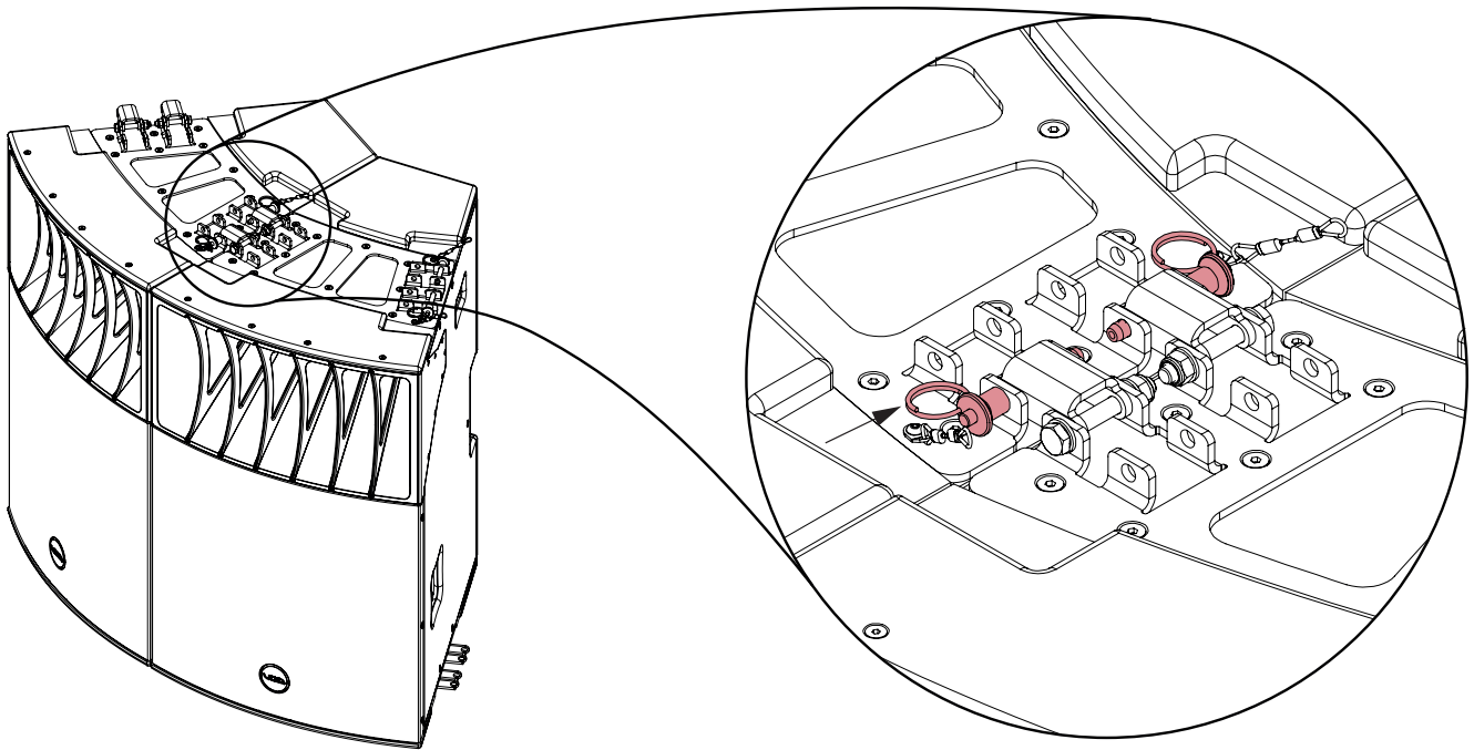
Figure 5.7: Insert pins
