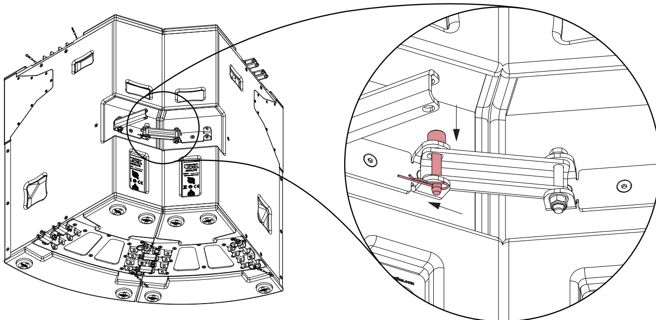
Figure 5.12: Link
