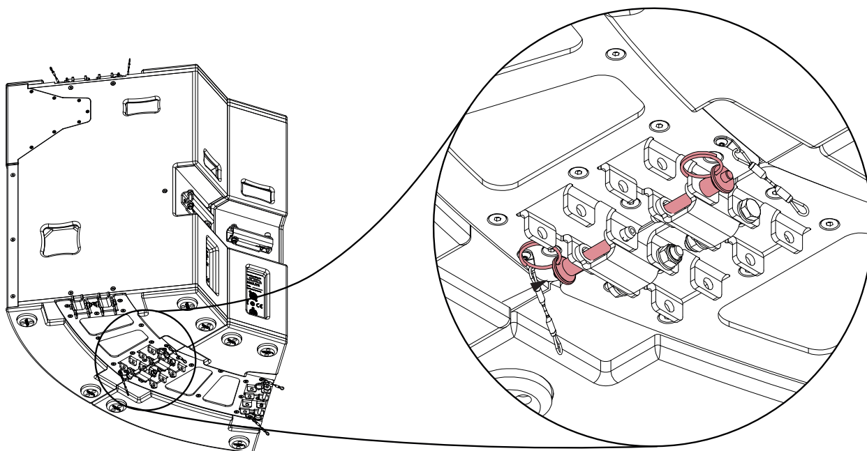
Figure 5.15: Insert pins
