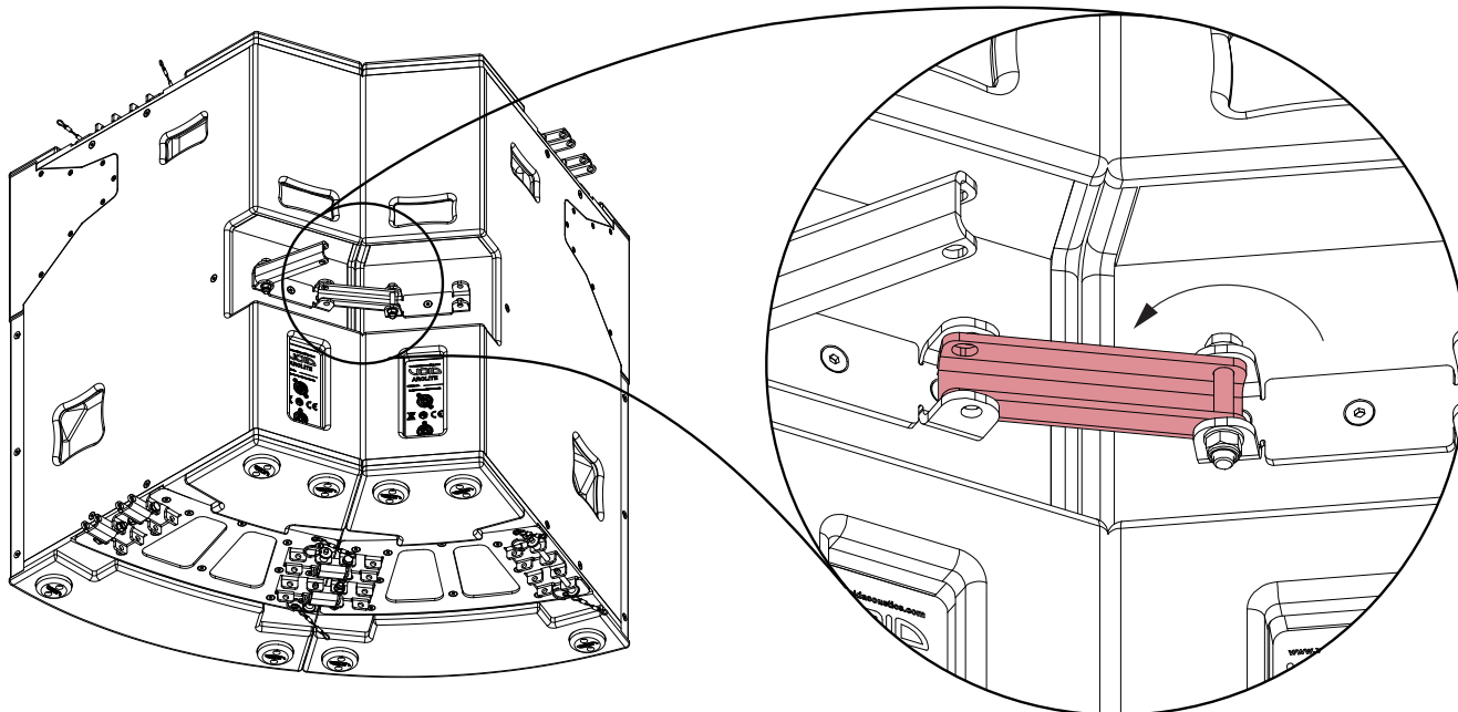
Figure 5.11: Rotate link
