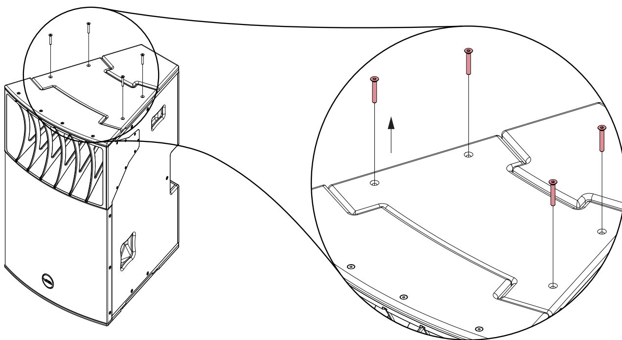
Figure 5.2: Bolt removal
