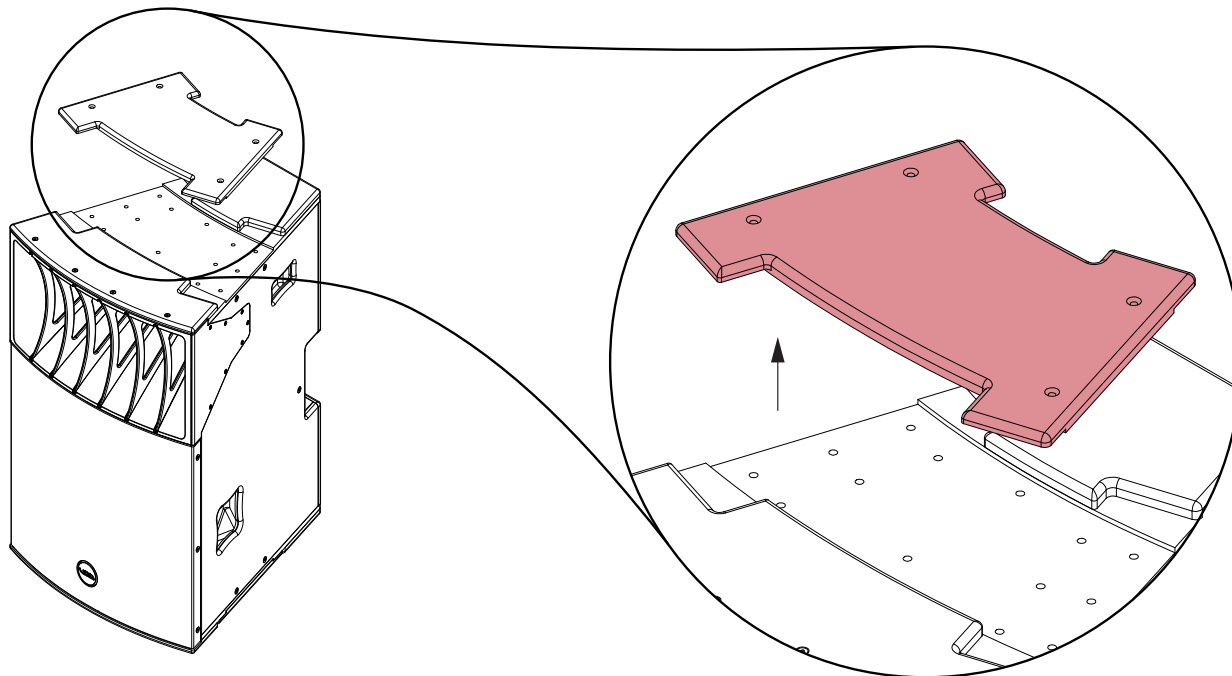
Figure 5.3: Remove infill
