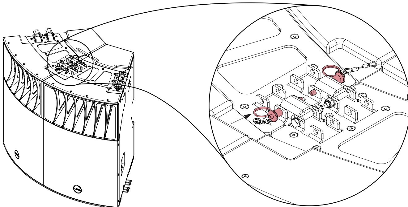
Figure 5.7: Insert pins
