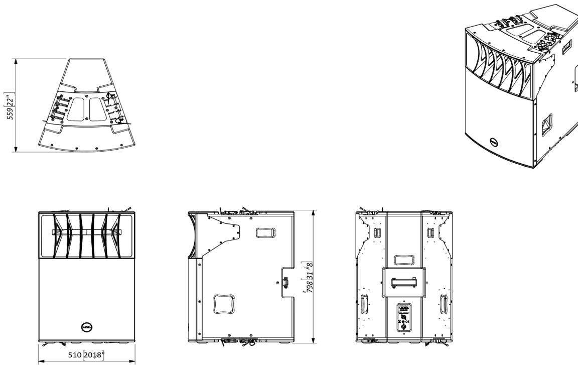
Figure 3.2: Dimensions
