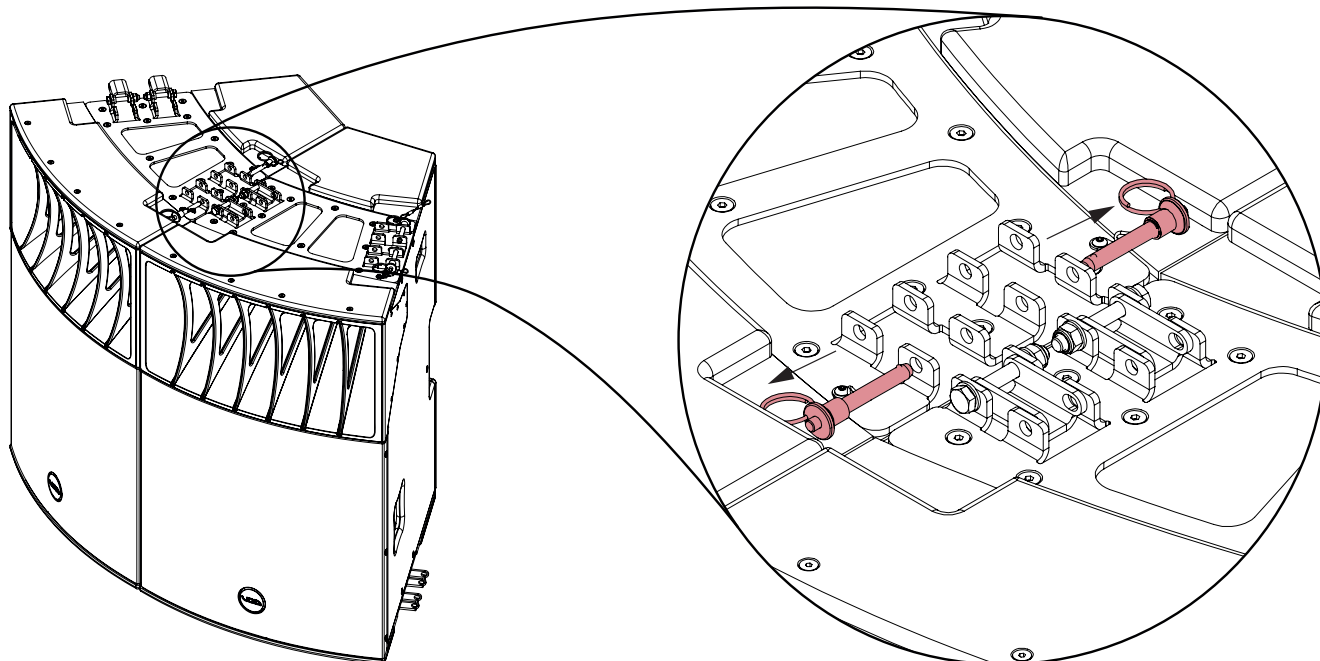
Figure 5.5: Quick release
