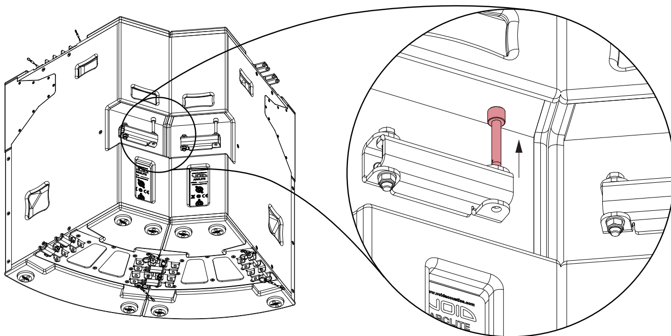
Figure 5.10: Remove pin
