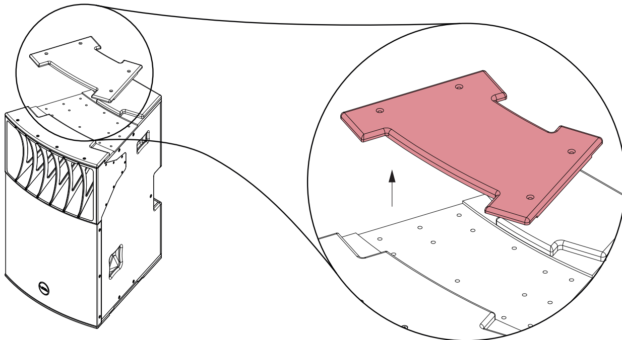
Figure 5.3: Remove infill
