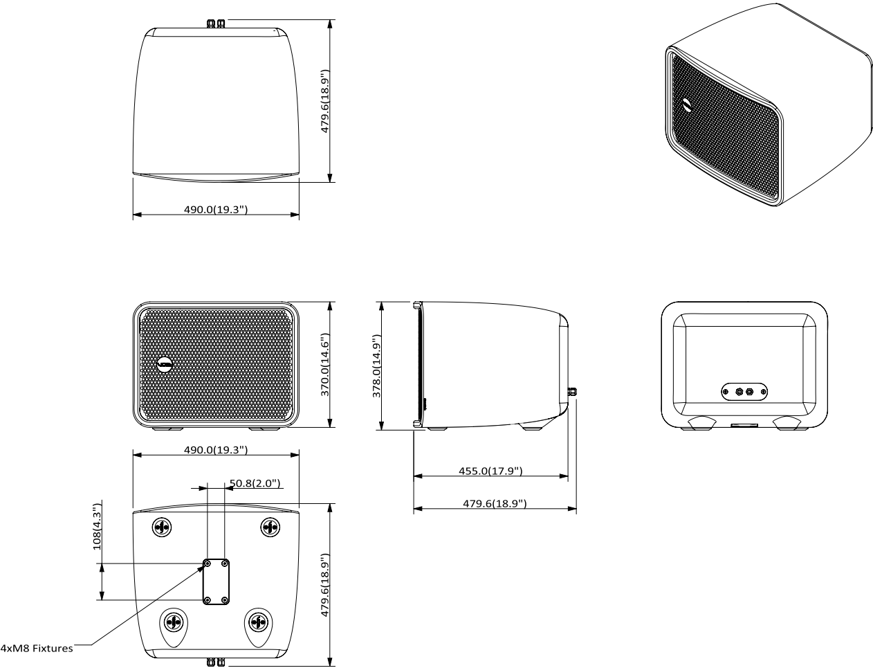
Figure 3.2: Dimensions
