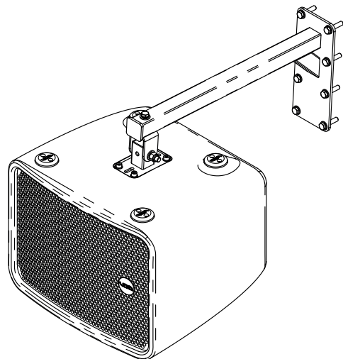
Figure 5.6: Loudspeaker positioning
