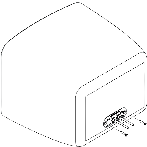
Figure 4.5: Phoenix attachment
