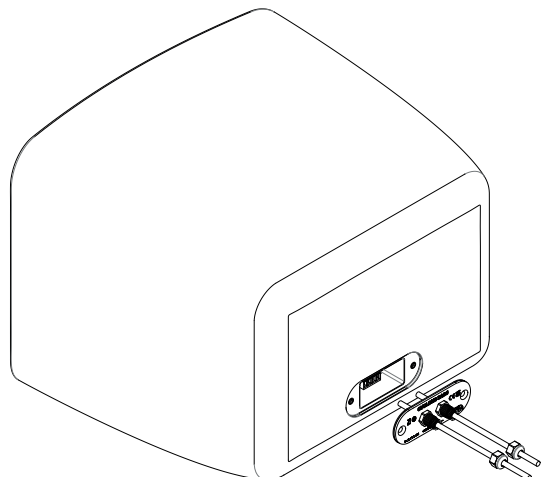
Figure 4.4: Cable connection
