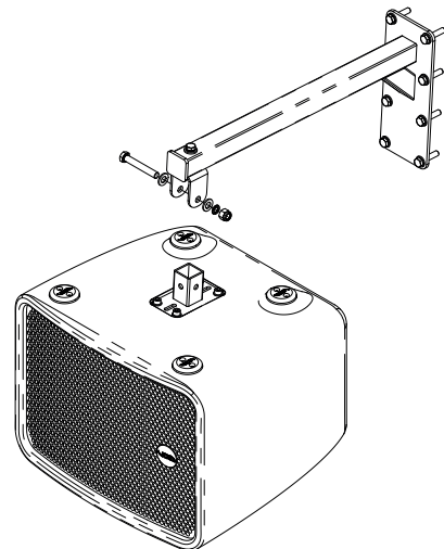
Figure 5.5: Loudspeaker fixing
