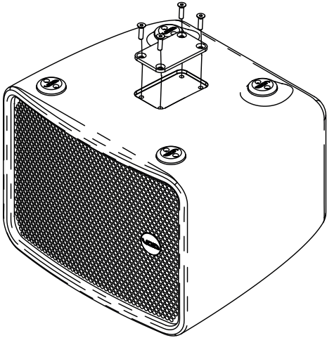
Figure 5.9: Bolt removal
