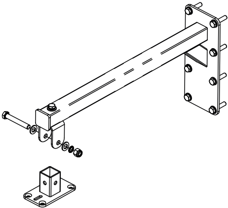
Figure 5.2: Nut removal
