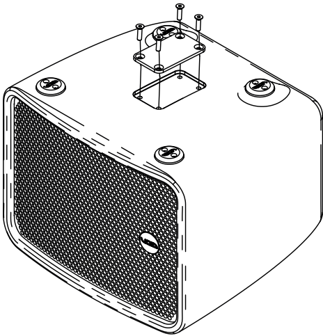
Figure 5.3: Bolt removal
