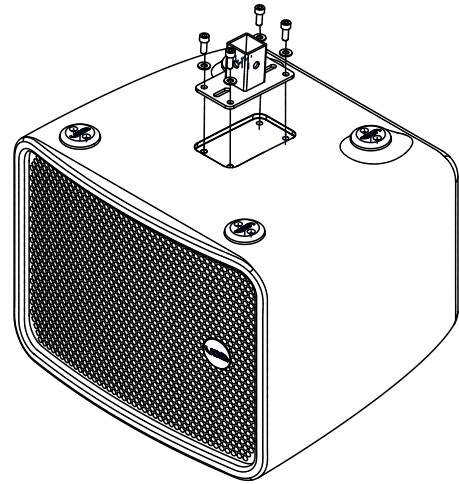
Figure 5.4: Attaching the type 75 plate
