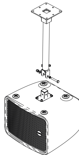
Figure 5.11: Loudspeaker fixing
