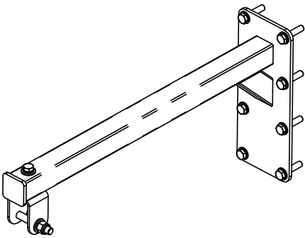
Figure 5.1: T75 wall bracket
