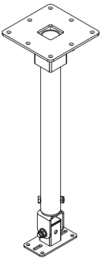
Figure 5.7: T75 ceiling bracket
