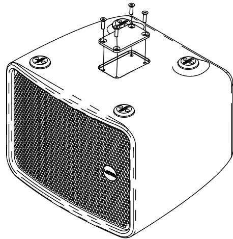
Figure 5.10: Attaching the type 75 plate
