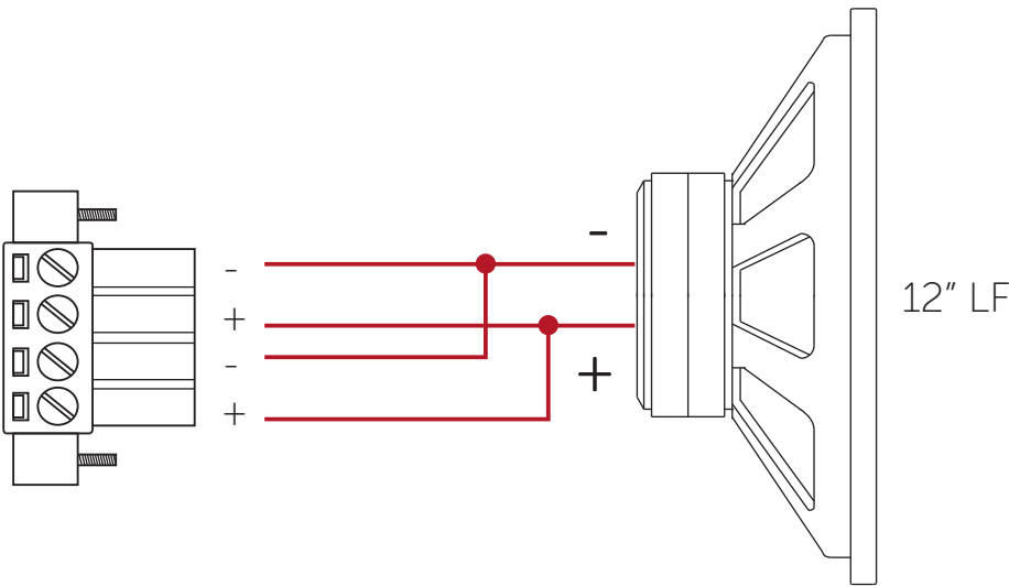
Figure 4.6: Wiring diagram
