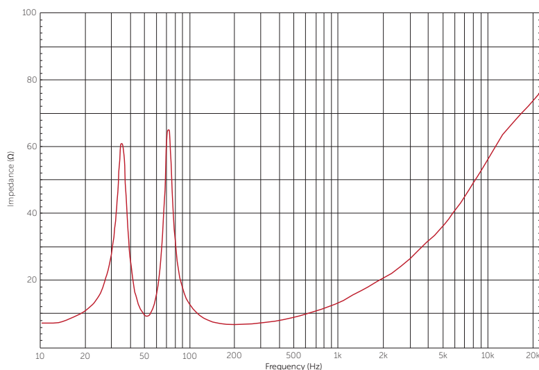
Figure 3.1: Impedance graph
