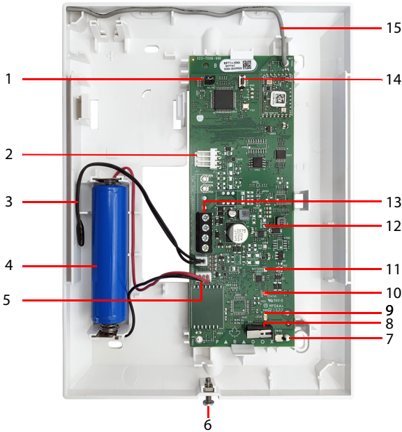
Figure 1: RPT1+ PCB
