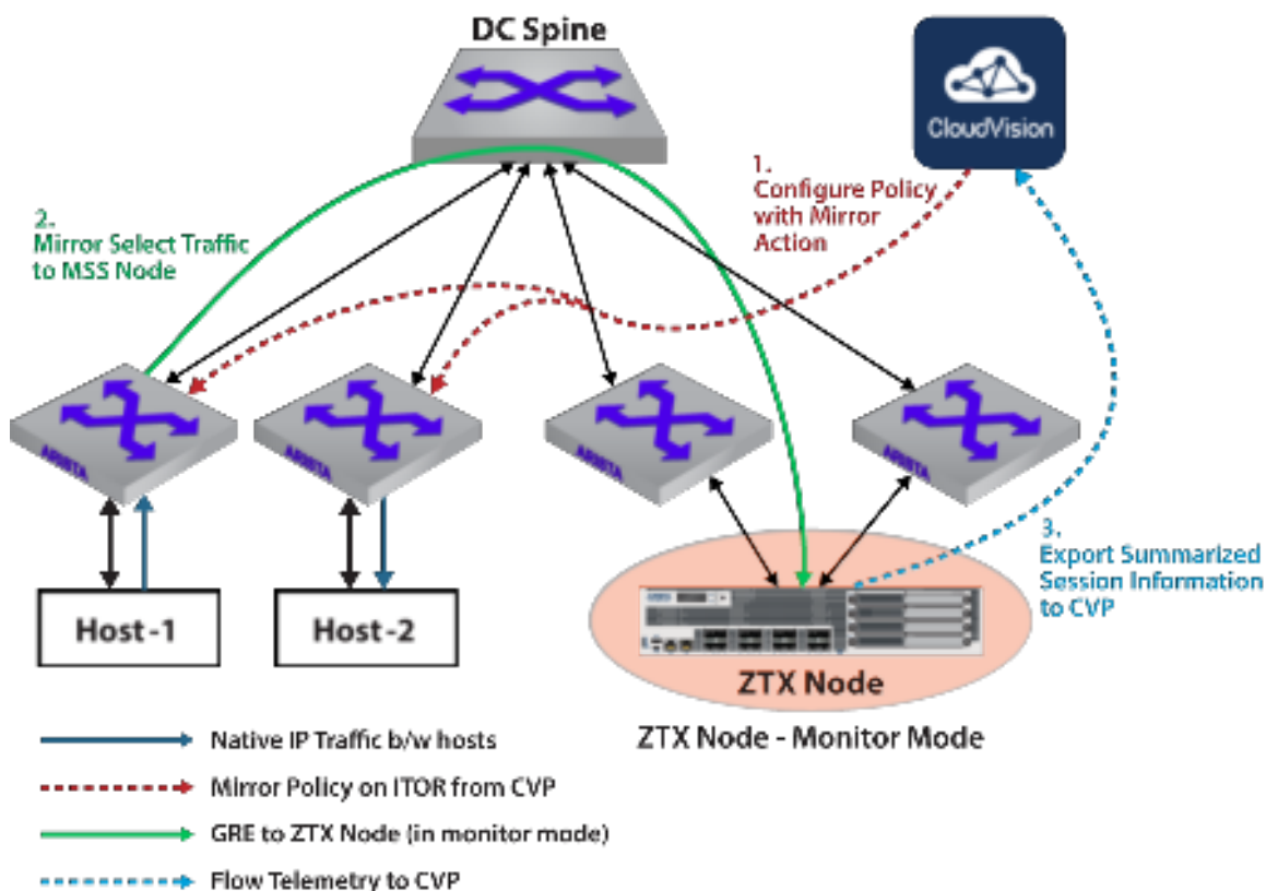
Figure 1-2: ZTX Node - Monitor Mode and Flow
