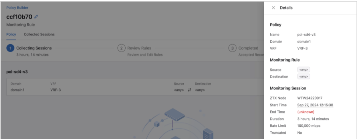
Figure 4-24: Monitoring Rule Details
