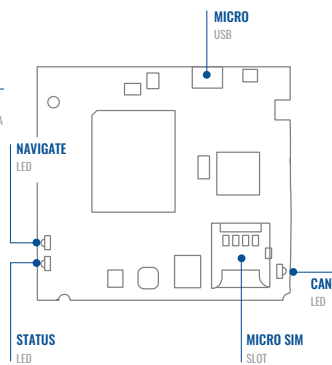
TOP VIEW (WITHOUT COVER)
