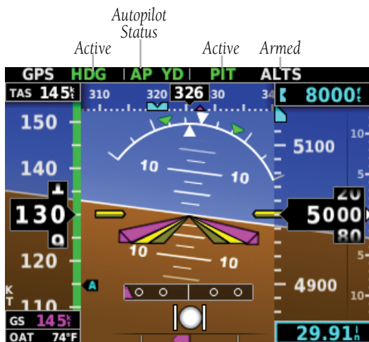
Figure 3-1 Autopilot Status Box
