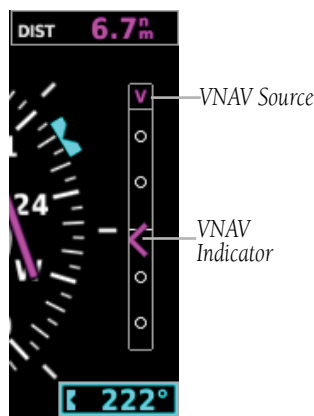
Figure 2-29 VNAV Indicator - HSI
