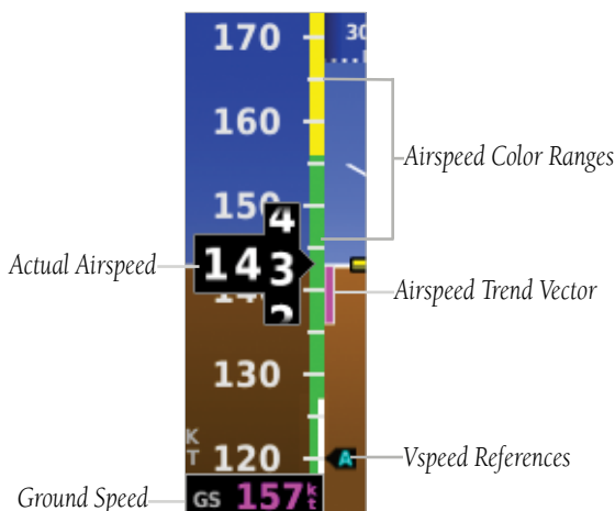
Figure 2-2 Airspeed Indicator
