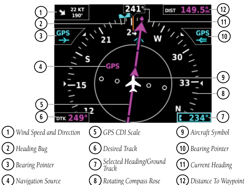
Figure 2-16 Horizontal Situation Indicator (HSI) - Expanded
