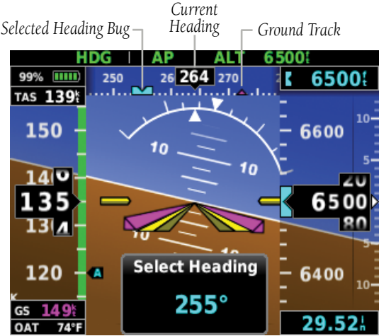
Figure 2-12 PFD Page - Selected Heading
