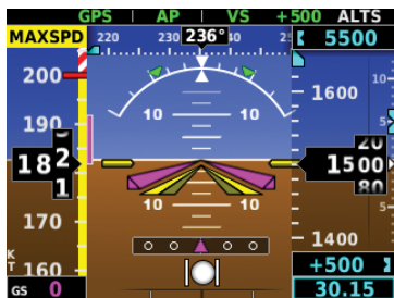
Figure 3-24 MAXSPD Alert
