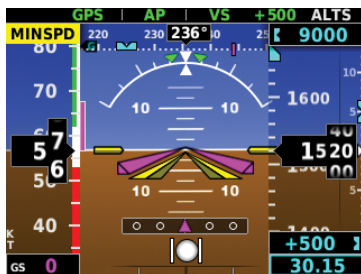
Figure 3-25 MINSPD Alert
