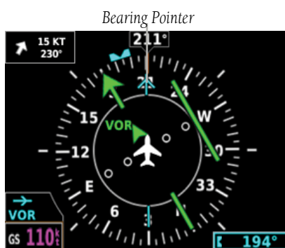
Figure 2-18 VOR Source Bearing Pointer
