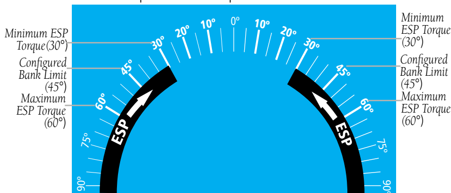
Figure 3-29 ESP Roll Operating Range When Engaged (Force Increases as Roll Increases & Decreases as Roll Decreases)
