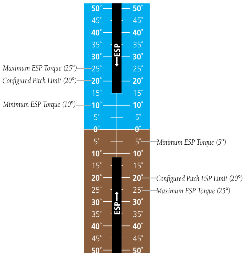
Figure 3-30 ESP Pitch Operating Range When Engaged (Force Increases as Pitch Increases & Decreases as Pitch Decreases)
