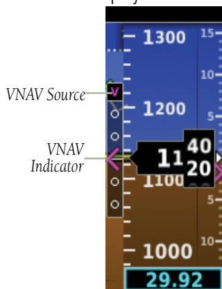
Figure 2-28 VNAV Indicator - PFD
