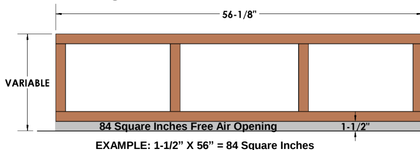
EXAMPLE 2: FRONT VIEW
