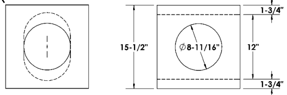
Z58FS Firestop - Hole may need to be elongated to due to ceiling angle. Trim to 12\"/>
