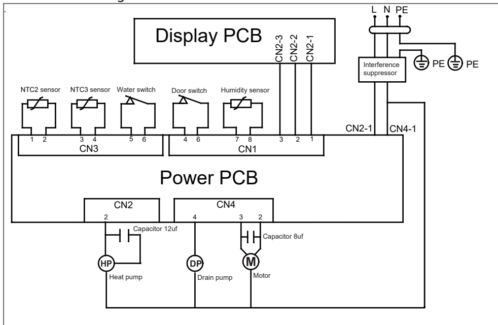
Electric circuit diagram HD90-A2979:
