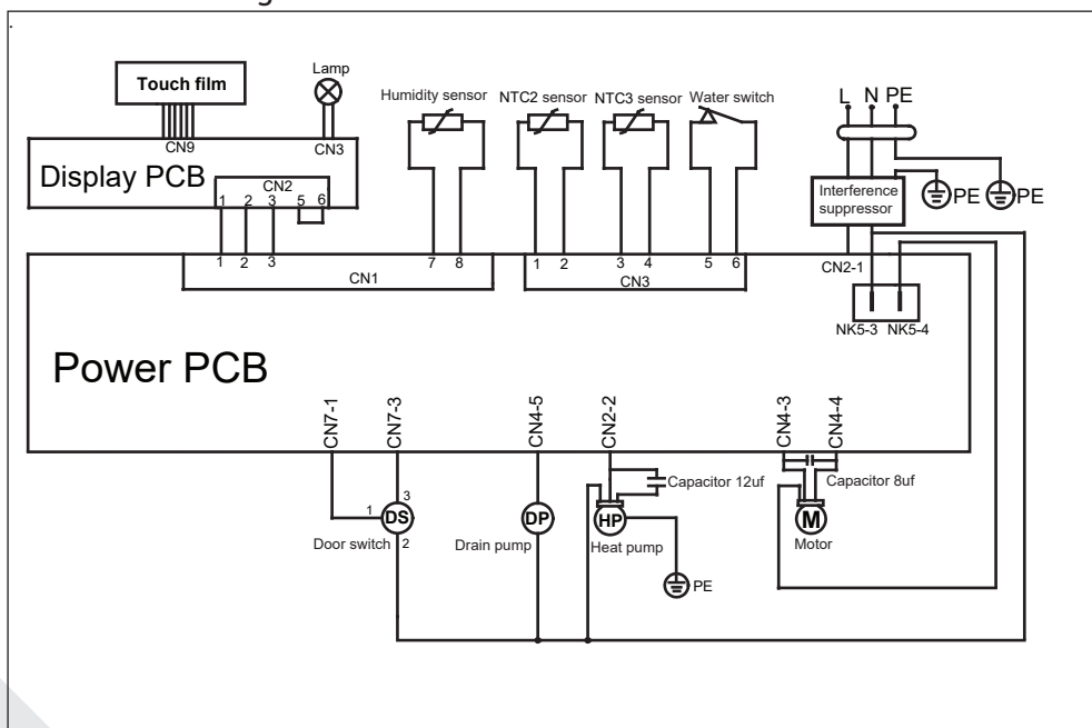
Electric circuit diagram HD100-A2979:
