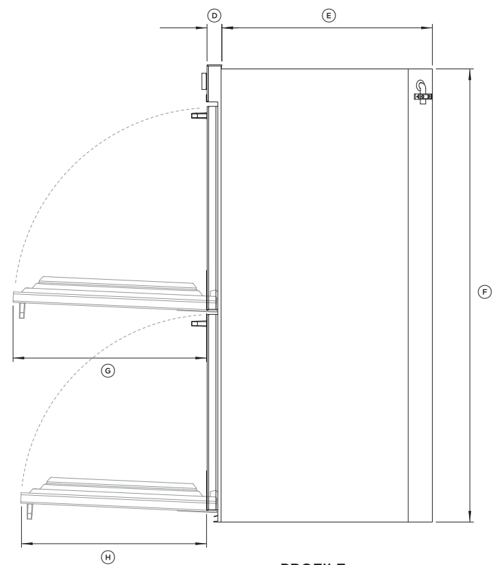
PROFILE
