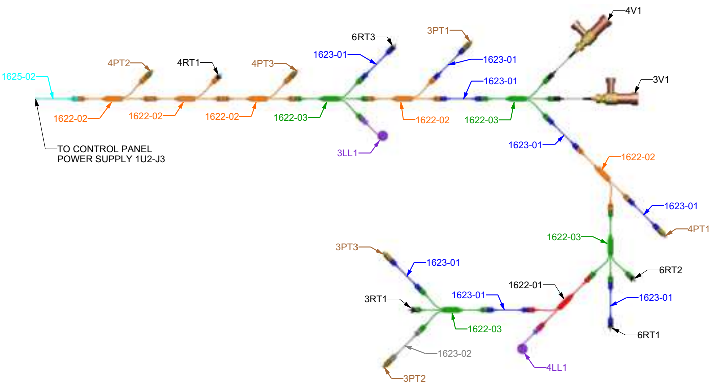
Figure 44. Global harness wiring diagram — 2 compressor unit, 21 foot base
