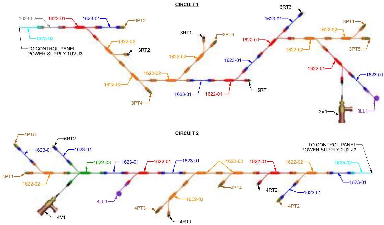
Figure 52. Global harness wiring diagram — 4 compressor unit, 3-pass, 39 foot base
