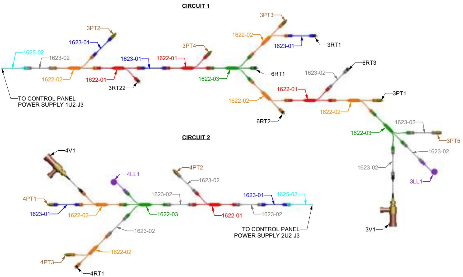
Figure 49. Global harness wiring diagram — 3 compressor unit, 2-pass, 39 foot base
