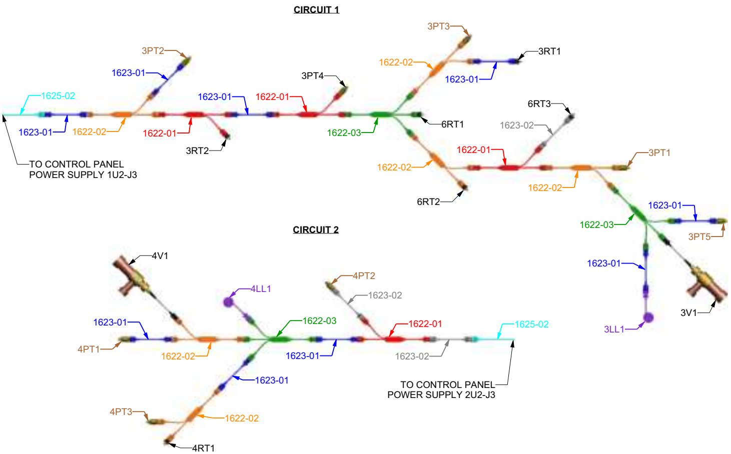
Figure 47. Global harness wiring diagram — 3 compressor unit, 2-pass, 36 foot base
