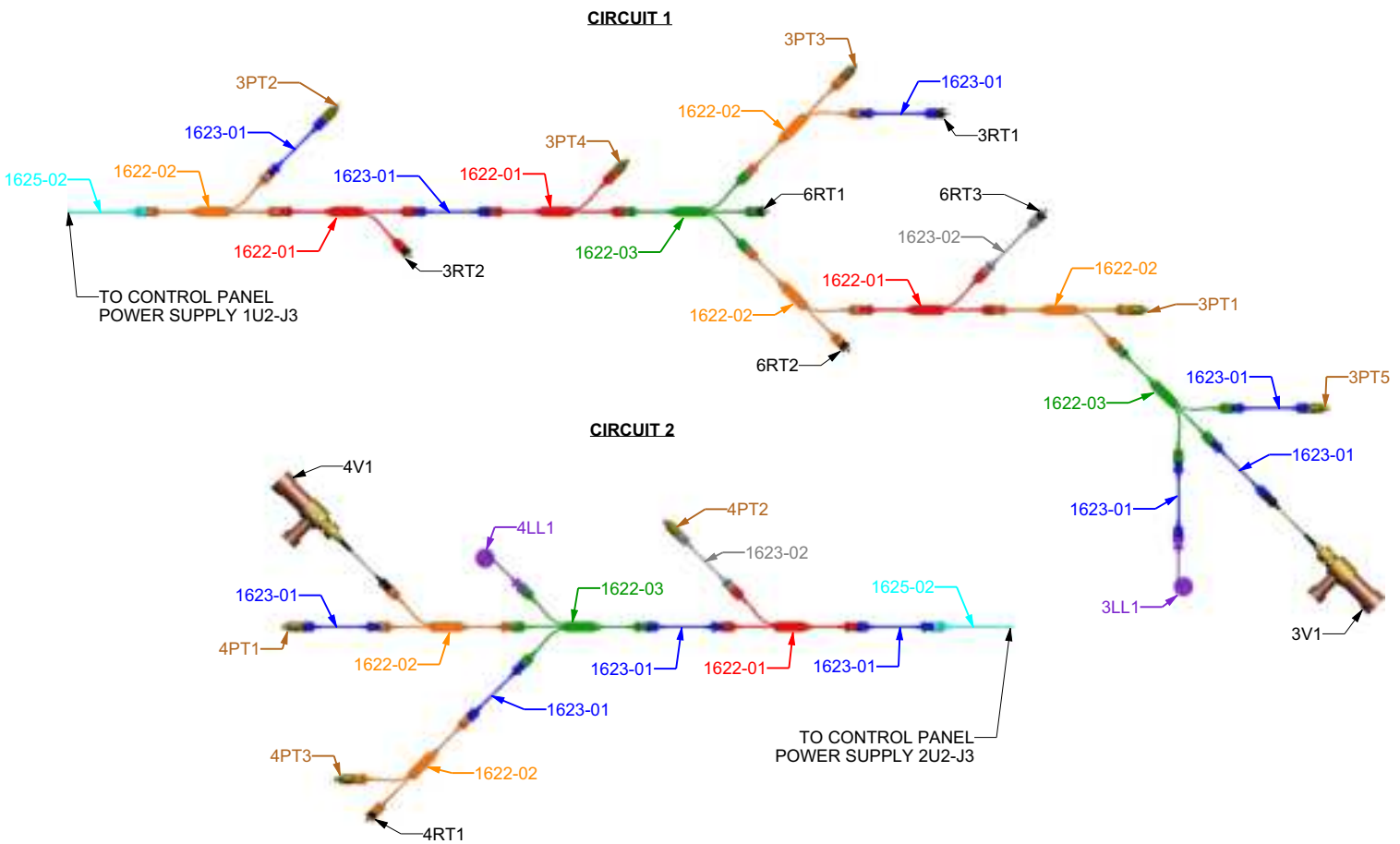
Figure 45. Global harness wiring diagram — 3 compressor unit, 2-pass, 30 foot base
