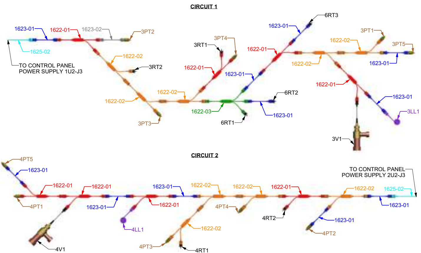
Figure 51. Global harness wiring diagram — 4 compressor unit, 2-pass, 39 foot base
