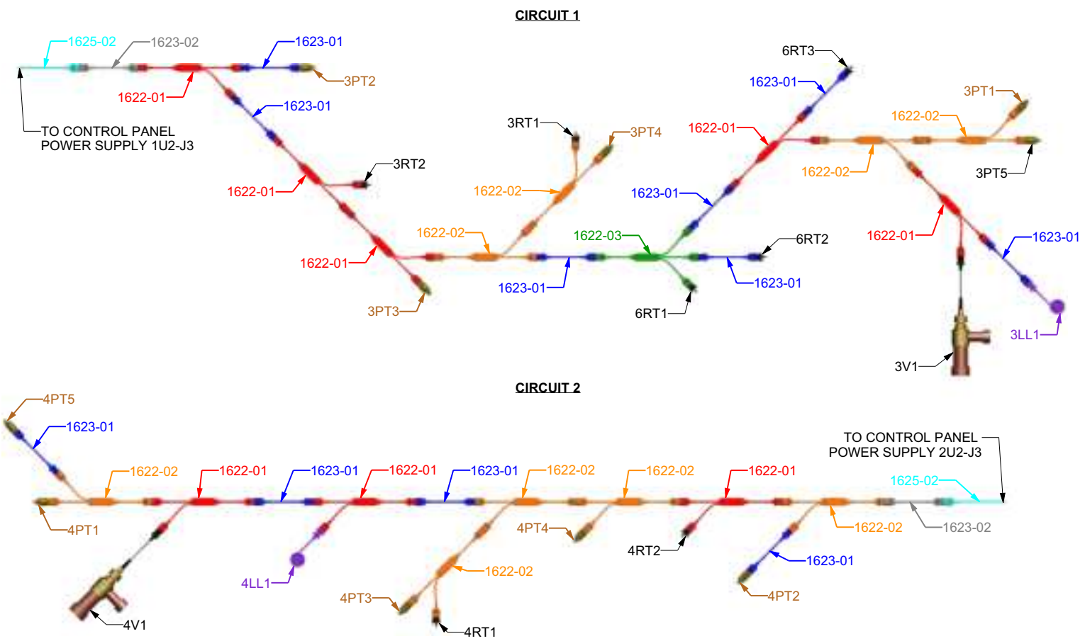
Figure 53. Global harness wiring diagram — 4 compressor unit, 2-pass, 45 foot base
