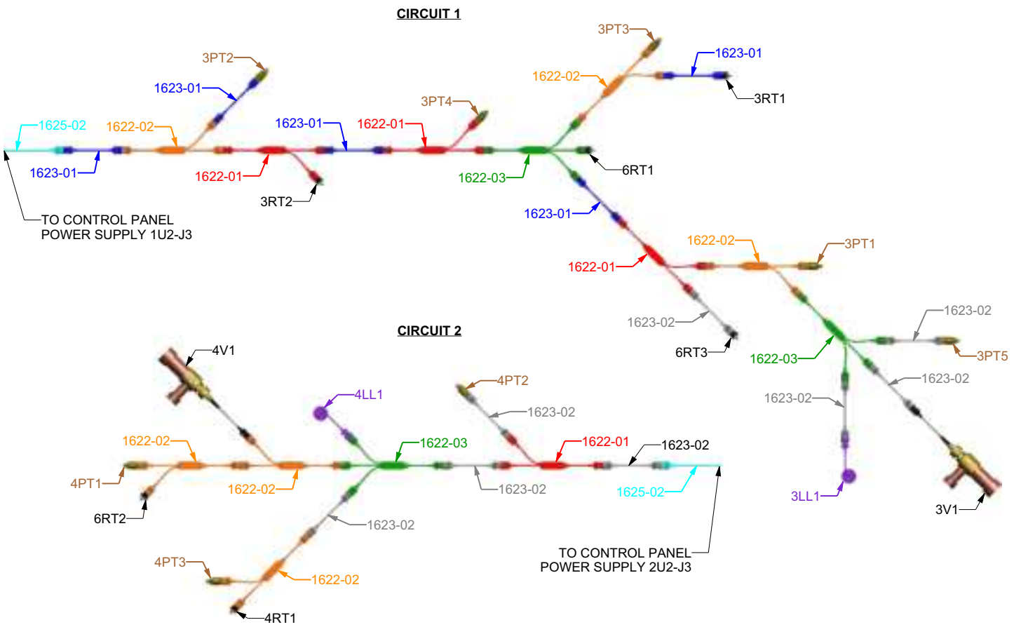
Figure 48. Global harness wiring diagram — 3 compressor unit, 3-pass, 36 foot base
