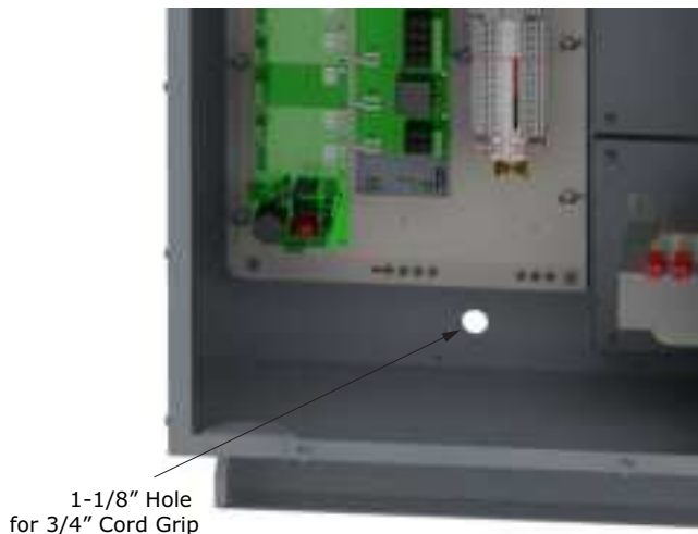
Figure 6. Hole for 3/4-inch cord grip
