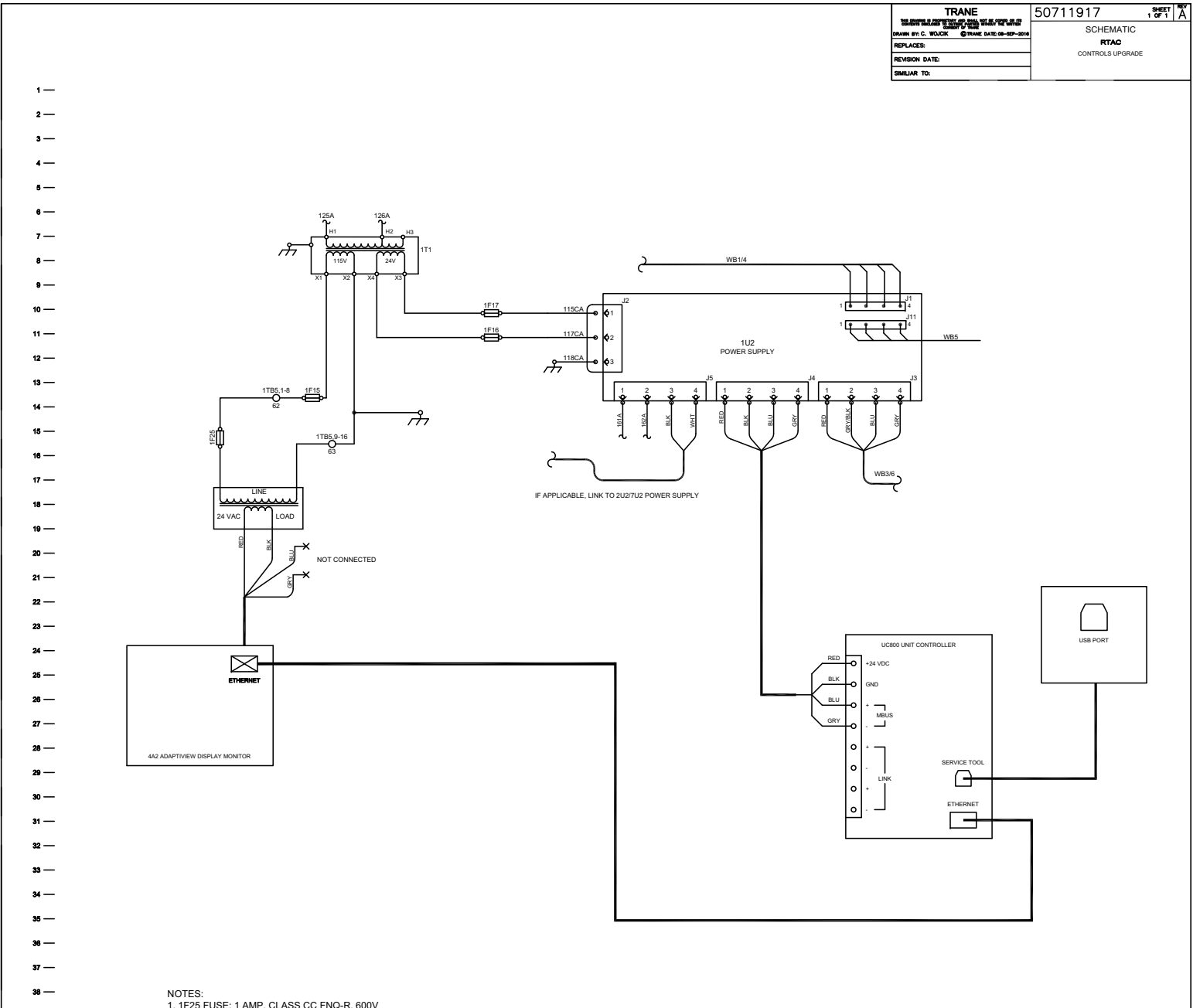
Figure 40. RTAC UC800/Tracer AdaptView upgrade schematic
