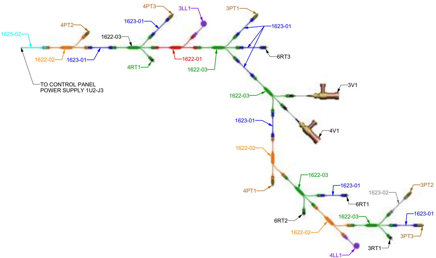
Figure 43. Global harness wiring diagram — 2 compressor unit, 18 foot base
