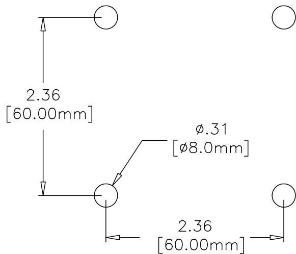
Figure 55. Arm mounting holes template, mm (in.)
