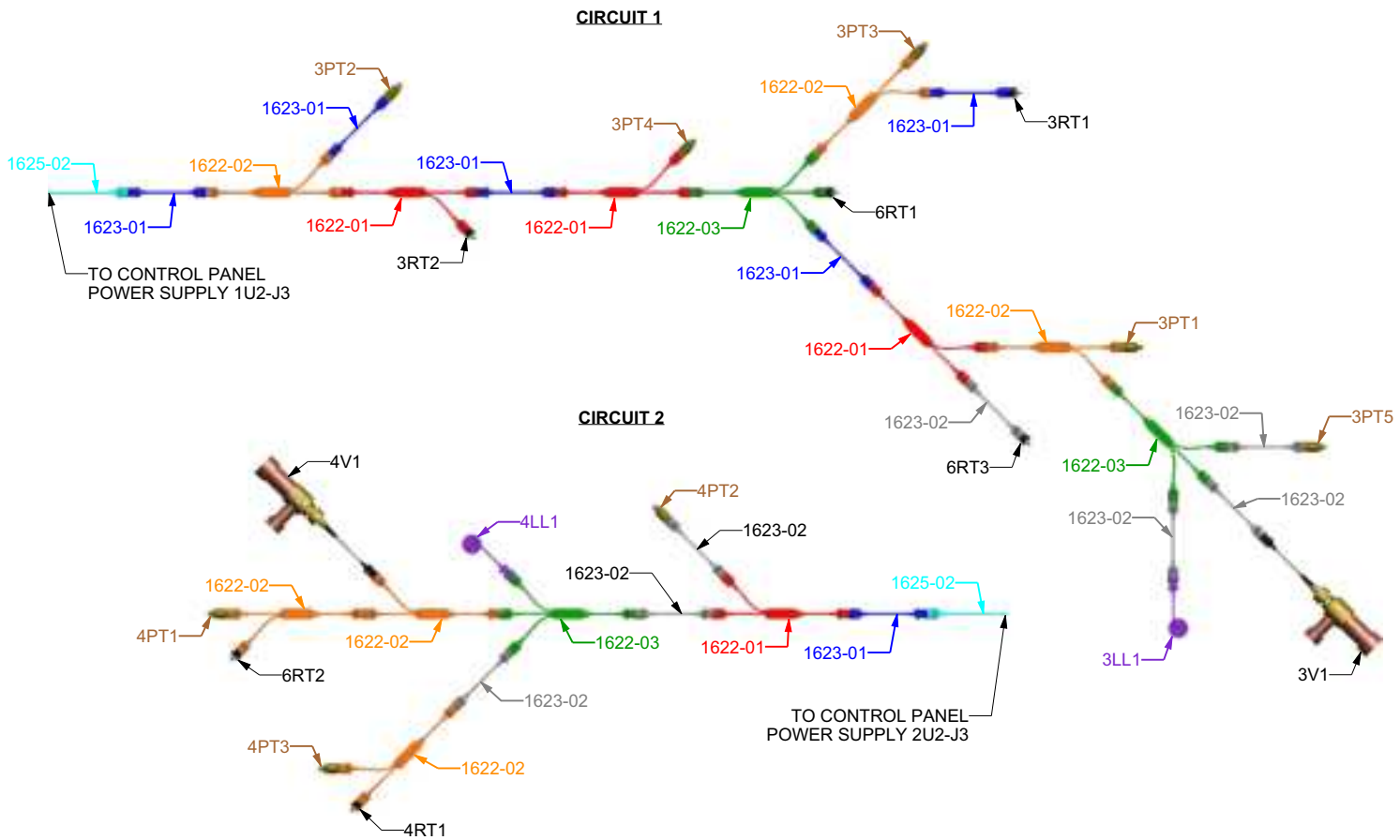
Figure 46. Global harness wiring diagram — 3 compressor unit, 3-pass, 30 foot base
