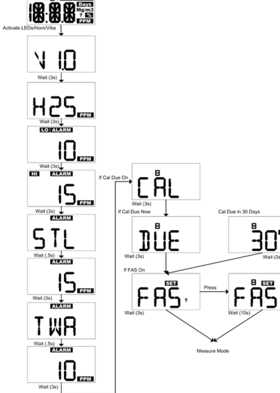
Figure 2-4. ALTAIR Pro Turn-ON Flow Chart
