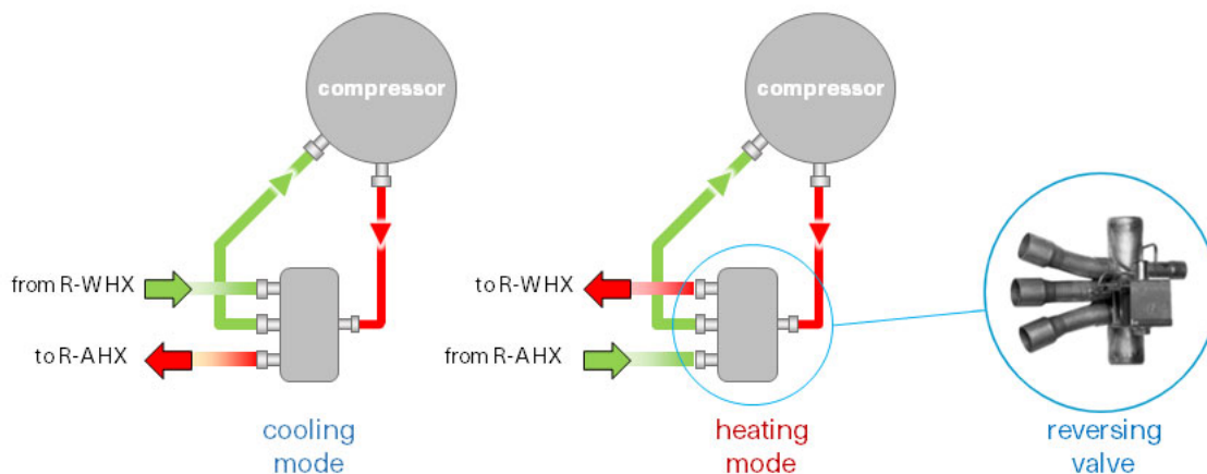
Figure 3. Reversing (four-way) valve
