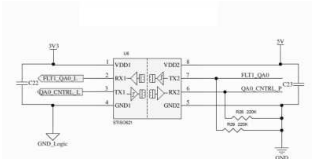
Figure 8. Isolator STISO621
