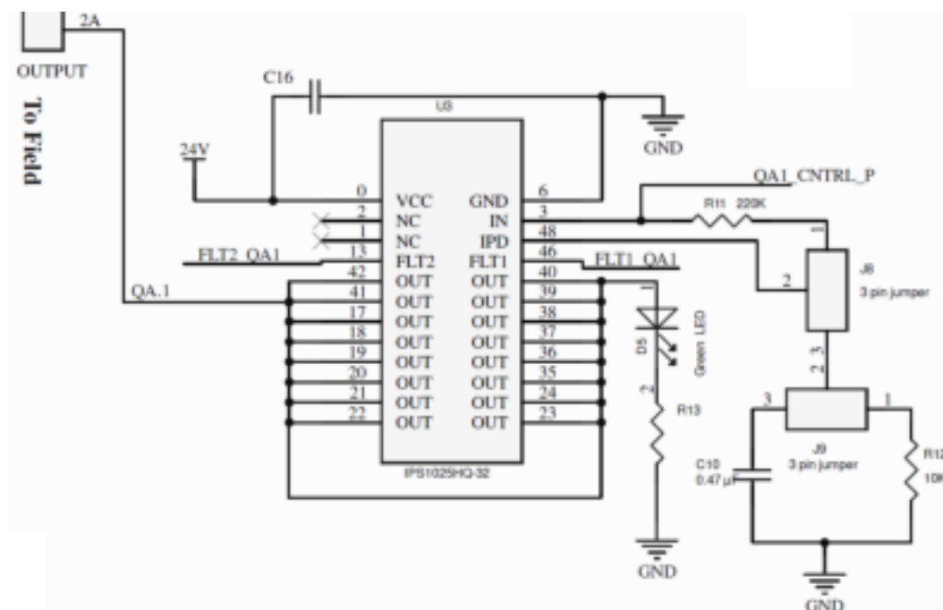
Figure 11. High-side switch
