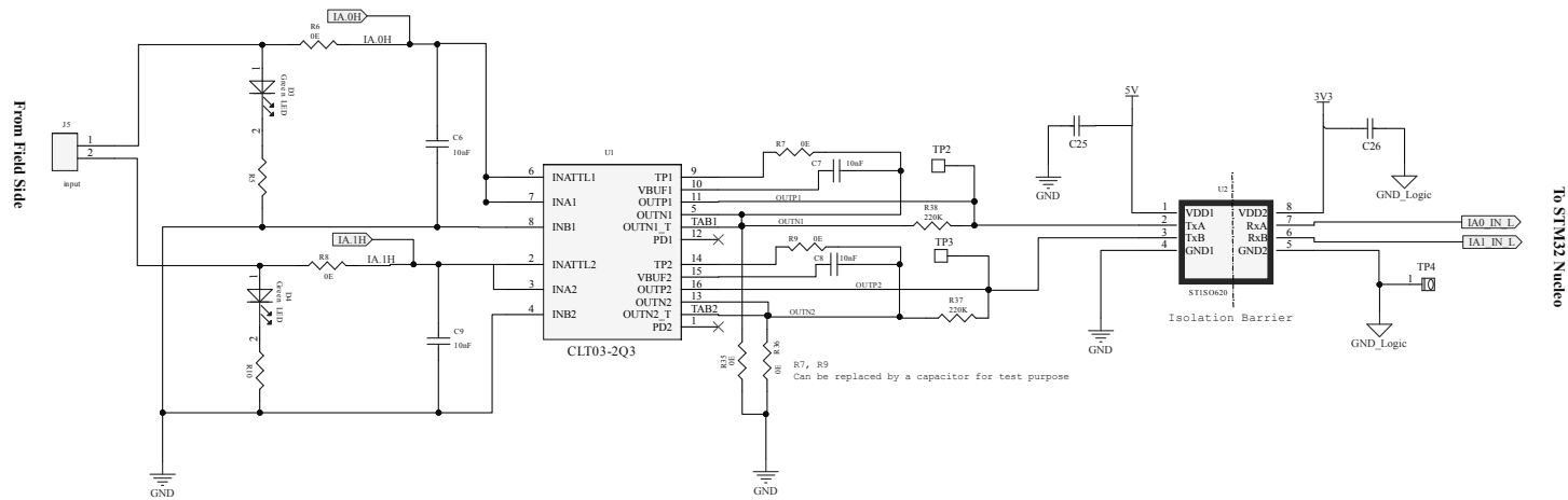
Figure 20. X-NUCLEO-ISO1A1 circuit schematic (2 of 4)
