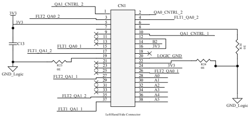
Figure 22. X-NUCLEO-ISO1A1 circuit schematic (4 of 4)
