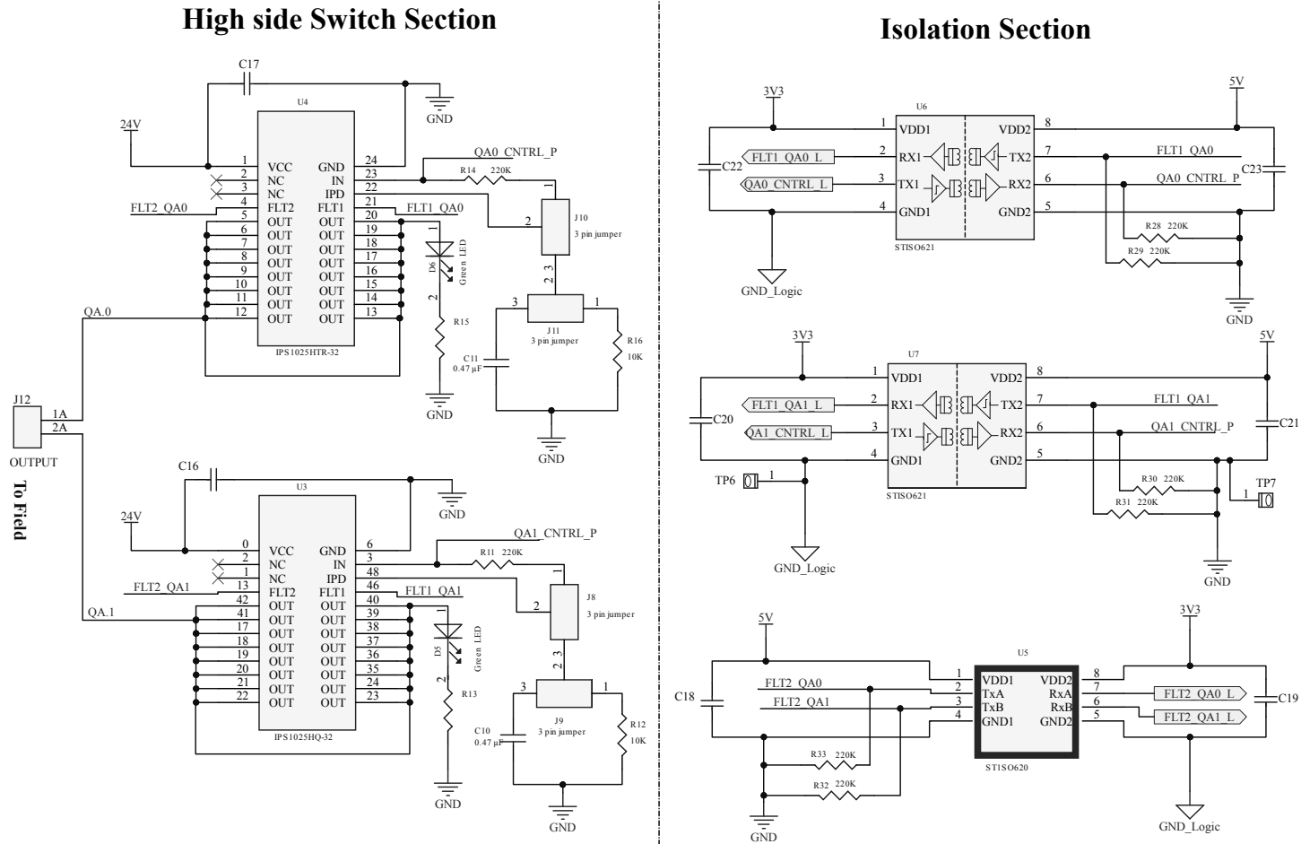
Figure 21. X-NUCLEO-ISO1A1 circuit schematic (3 of 4)
