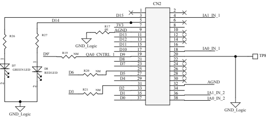
Figure 22. X-NUCLEO-ISO1A1 circuit schematic (4 of 4)
