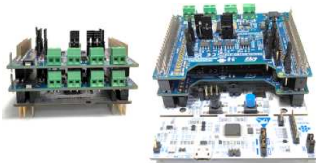
Figure 16. Stack of two X-NUCLEO boards
