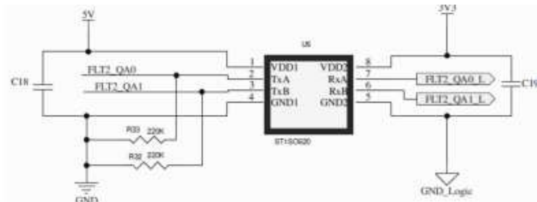
Figure 9. Isolator STISO620
