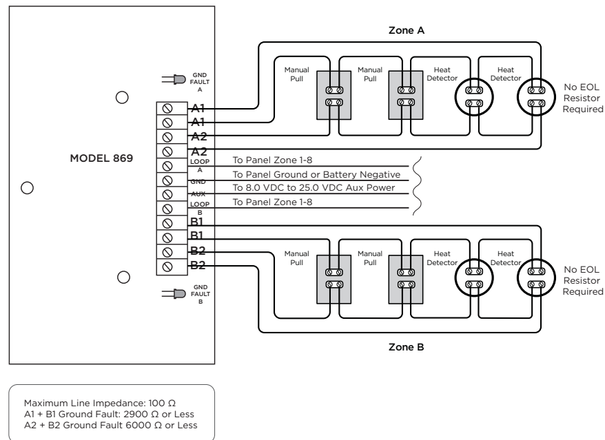
Figure 3: Wiring Diagram
