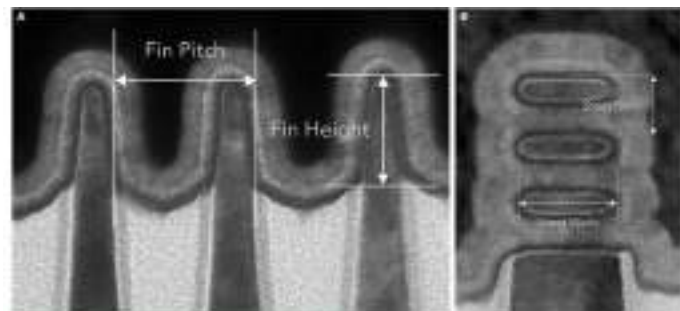
Figure 1: TEM Cross-sections of a FinFET and a Nanosheet In both cases the orientation is such that current flows into the page. (A) The scale of FinFET body controls the electrostatics, and the spacing between the fins determines the parasitic gate-drain capacitance. (B) In the nanosheet, the thickness of the sheet controls the electrostatics, and the sheet-sheet spacing, which is vertically oriented and created by spacers, determines the parasitic gate-drain capacitance.
