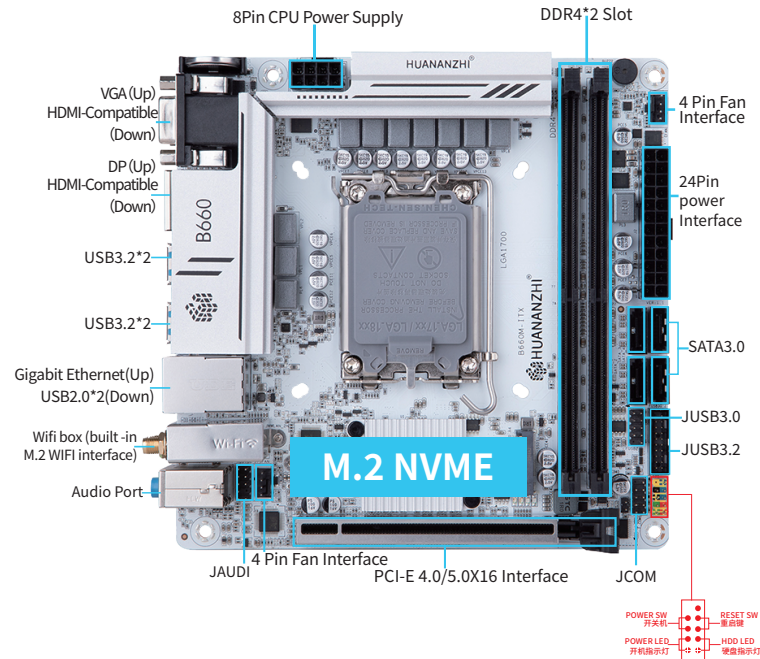
1-1 B660M-ITX MotherBoard Illustration
