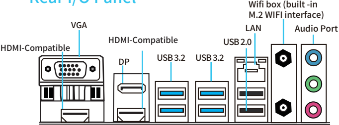
1-2 Overall Rear I/O Panel Display
