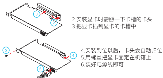
2-11 显卡安装
