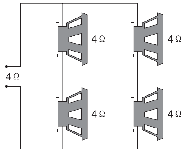
Series/parallel wiring
