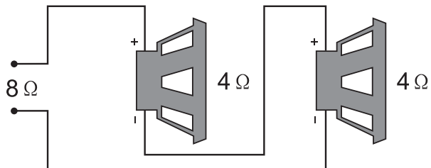
Series wiring
