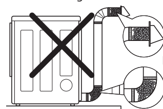
Excess or crushed transition duct
