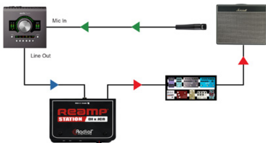
Reamping through pedals and an amp with the Reamp Station
