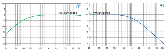
The frequency response of the high-pass and low-pass filters
