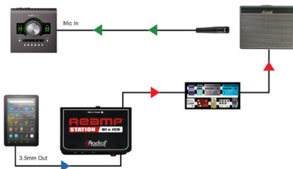
Reamping using a mobile device as the sound source
