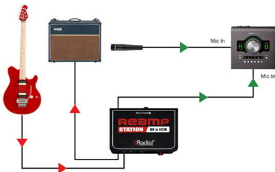
Recording your instrument with the Reamp Station
