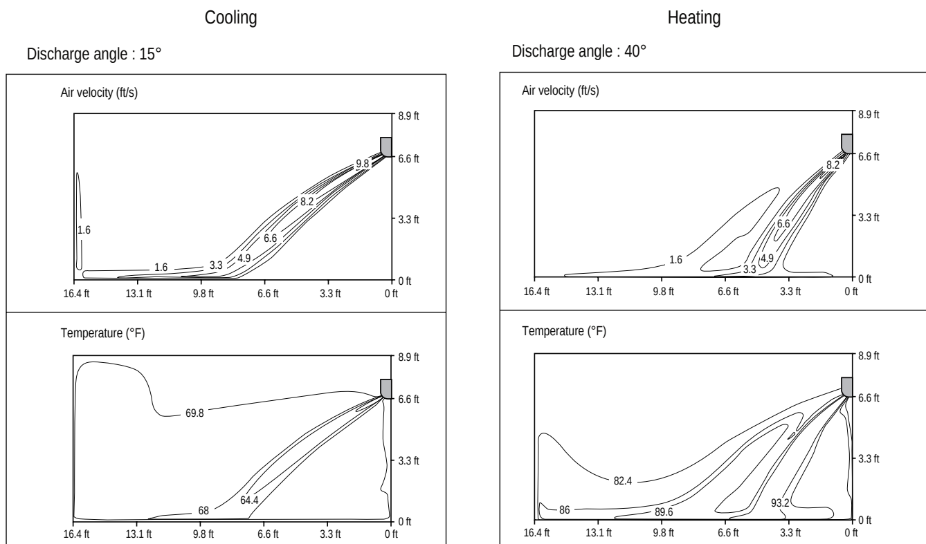
Figure 77: LMN158HVT Air Velocity and Temperature Distribution Charts.
