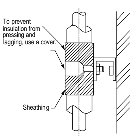
Figure 269: U-Bolt Support with an Insulated Pipe.
