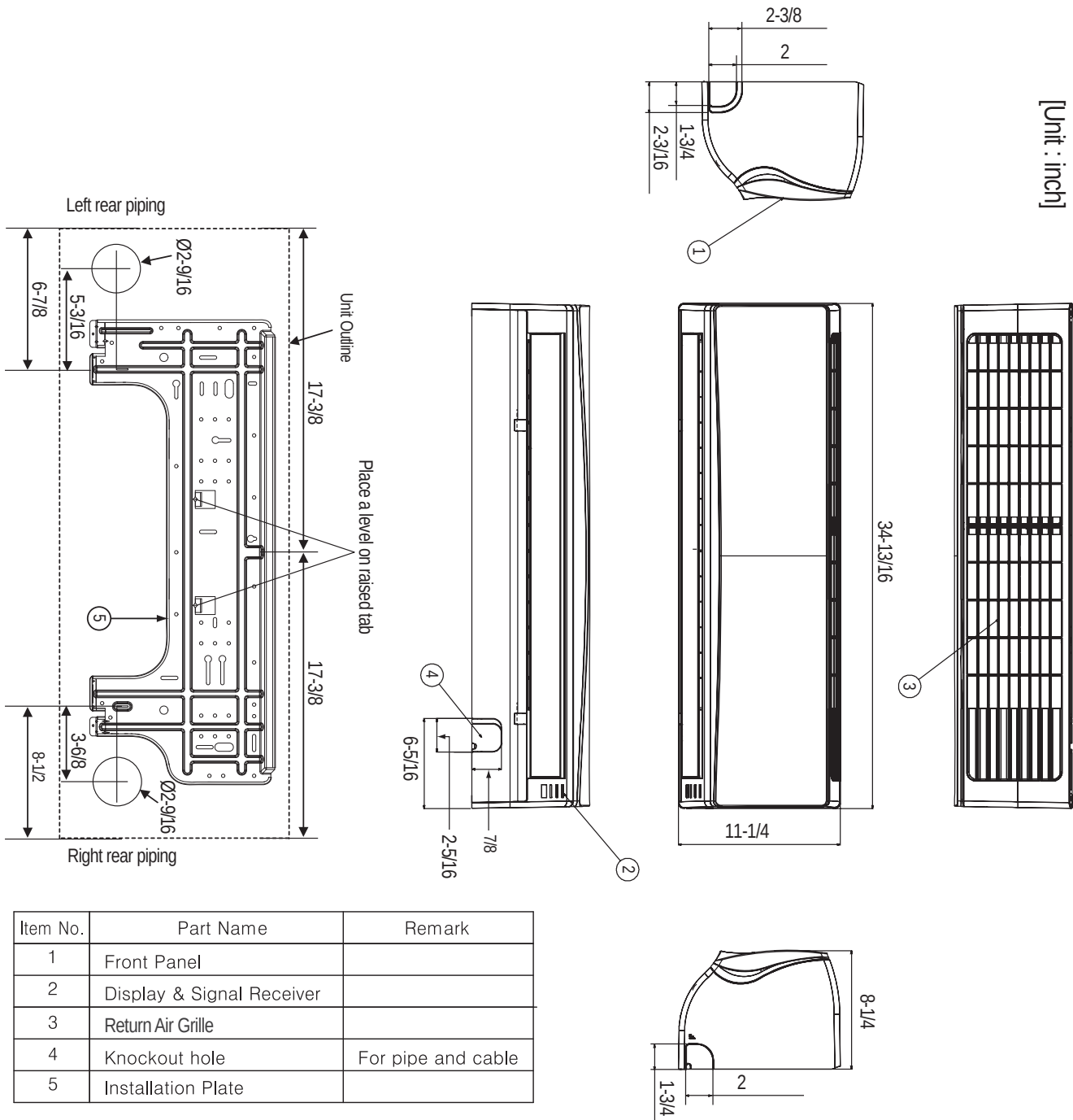
Figure 69: LSN090HSV4 and LSN120HSV4 Dimensions.
