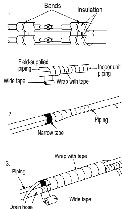
Figure 98: Insulating the Piping.
