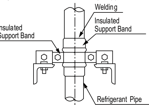
Figure 272: Two-Point Down-Stop Support.
