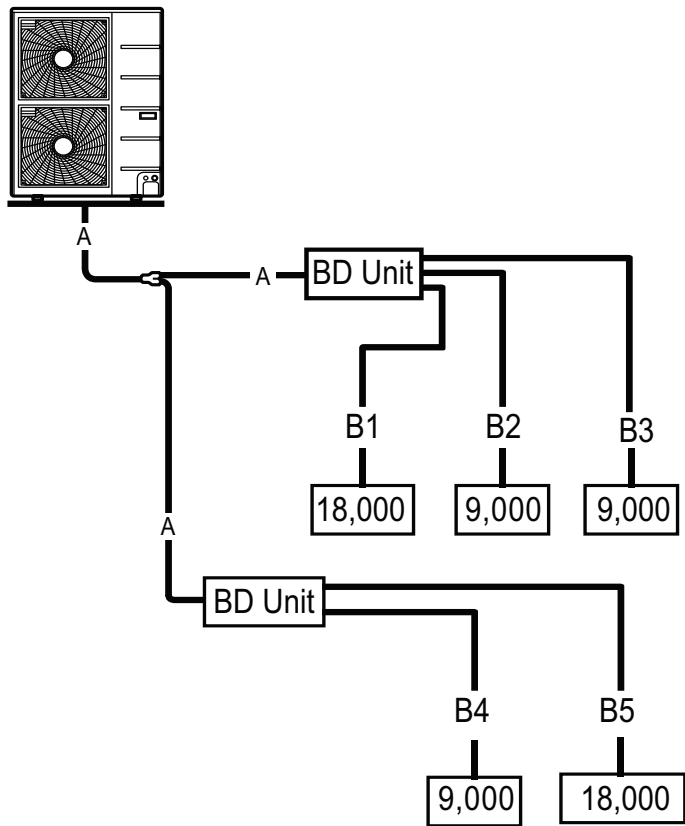
Figure 258: Multi F MAX Additional Refrigerant Charge Example.
