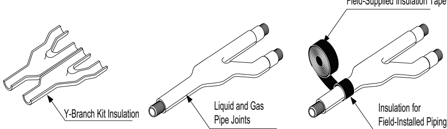
Figure 293: Y-Branch Insulation Jacket Diagram.
