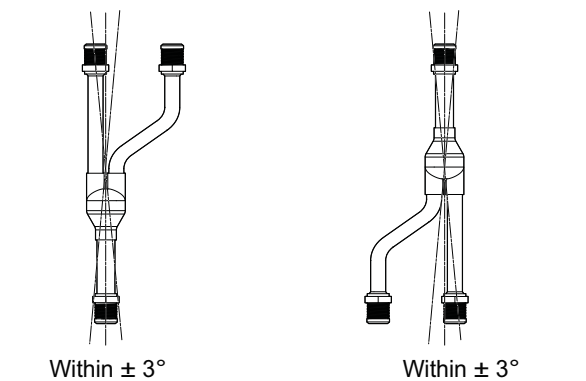
Figure 255: Y-branch Installation Alignment Specification.
