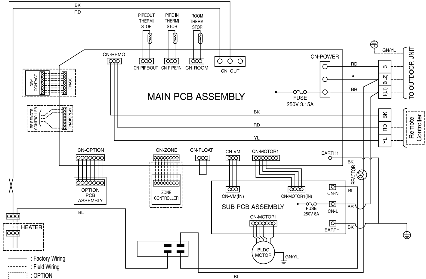
Figure 215: Multi F Vertical-Horizontal Air-Handling Indoor Unit Wiring Diagram.
