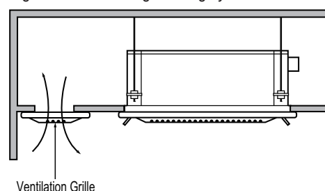
Figure 189: Installing in a Highly Humid Location.
