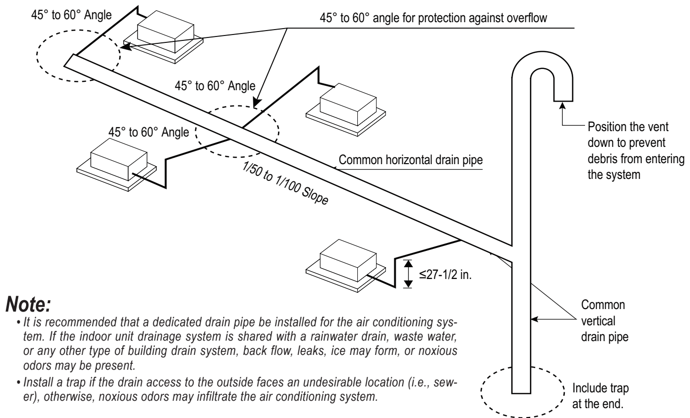
Figure 289: Example of a Common Indoor Unit Drainage System.
