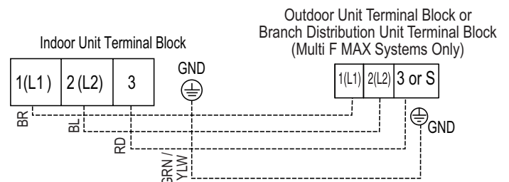
Figure 164: Indoor Unit to Outdoor Unit / Branch Distribution Unit (Multi F MAX systems only) Power Wiring / Communications Cable Connections.
