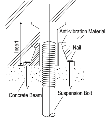
Figure 262: Pipe Hanger Details.
