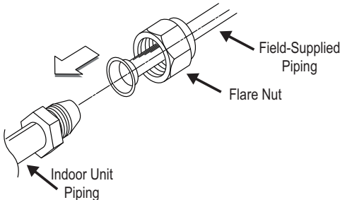
Figure 283: Flare Connection, Isometric View.
