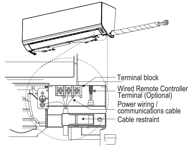
Figure 101: Connecting Power Wiring / Communications Cable.
