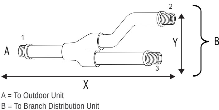
Figure 292: Y-Branch Dimensions Diagram.
