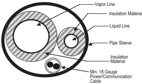
Figure 274: Typical Arrangement of Refrigerant Pipe and Cable(s) in a Utility Conduit.
