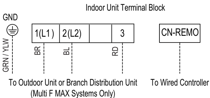
Figure 107: Wired Controller Connection on Indoor Unit Terminal Block—LSN180HSV4 and LMN248HVT Models.
