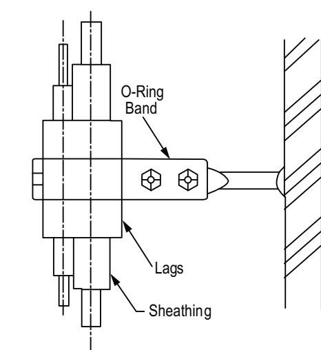
Figure 270: O-Ring Band Support with an Insulated Pipe.
