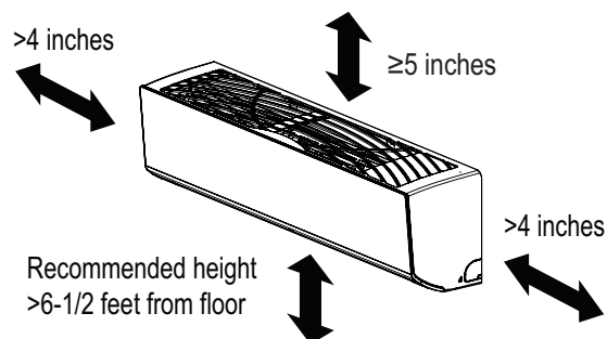
Figure 85: Minimum Clearance Requirements.
