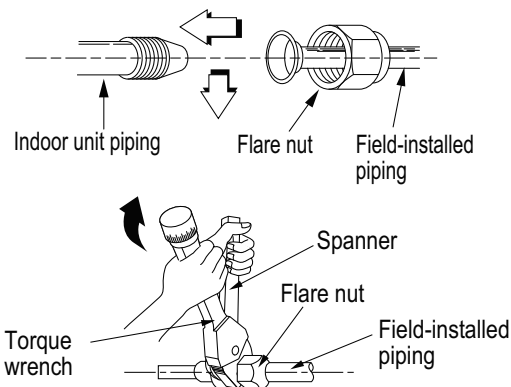
Figure 96: Indoor Unit to Field-Installed Piping Connection.
