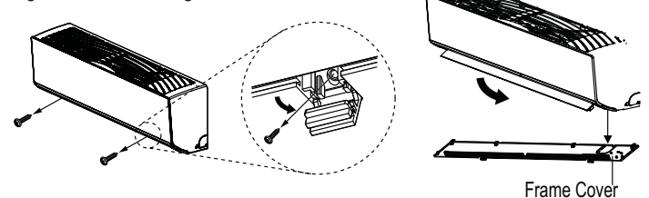
Figure 17: Removing the Frame Cover.
