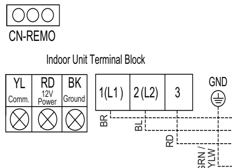
Figure 168: Wired Controller Connections on the Indoor Unit Terminal Block.
