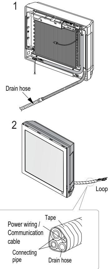
Figure 50: Preparing the Refrigerant / Drain Connections.
