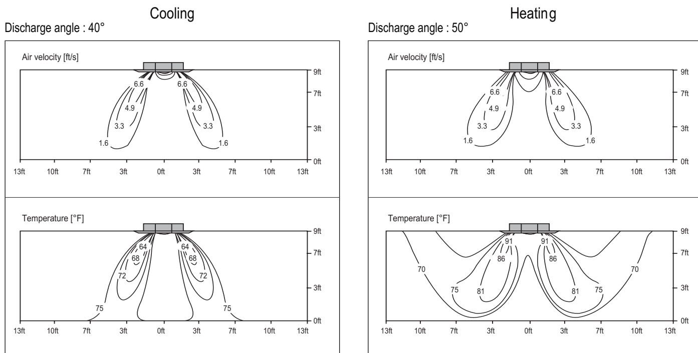
Figure 185: LMCN185HV Air Velocity and Temperature Distribution Charts.
