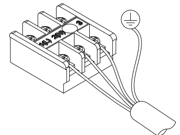
Figure 297: Close up of the Indoor Unit Terminal Block.
