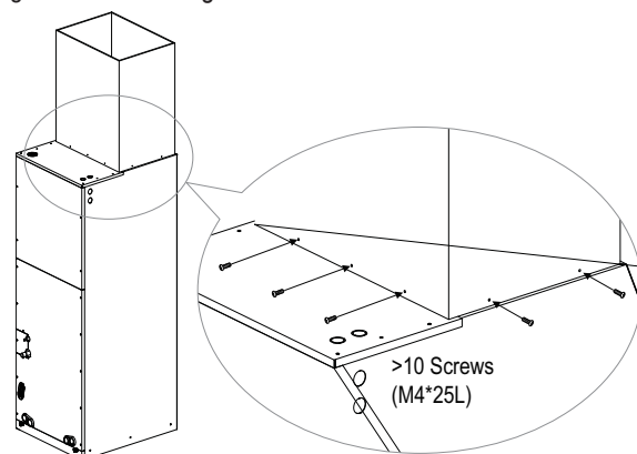
Figure 221: Securing the Ducts to the Unit.
