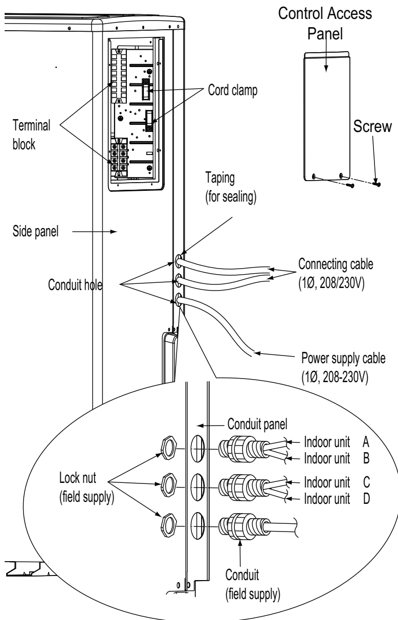
Figure 300: Example of Power Wiring and Communications Cable Terminations.
