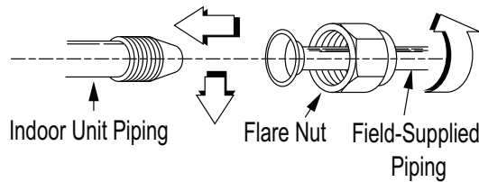
Figure 284: Flare Connection, Side View.
