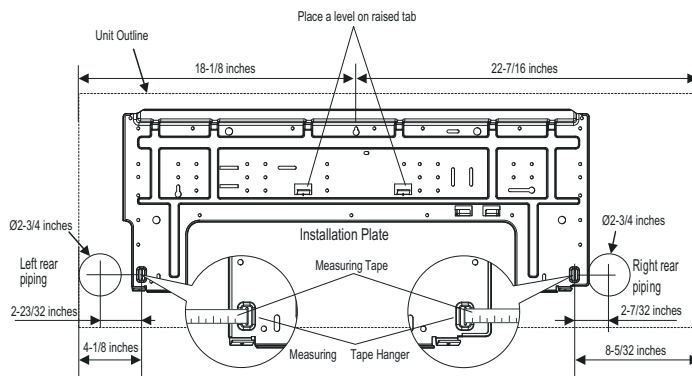
Figure 88: Installation Plate for LSN180HSV4 and LMN248HVT Units.
