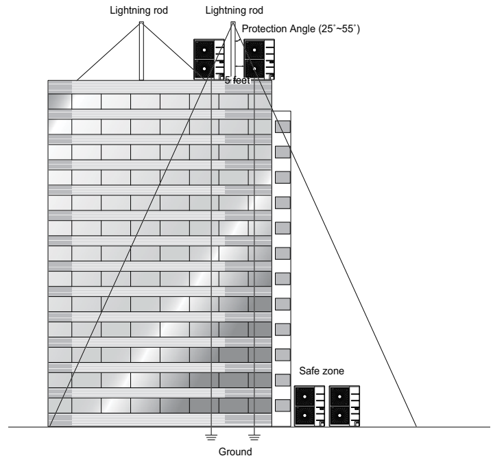
Figure 247: Lightning Protection Diagram.
