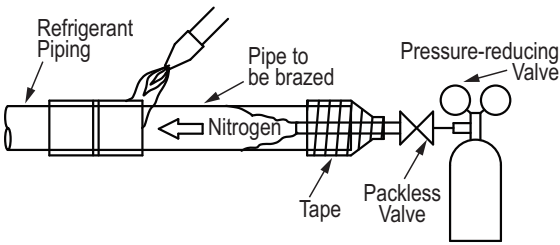
Figure 282: Refrigerant Pipe Brazing.
