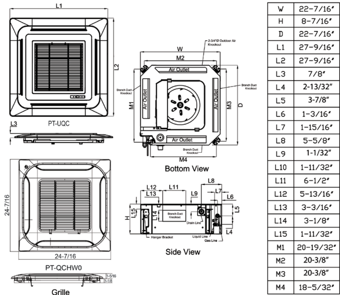
Figure 177: LMCN077HV, LCN097HV4, and LCN127HV4 Dimensions.
