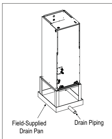
Figure 222: Vertical Installation Drain System.
