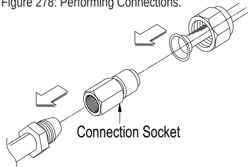
Figure 278: Performing Connections.
