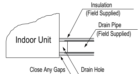
Figure 128: Drain Connection.
