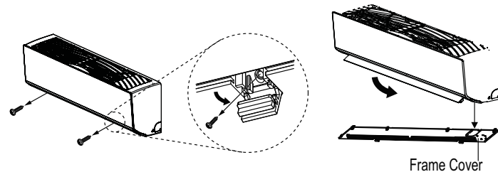
Figure 92: Removing the Frame Cover.
