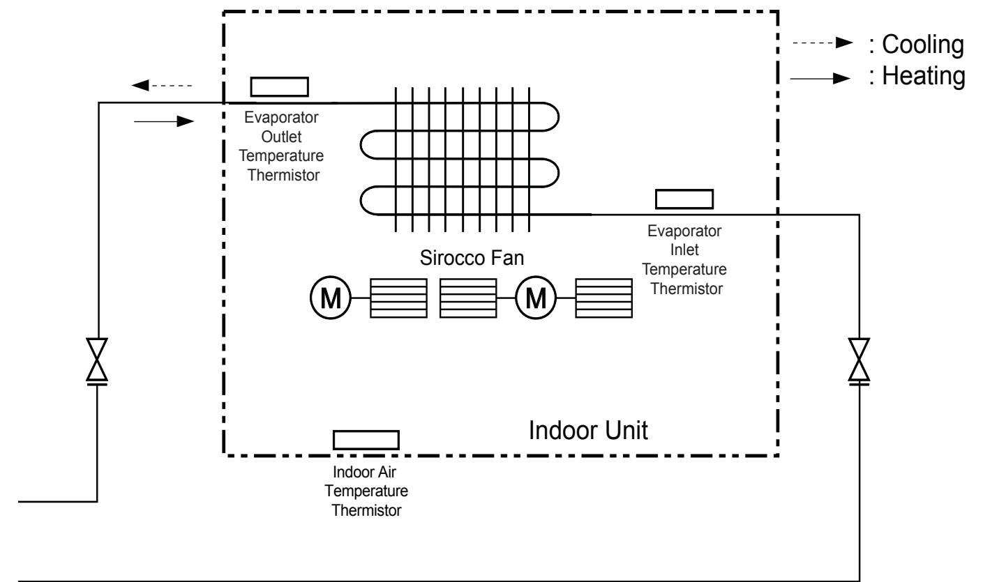
Figure 119: LDN127HV4 and LMDN186HV Refrigerant Flow Diagram.
