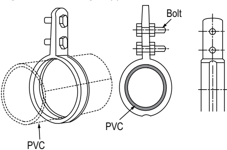
Figure 267: O-Ring Support with Insulation.
