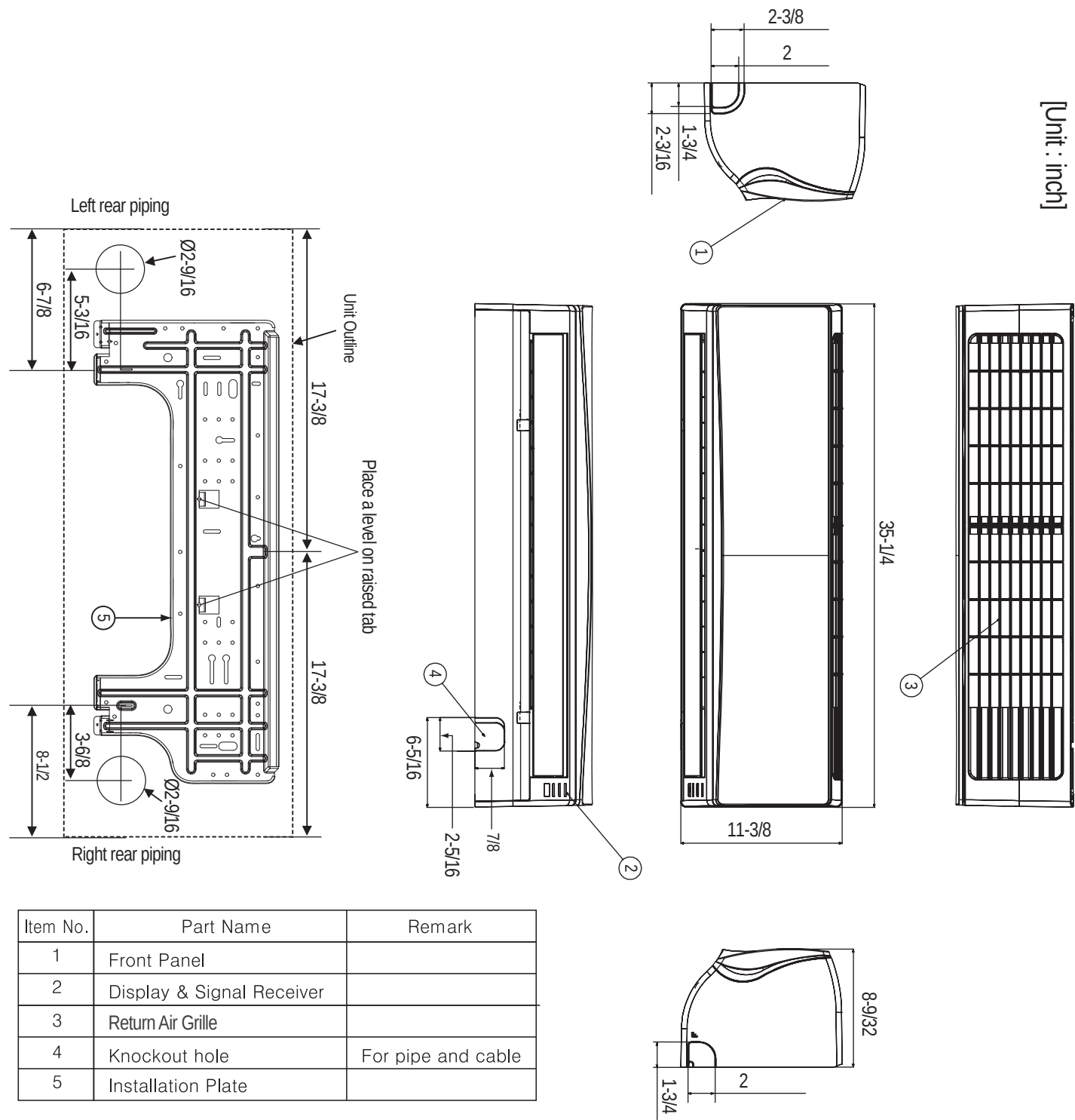
Figure 68: LMN078HVT and LMN158HVT Dimensions.
