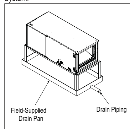
Figure 223: Horizontal Installation Drain System.
