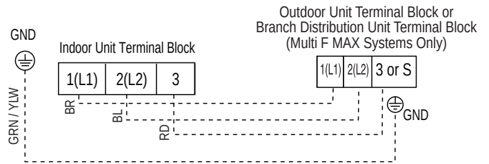
Figure 102: Simplified View of Indoor Unit to Outdoor Unit / Branch Distribution Unit Terminal Connections—LMN078HVT, LSN090HSV4, LSN120HSV4 and LMN158HVT.
