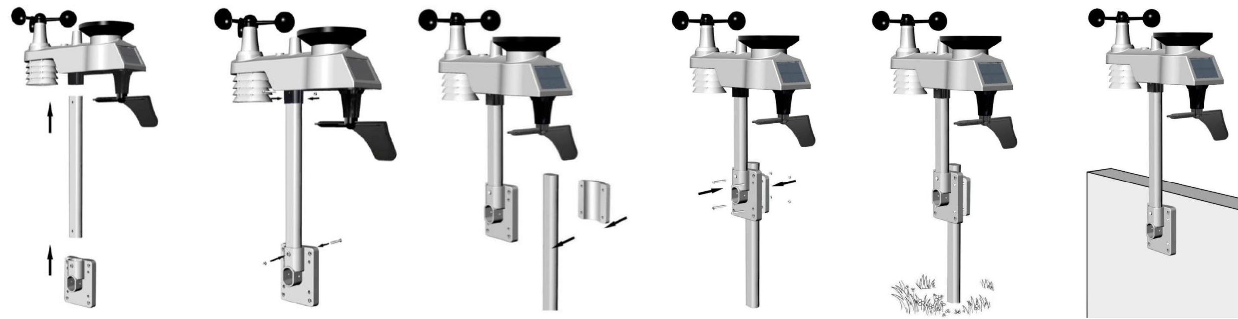
Vertical Installation
