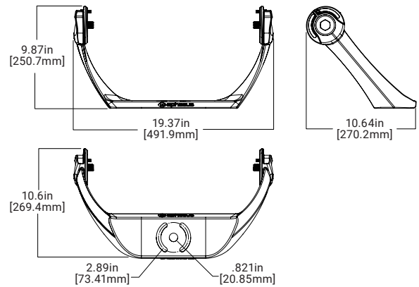
YOKE MOUNT
