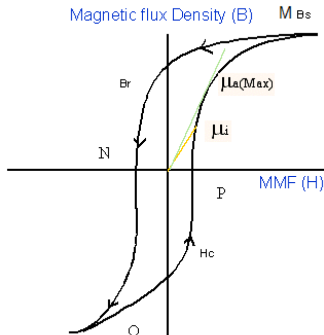
Figure 18: B-H curve
