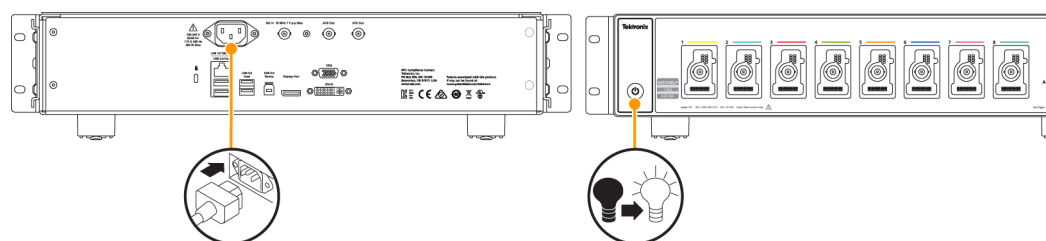
Figure 3: MSO58LP power cord connector and power standby switch
