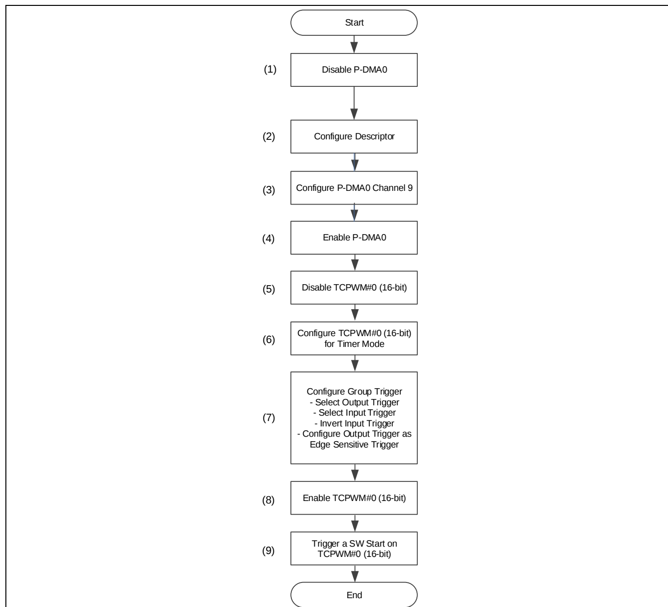
Figure 11 Example of setting for group trigger in CYT2B7 series
