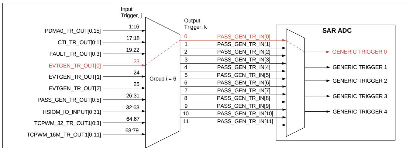
Figure 4 Trigger routing between TCPWM 16-bit Motor and Generic Trigger 2 in ADC of CYT2B7 series
