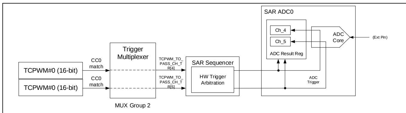
Figure 17 Example of one-to-one trigger in CYT2B7 series
