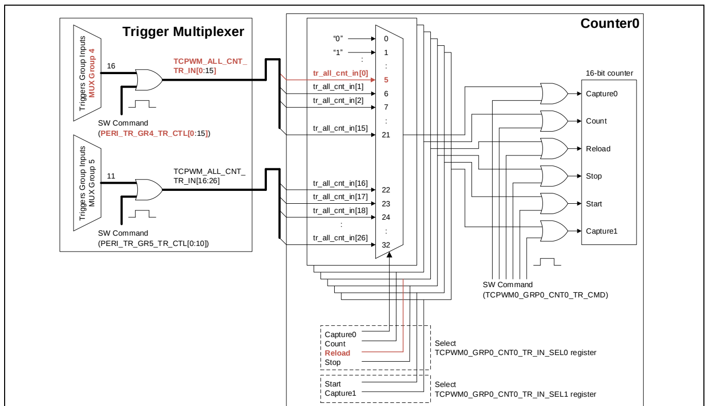
Figure 22 Connection between MUX Group 4 and TCPWM 16-bit motor control counter
