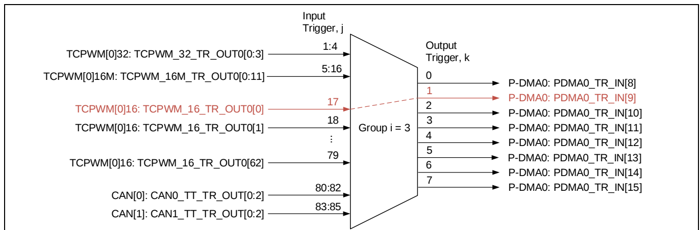
Figure 12 Trigger routing between 16-bit TCPWM and P-DMA0 of CYT2B7 series
