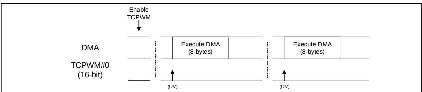
Figure 10 Example operation: Triggering P-DMA transfer by TCPWM counter overflow
