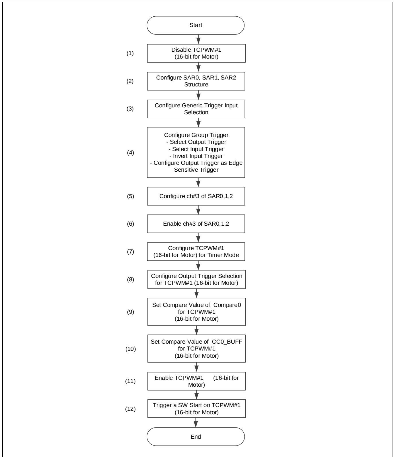
Figure 15 Setting for ADC generic trigger input and group trigger in CYT2B7 series
