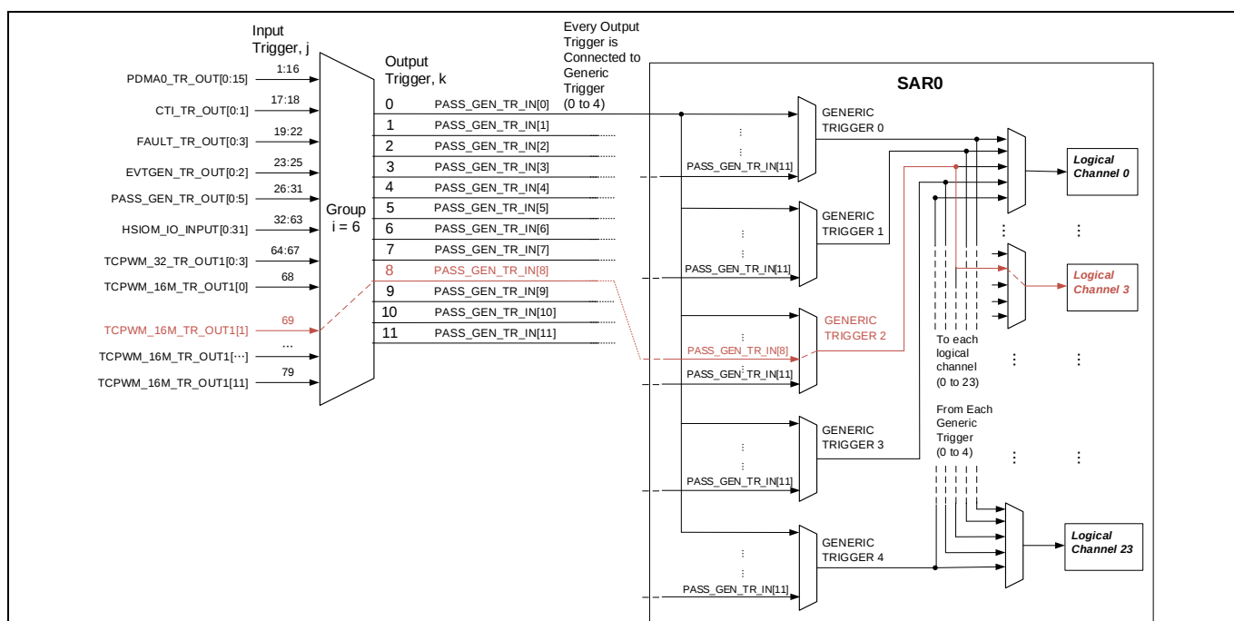
Figure 16 Trigger routing between TCPWM 16-bit motor and generic trigger 2 in SAR0 unit of CYT2B7 series
