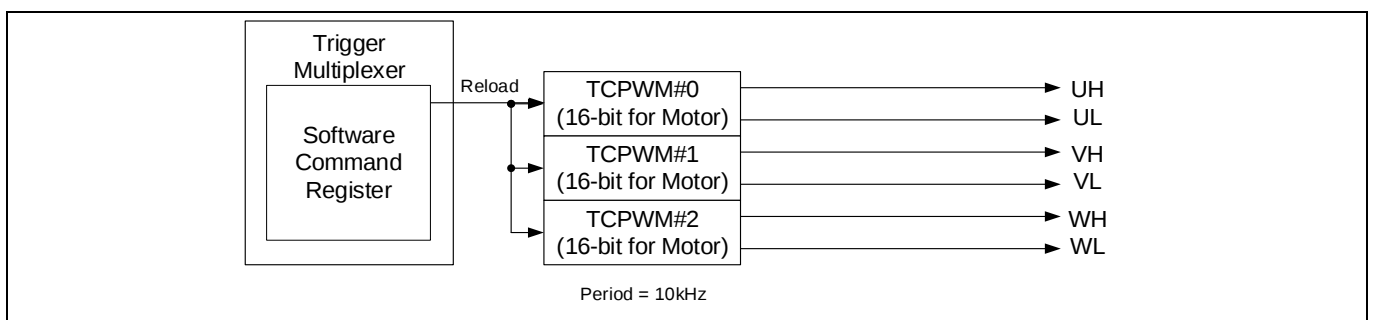
Figure 20 Example of SW trigger in CYT2B7 series
