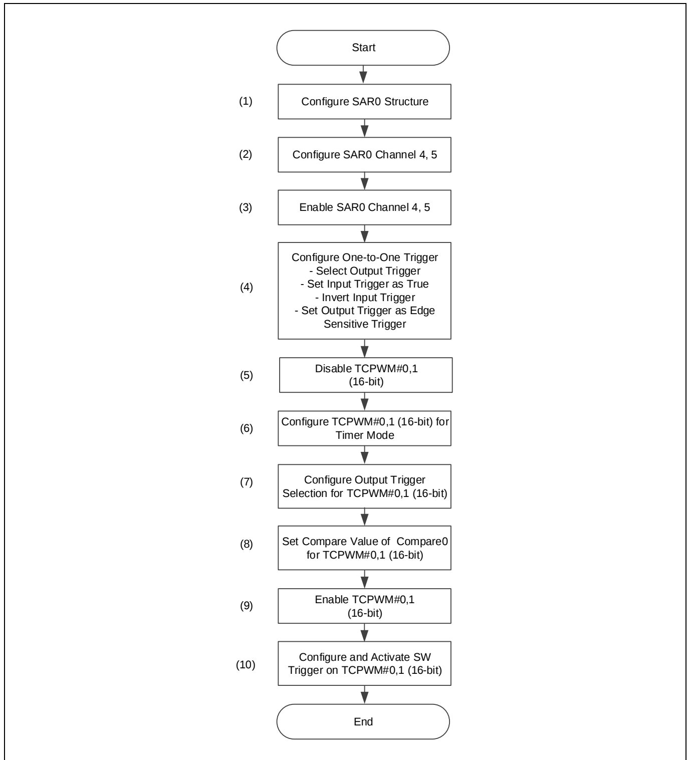
Figure 19 Setting for one-to-one trigger in CYT2B7 series
