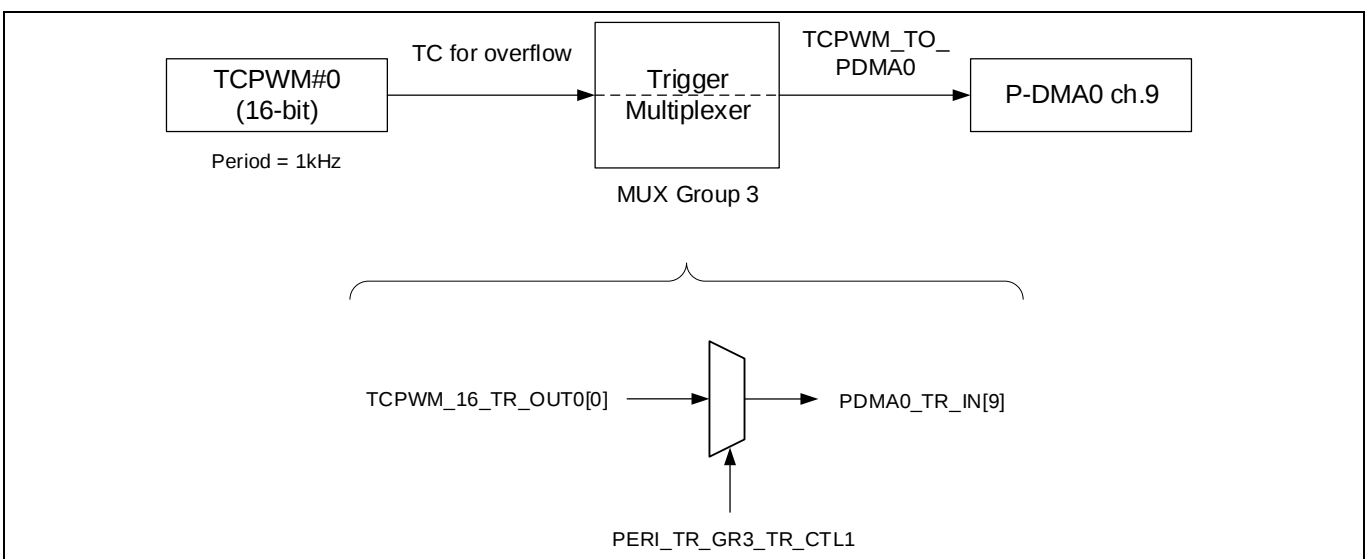
Figure 9 Example of group trigger in CYT2B7 series
