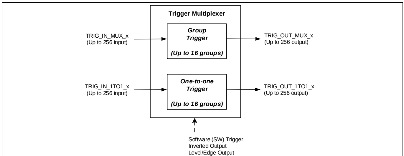
Figure 1 Trigger multiplexer block diagram
