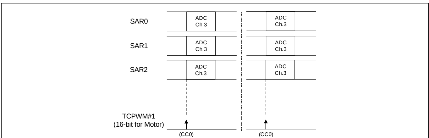
Figure 14 Example operation: Simultaneous ADC conversion on three SARs by single TCPWM timer
