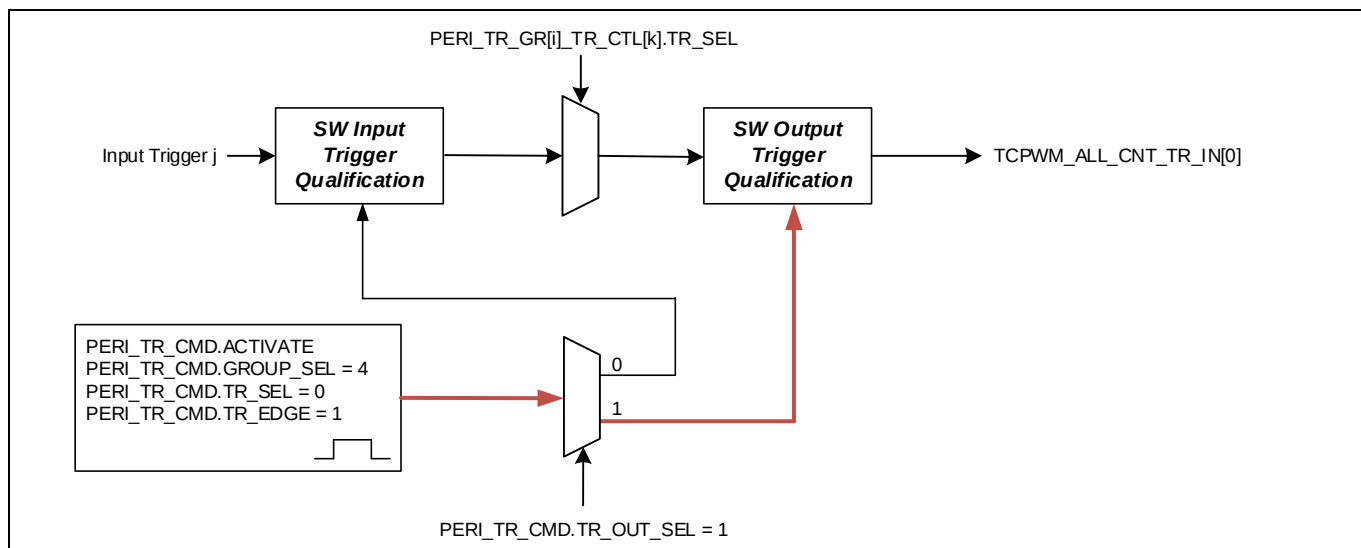
Figure 24 SW triggering TCPWM counter
