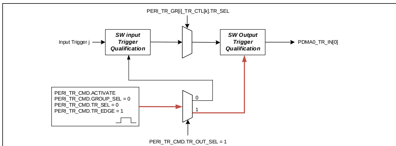
Figure 8 P-DMA0 data transfer start by SW
