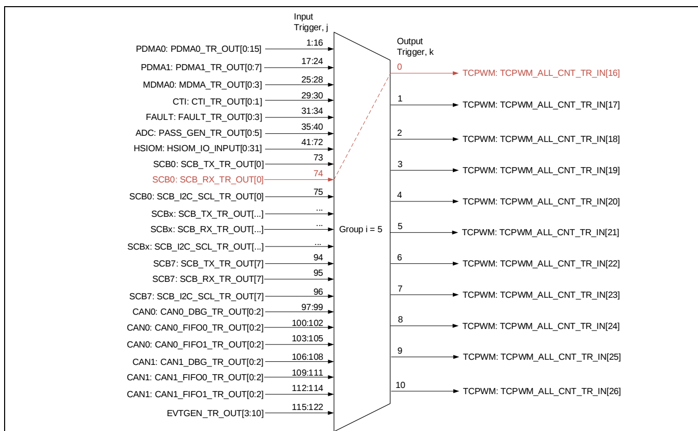
Figure 3 Trigger routing between 16-bit TCPWM and P-DMA0 of CYT2B7 series
