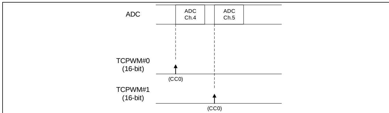
Figure 18 Example operation: Triggering ADC conversion by TCPWM timer
