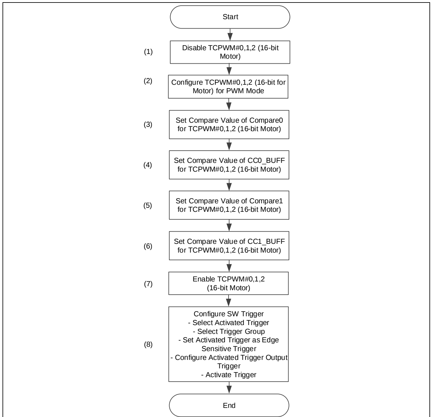
Figure 23 Setting for one-to-one trigger in CYT2B7 series
