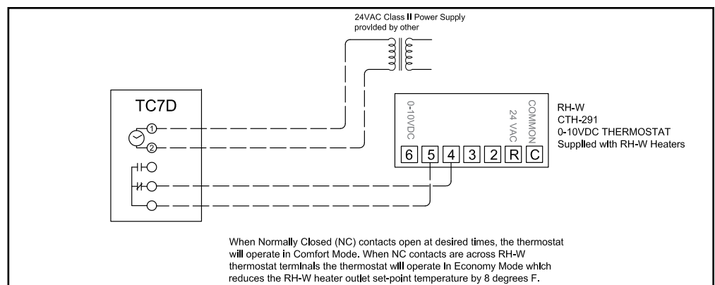
FIGURE 3.1.9 RH-W ELECTRIC HEATER SCHEMATIC
