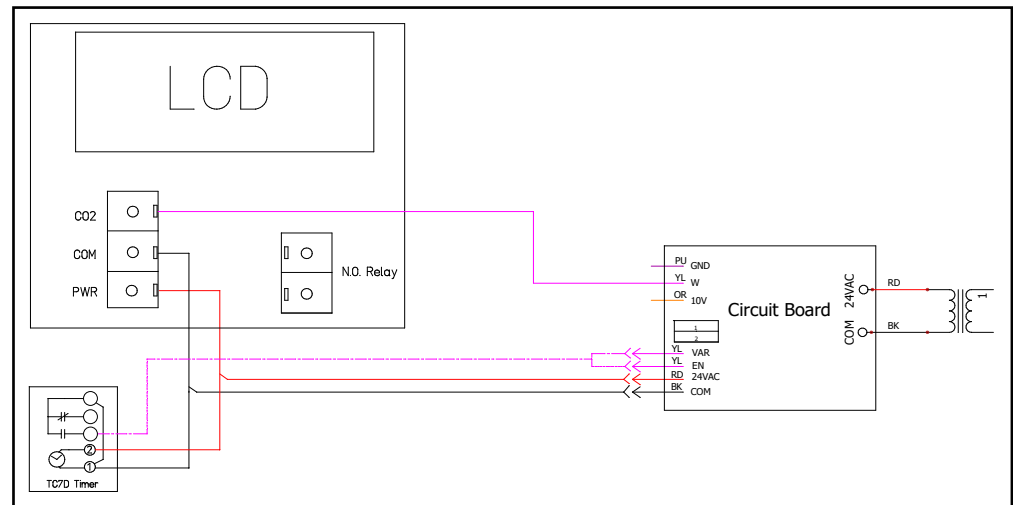
FIGURE 3.1.8 EV450, HE1X, AND HE1.5 ECM WITH CIRCUIT BOARD AND CO2 SCHEMATIC
