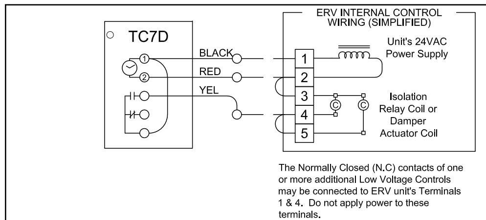
FIGURE 3.1.6 HE1X AND HE1.5 ECM WITH TERMINAL BLOCK SCHEMATIC
