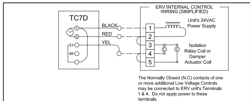
FIGURE 3.1.4 HE1XRT AND HE1.5RT WITH INDEPENDENT BLOWER CONTROL AND HE2X-LE10X SCHEMATIC
