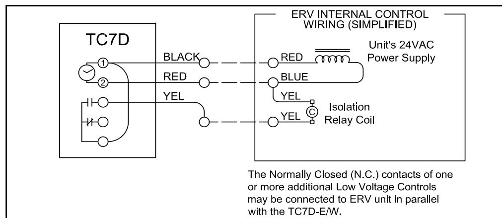
FIGURE 3.1.3 EV450, HE1X, AND HE1.5 STANDARD WIRING SCHEMATIC
