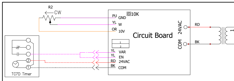
FIGURE 3.1.7 EV450, HE1X AND HE1.5 ECM WITH CIRCUIT BOARD SCHEMATIC
