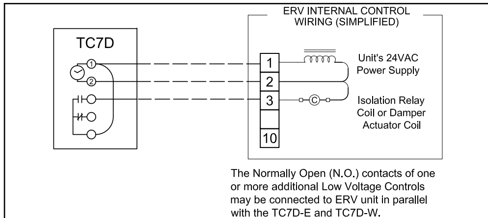
FIGURE 3.1.5 EV450 ECM WITH TERMINAL BLOCK SCHEMATIC
