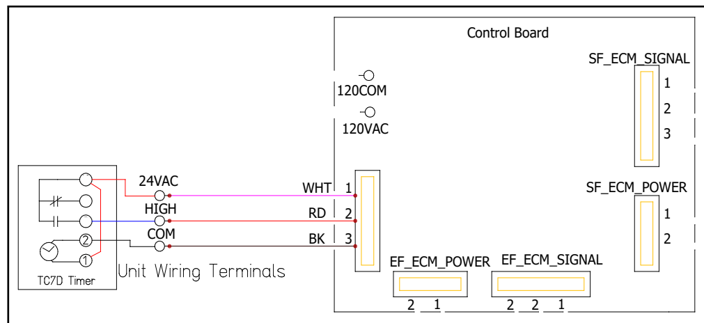
FIGURE 3.1.2 EV PREMIUM AND SL75 SCHEMATIC
