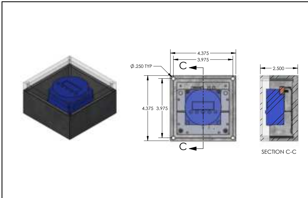
FIGURE 1.2.1 TC7D-E ENCLOSURE DIMENSIONS
