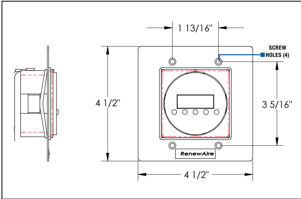
FIGURE 1.2.0 TC7D-W DIMENSIONS
