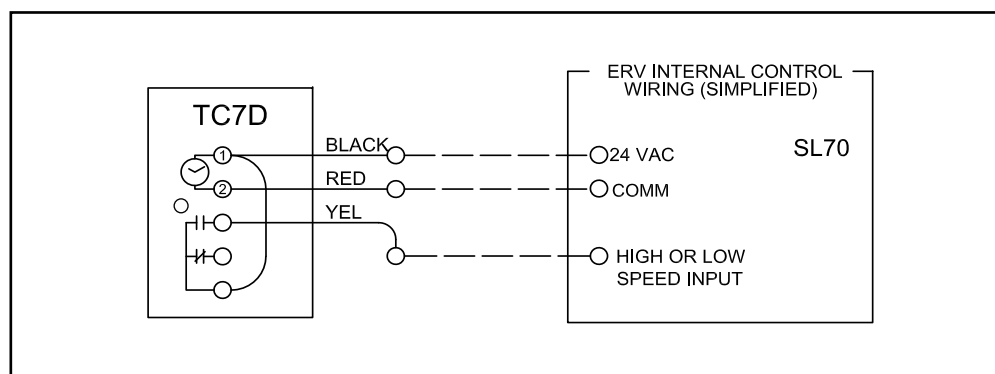
FIGURE 3.1.1 SL70 SCHEMATIC
