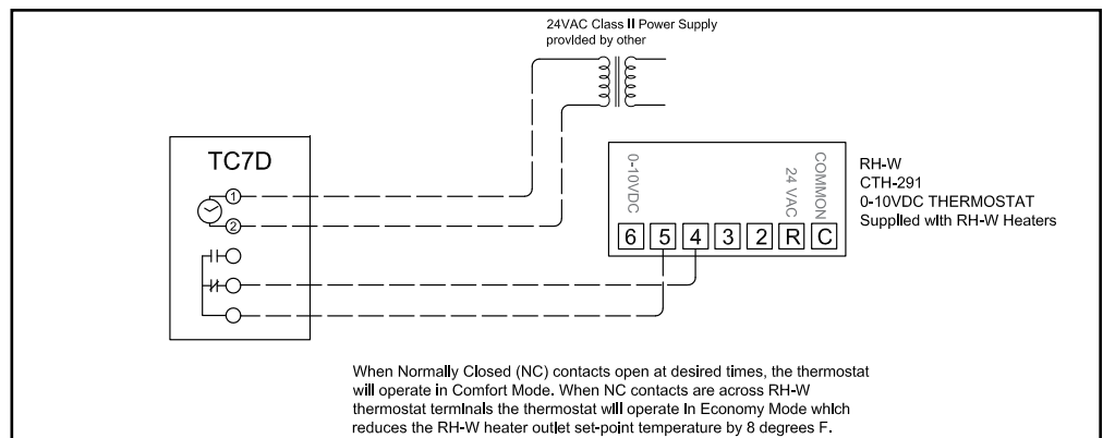
FIGURE 3.1.9 RH-W ELECTRIC HEATER SCHEMATIC
