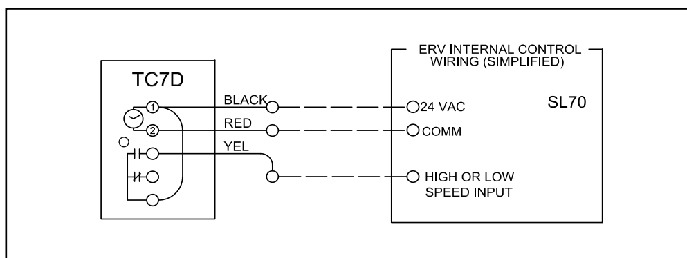
FIGURE 3.1.1 SL70 SCHEMATIC
