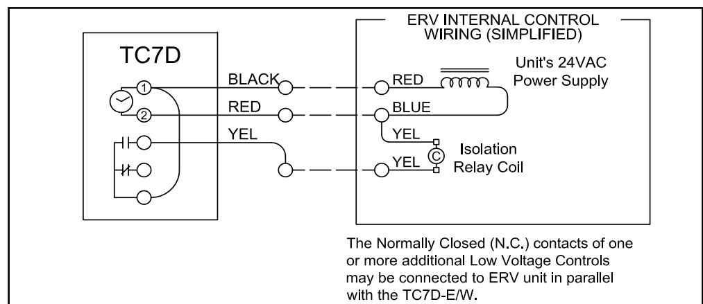
FIGURE 3.1.3 EV450, HE1X, AND HE1.5 STANDARD WIRING SCHEMATIC
