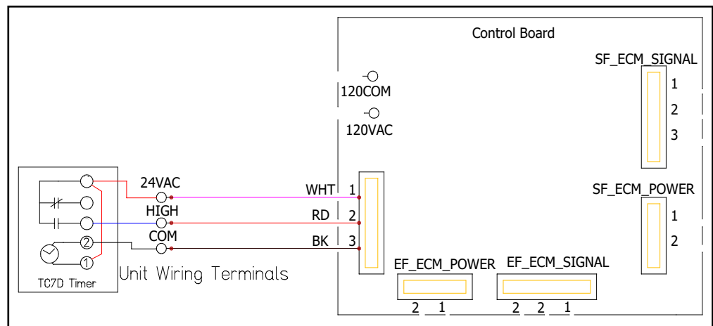
FIGURE 3.1.2 EV PREMIUM AND SL75 SCHEMATIC
