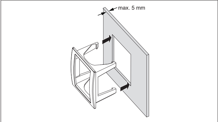
Fig. 13: Insert the front frame in the cut-out
