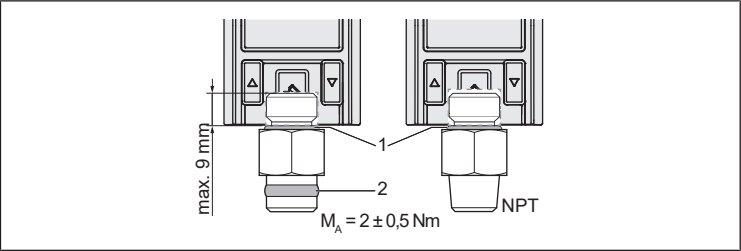
Fig. 17: Double nipples for pressure sensor (1 = O-ring, 2 = PTFE sealing ring)
