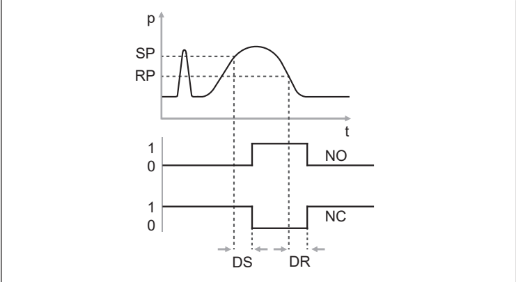
Fig. 6: Delays
