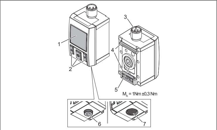
Fig. 1: Device overview
