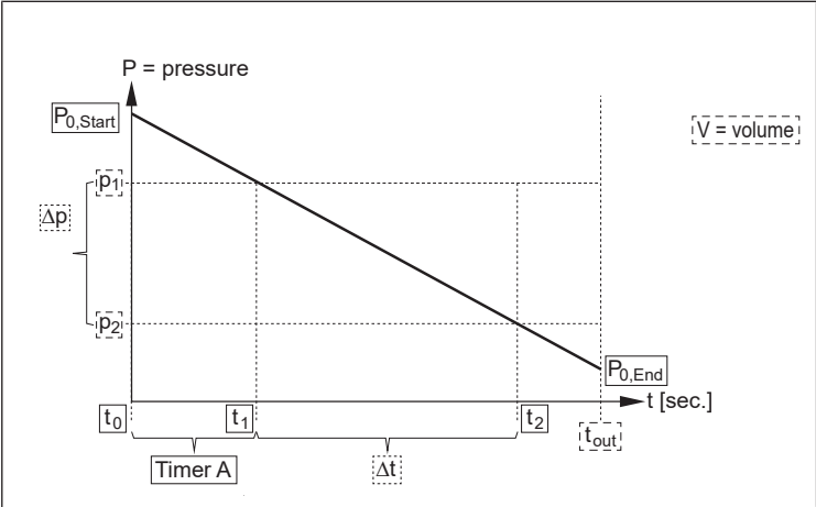
Fig. 23: Leakage characteristic
