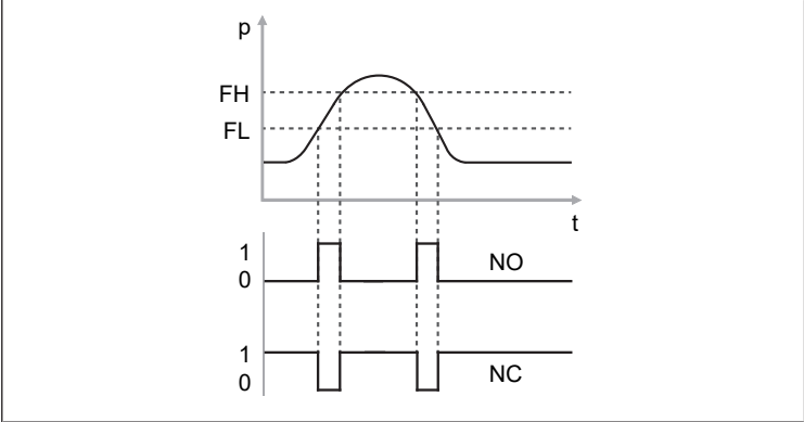
Fig. 5: Window function
