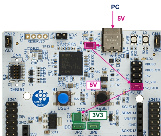
Figure 10. Power supply input from STLINK-V3EC USB connector with PC (5 V, 500 mA maximum)
