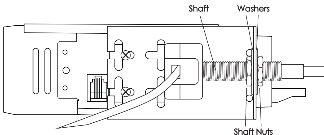
Figure 3 - Mount Shafts to Brackets
