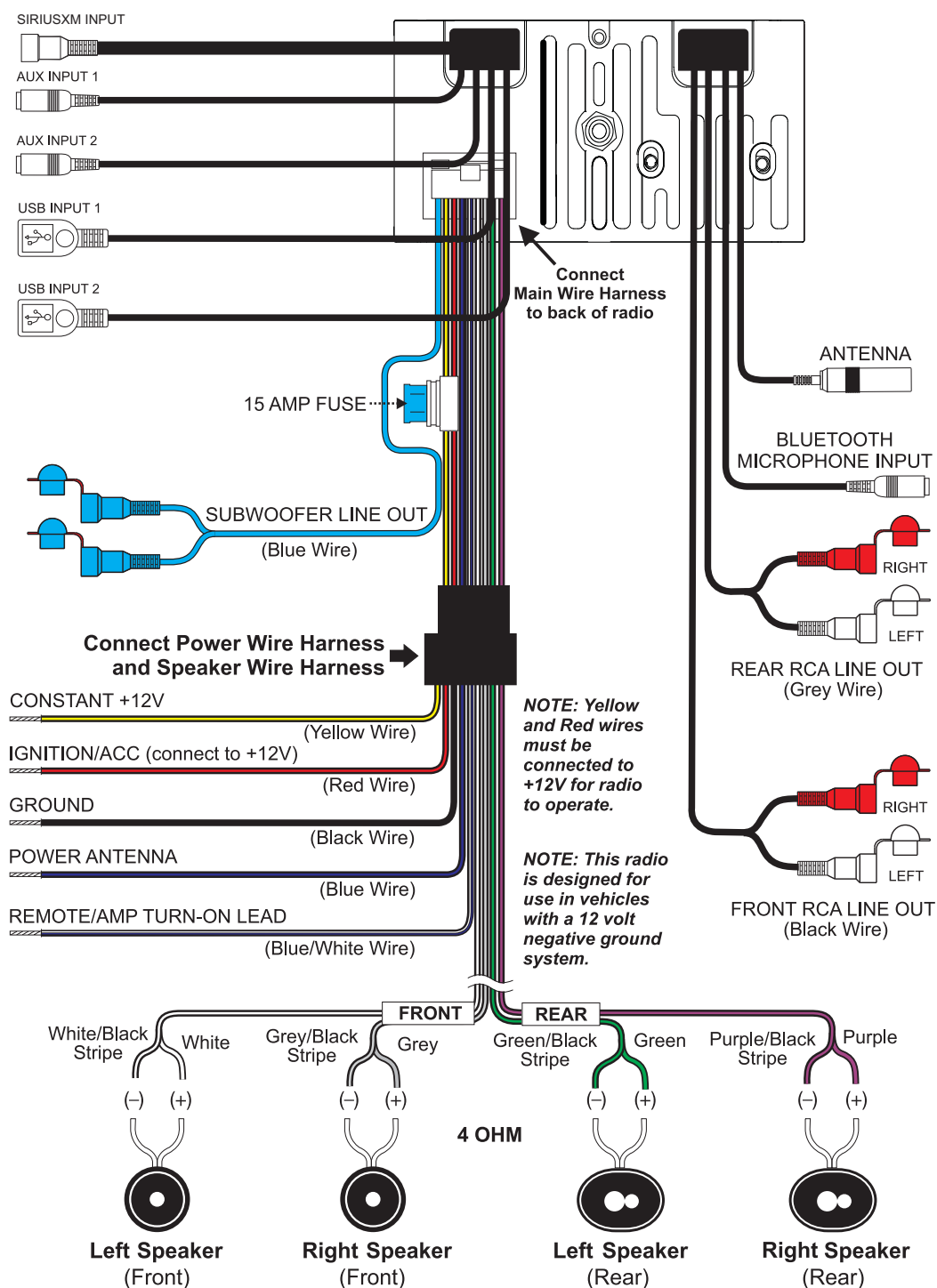
Figure 5 - Wiring Diagram
