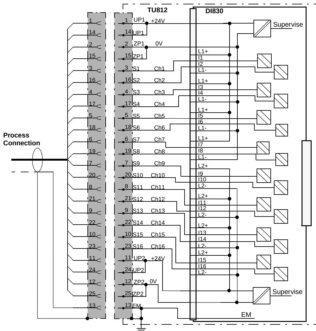
Figure 118. DI830 with TU812 Compact MTU Process Connections
