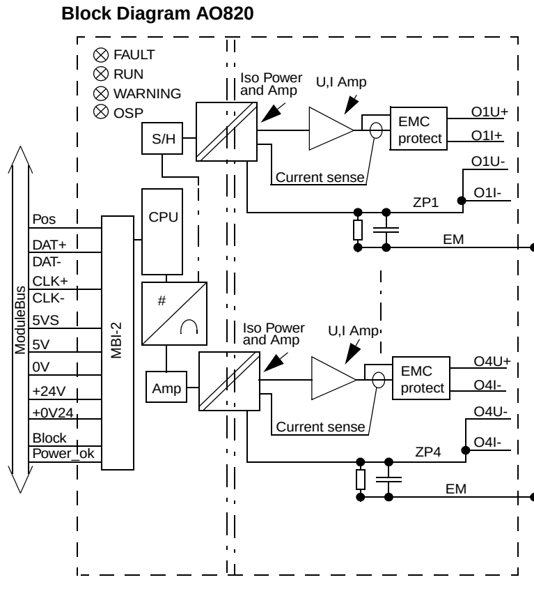
Figure 70. AO820 Block Diagram
