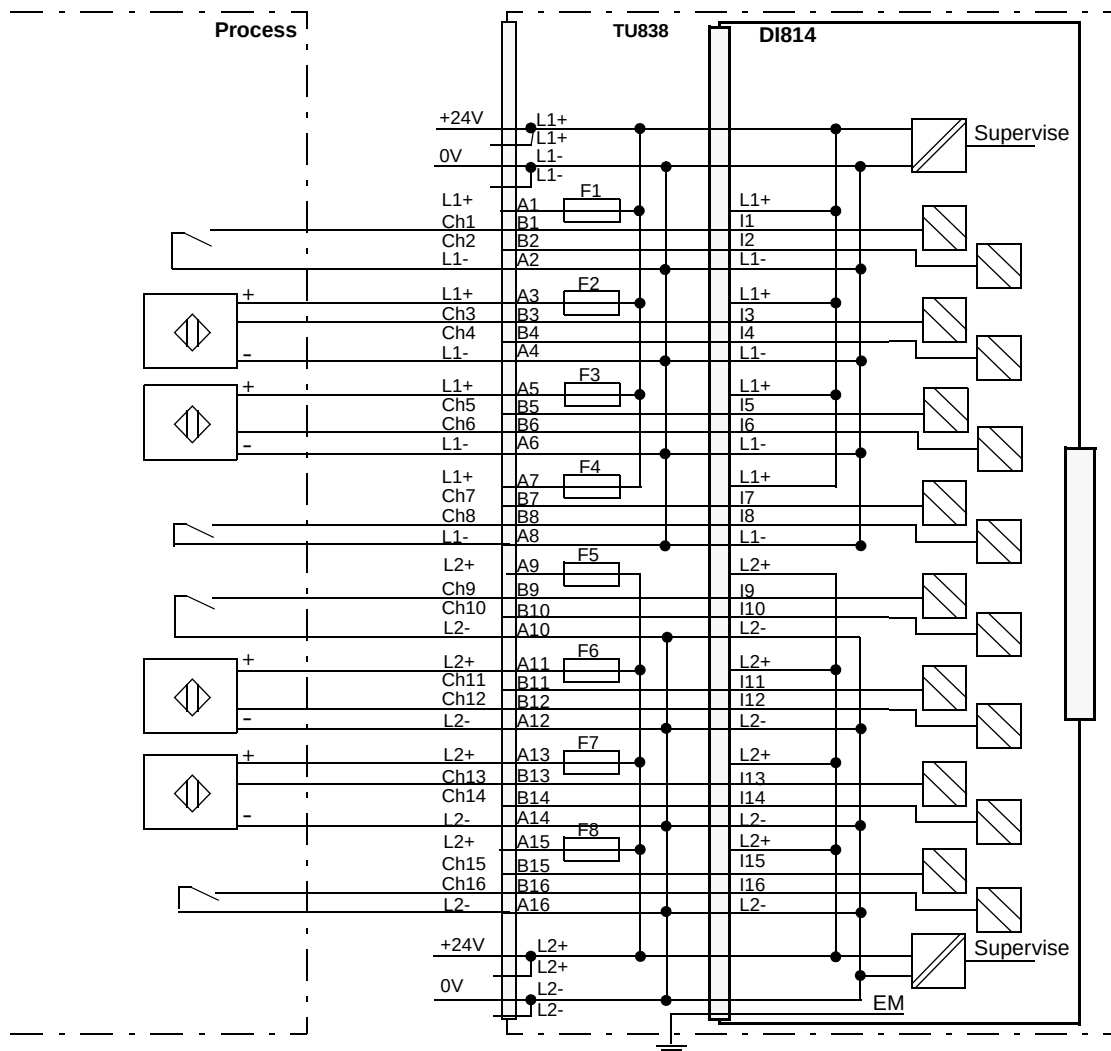
Figure 99. DI814 with TU838 Extended MTU Process Connections
