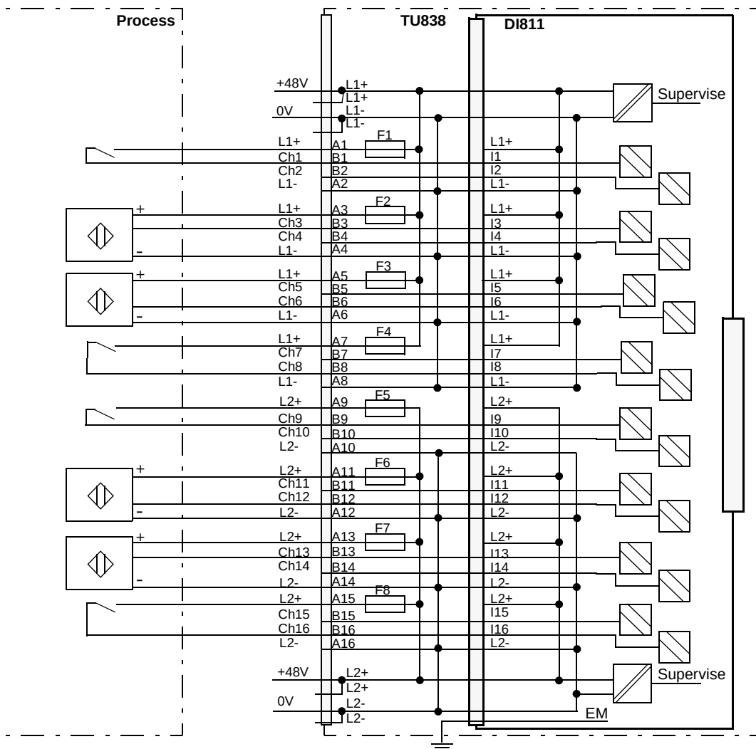
Figure 93. DI811 with TU838 Extended MTU Process Connections
