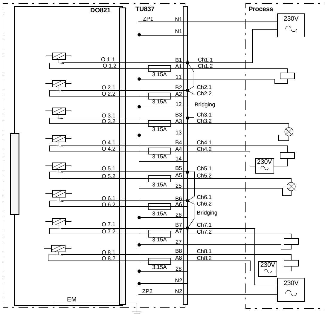
Figure 167. DO821 with TU837 Extended MTU Process Connections
