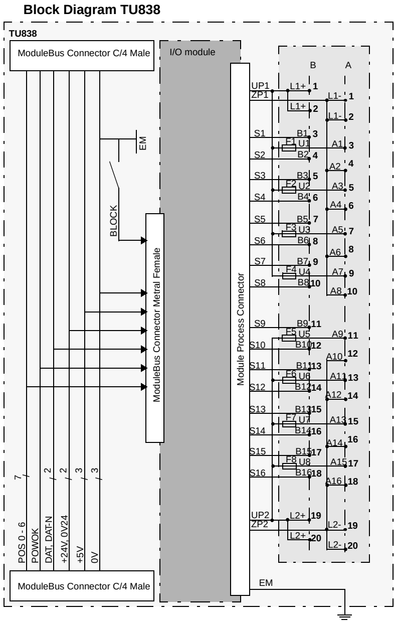
Figure 212. TU838 Block Diagram
