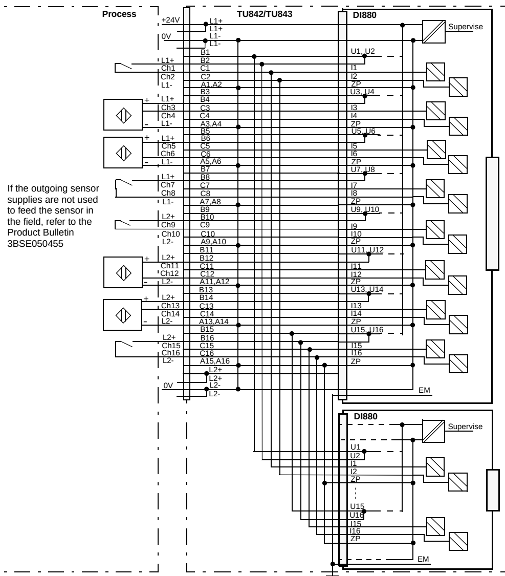
Figure 136. DI880 with TU842 or TU843 Redundant MTU Process Connections
