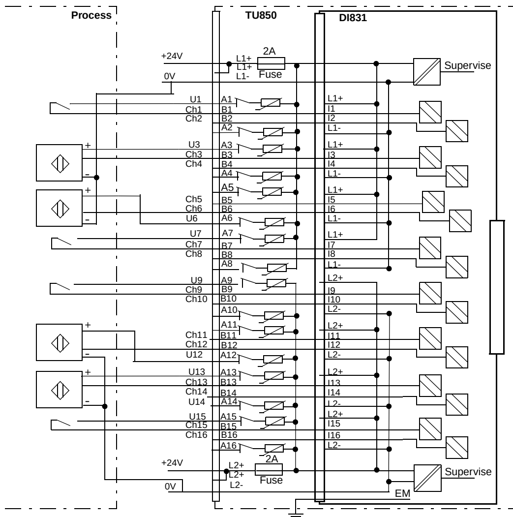
Figure 125. DI831 with TU850 Extended MTU Process Connection.
