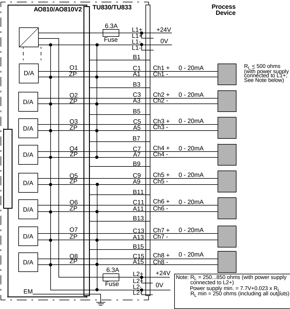
Figure 63. AO810/AO810V2 with TU830 Extended MTU Process Connections
