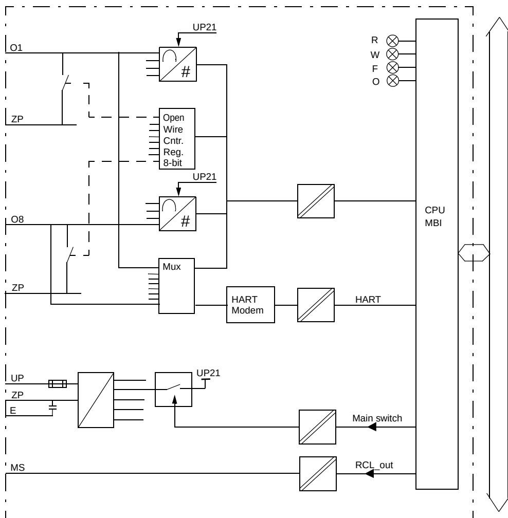
Figure 66. AO815 Block Diagram
