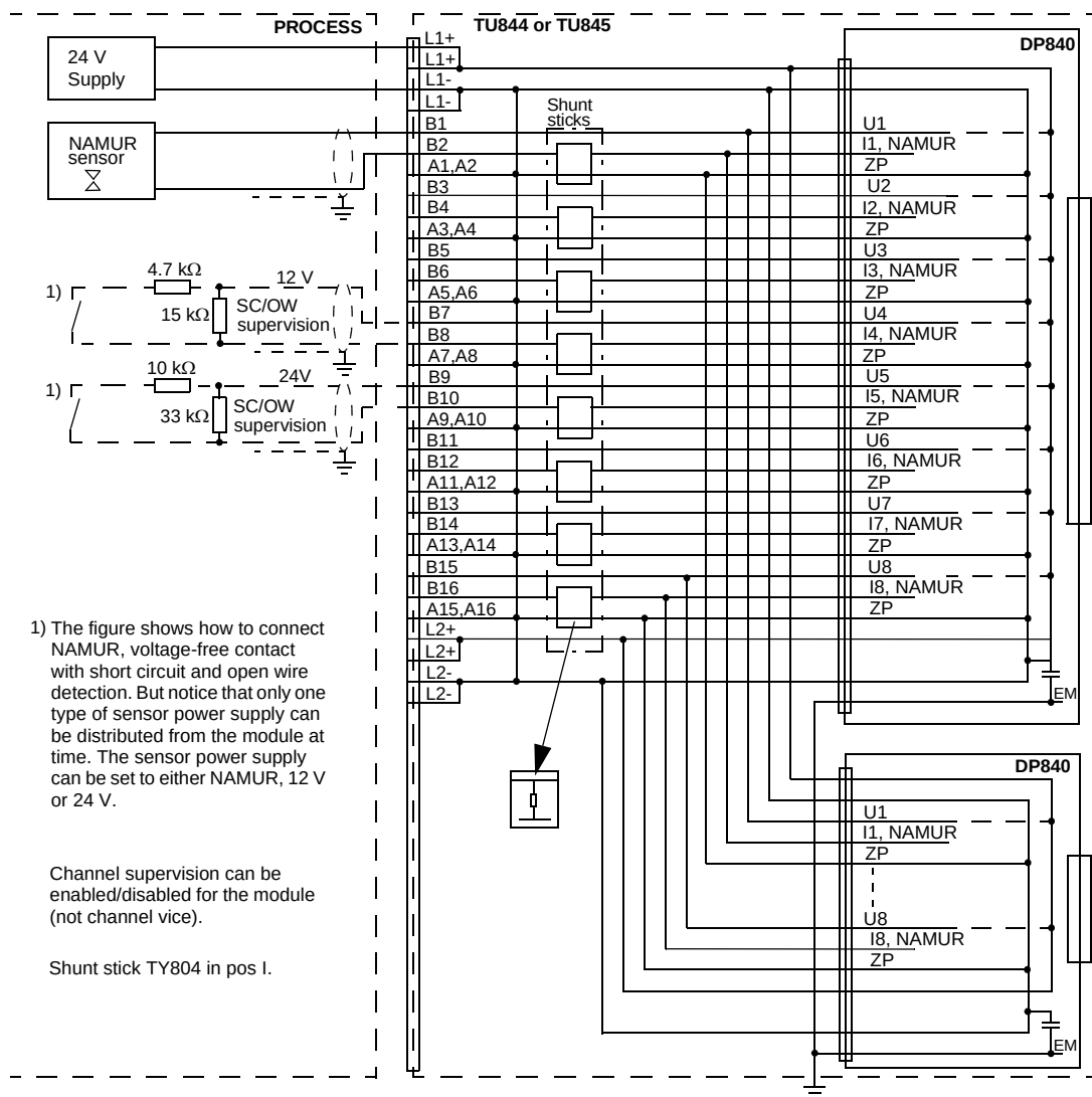
Figure 196. DP840 with TU844 or TU845 MTU Process Connections
