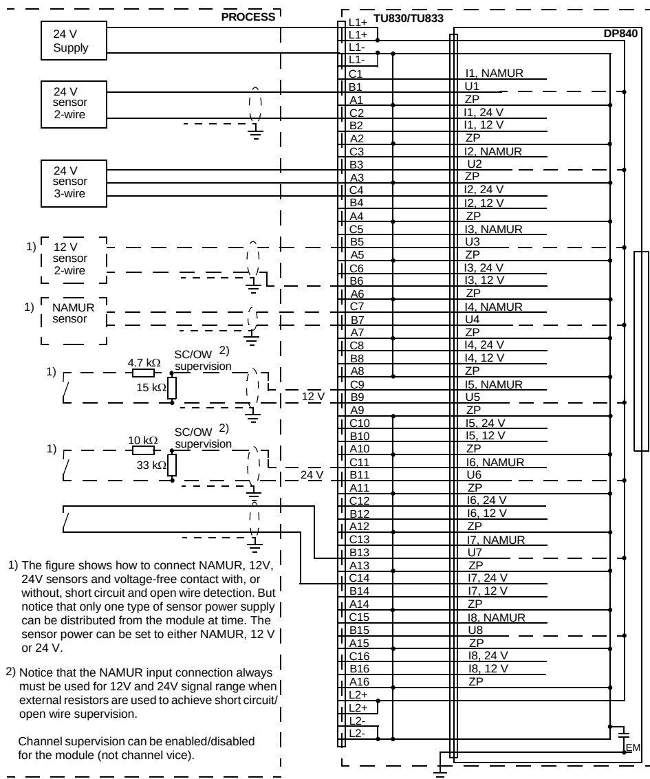
Figure 194. DP840 with TU830 MTU Process Connections
