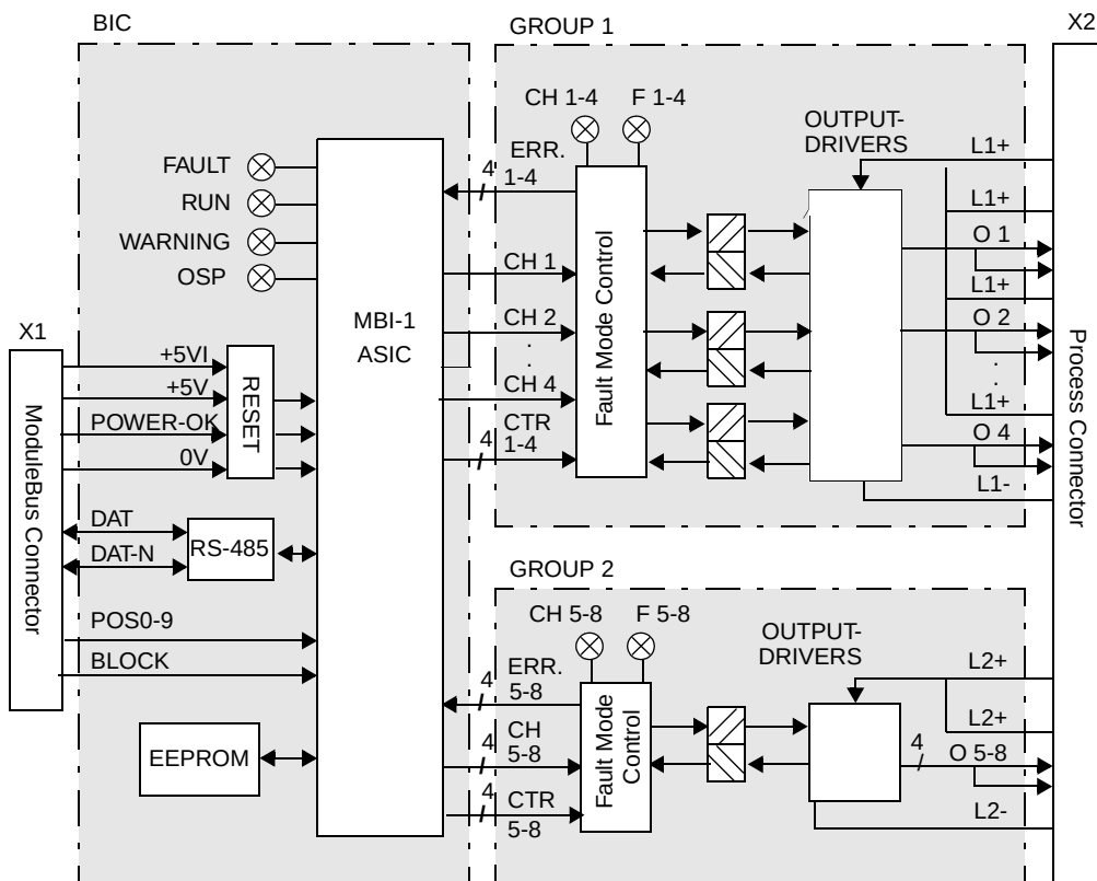
Figure 154. DO815 Block Diagram
