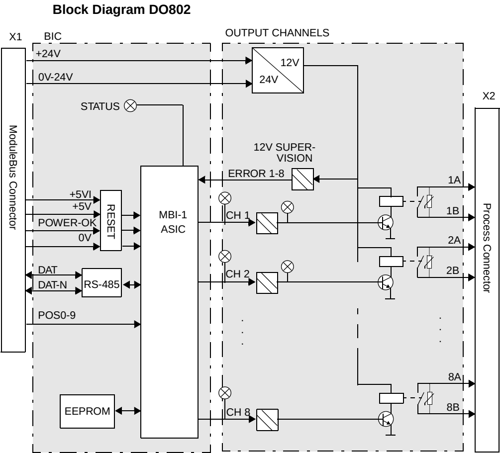
Figure 143. DO802 Block Diagram
