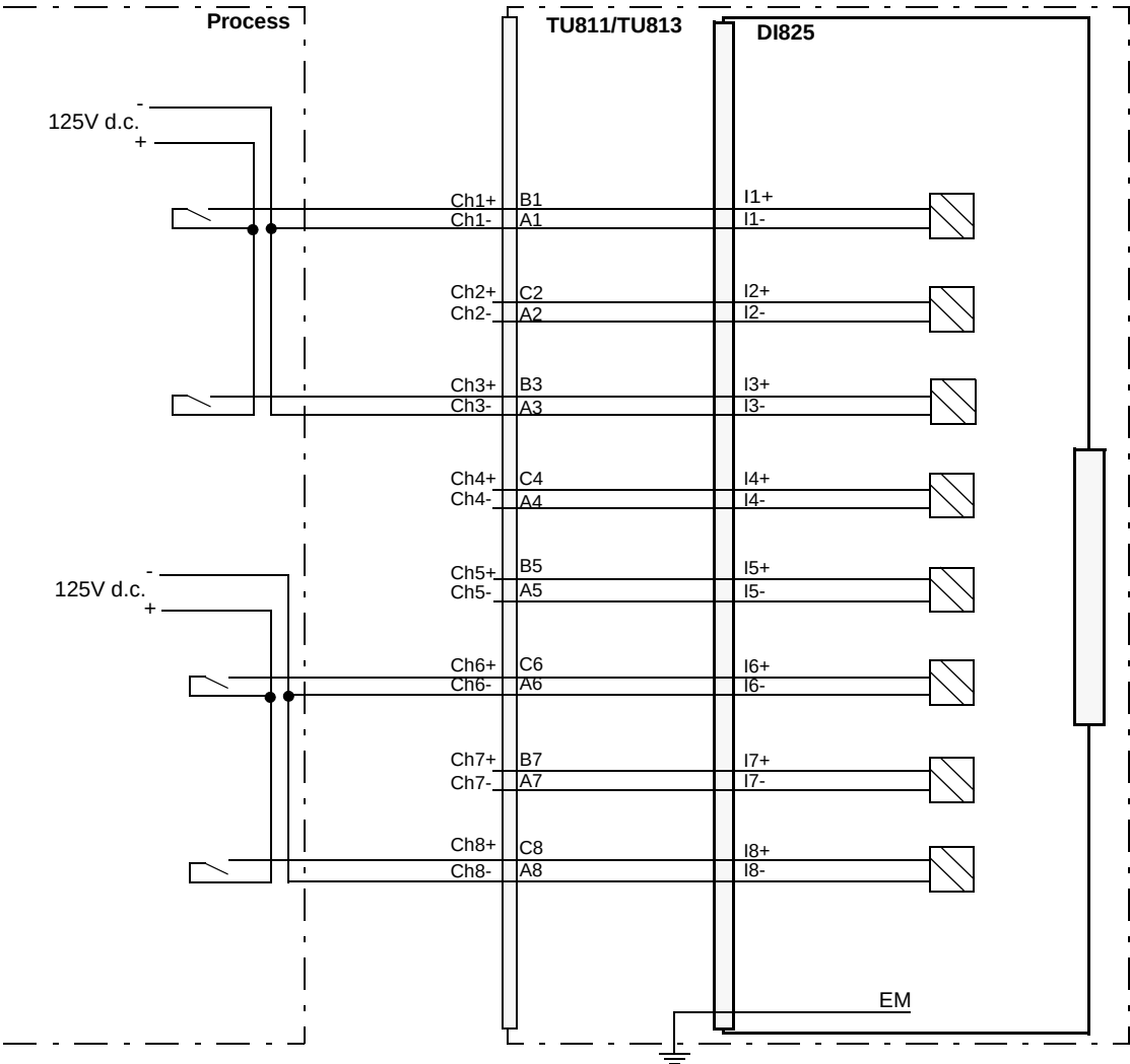
Figure 111. DI825 with TU811 or TU813 Compact MTU Process Connections
