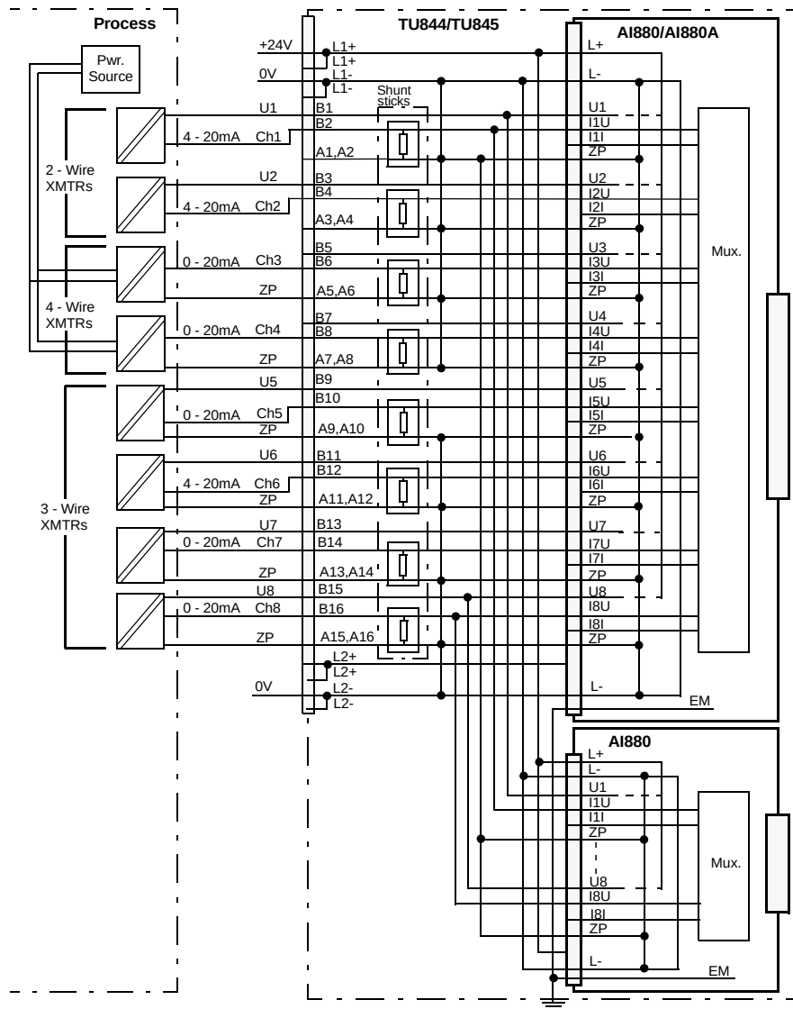
Figure 56. AI880/AI880A with TU844 or TU845 Redundant MTU Process Connections
