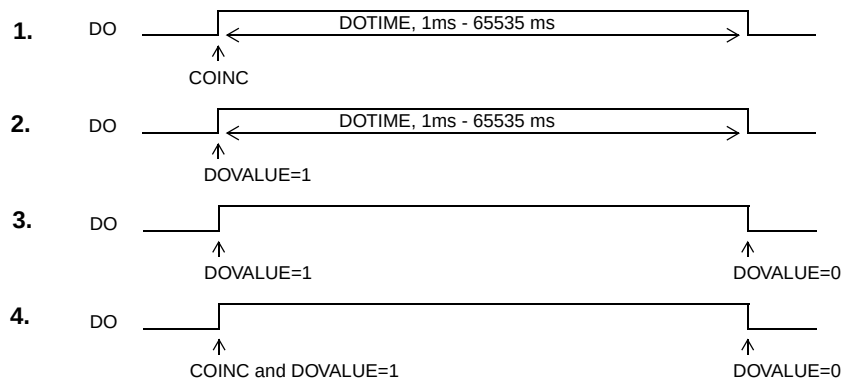
Figure 185. Configuration of Digital Output Function
