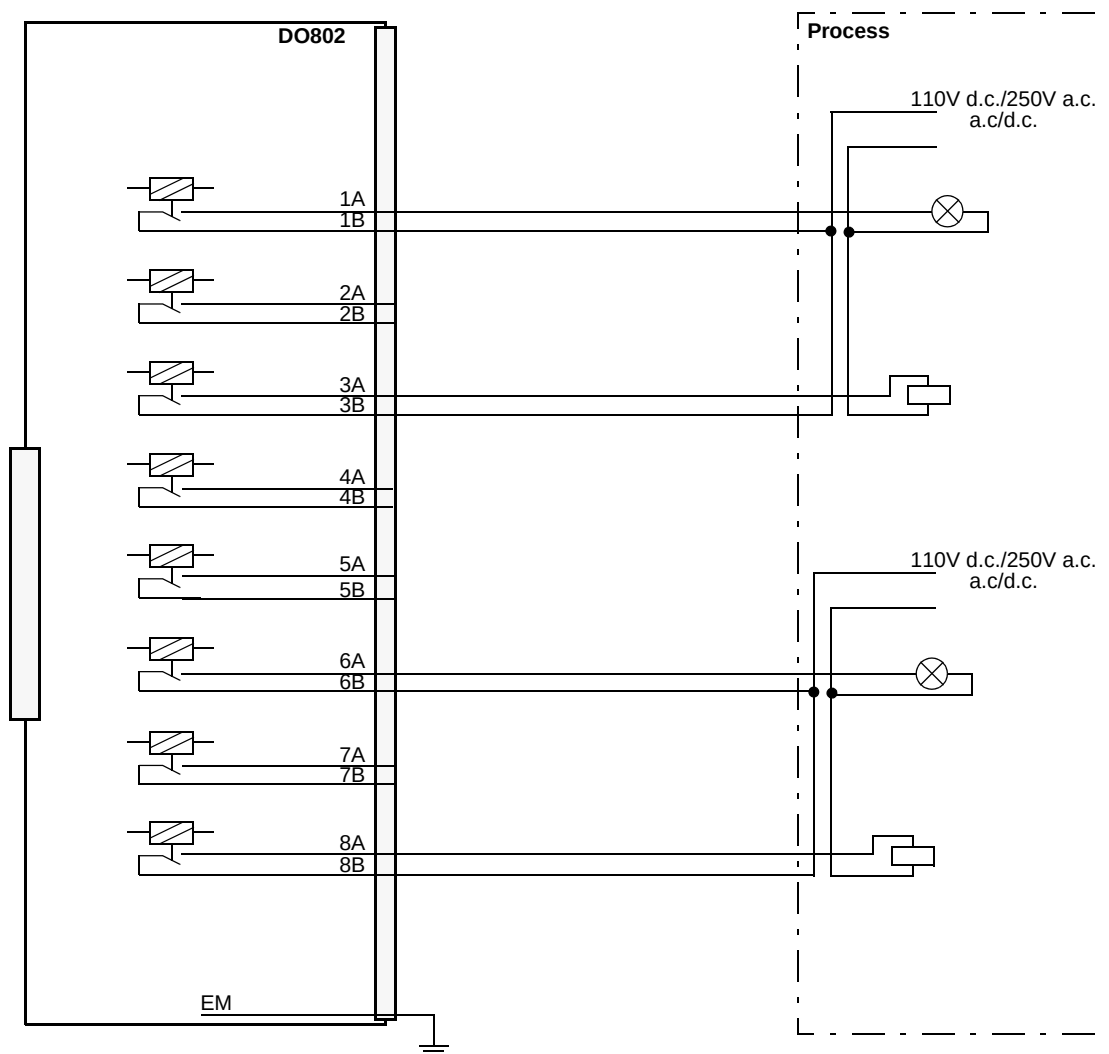
Figure 144. DO802 Process Connections
