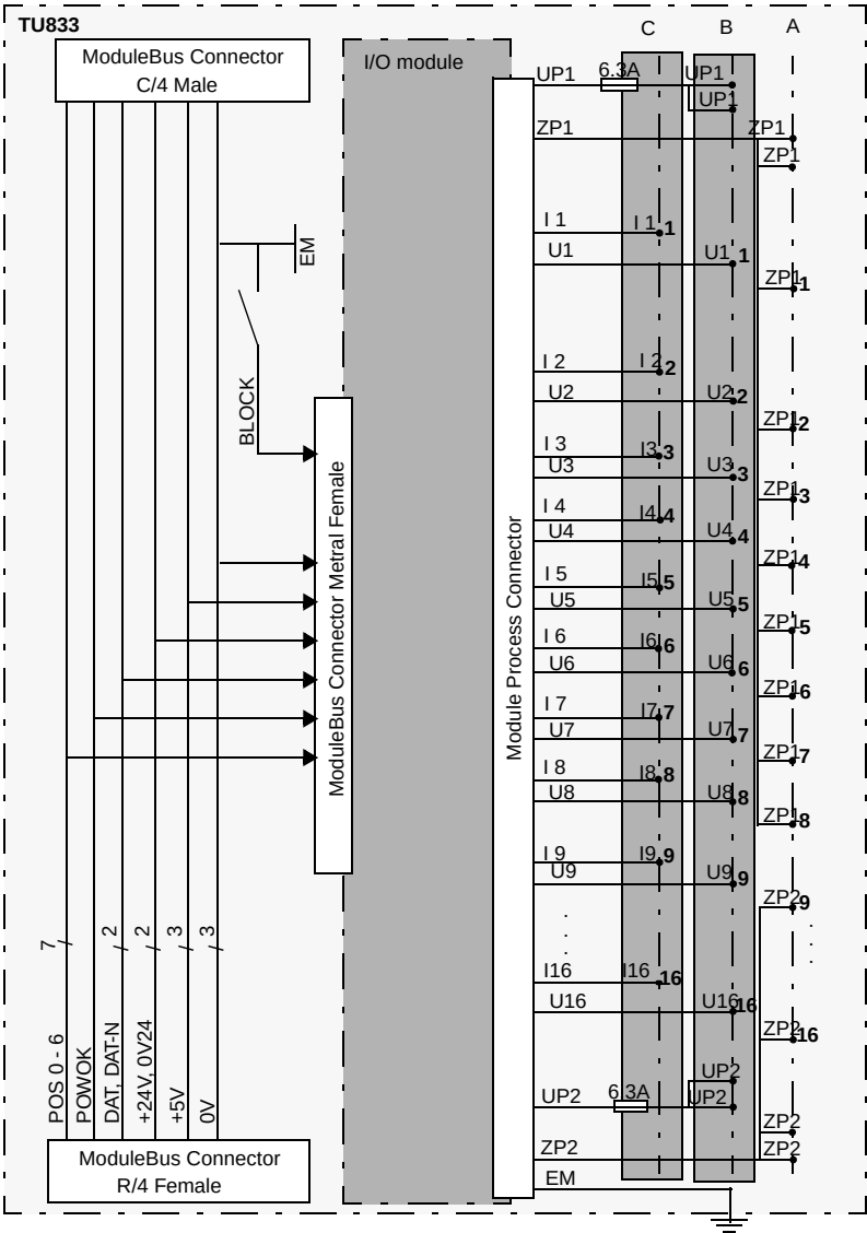
Figure 207. TU833 Block Diagram
