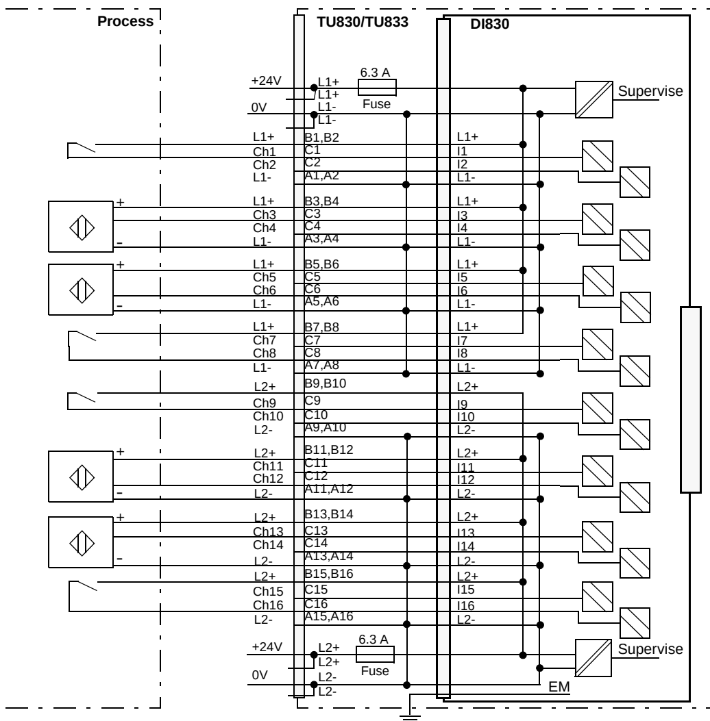
Figure 115. DI830 with TU830 Extended MTU Process Connections
