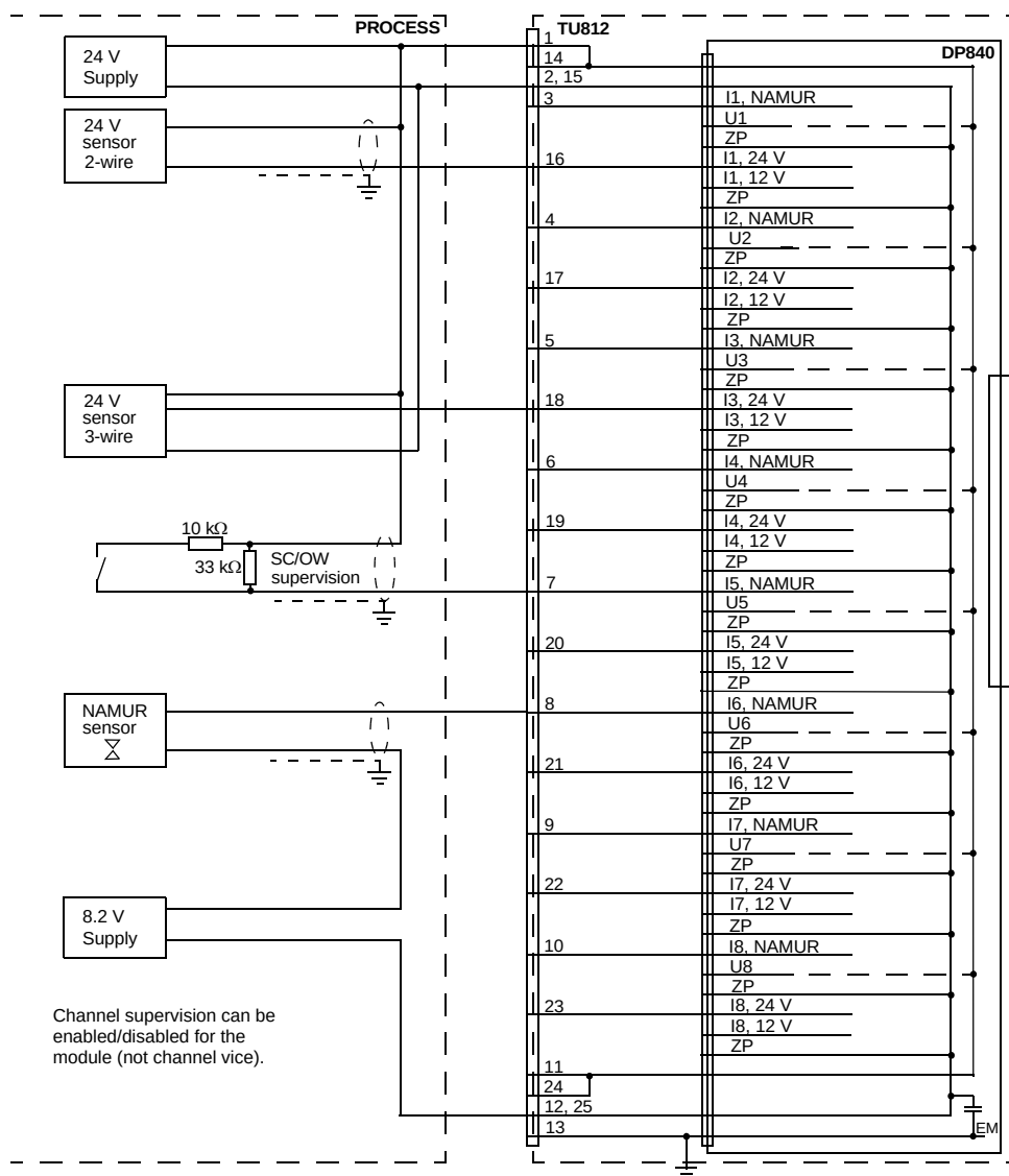
Figure 193. DP840 with TU812 MTU Process Connections
