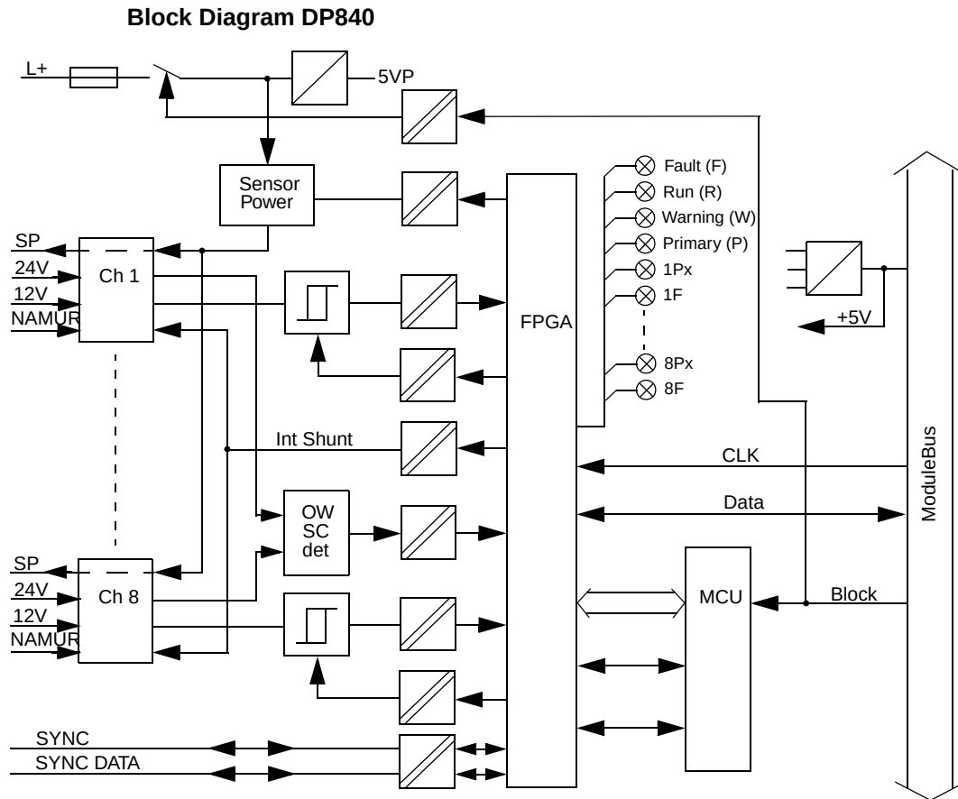
Figure 191. DP840 Block Diagram
