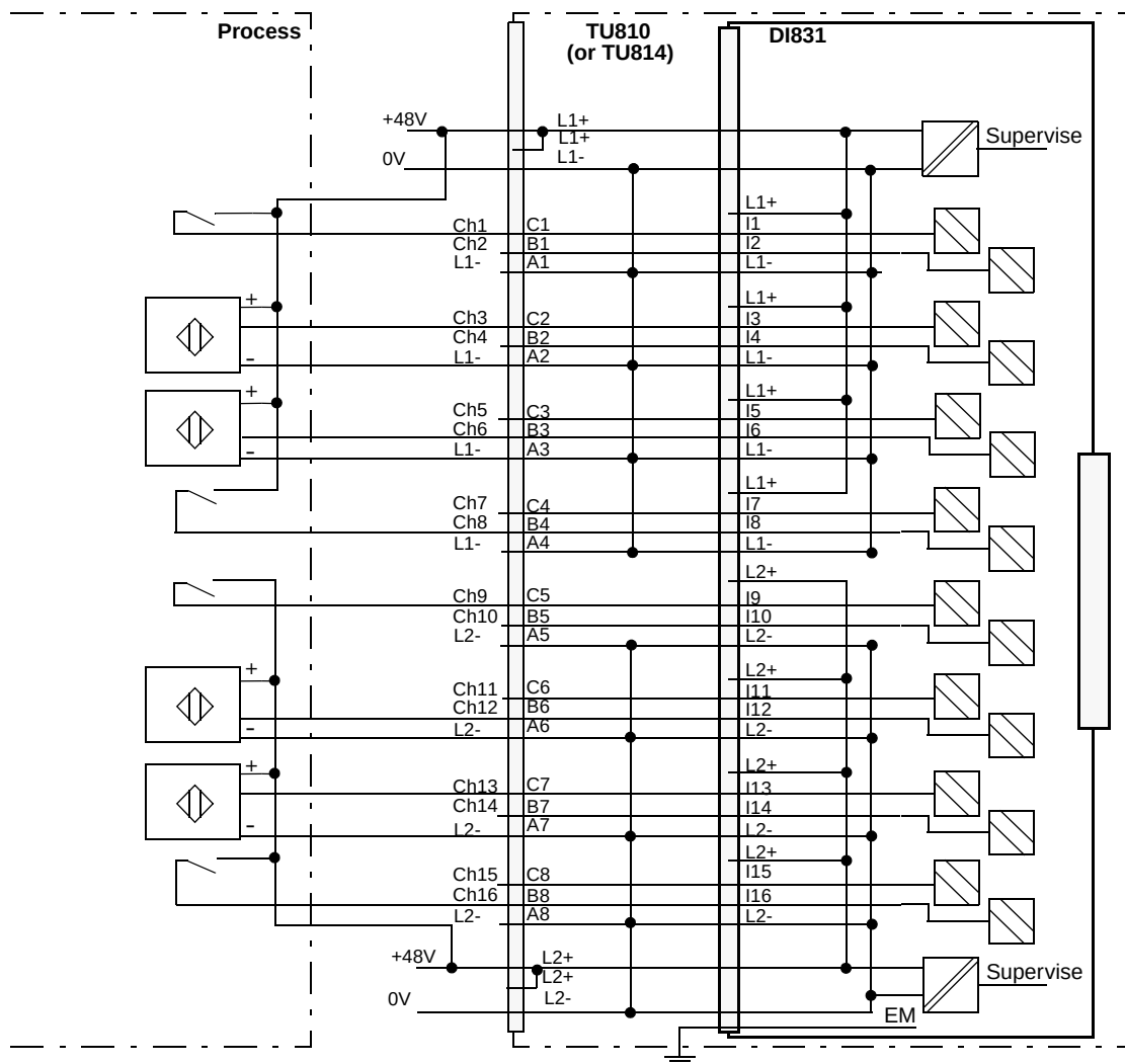
Figure 123. DI831 with TU810 or TU814 Compact MTU Process Connections
