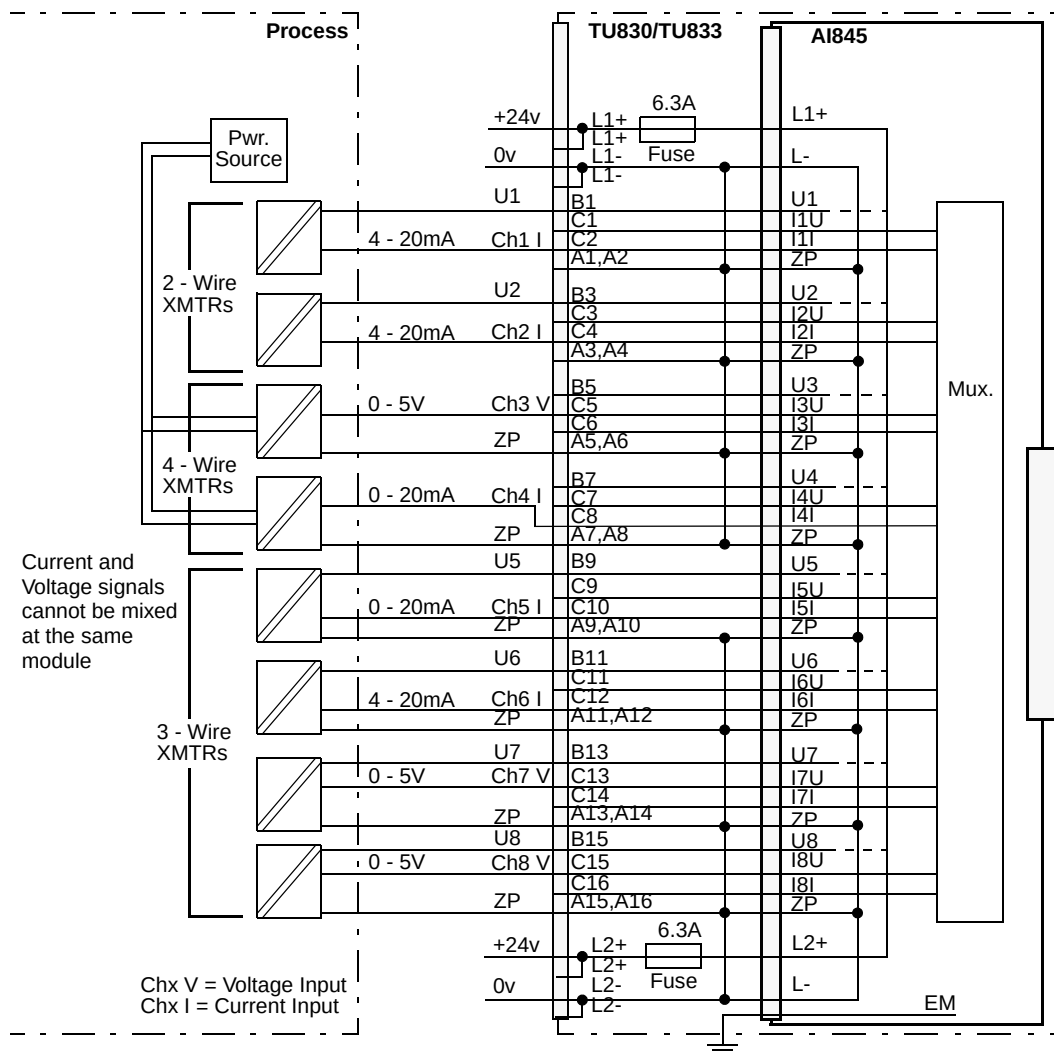
Figure 47. AI845 with TU830/TU833 Extended MTU Process Connections
