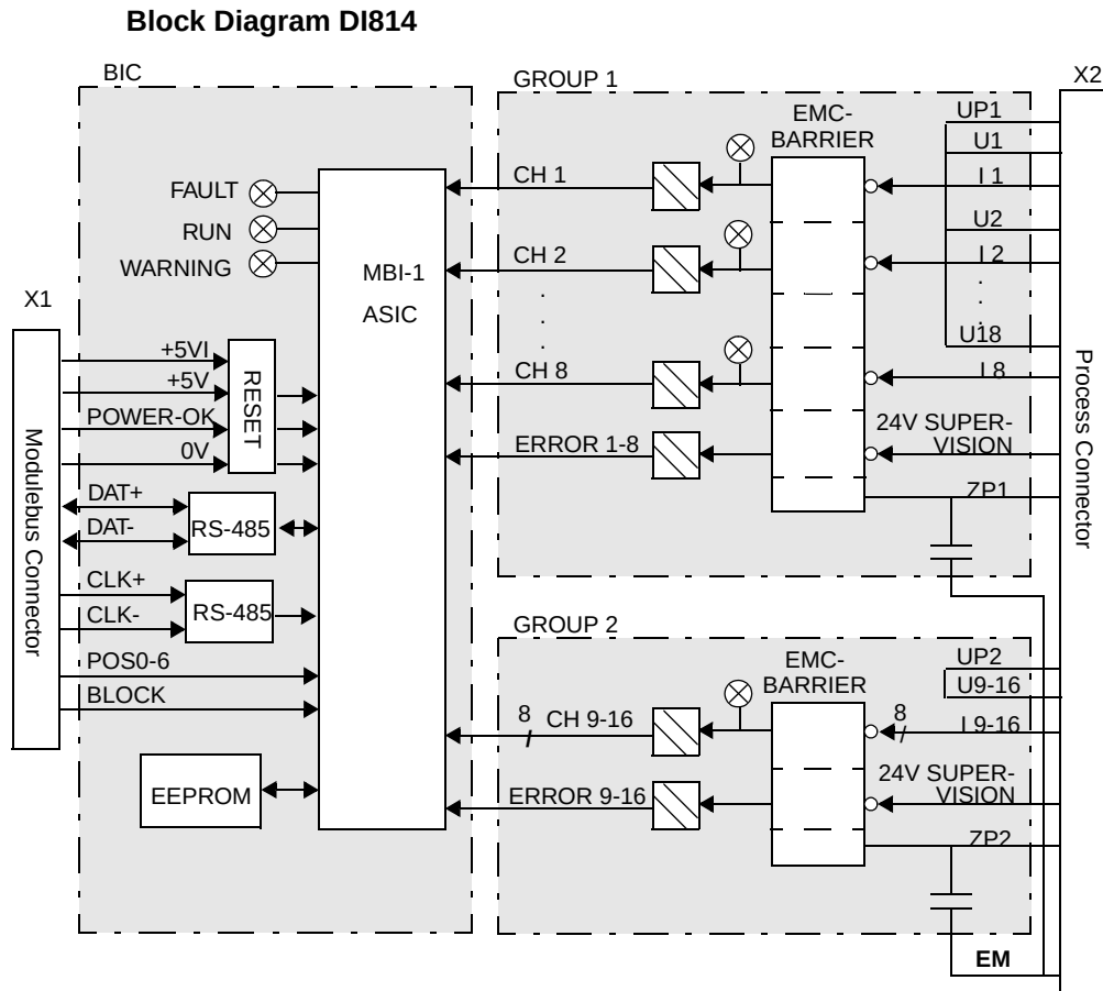
Figure 97. DI814 Block Diagram
