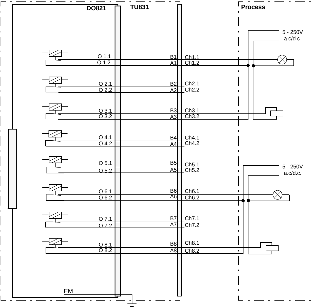
Figure 164. DO821 with TU831 Extended MTU Process Connections
