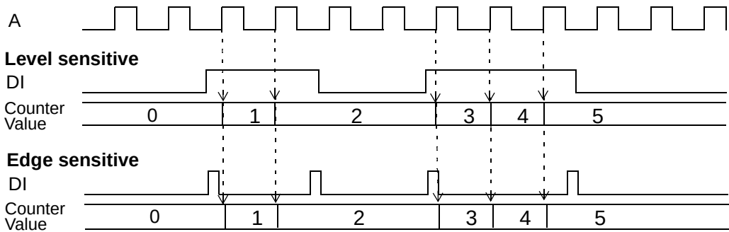
Figure 184. Gated Count Mode in Two different Ways
