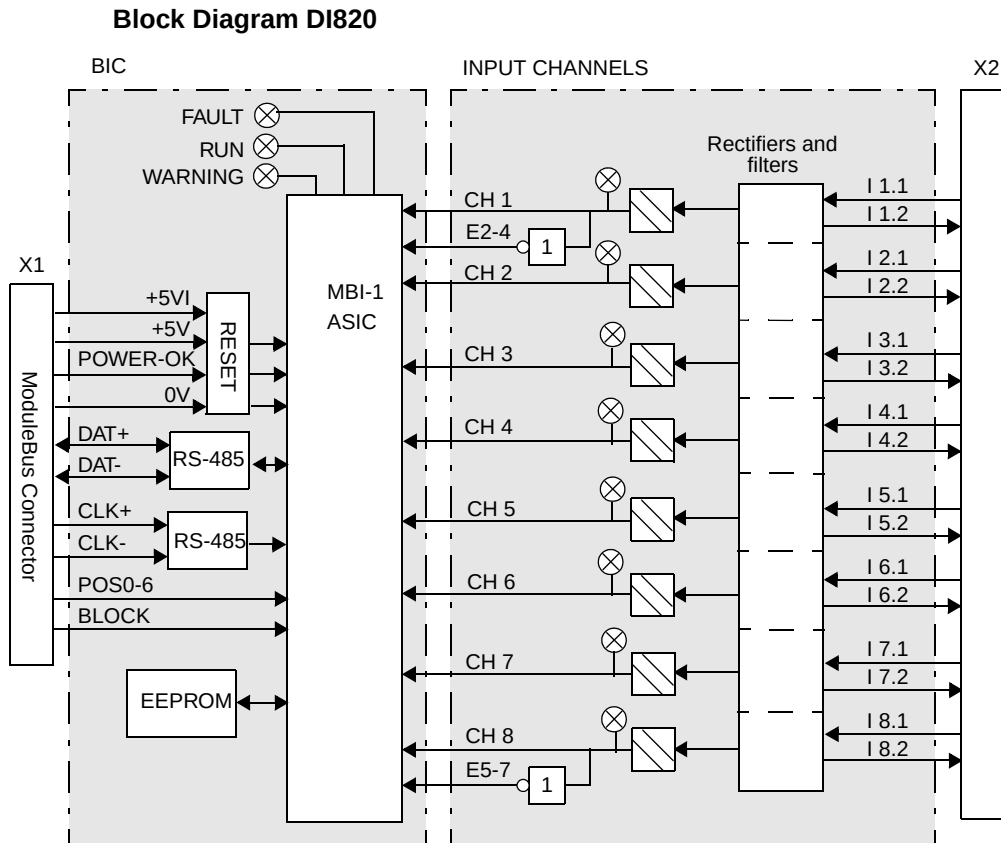
Figure 102. DI820 Block Diagram
