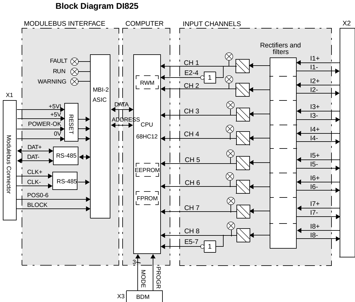
Figure 110. DI825 Block Diagram
