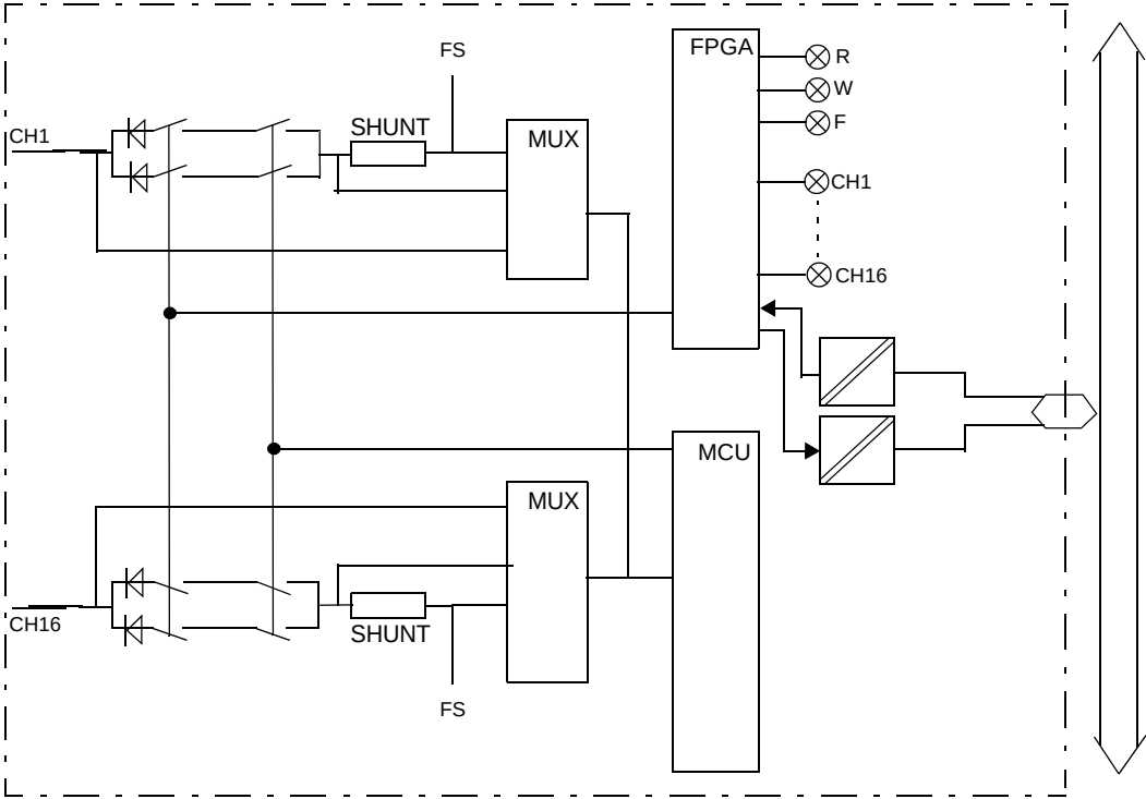
Figure 174. Block Diagram D0880
