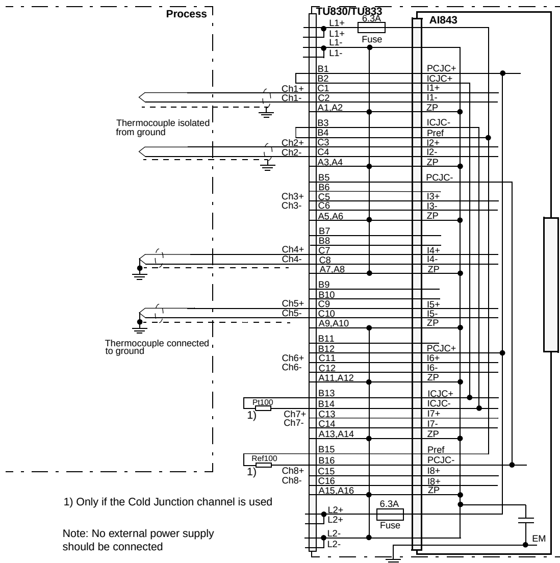
Figure 43. AI843 with TU830 Extended MTU Process Connections
