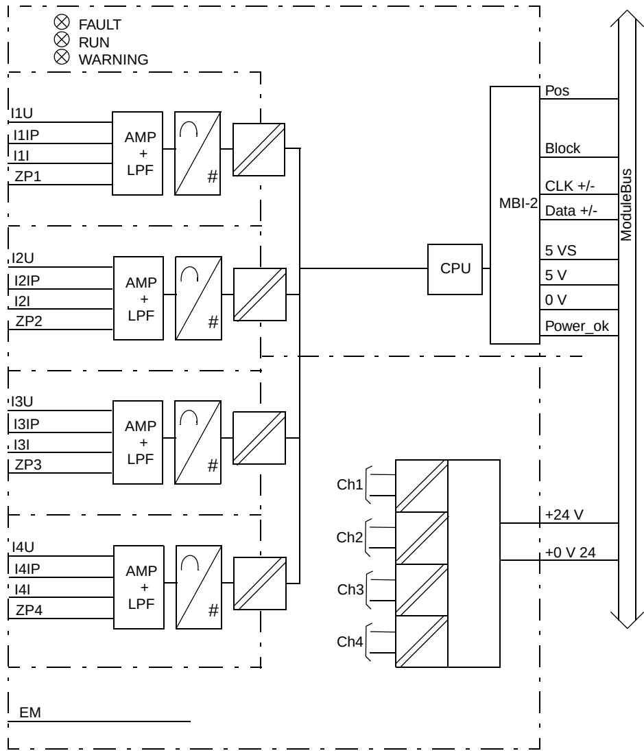
Figure 29. AI825 Block Diagram
