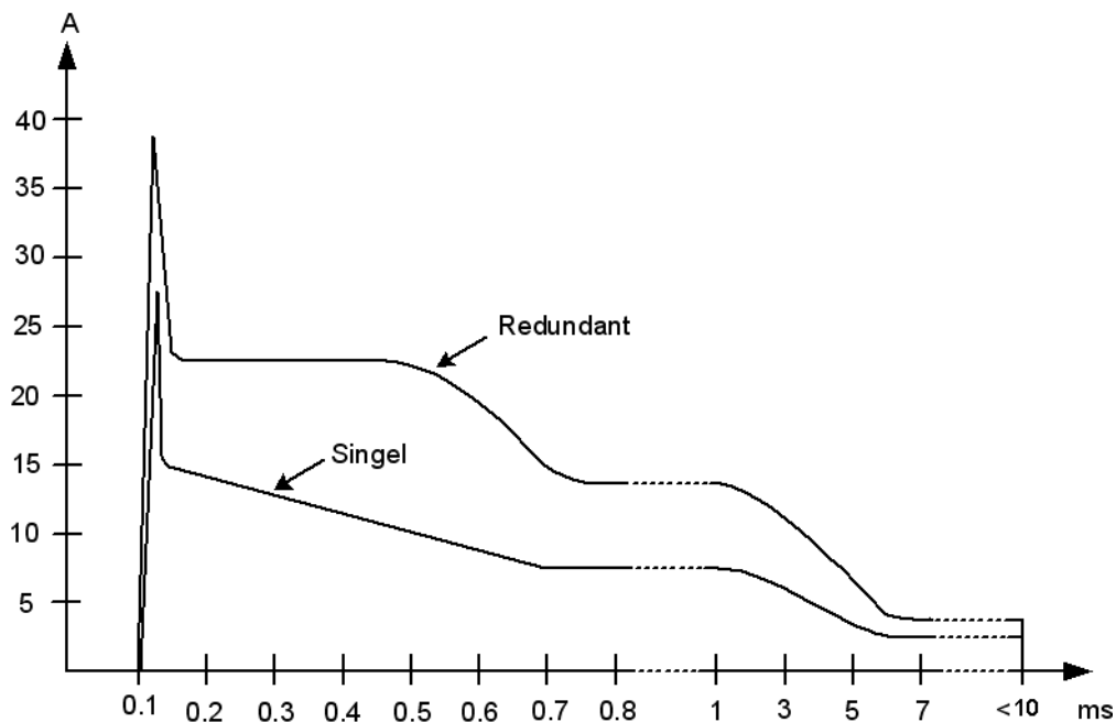
Figure 173. Short circuit current, worst case
