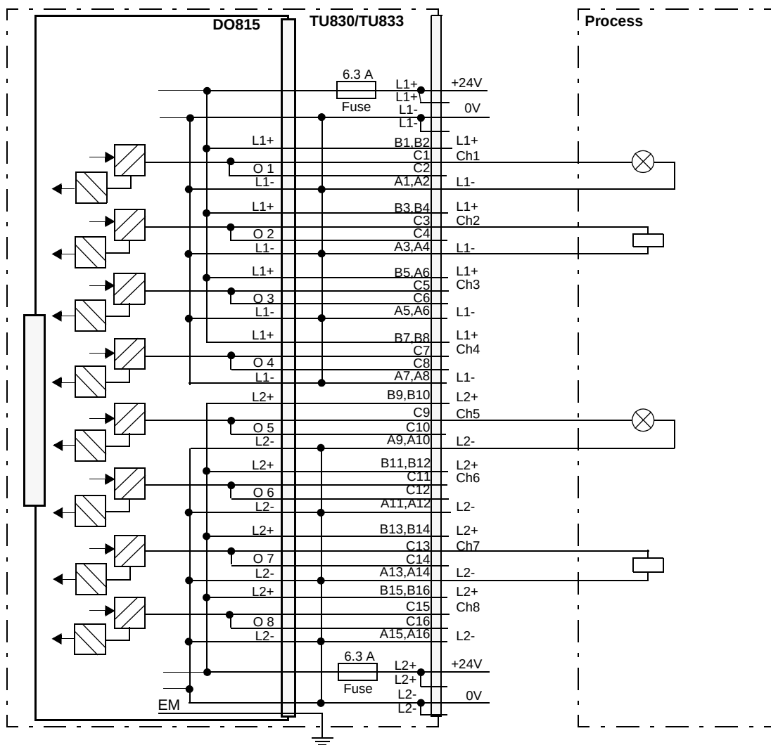
Figure 155. DO815 with TU830/TU833 Extended MTU Process Connections
