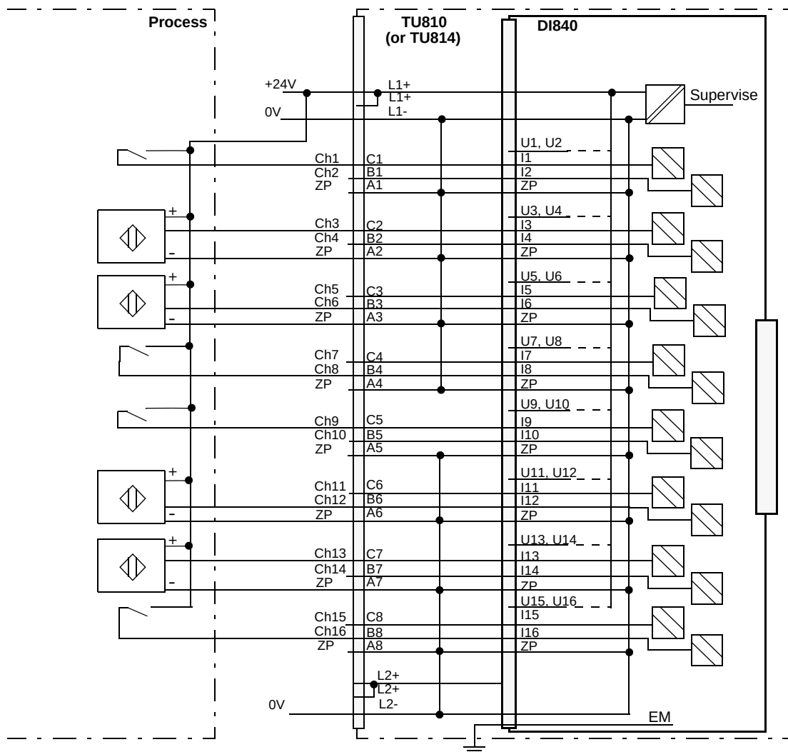
Figure 129. DI840 with TU810 or TU814 Compact MTU Process Connections
