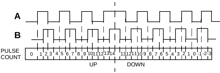
Figure 183. Quadrature Mode, #4 (Count on Pos. Edge and Neg. Edge Input A and Input B)
