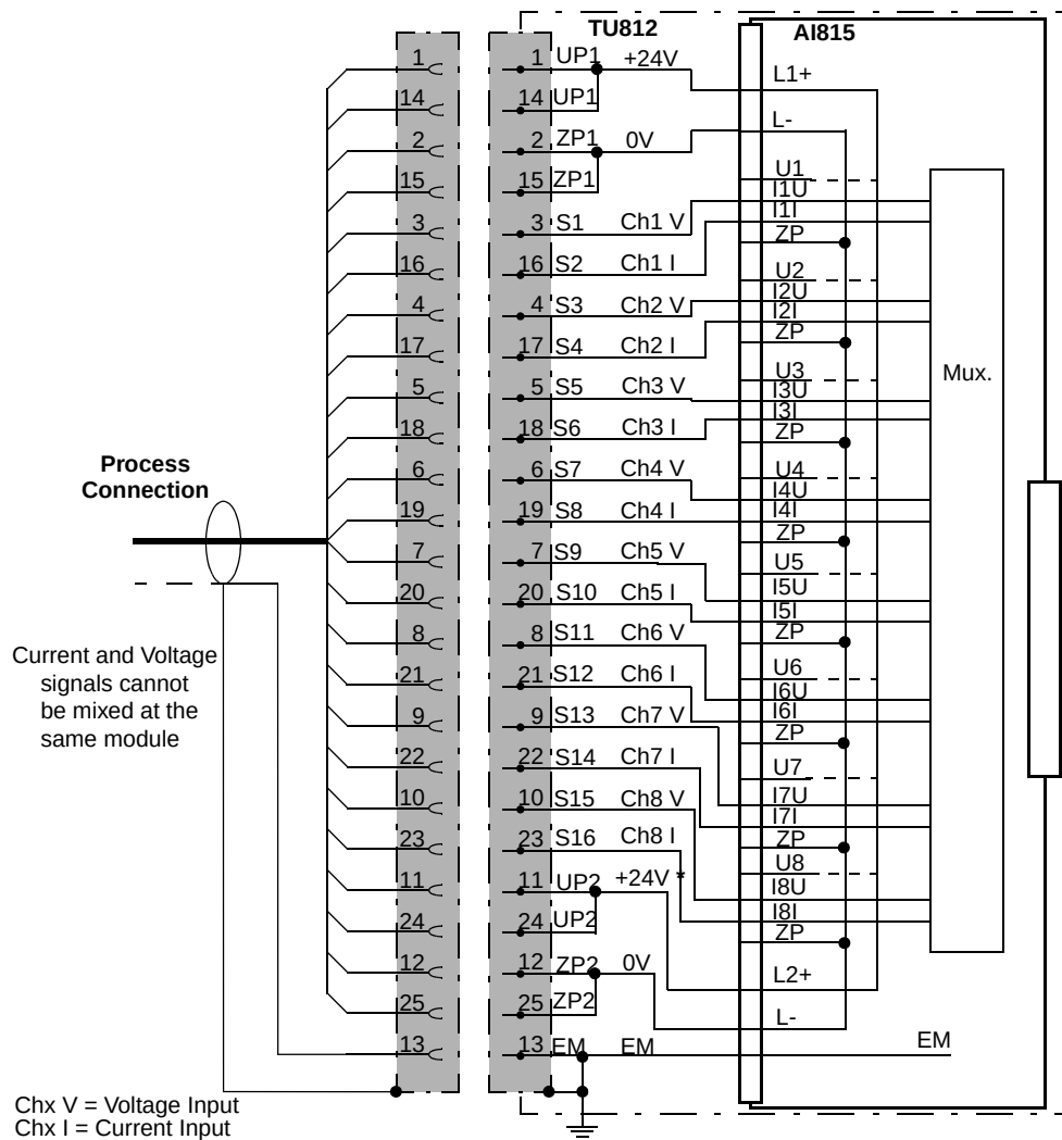
Figure 24. AI815 with TU812 Compact MTU Process Connections
