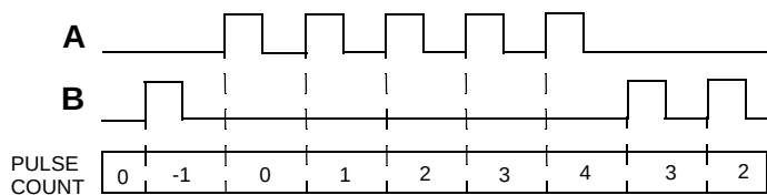
Figure 179. Up/Down Pulse Mode
