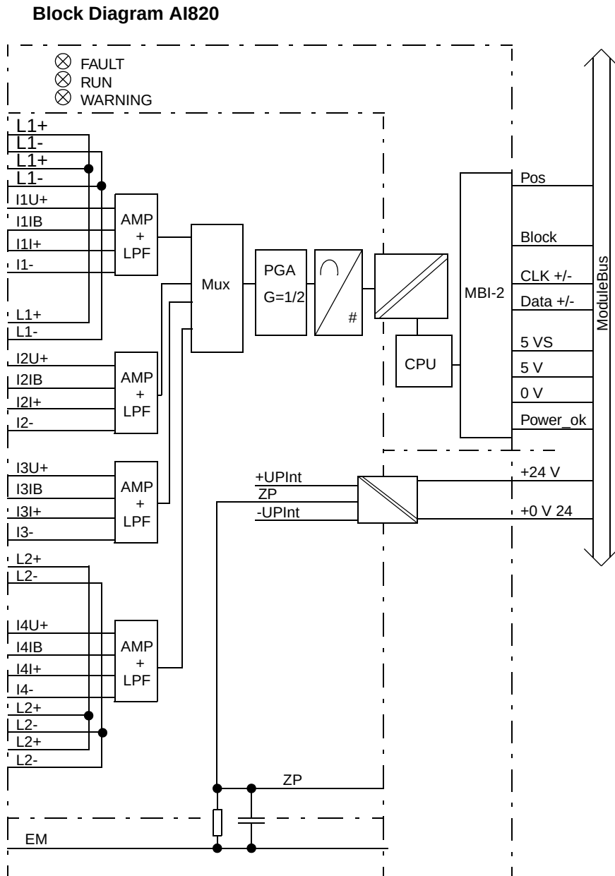
Figure 25. AI820 Block Diagram
