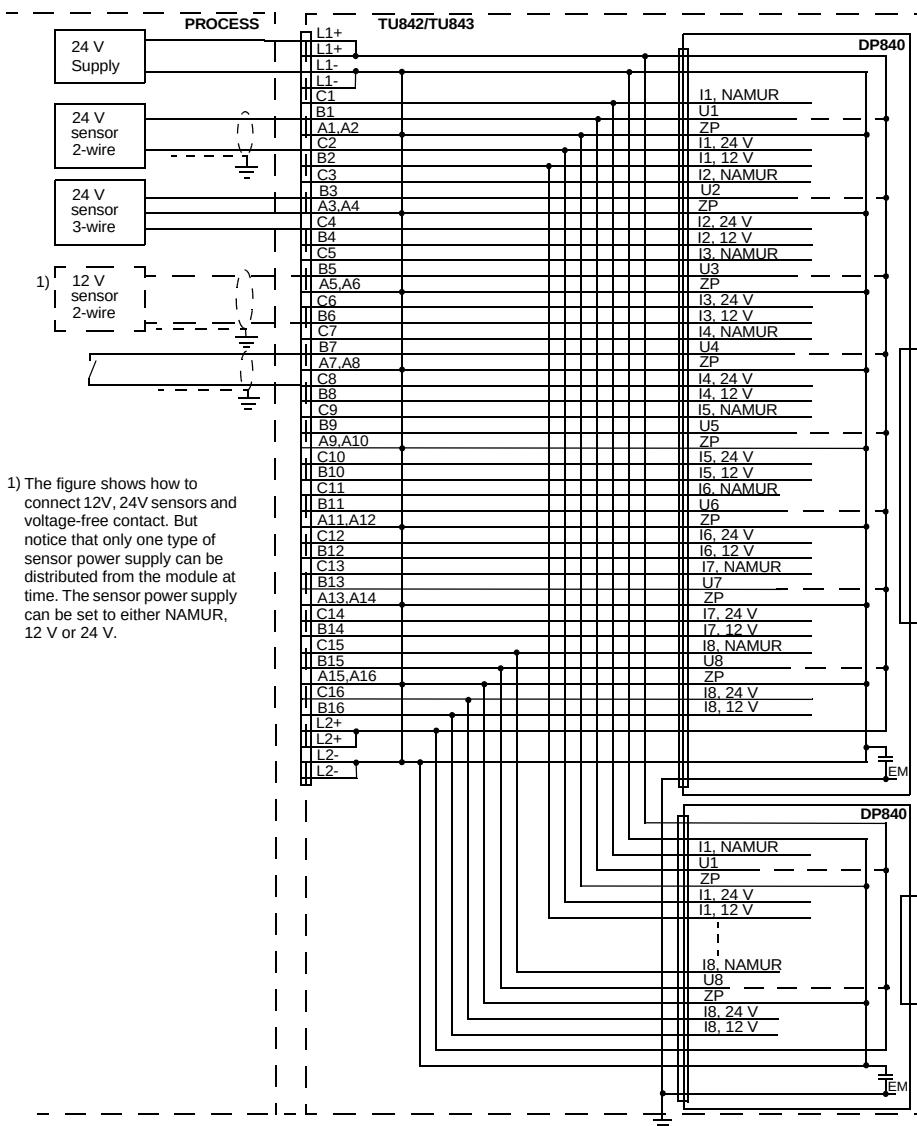
Figure 195. DP840 with TU842 or TU843 MTU Process Connections
