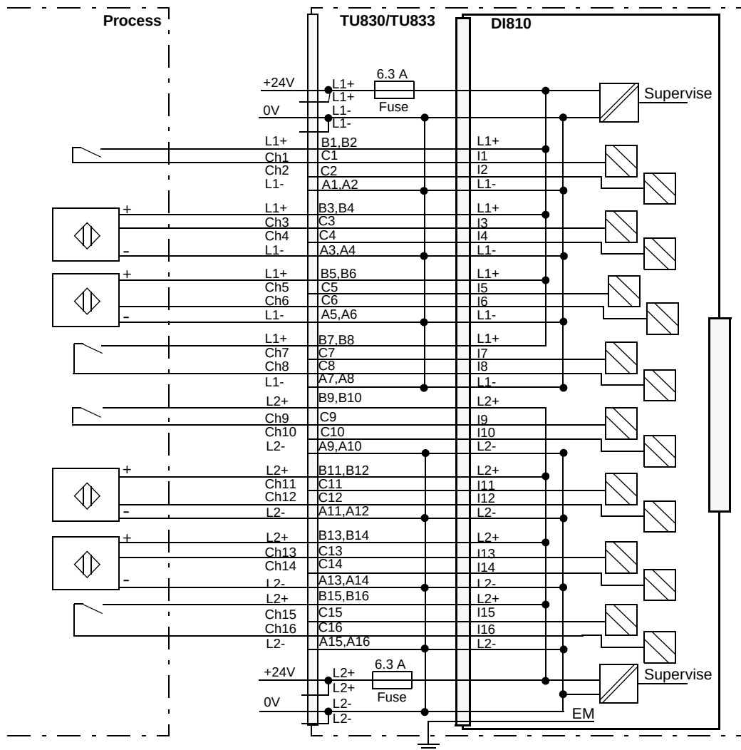
Figure 86. DI810 with TU830 Extended MTU Process Connections
