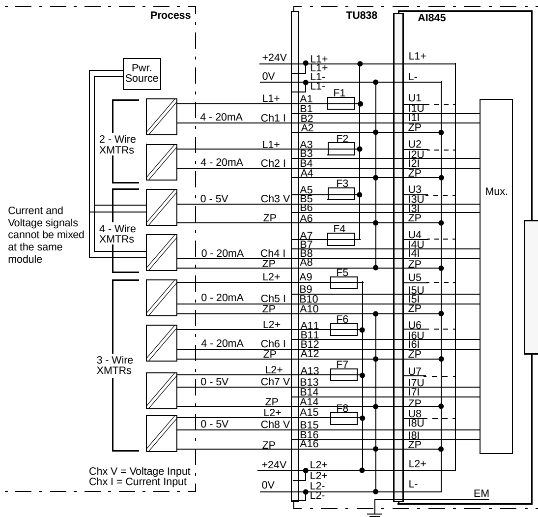
Figure 49. AI845 with TU838 Extended MTU Process Connections
