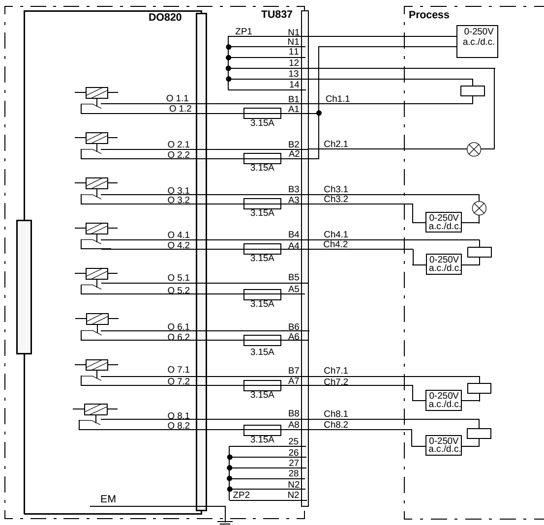
Figure 162. DO820 with TU837 Extended MTU Process Connections
