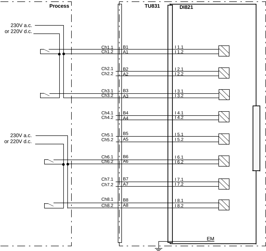
Figure 107. DI821 with TU831 Extended MTU Process Connections
