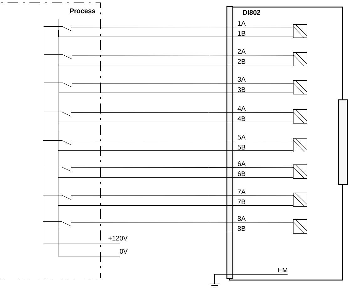
Figure 82. DI802 Process Connections
