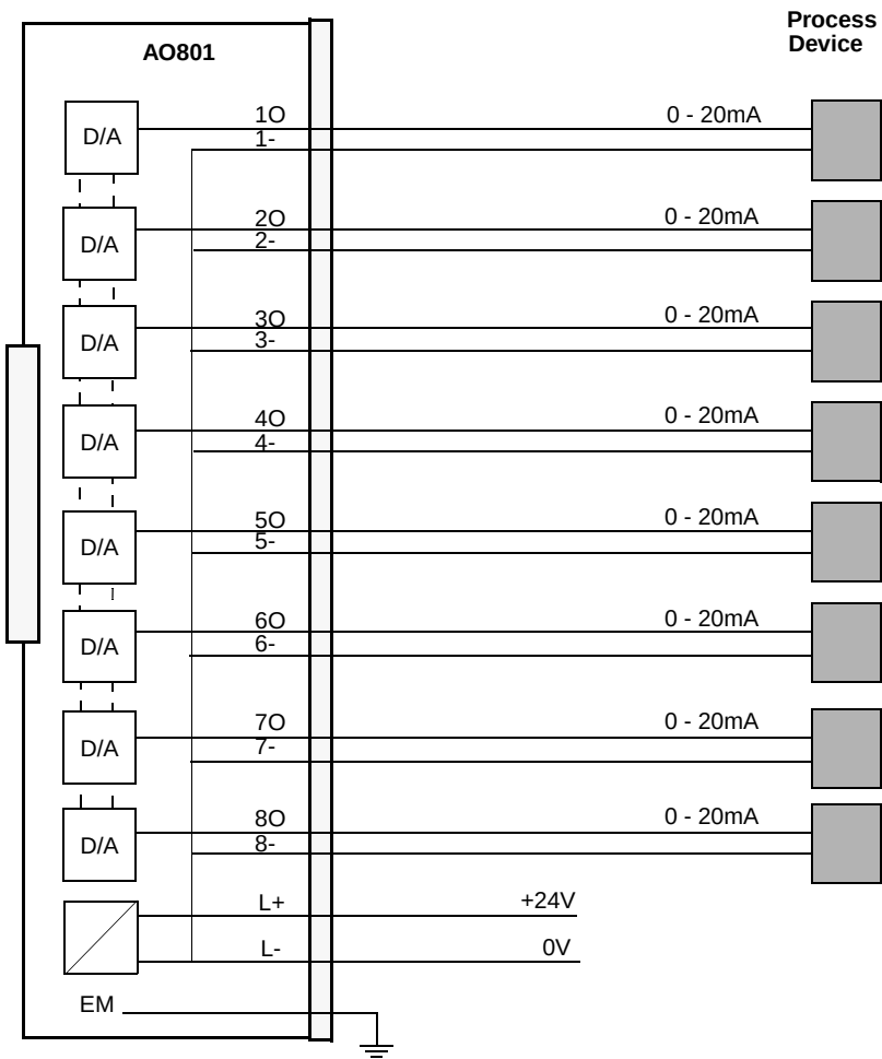
Figure 61. AO801 Process Connections
