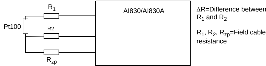
Figure 32. Error dependency of the field cable resistance
