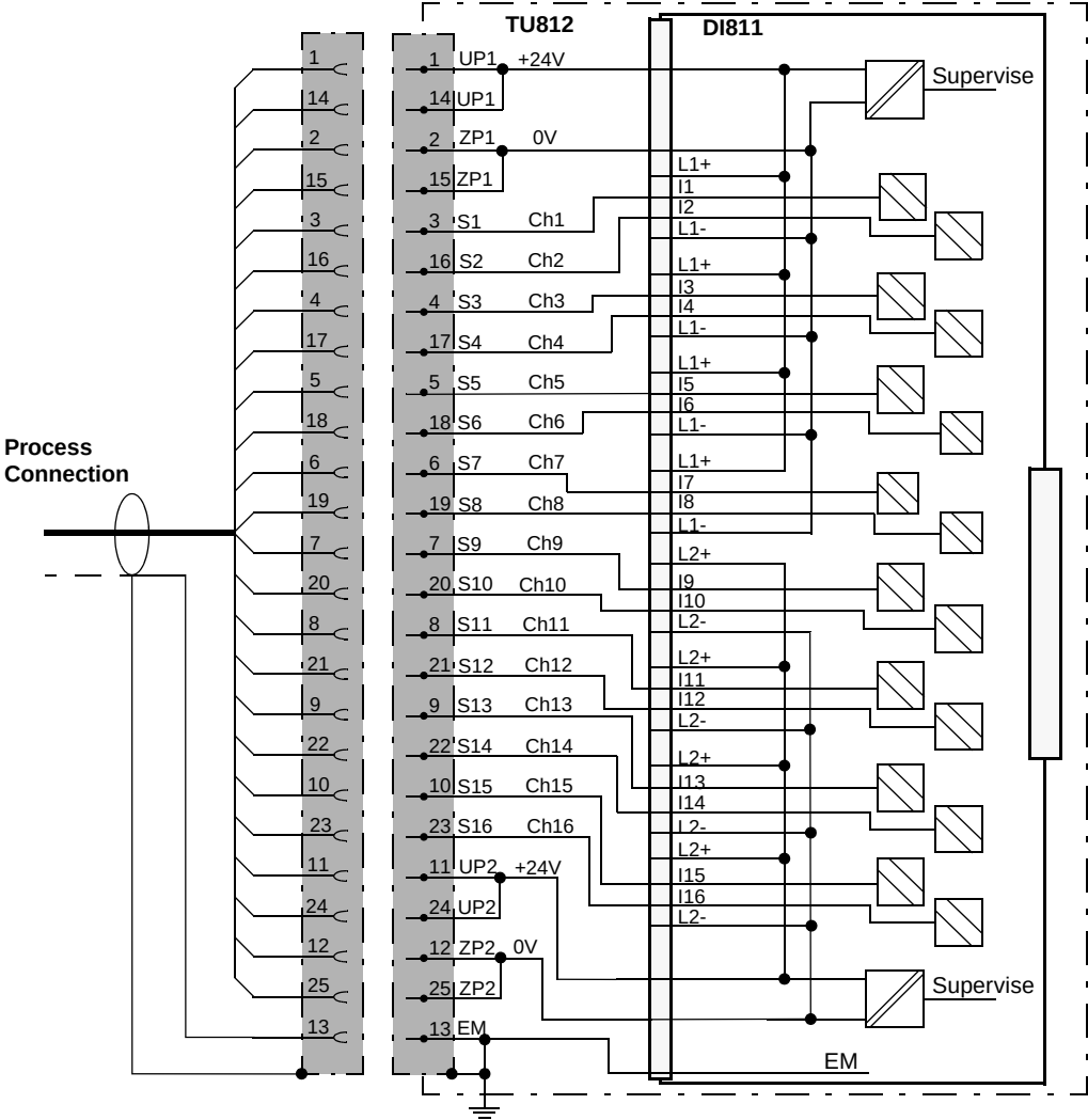
Figure 95. DI811 with TU812
