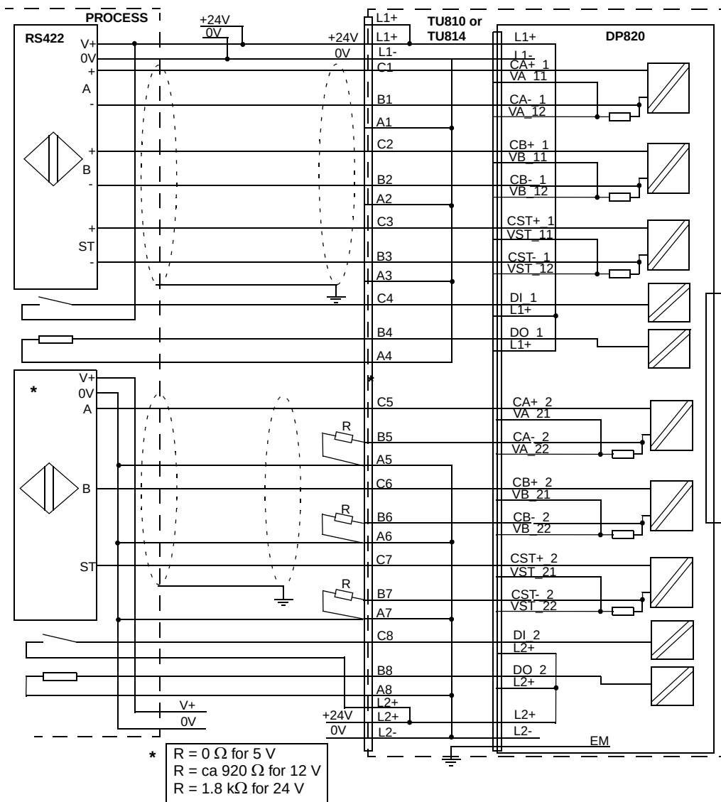
Figure 187. DP820 with TU810 or TU814 MTU Process Connections
