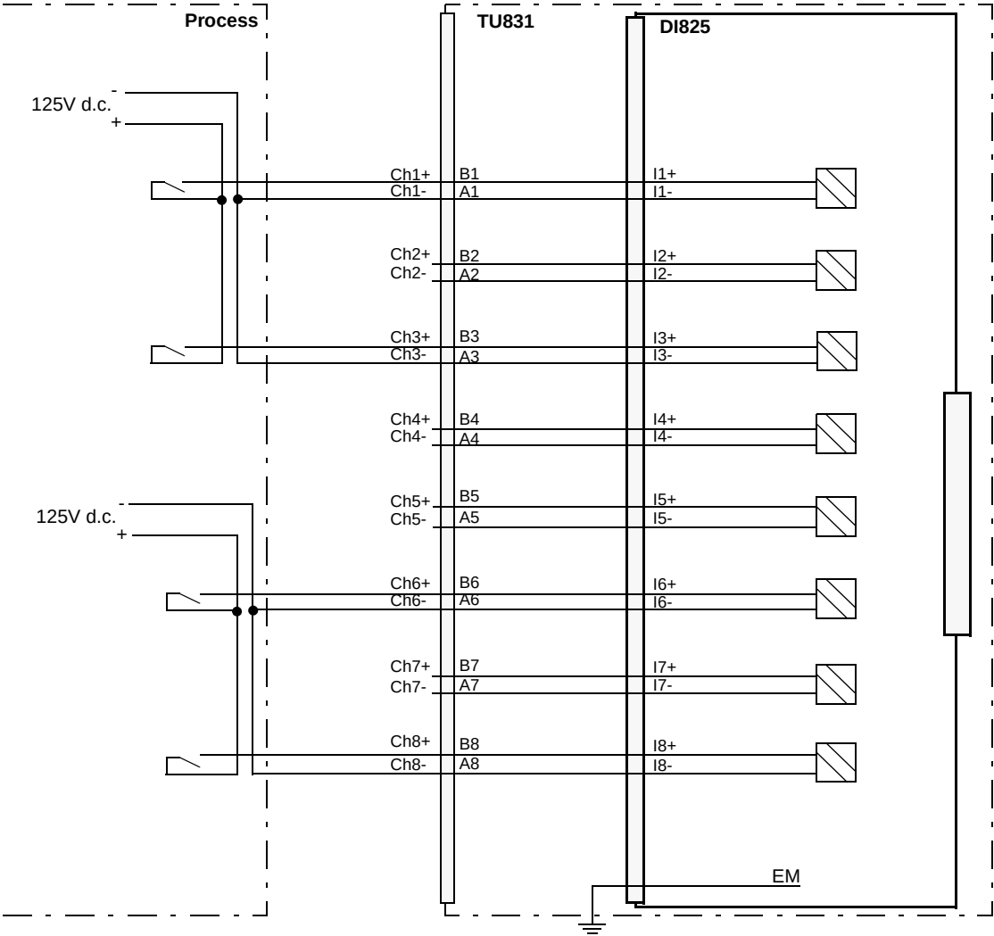
Figure 112. DI825 with TU831 Extended MTU Process Connections
