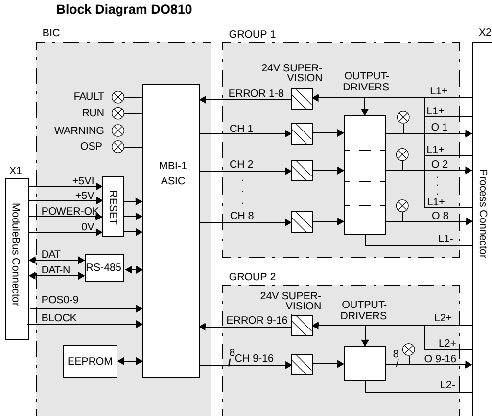
Figure 145. DO810 Block Diagram
