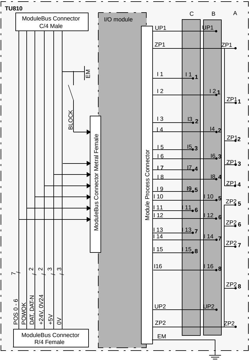
Figure 198. TU810/TU810V1 Block Diagram
