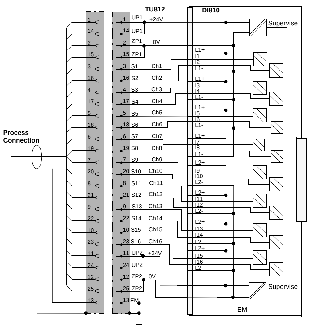
Figure 89. DI810 with TU812 Compact MTU Process Connections
