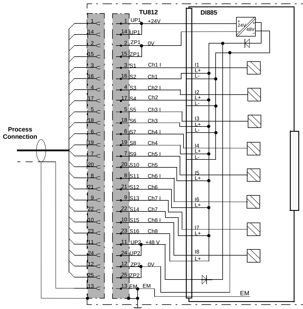
Figure 140. DI885 with TU812 Compact MTU Process Connections
