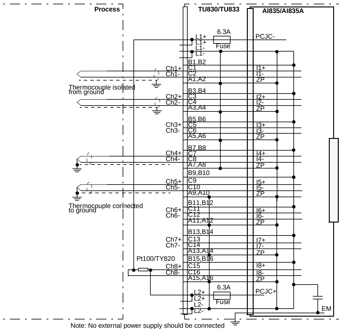
Figure 38. AI835/AI835A with TU830/TU833 Extended MTU Process Connections
