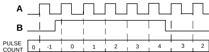
Figure 180. Count/Direction Mode
