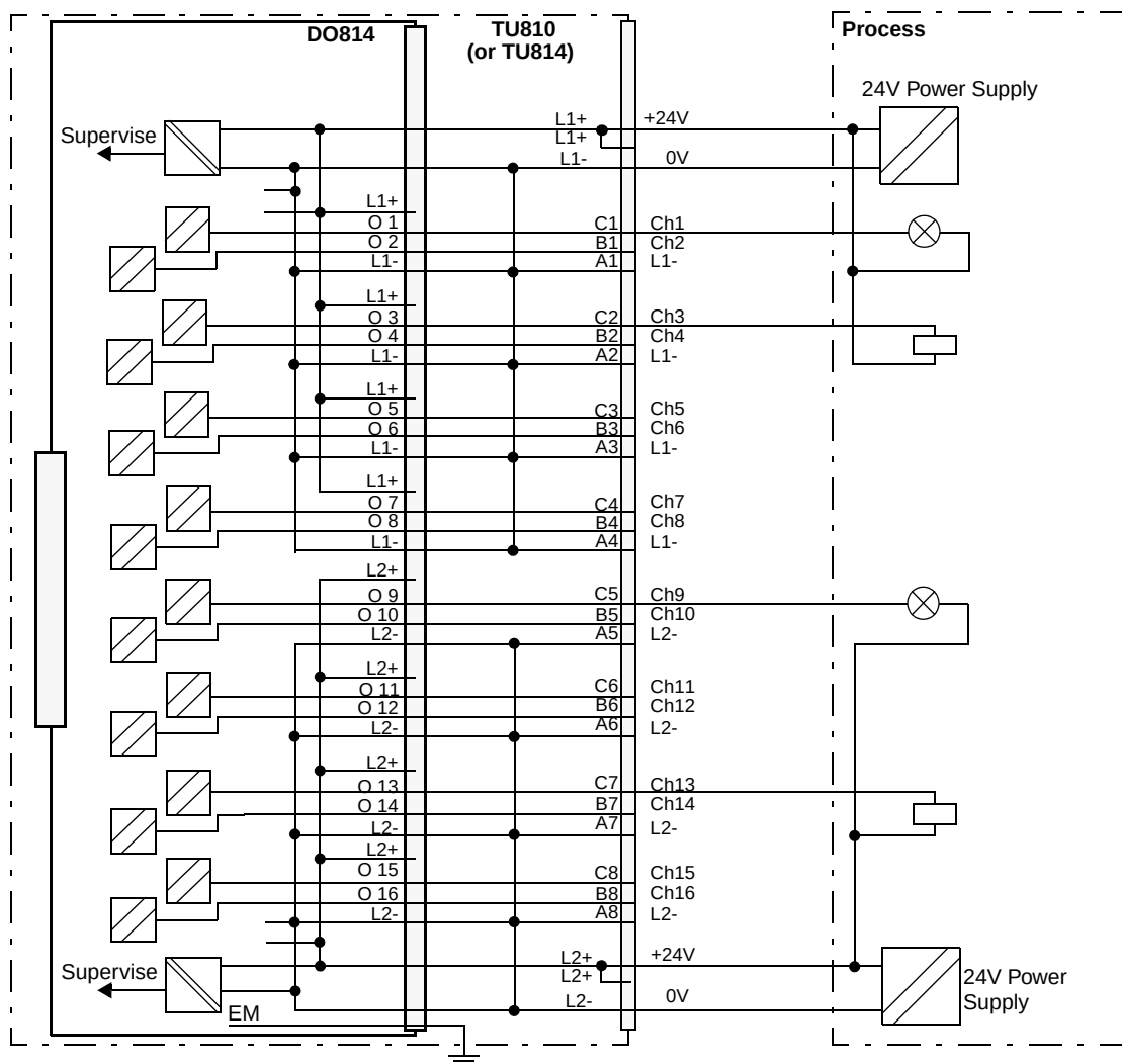
Figure 152. DO814 with TU810 or TU814 Compact MTU Process Connections
