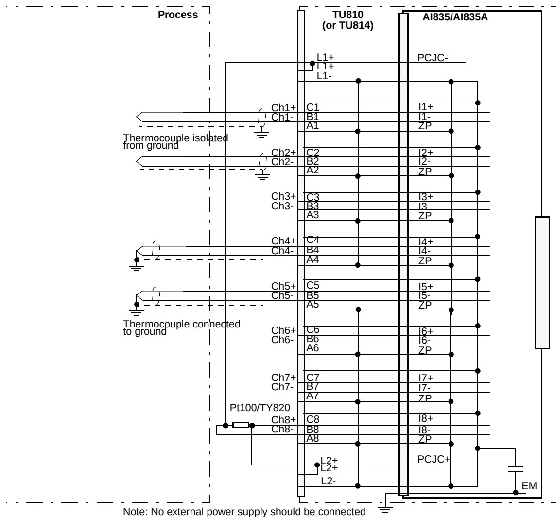
Figure 39. AI835/AI835A with TU810 or TU814 Compact MTU Process Connections
