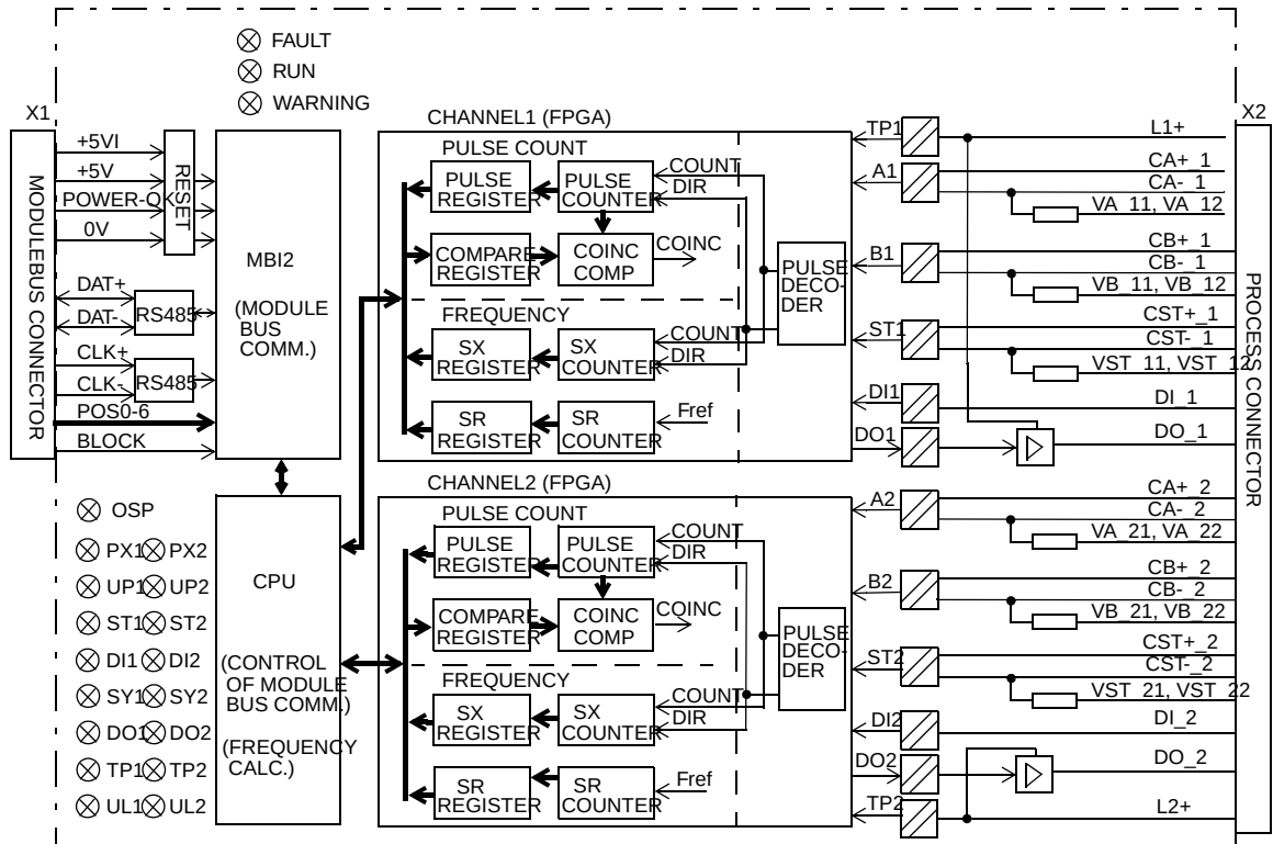
Block Diagram DP820
