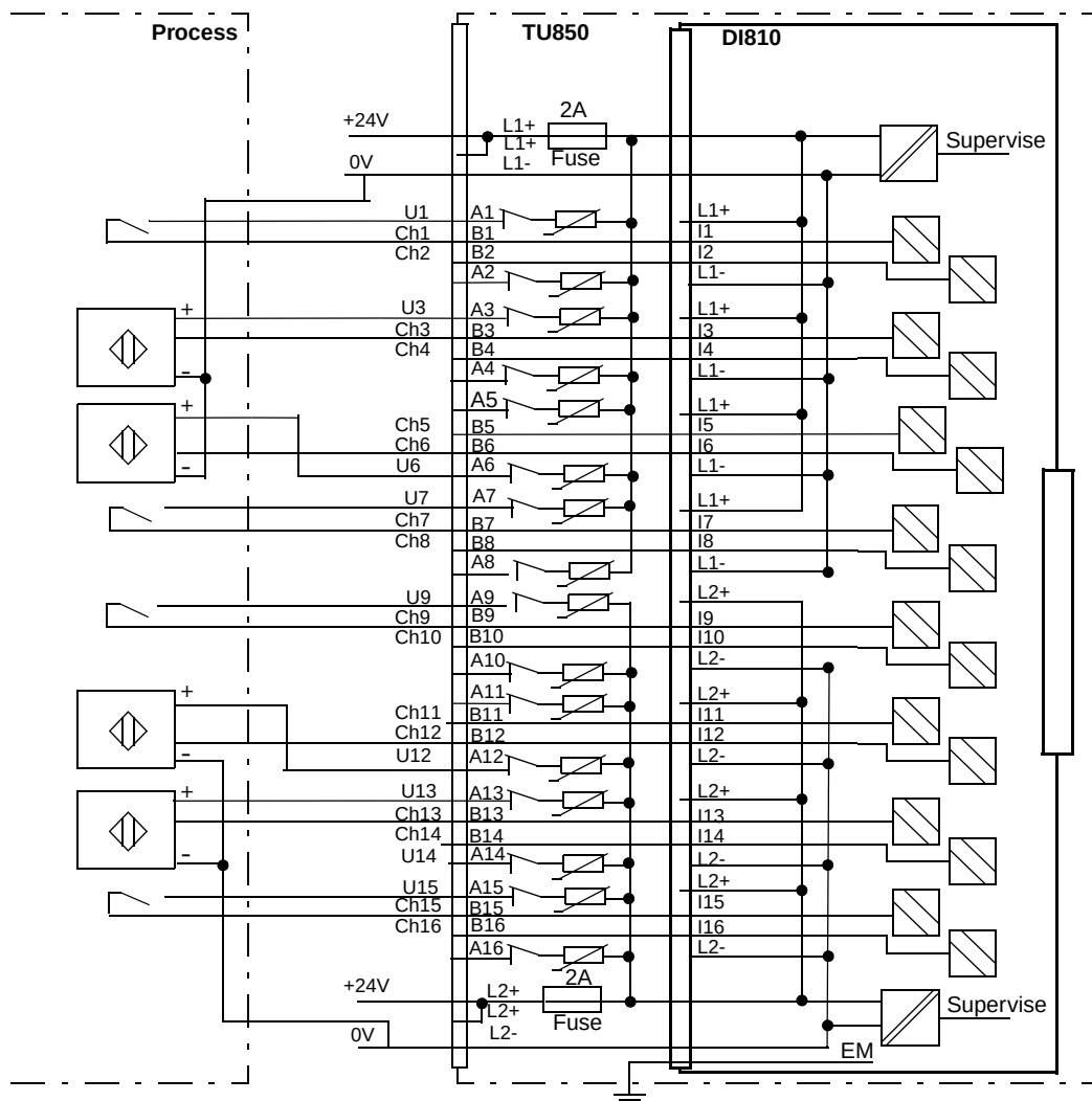
Figure 90. DI810 with TU850 Extended MTU Process Connection
