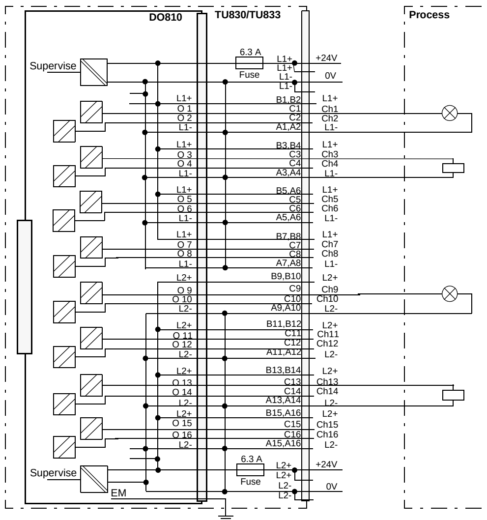
Figure 146. DO810 with TU830/TU833 Extended MTU Process Connections
