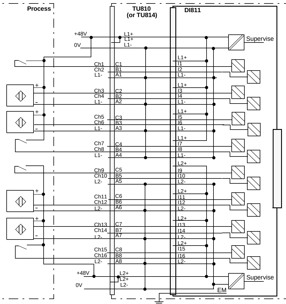
Figure 94. DI811 with TU810 or TU814 Compact MTU Process Connections
