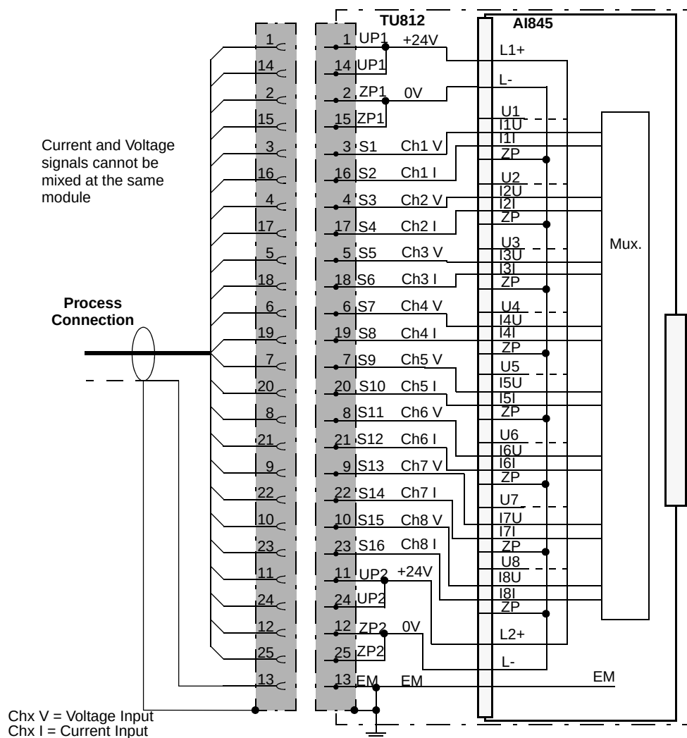
Figure 51. AI845 with TU812 Compact MTU Process Connections
