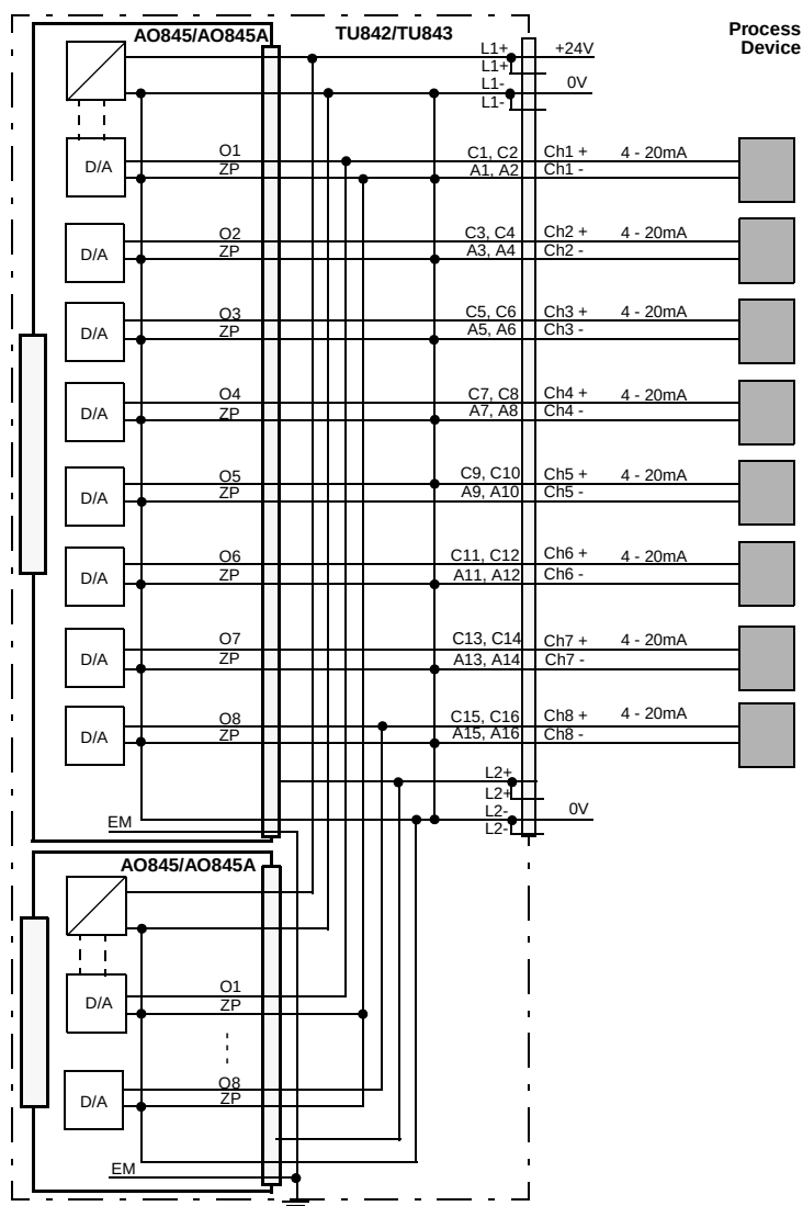
Figure 78. AO845/AO845A with TU842 or TU843 Redundant MTU Process Connections
