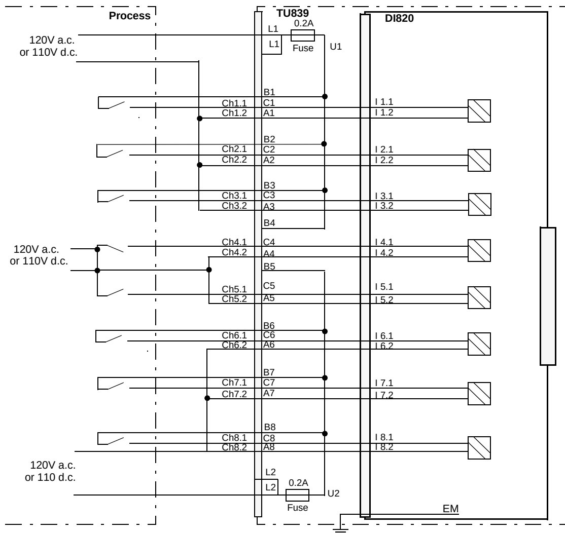
Figure 105. DI820 with TU839 Extended MTU Process Connections
