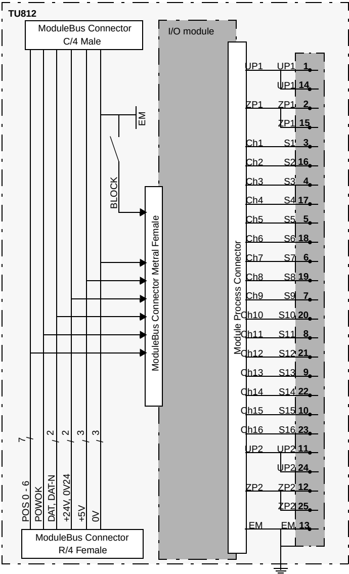
Figure 200. TU812/TU812V1 Block Diagram
