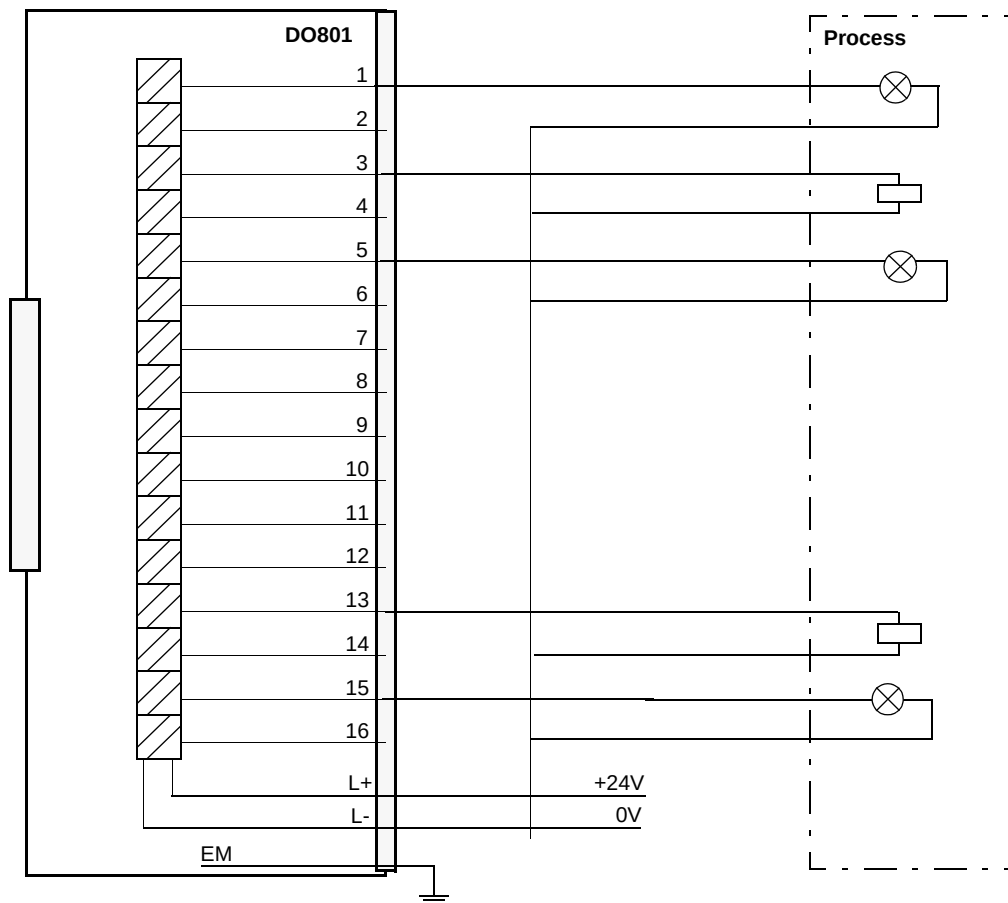
Figure 142. DO801 Process Connections
