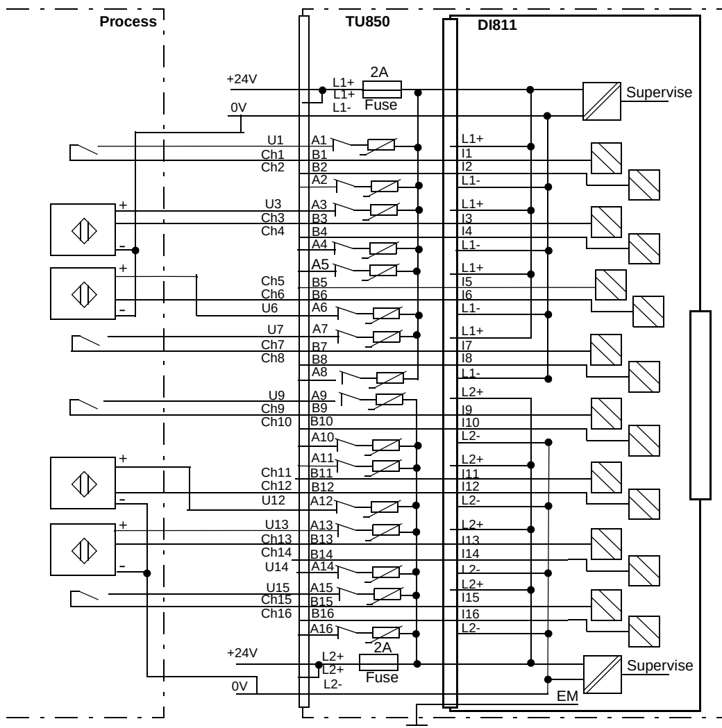
Figure 96. DI811 with TU850 Extended MTU Process Connections
