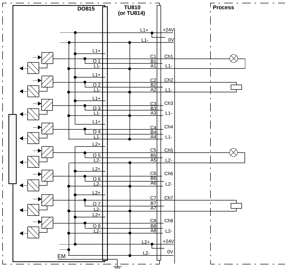
Figure 157. DO815 with TU810 or TU814 Compact MTU Process Connections
