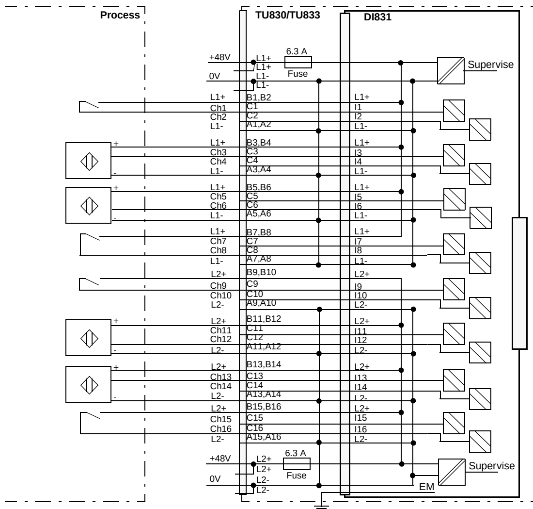
Figure 121. DI831 with TU830 Extended MTU Process Connections
