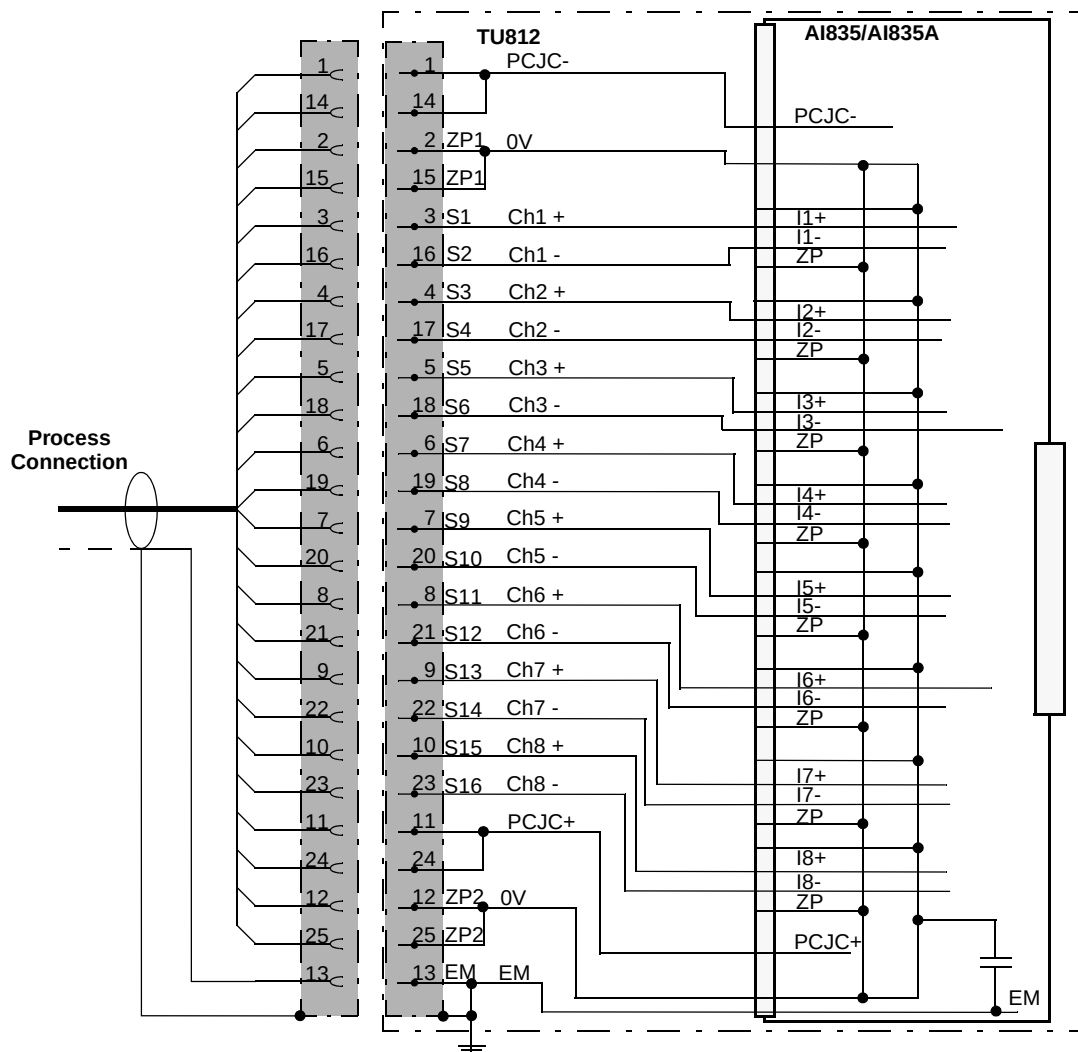
Figure 41. AI835/AI835A with TU812 Compact MTU Process Connections
