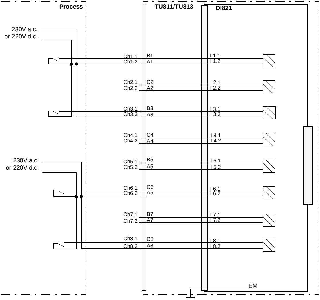
Figure 108. DI821 with TU811 or TU813 Compact MTU Process Connections
