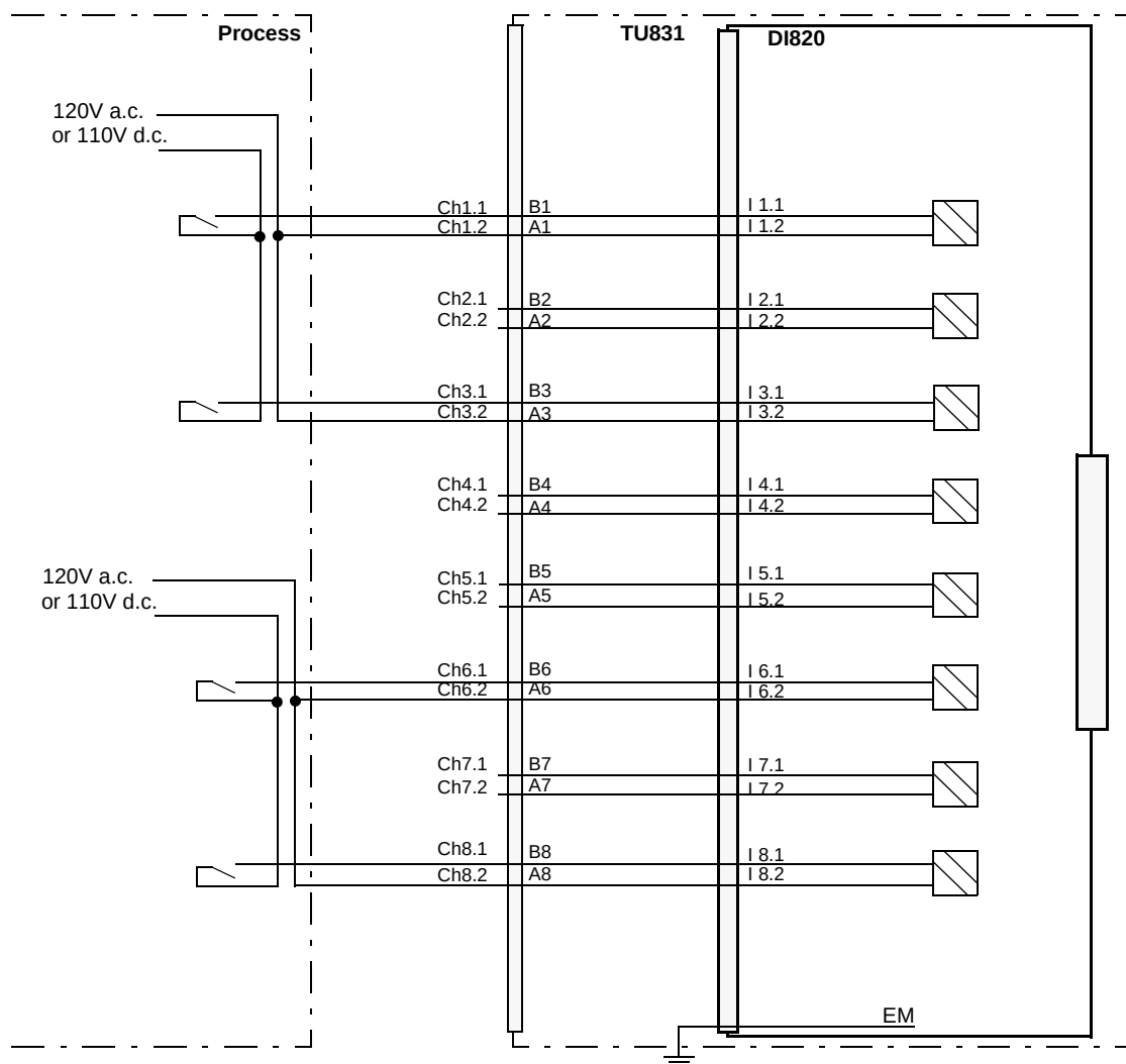
Figure 103. DI820 with TU831 Extended MTU Process Connections
