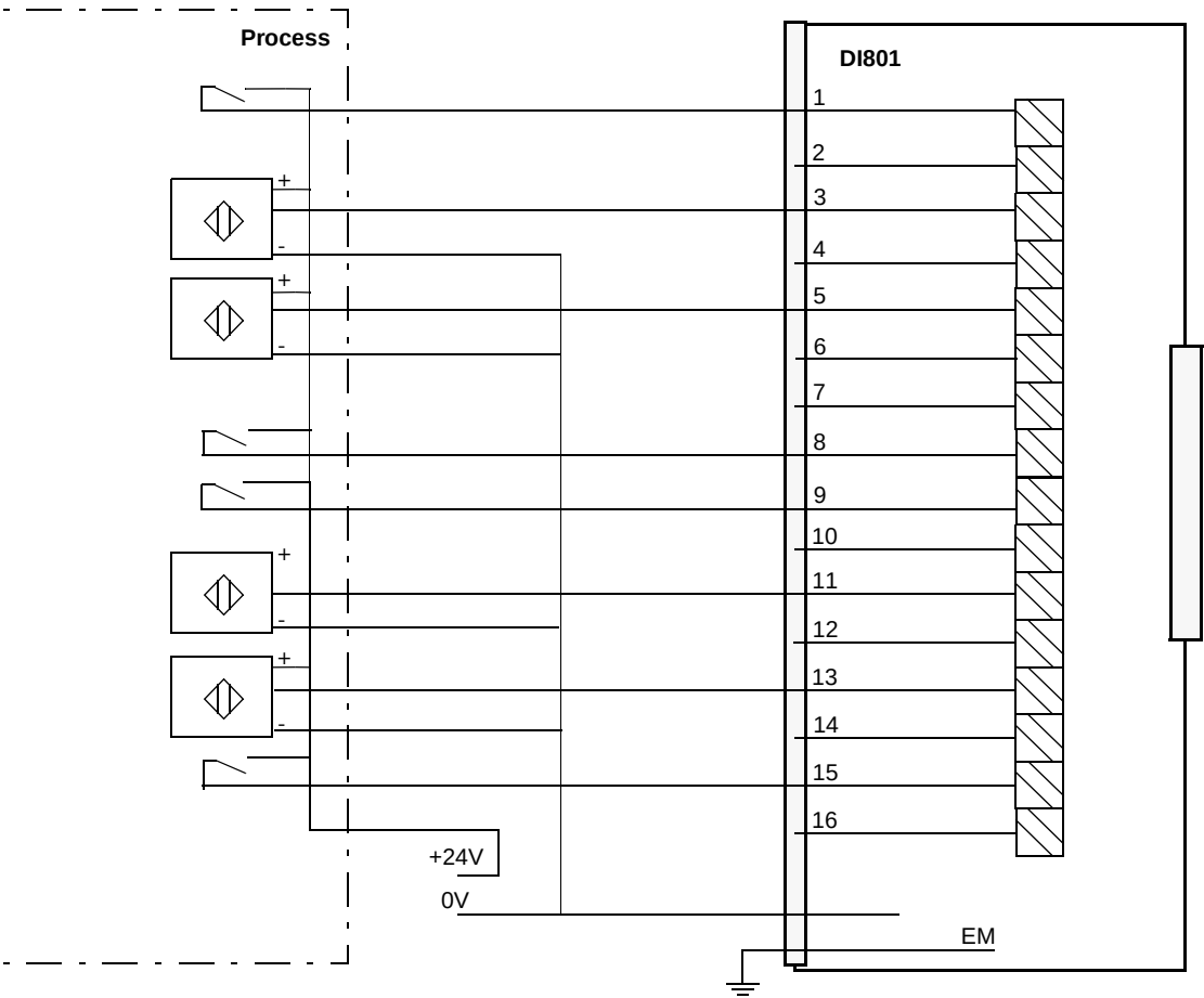
Figure 80. DI801 Process Connections
