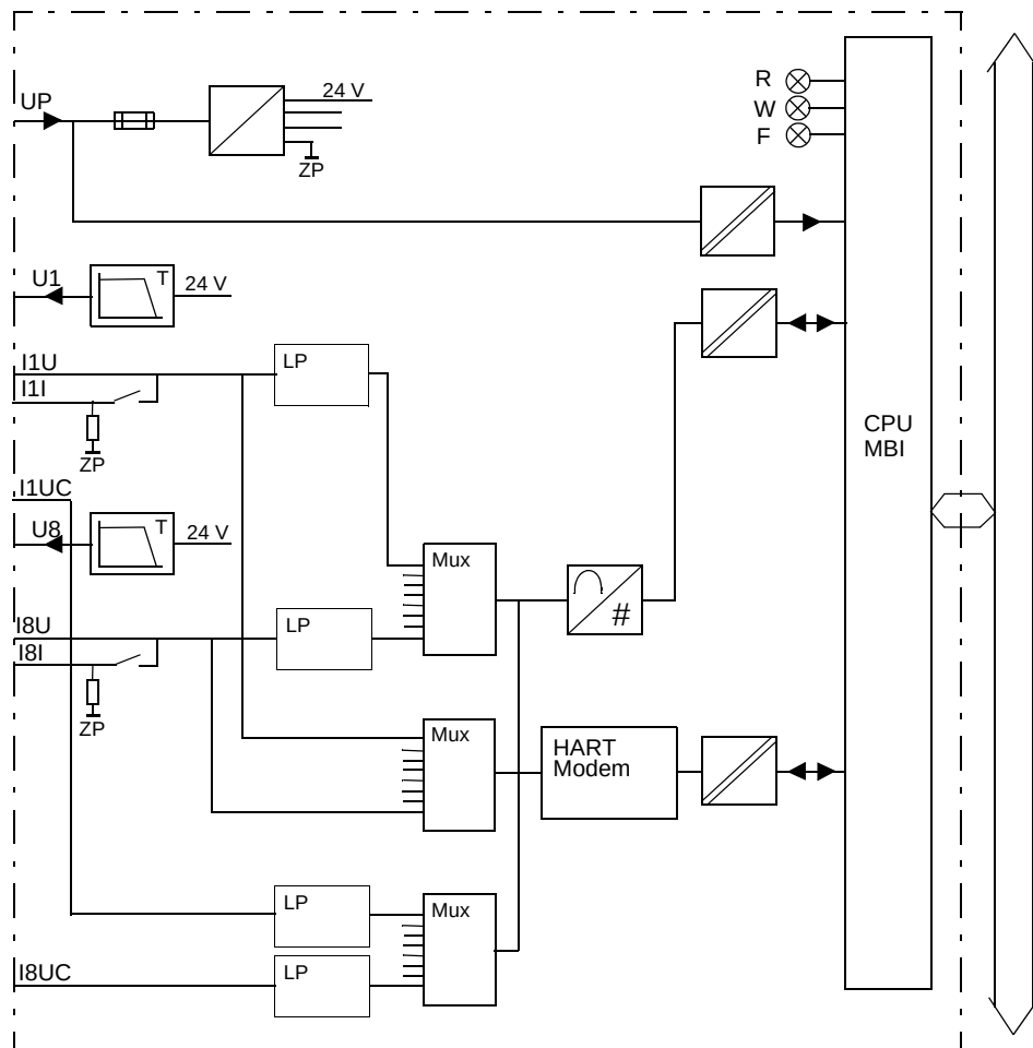
Figure 46. AI845 Block Diagram
