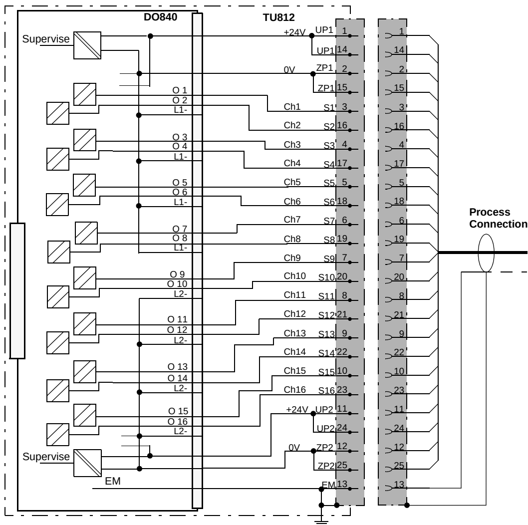
Figure 171. DO840 with TU812 Compact MTU Process Connections
