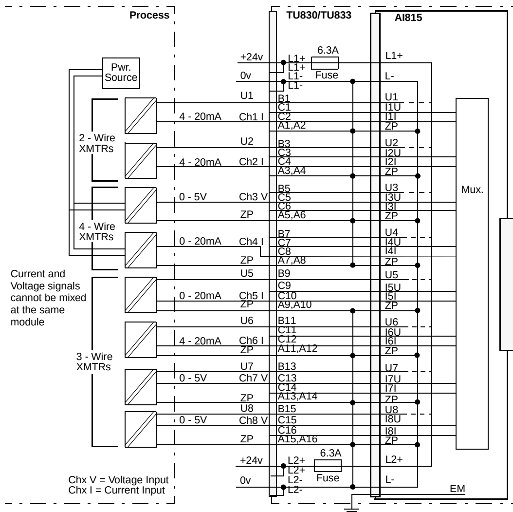
Figure 20. AI815 with TU830/TU833 Extended MTU Process Connections
