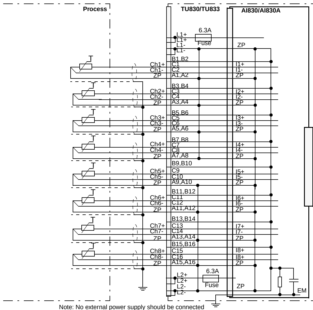
Figure 34. AI830/AI830A with TU830 Extended MTU Process Connections
