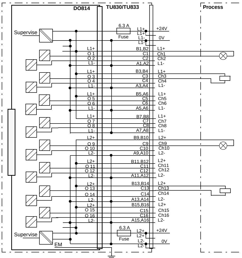
Figure 150. DO814 with TU830/TU833 Extended MTU Process Connections
