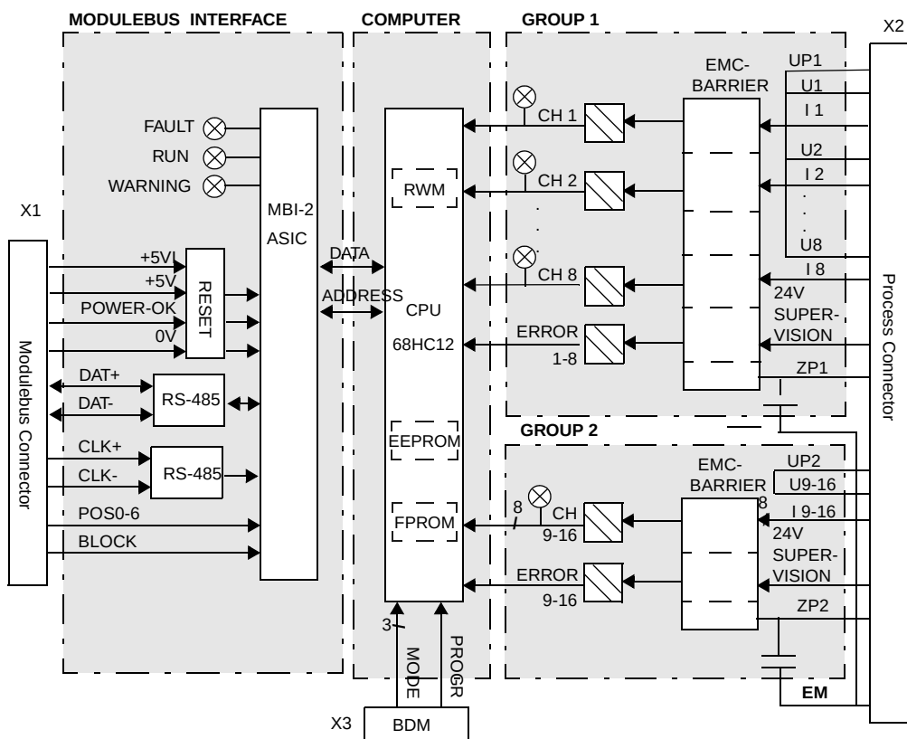
Figure 120. DI831 Block Diagram
