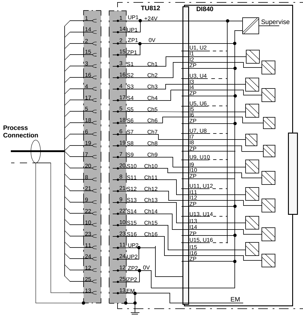
Figure 130. DI840 with TU812 Compact MTU Process Connections
