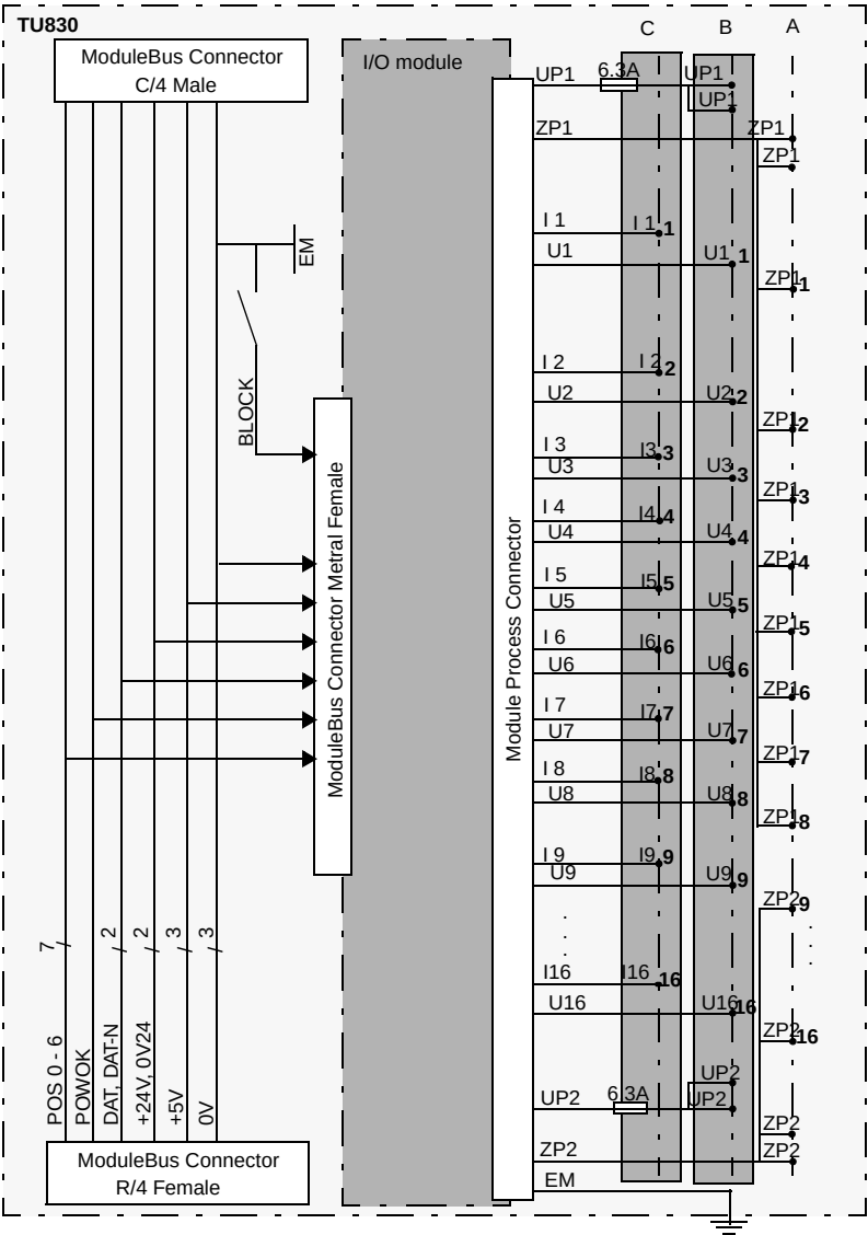
Figure 205. TU830/TU830V1 Block Diagram
