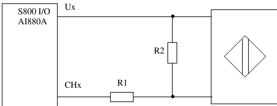
Figure 54. Field Loop Arrangement
