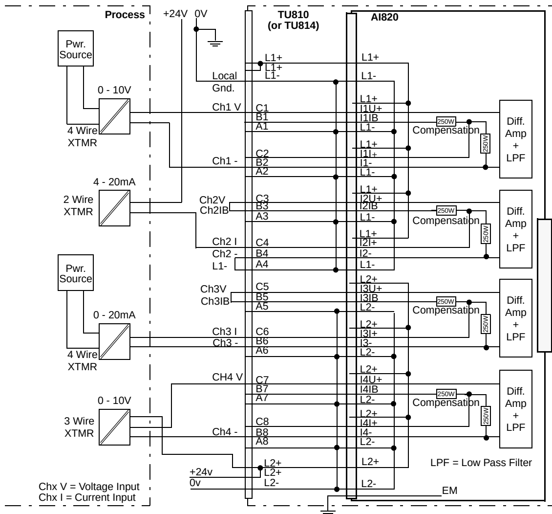
Figure 27. AI820 with TU810 or TU814 Compact MTU Process Connections
