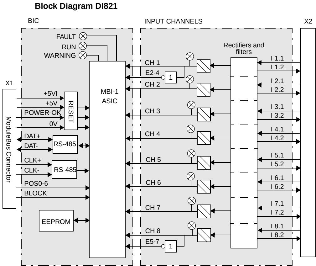
Figure 106. DI821 Block Diagram
