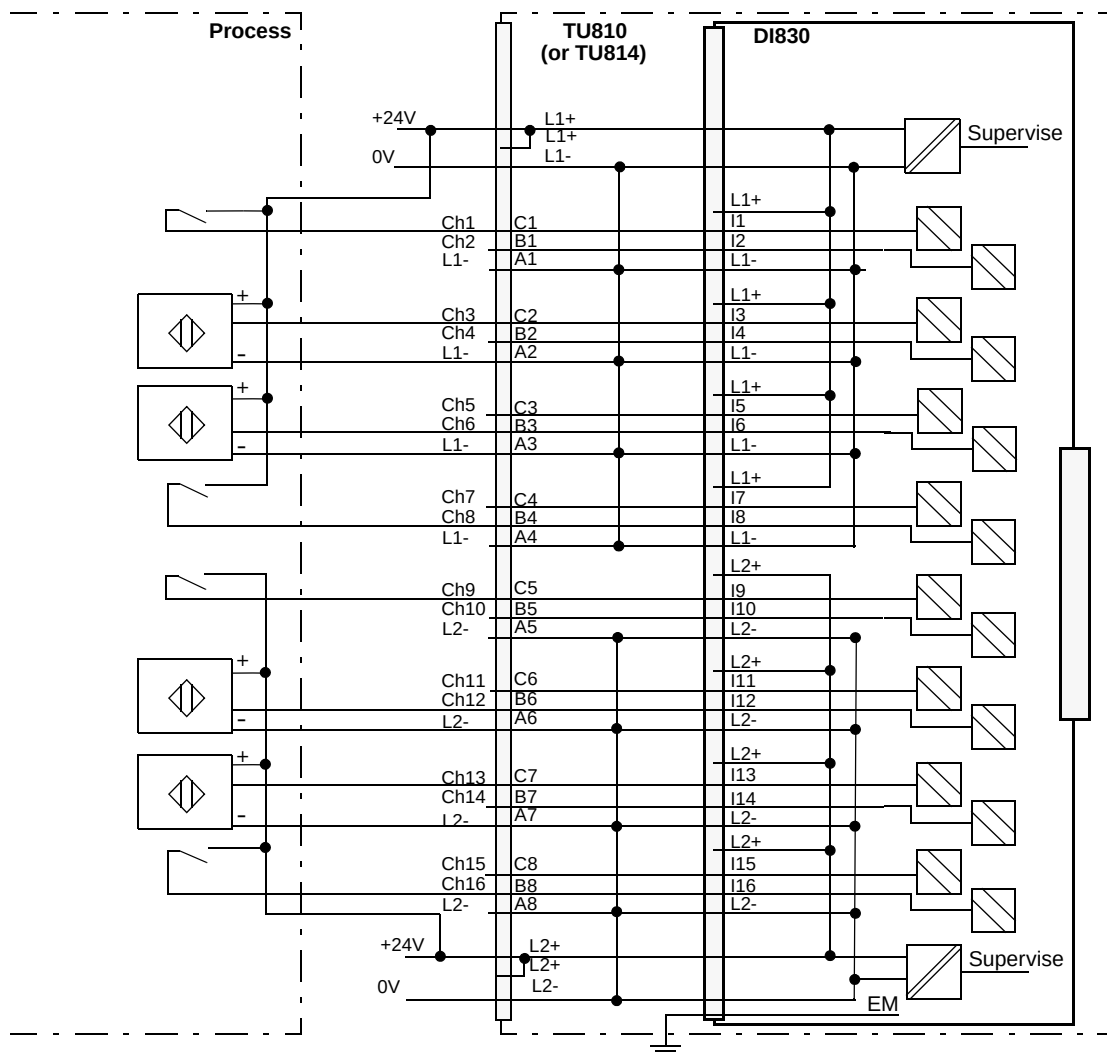
Figure 117. DI830 with TU810 or TU814 Compact MTU Process Connections
