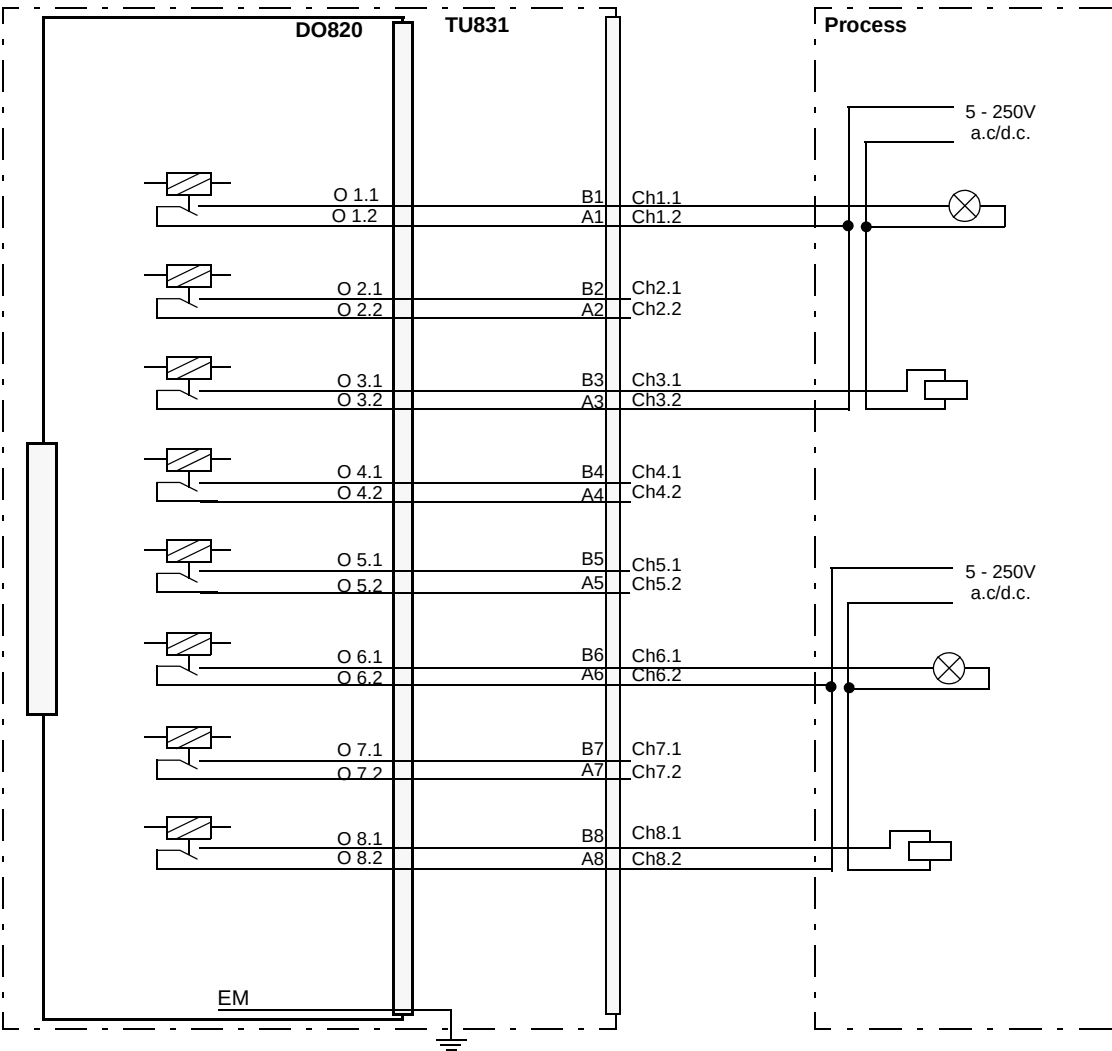
Figure 159. DO820 with TU831 Extended MTU Process Connections
