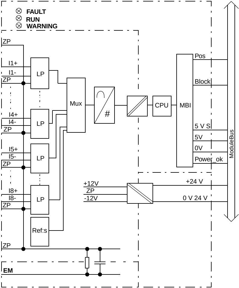
Figure 33. AI830/AI830A Block Diagram
