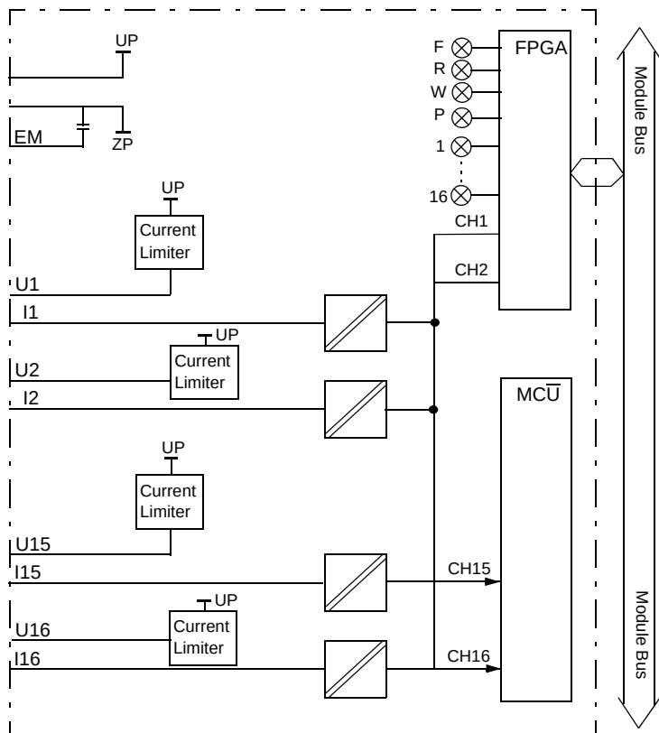
Figure 132. DI880 Block Diagram
