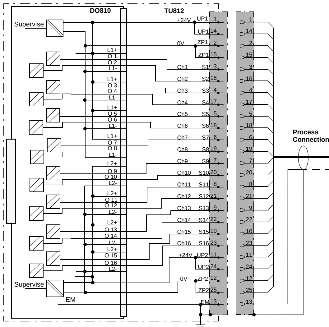
Figure 148. DO810 with TU812 Compact MTU Process Connections
