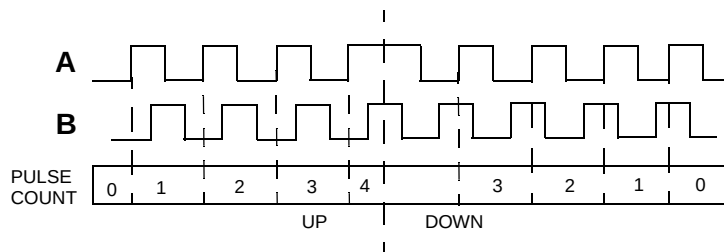
Figure 181. Quadrature Mode, #1 (Count on Pos. Edge Input A)
