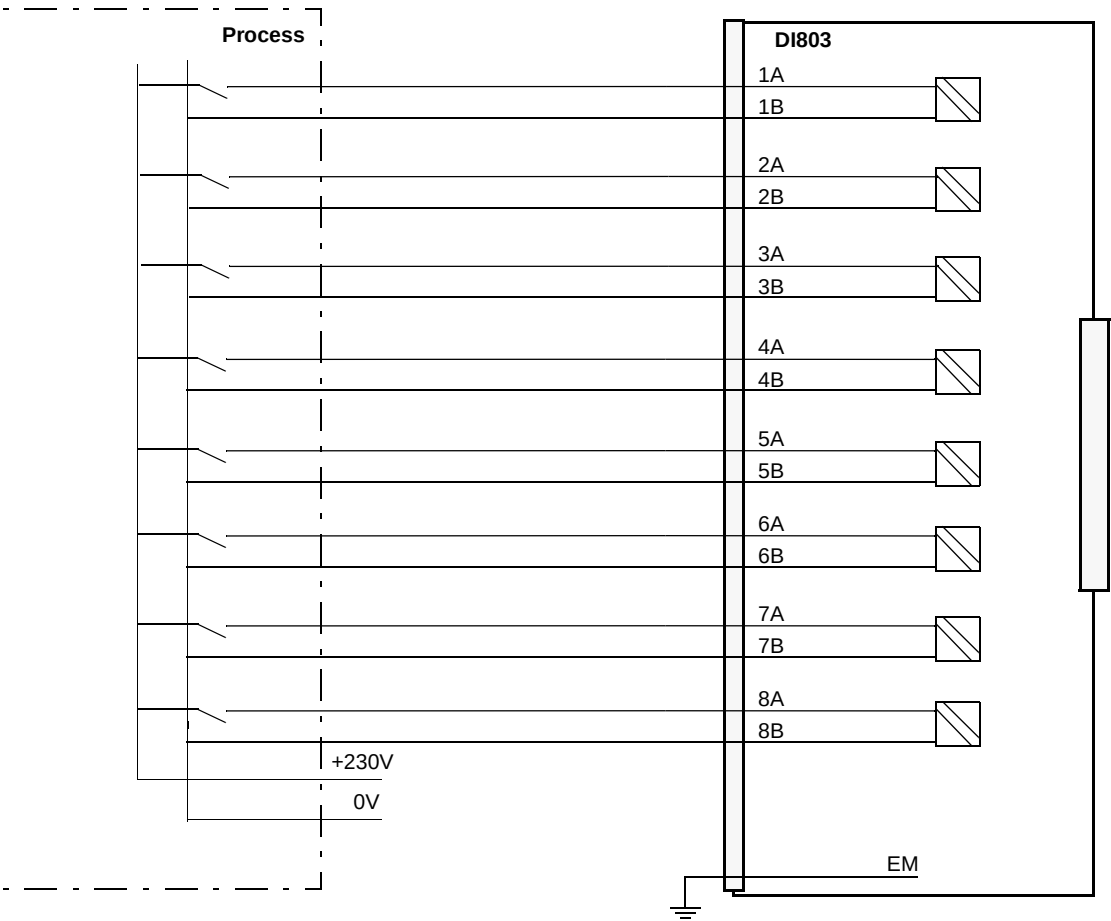
Figure 84. DI803 Process Connections
