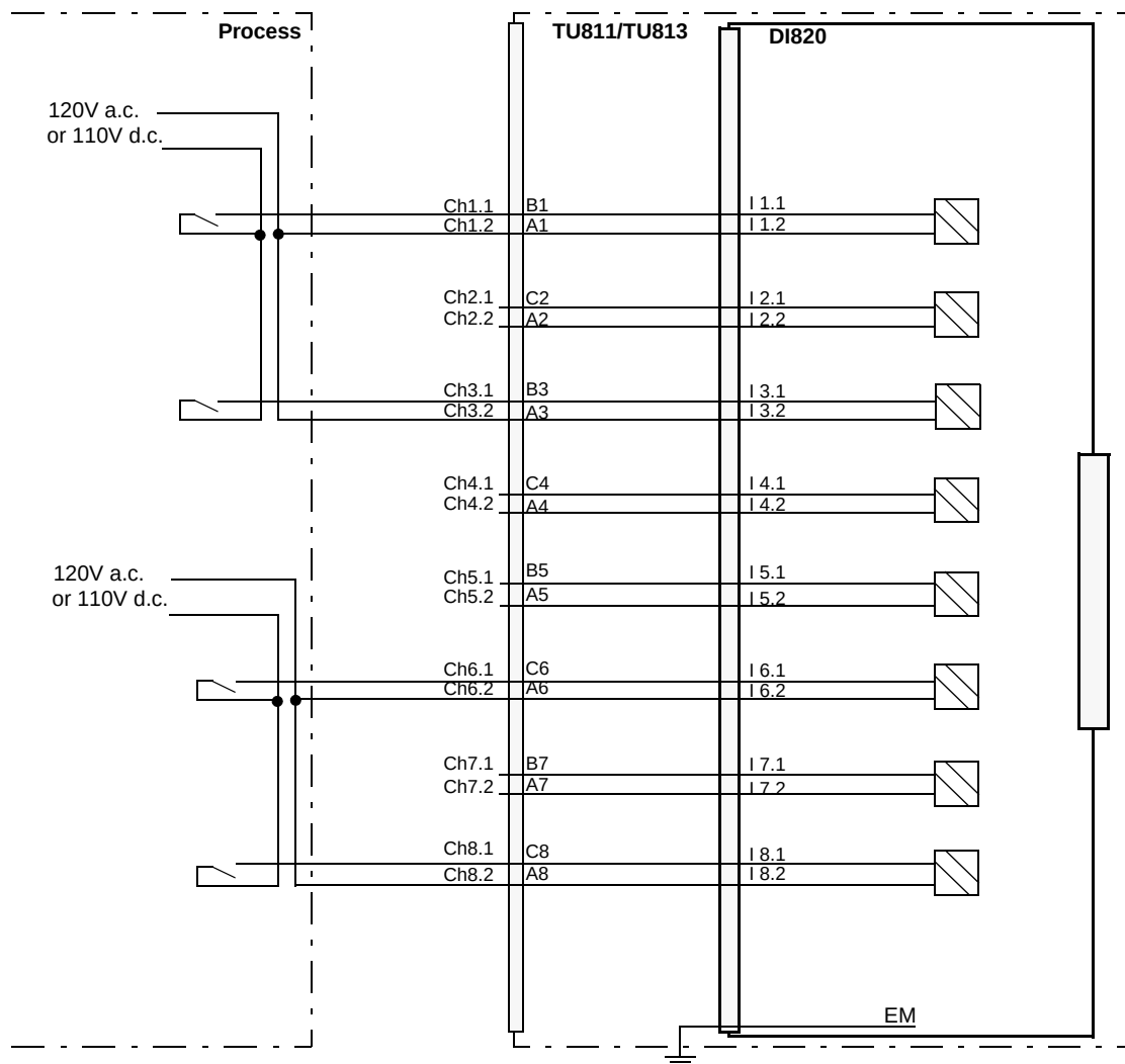
Figure 104. DI820 with TU811 or TU813 Compact MTU Process Connections
