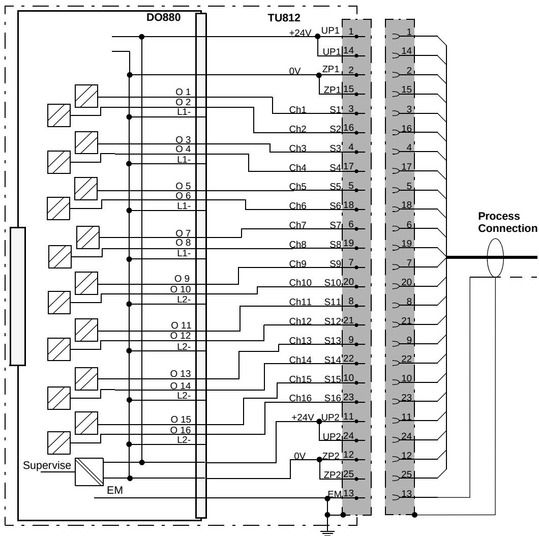
Figure 177. DO880 with TU812 Compact MTU Process Connections
