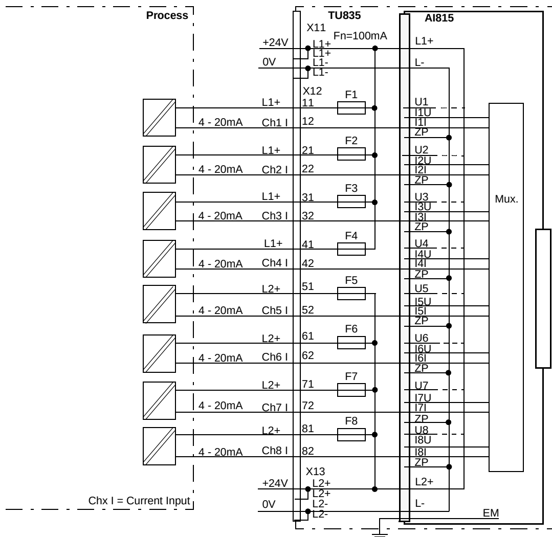
Figure 21. AI815 with TU835 Extended MTU Process Connections
