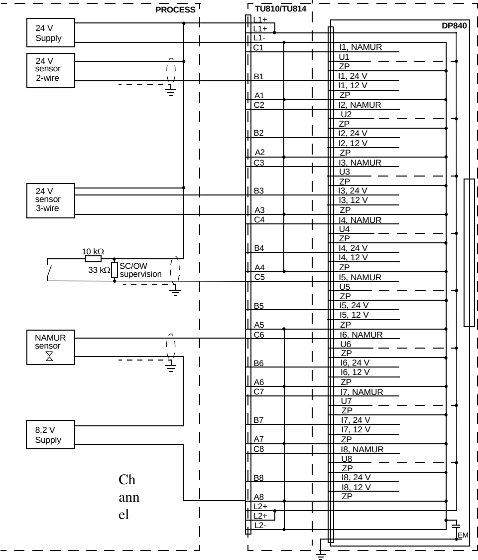
Figure 192. DP840 with TU810 or TU814 MTU Process Connections
