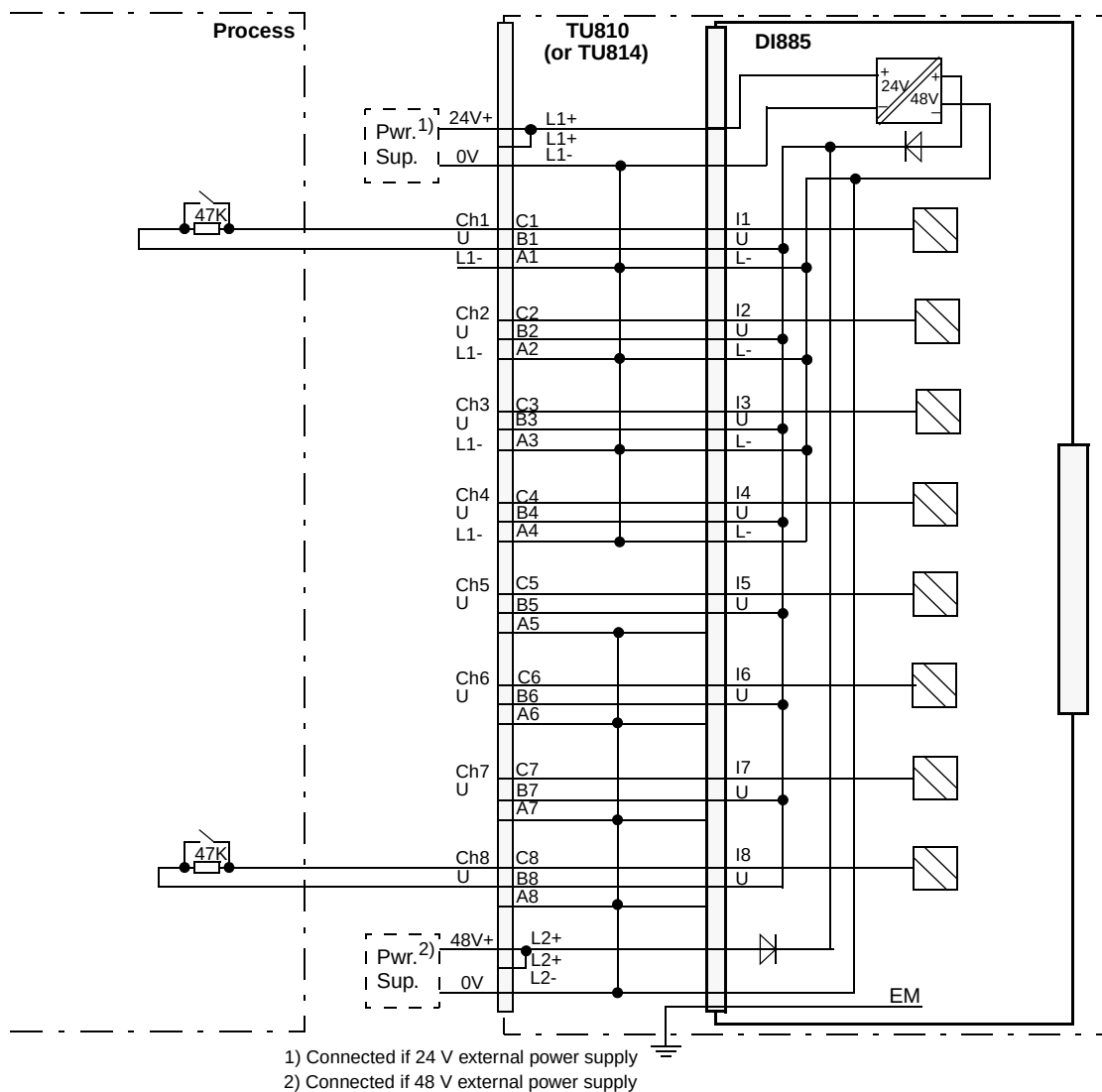
Figure 139. DI885 with TU810 or TU814 Compact MTU Process Connections
