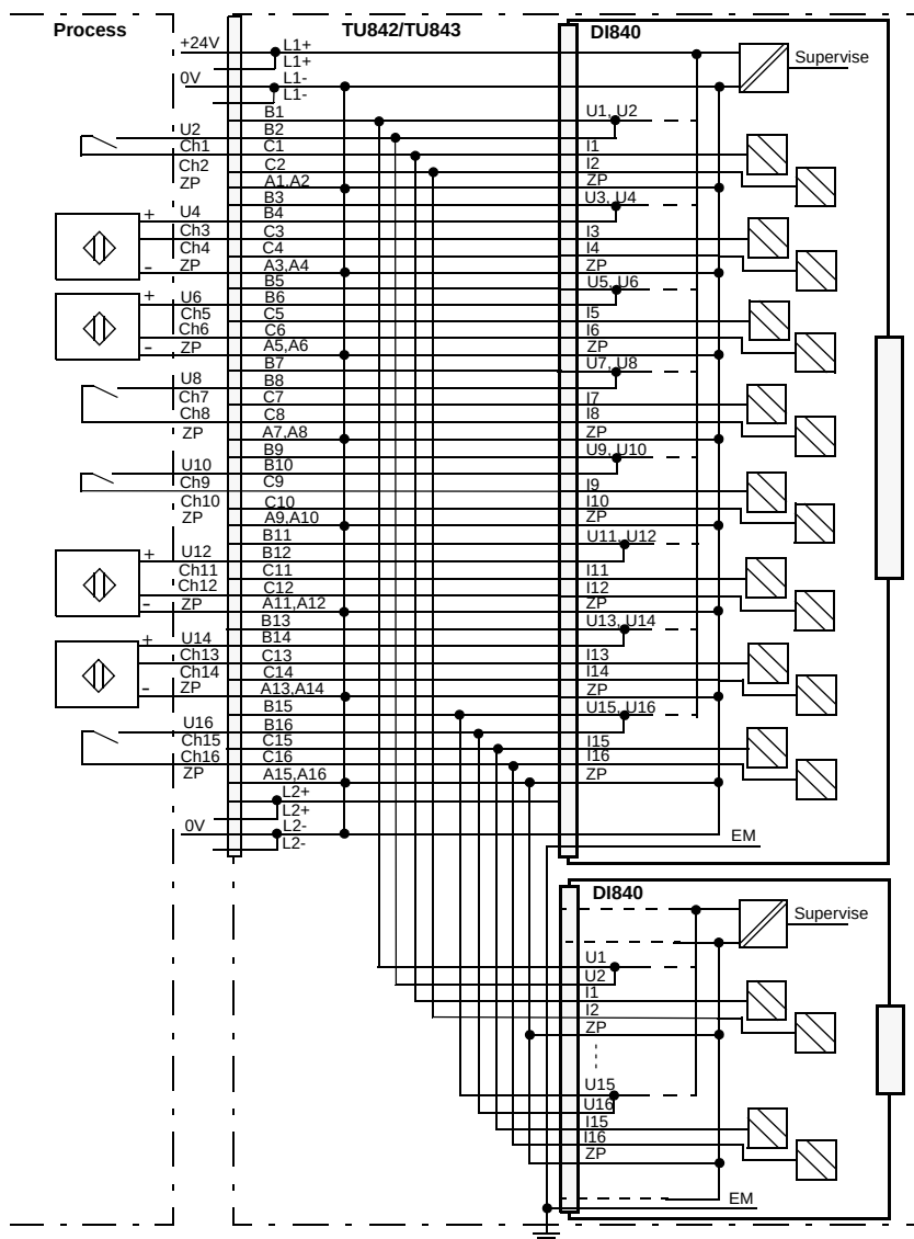
Figure 131. DI840 with TU842 or TU843 Redundant MTU Process Connections
