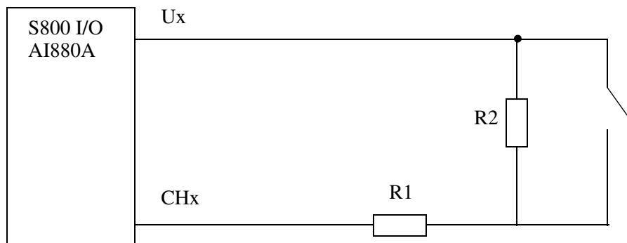
Figure 53. Field Loop Arrangement When using the function Loop Supervised DI
