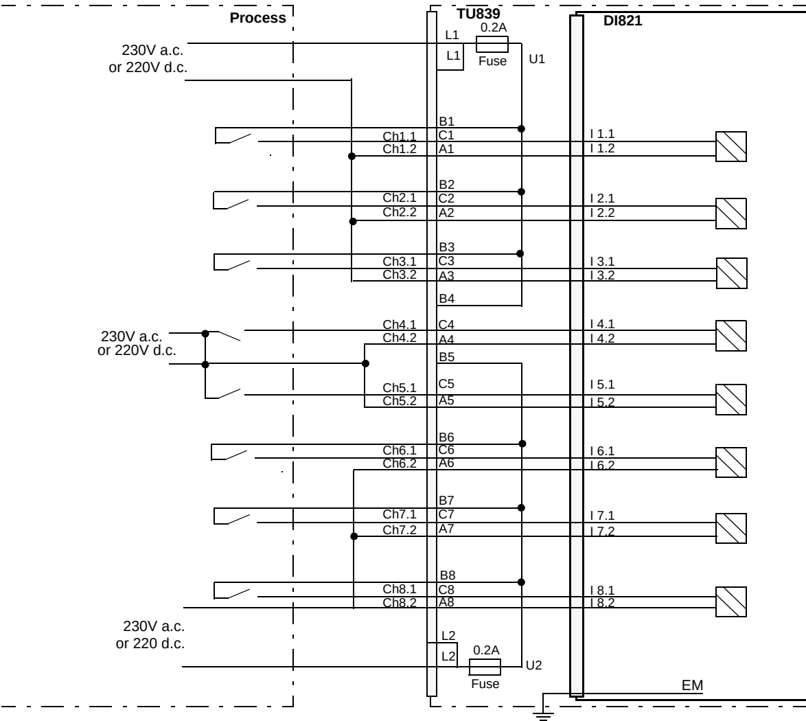
Figure 109. DI821 with TU839 Extended MTU Process Connections
