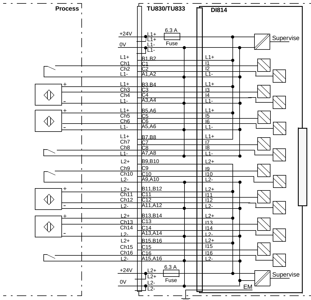
Figure 98. DI814 with TU830 Extended MTU Process Connections
