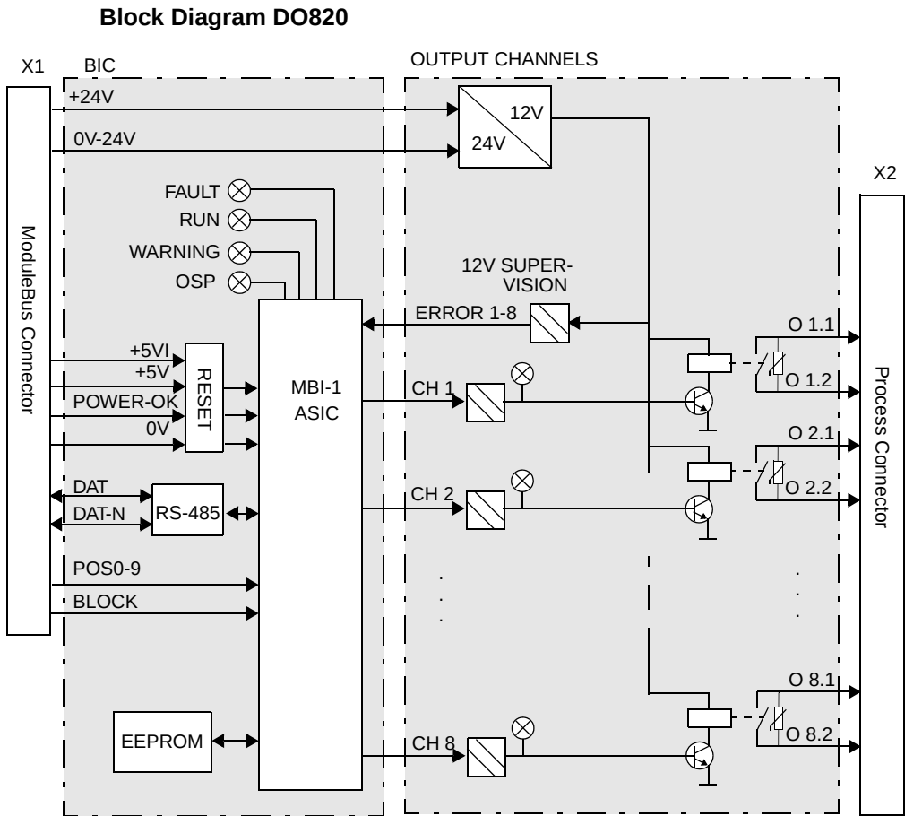
Figure 158. DO820 Block Diagram
