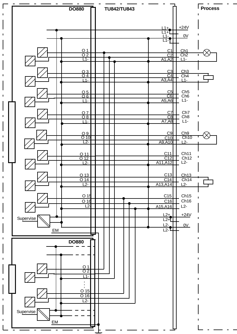
Figure 178. DO880 with TU842 or TU843 Redundant MTU Process Connections
