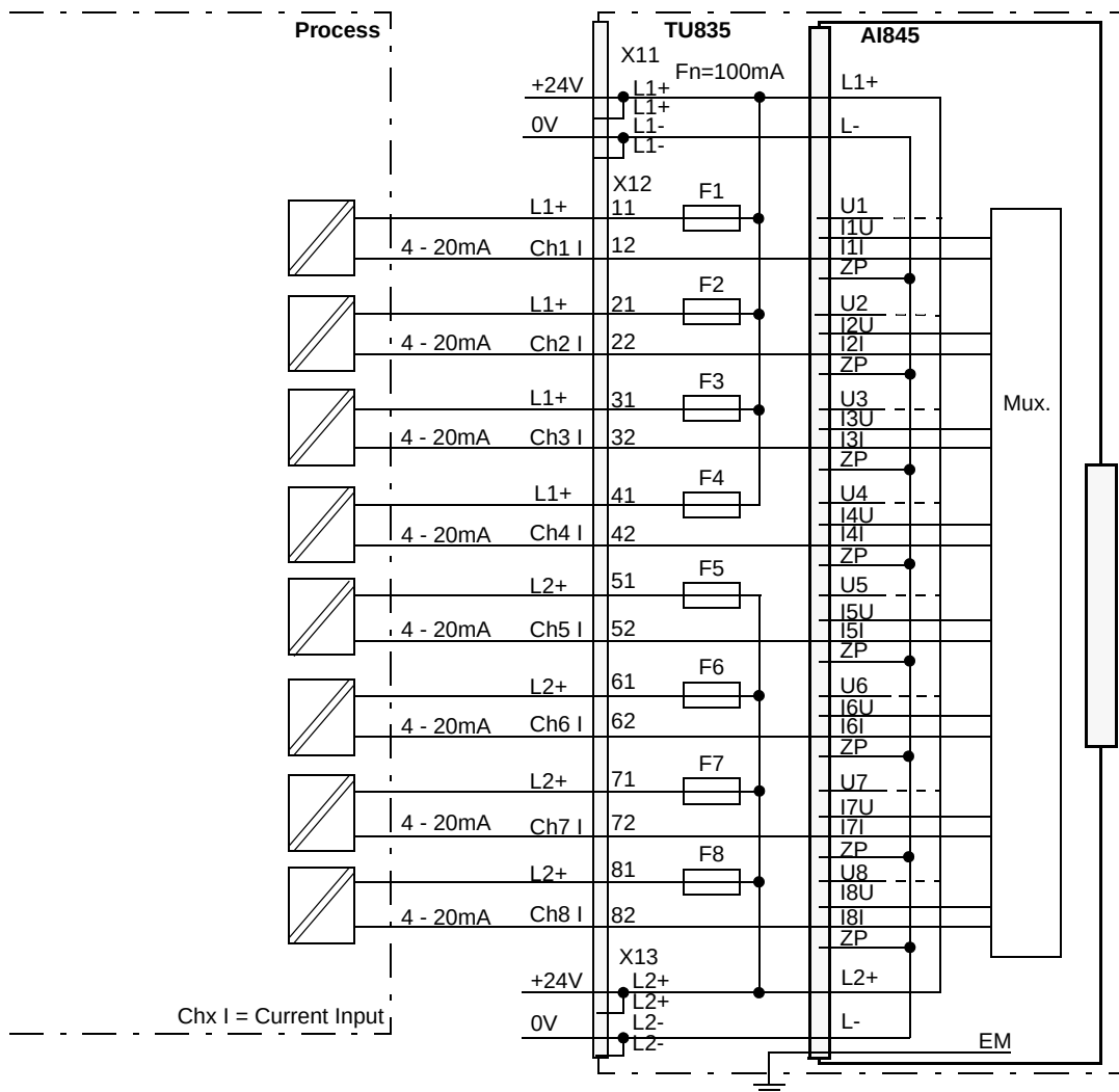
Figure 48. AI845 with TU835 Extended MTU Process Connections
