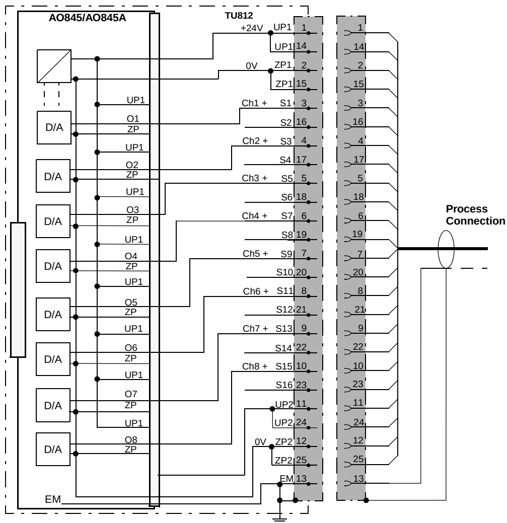
Figure 77. AO845/AO845A with TU812 Compact MTU Process Connections
