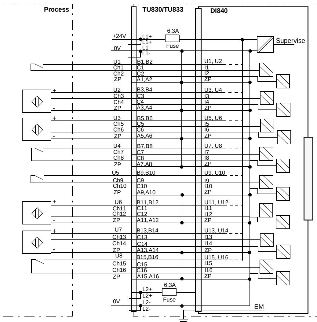
Figure 127. DI840 with TU830 Extended MTU Process Connections
