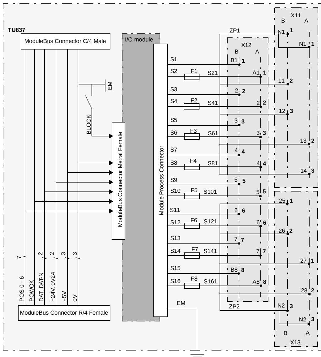
Figure 211. TU837/TU837V1 Block Diagram
