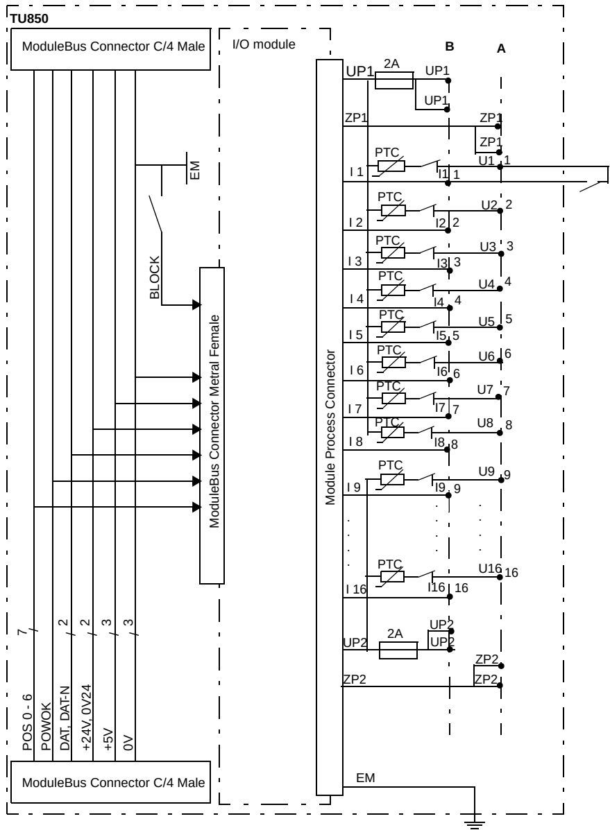
Block Diagram TU850
