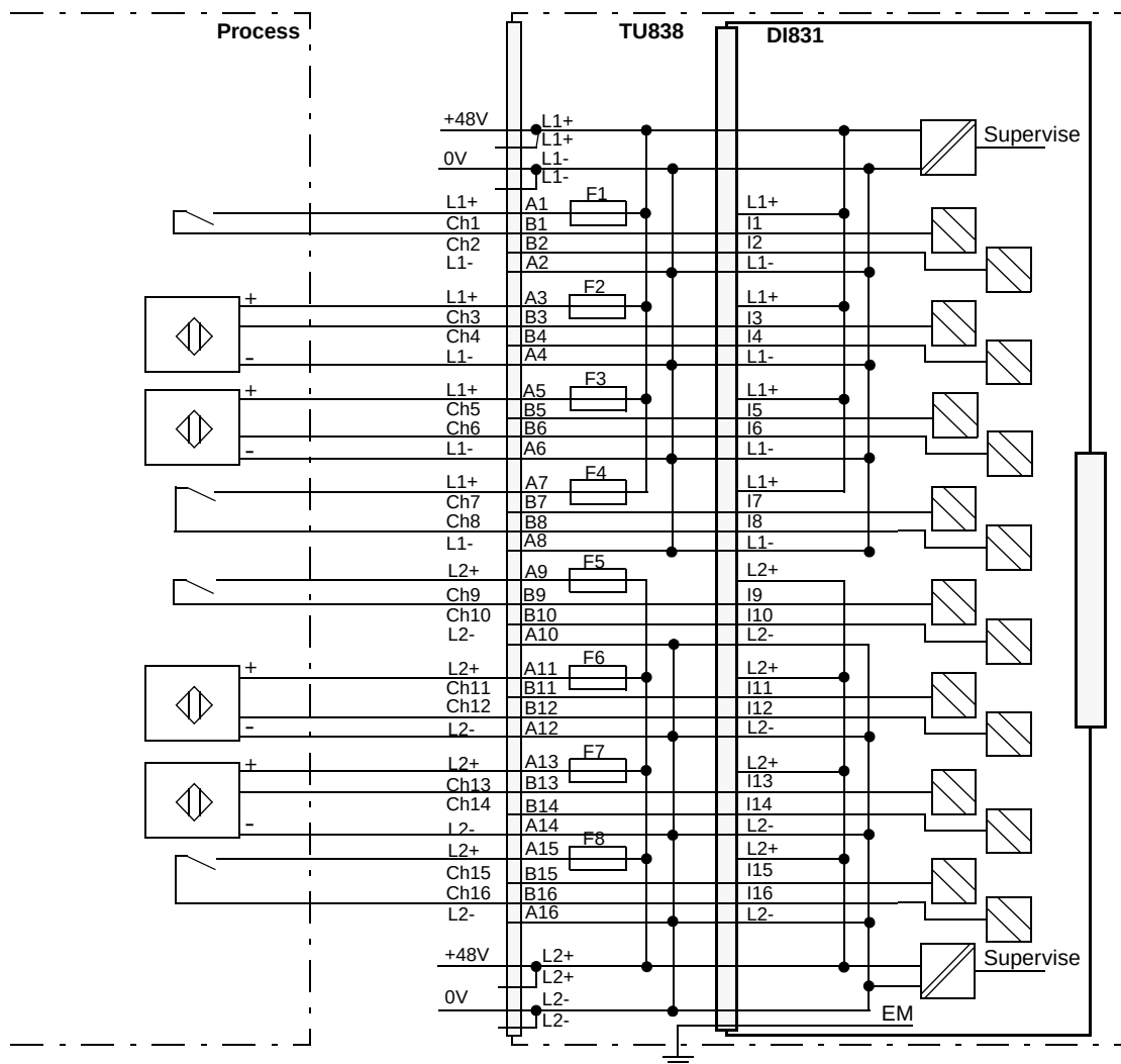
Figure 122. DI831 with TU838 Extended MTU Process Connections
