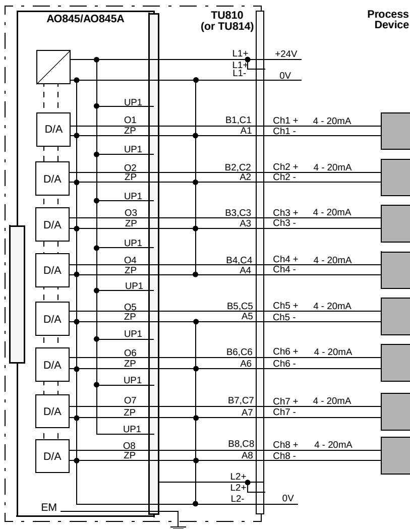
Figure 76. AO845/AO845A with TU810 or TU814 Compact MTU Process Connections
