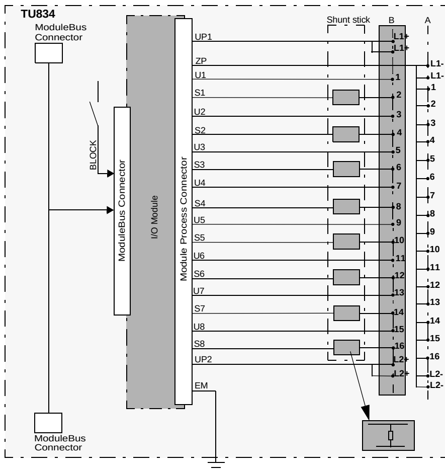
Figure 208. TU834 Block Diagram
