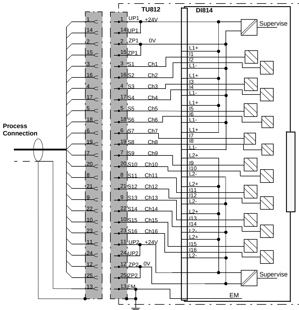
Figure 101. DI814 with TU812 Compact MTU Process Connections
