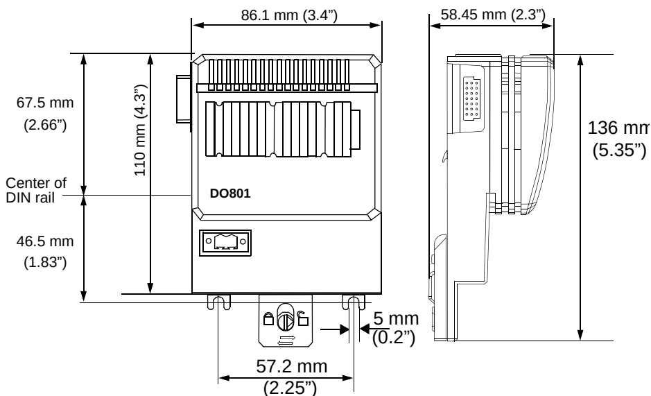
Figure 7. Dimensions for S800L Modules
