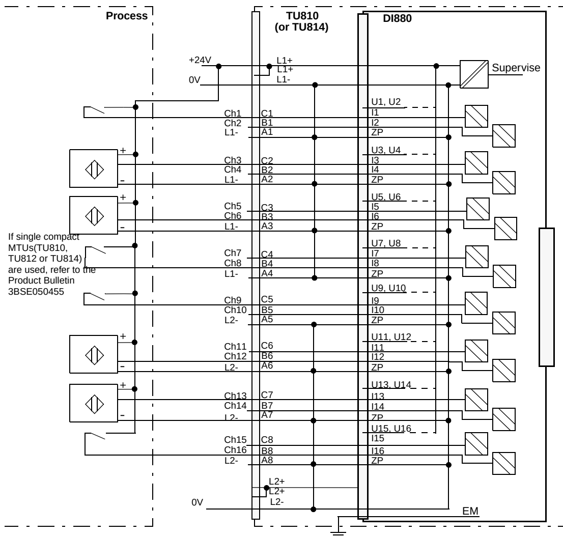
Figure 134. DI880 with TU810 or TU814 Compact MTU Process Connections
