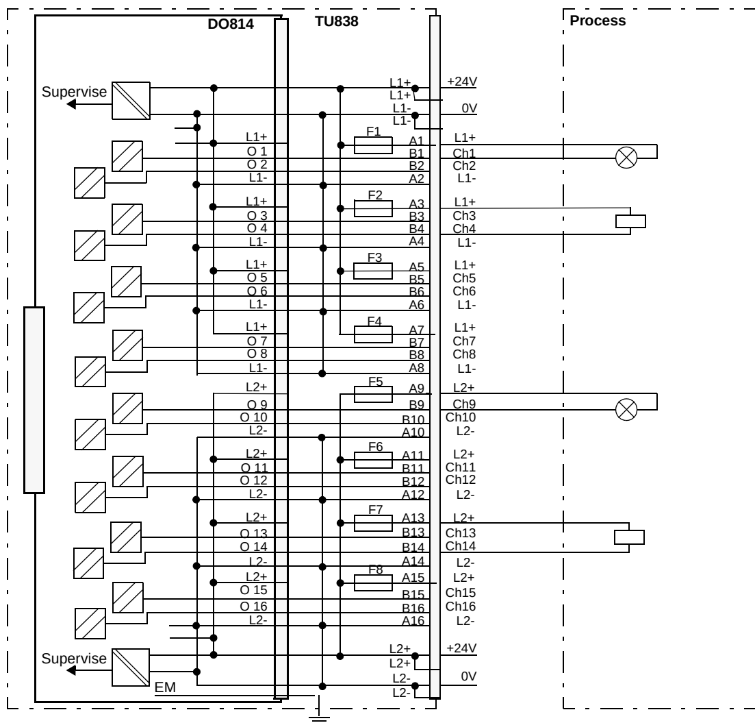
Figure 151. DO814 with TU838 Extended MTU Process Connections
