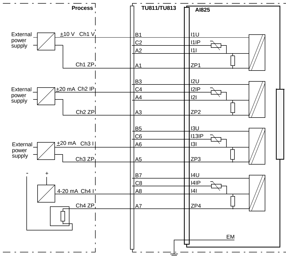
Figure 30. AI825 with TU811/TU811V1 or TU813 Compact MTU Process Connections
