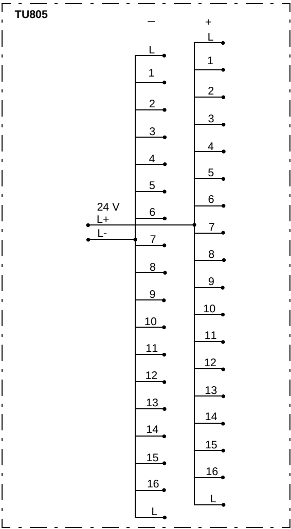
Figure 197. TU805 Block Diagram
