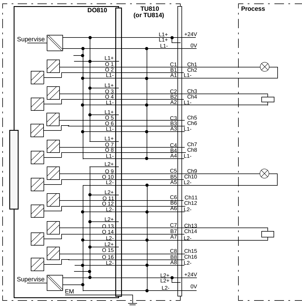
Figure 147. DO810 with TU810 or TU814 Compact MTU Process Connections
