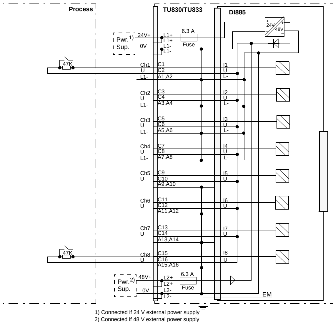
Figure 138. DI885 with TU830 Extended MTU Process Connections
