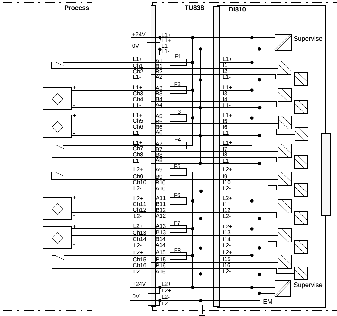
Figure 87. DI810 with TU838 Extended MTU Process Connections
