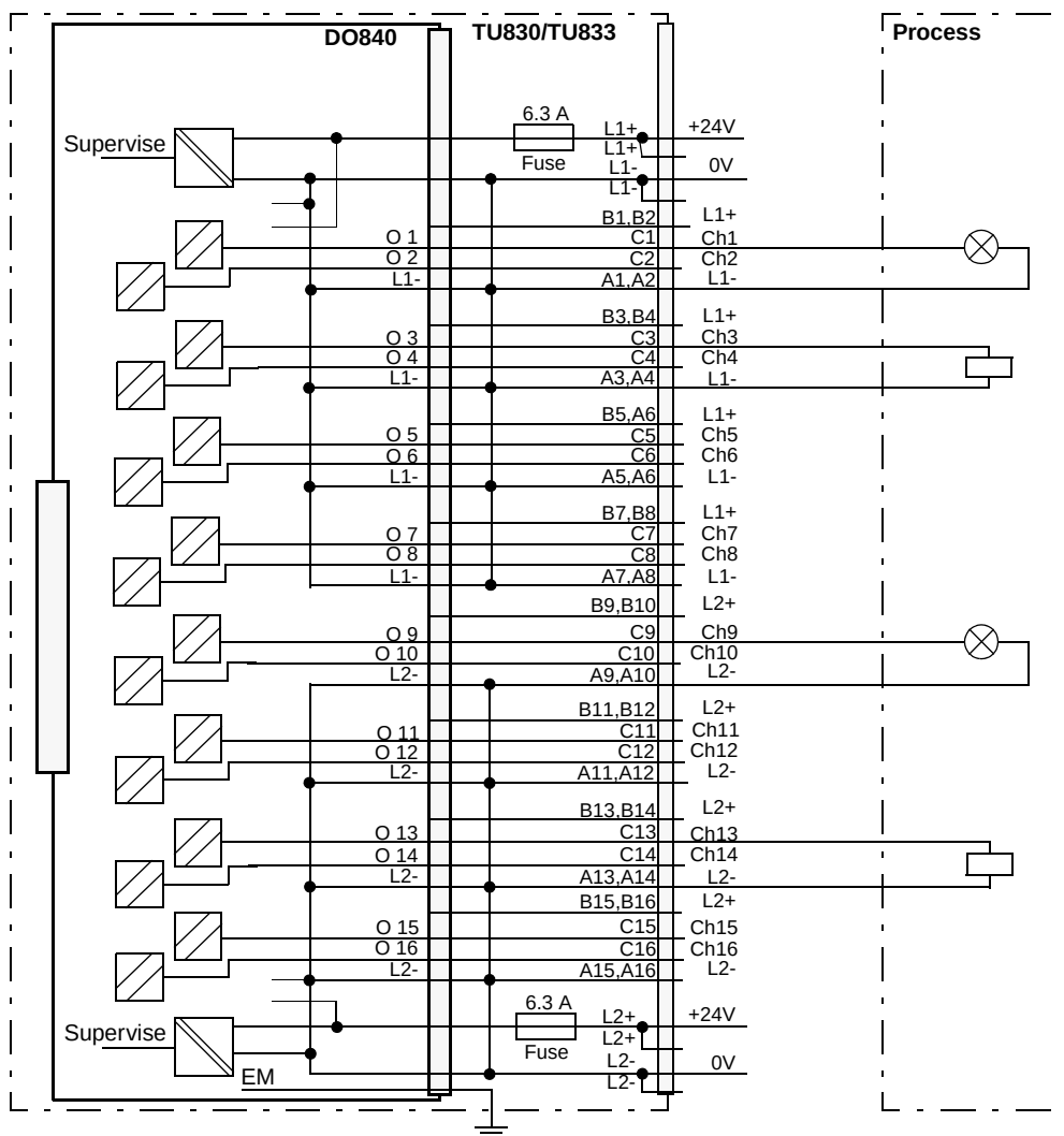
Figure 169. DO840 with TU830/TU833 Extended MTU Process Connections
