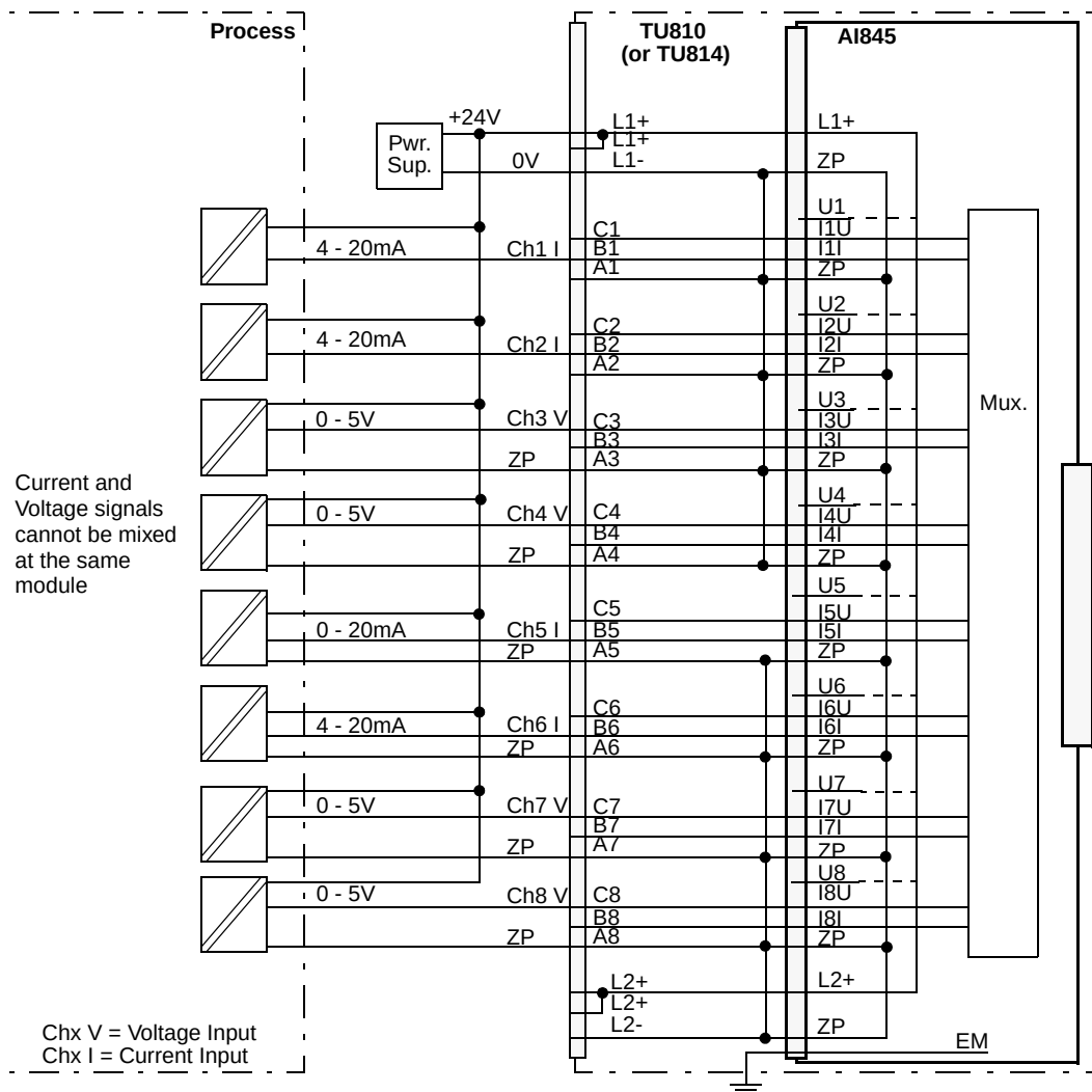
Figure 50. AI845 with TU810 or TU814 Compact MTU Process Connections
