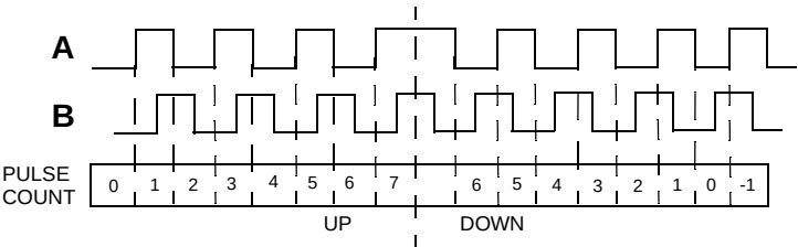
Figure 182. Quadrature Mode, #2 (Count on Pos. Edge and Neg. Edge Input A)
