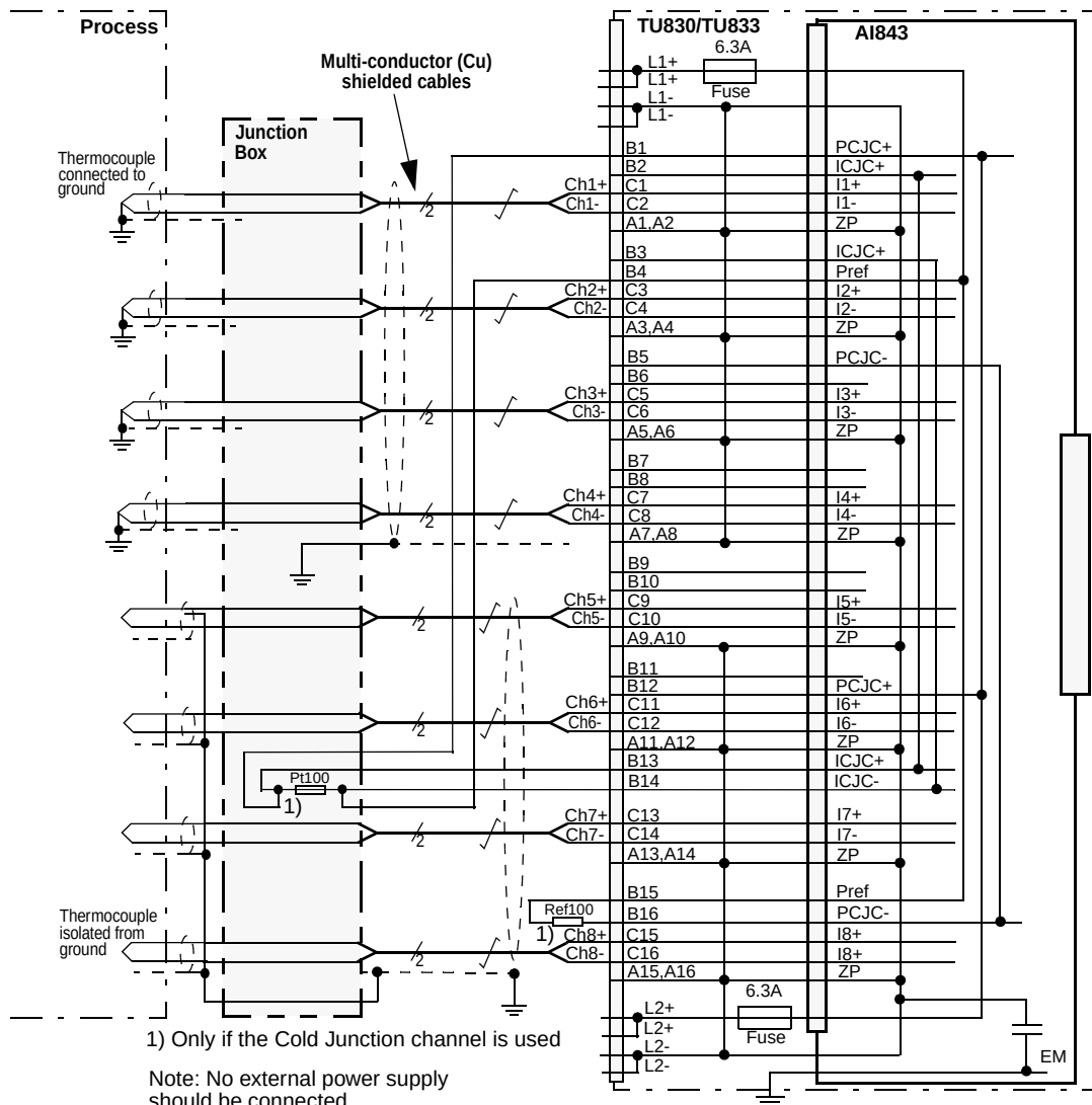
Figure 44. AI843 with TU830 Extended MTU Process Connections to Remote Junction Box
