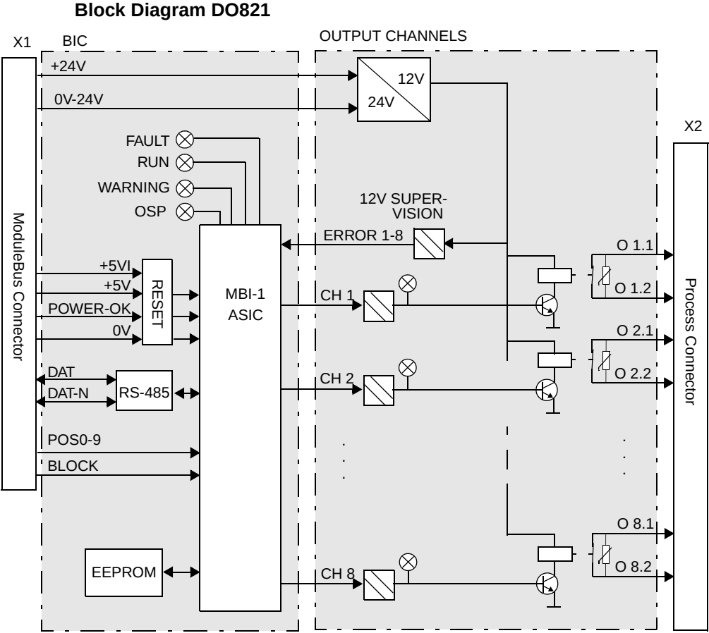
Figure 163. DO821 Block Diagram
