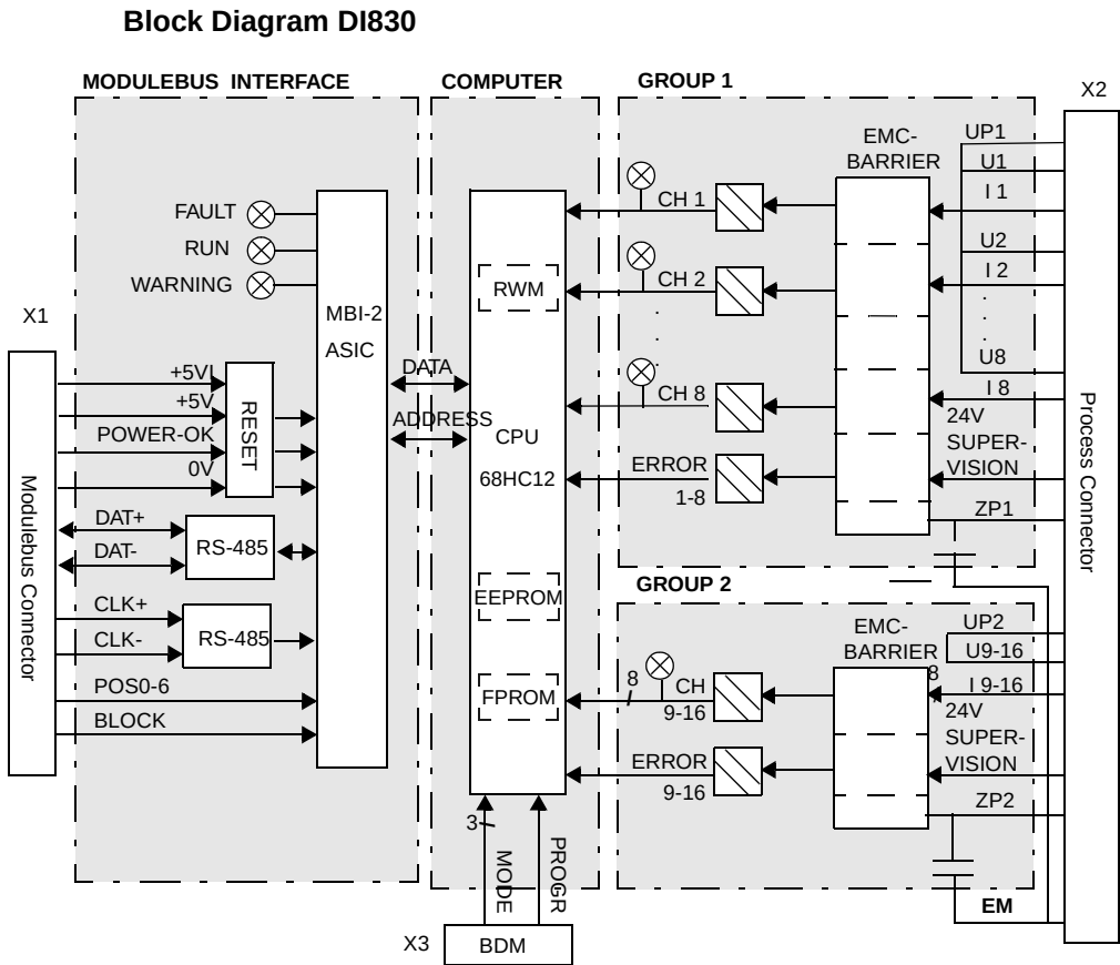
Figure 114. DI830 Block Diagram
