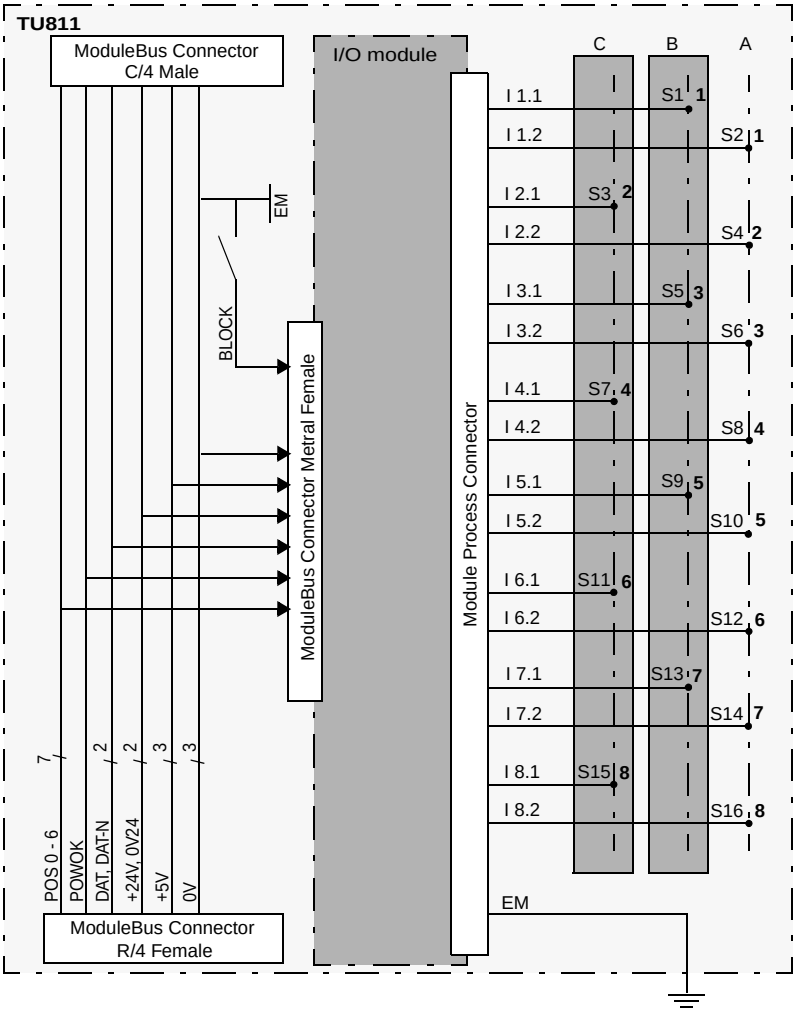
Figure 199. TU811/TU811V1 Block Diagram
