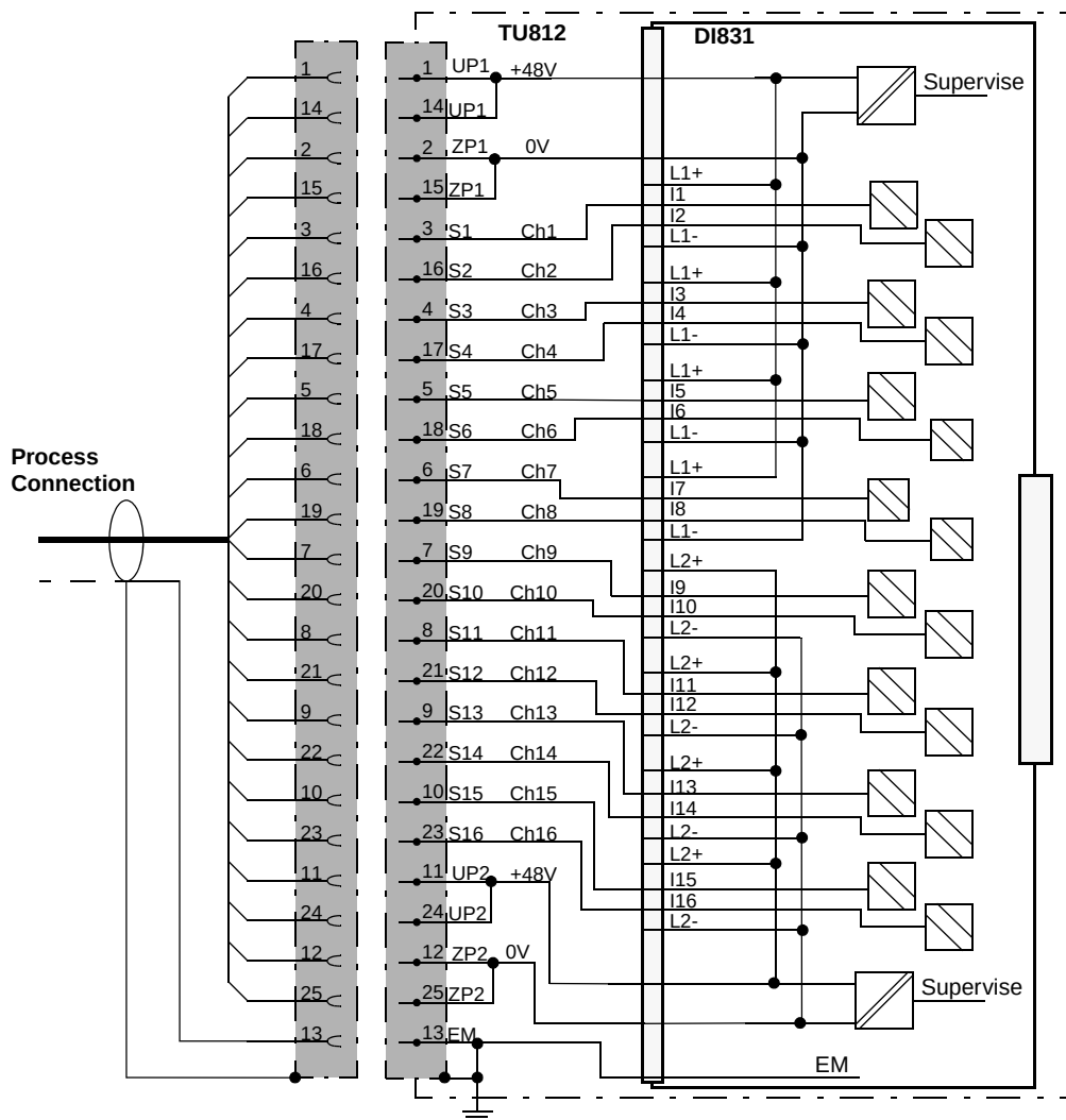
Figure 124. DI831 with TU812 Compact MTU Process Connections
