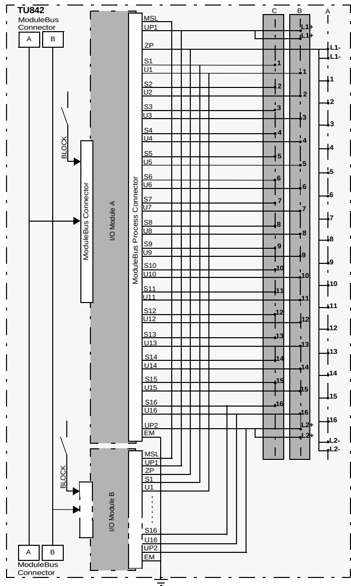
Figure 214. Block Diagram TU842
