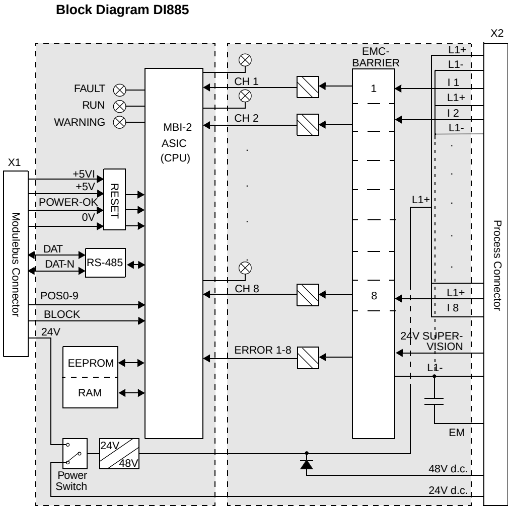
Figure 137. DI885 Block Diagram
