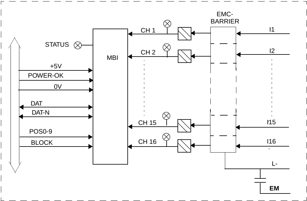
Figure 79. DI801 Block Diagram
