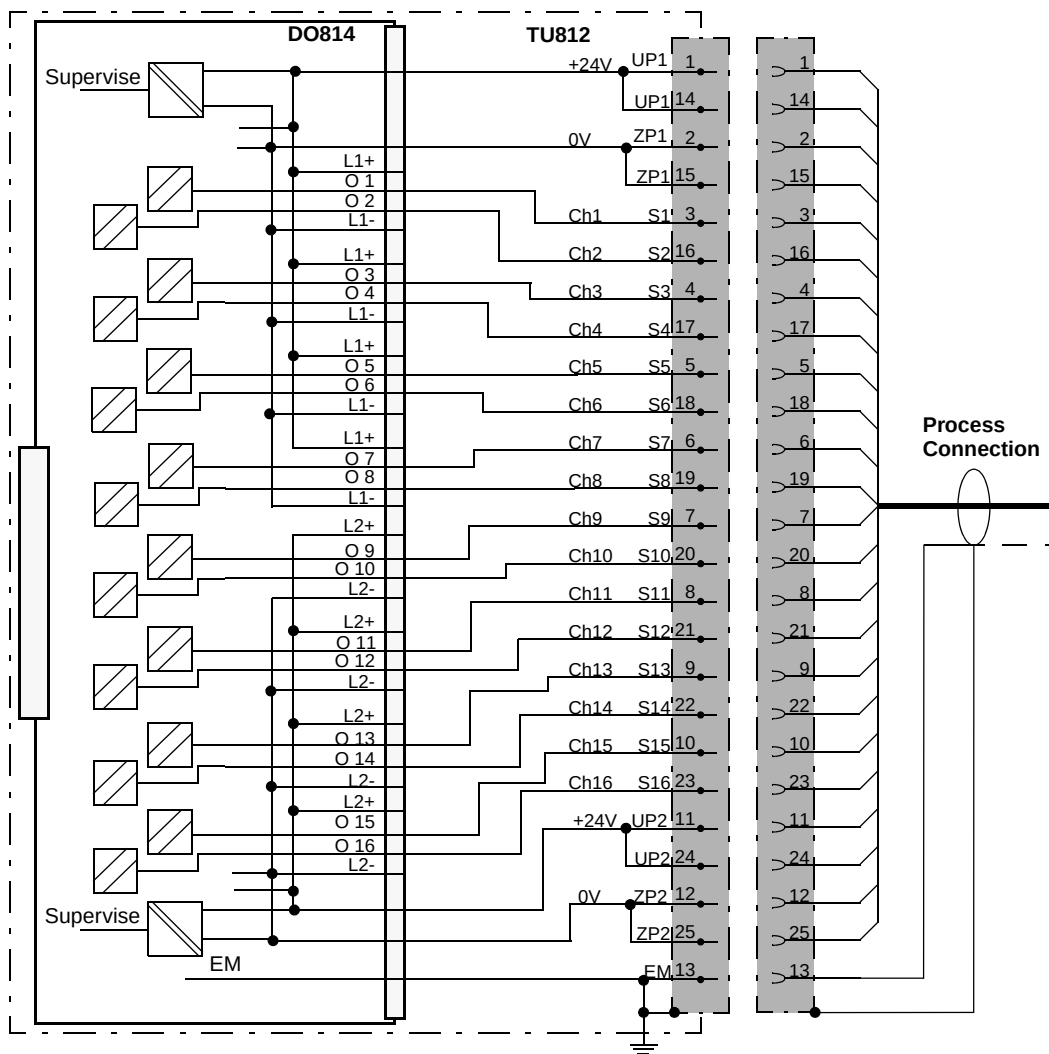
Figure 153. DO814 with TU812 Compact MTU Process Connections
