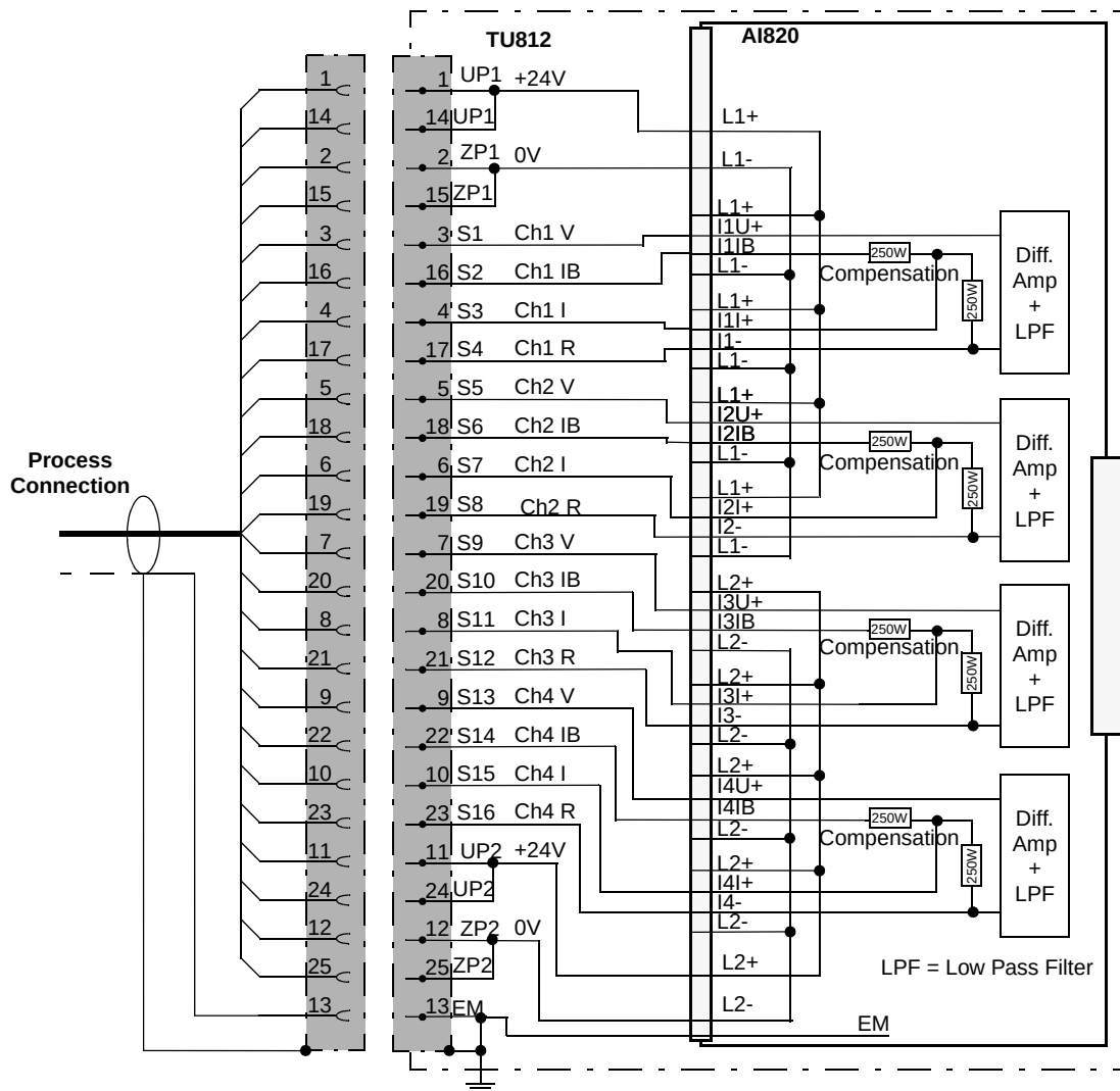
Figure 28. AI820 with TU812 Compact MTU Process Connections
