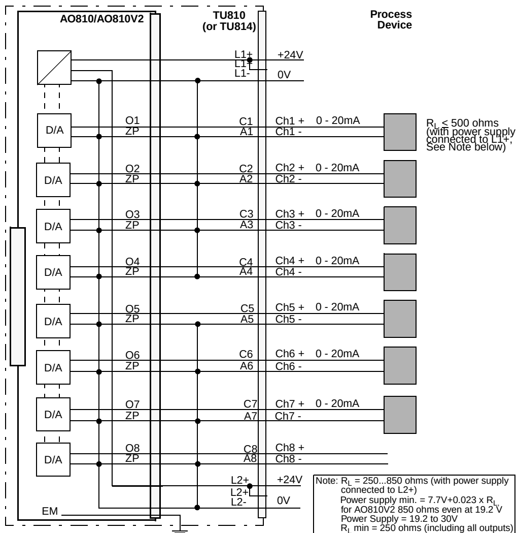
Figure 64. AO810/AO810V2 with TU810 or TU814 Compact MTU Process Connections
