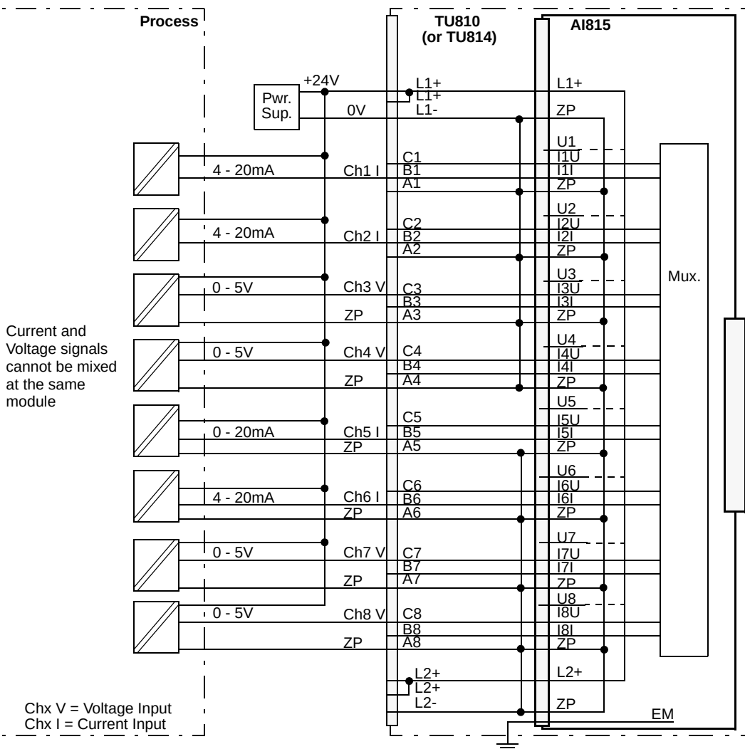
Figure 23. AI815 with TU810 or TU814 Compact MTU Process Connections
