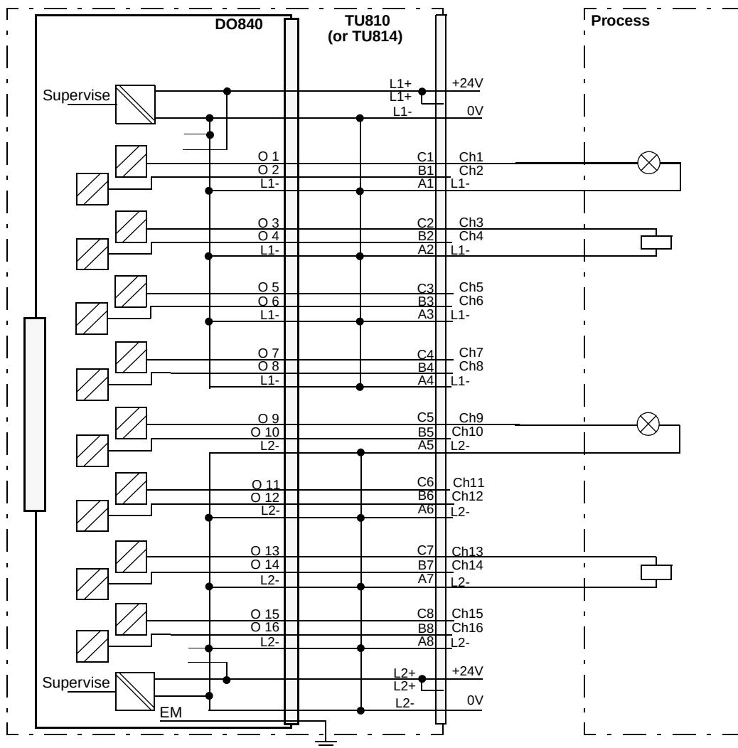
Figure 170. DO840 with TU810 or TU814 Compact MTU Process Connections
