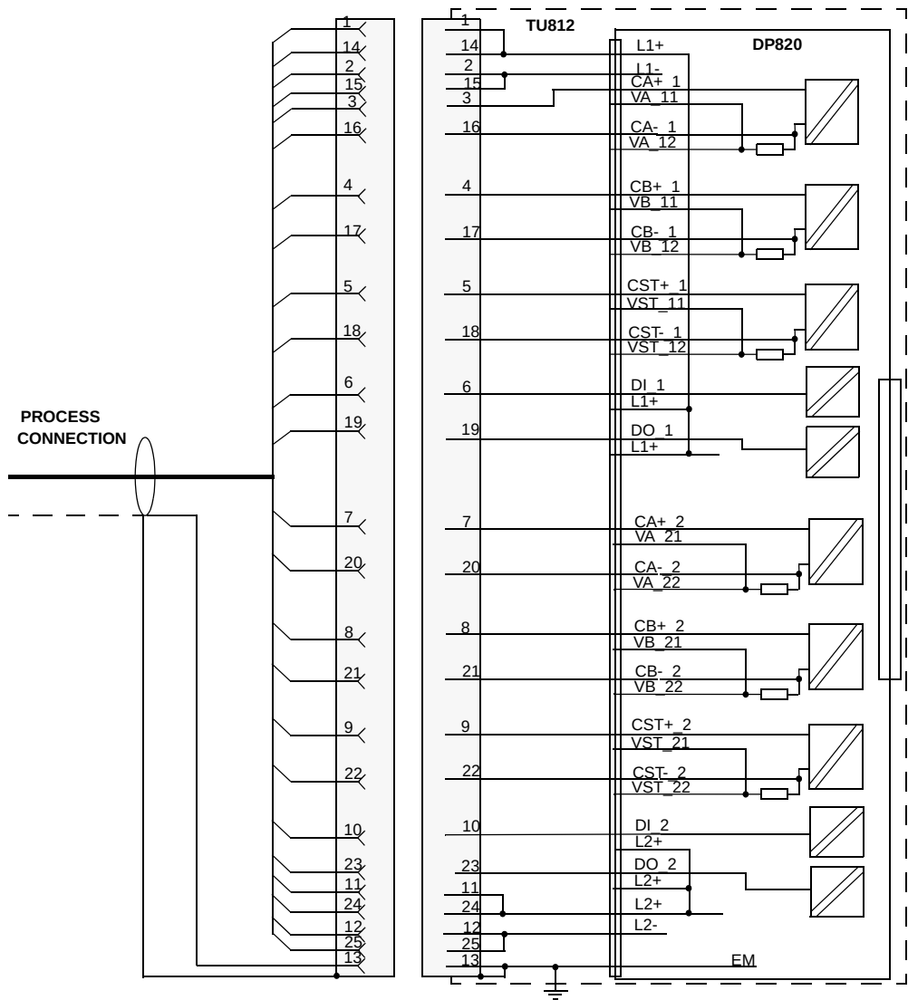
Figure 188. DP820 with TU812 MTU Process Connections
