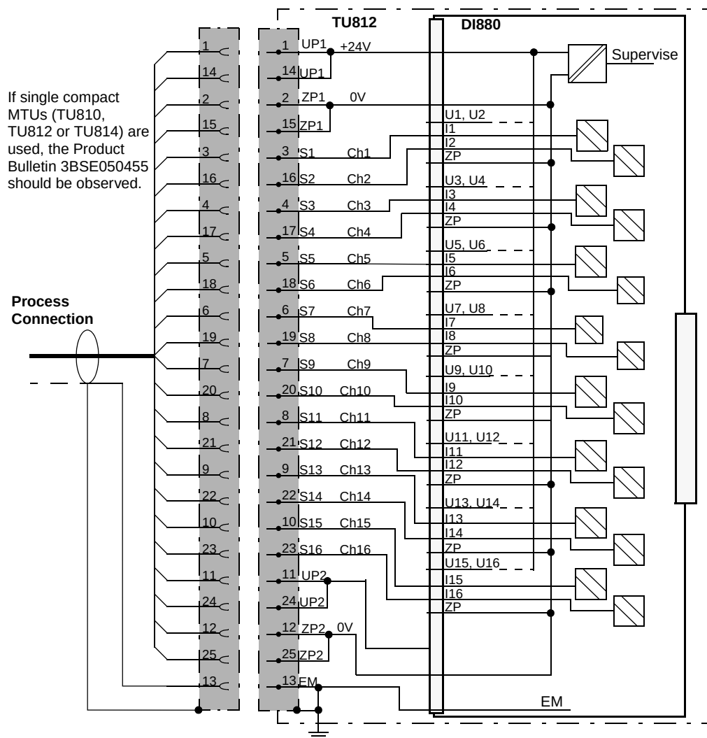
Figure 135. DI880 with TU812 Compact MTU Process Connections
