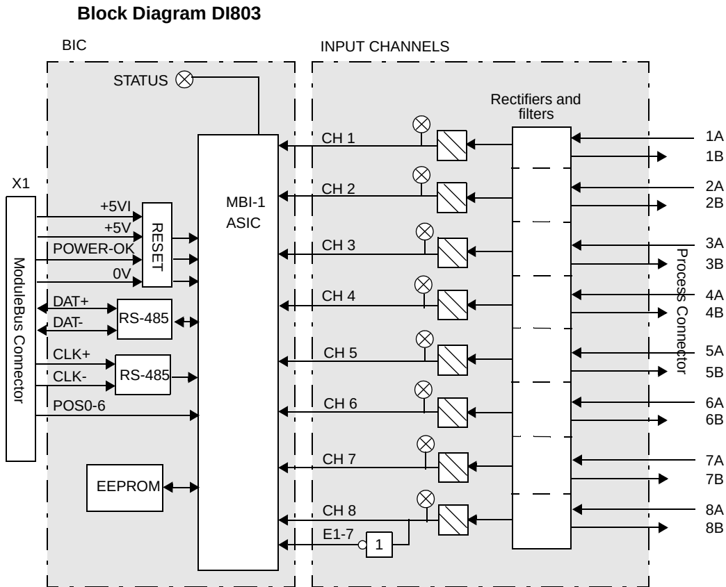
Figure 83. DI803 Block Diagram
