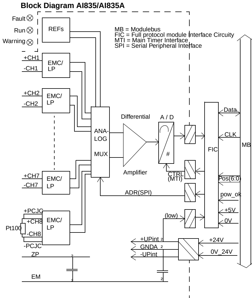
Figure 37. AI835/AI835A Block Diagram
