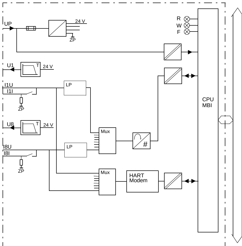
Figure 19. AI815 Block Diagram
