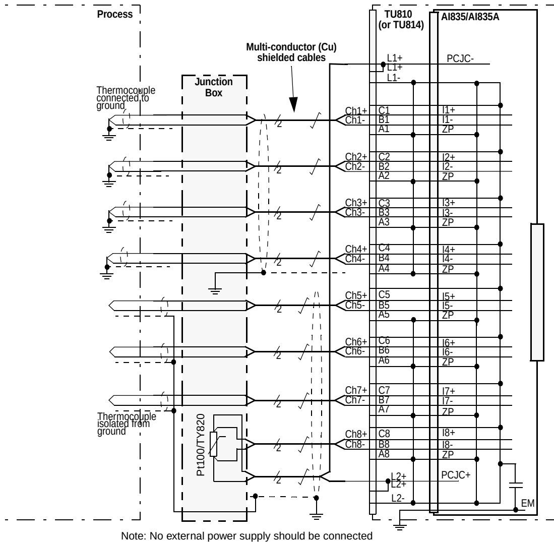
Figure 40. AI835/AI835A with TU810 or TU814 Compact MTU Process Connections to Remote Junction Box
