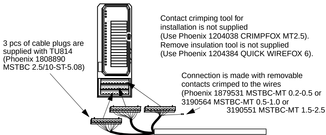
Figure 203. Connections to TU814/TU814V1
