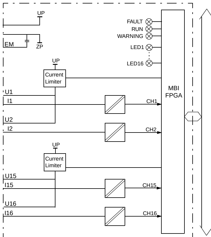
Figure 126. Block Diagram DI840
