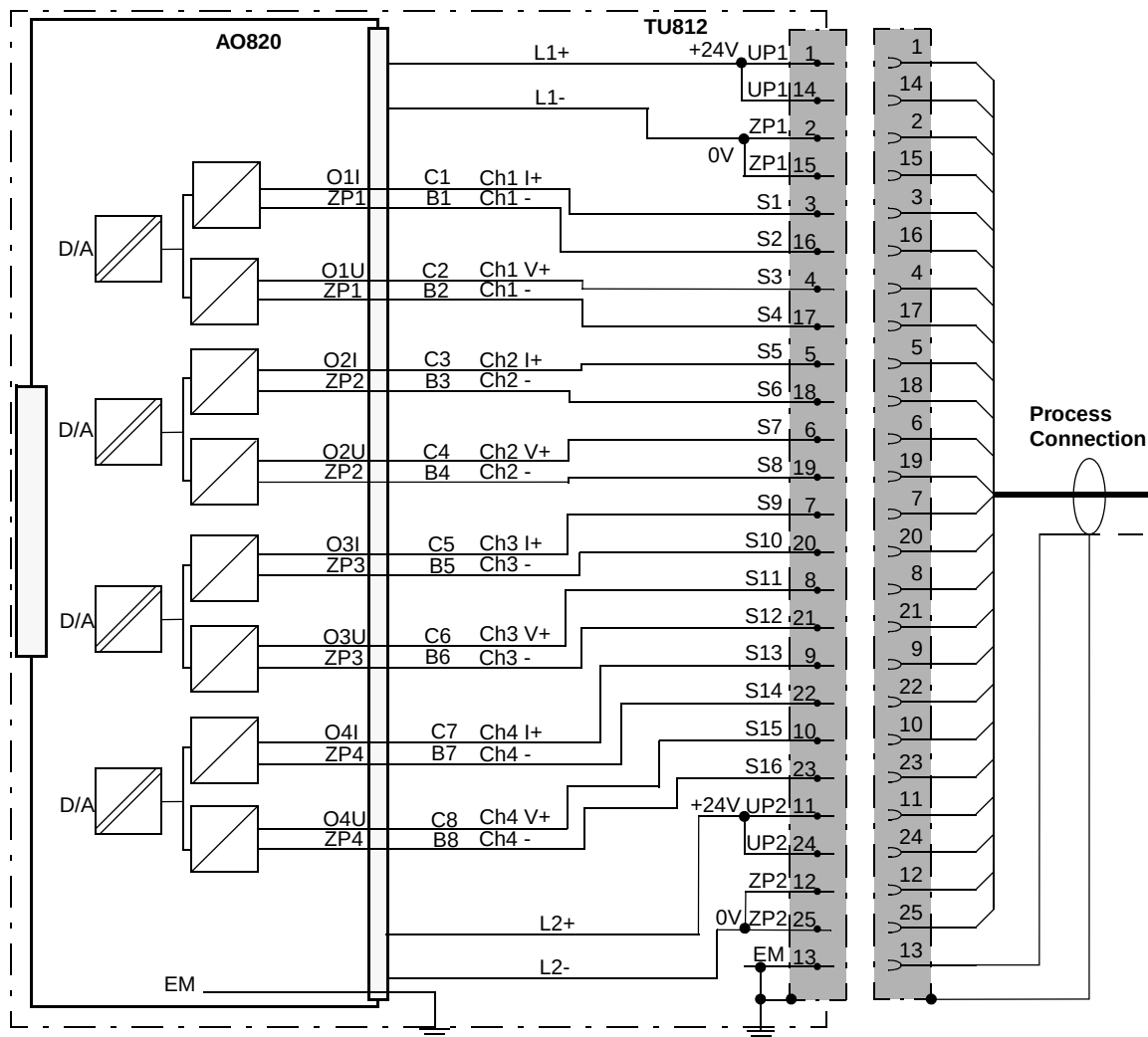
Figure 73. AO820 with TU812 Compact MTU
