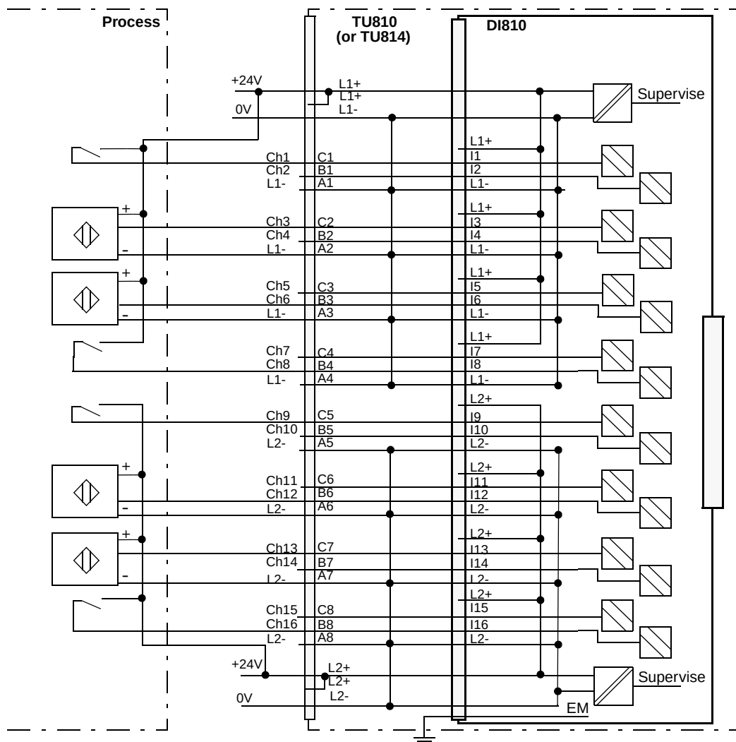
Figure 88. DI810 with TU810 or TU814 Compact MTU Process Connections
