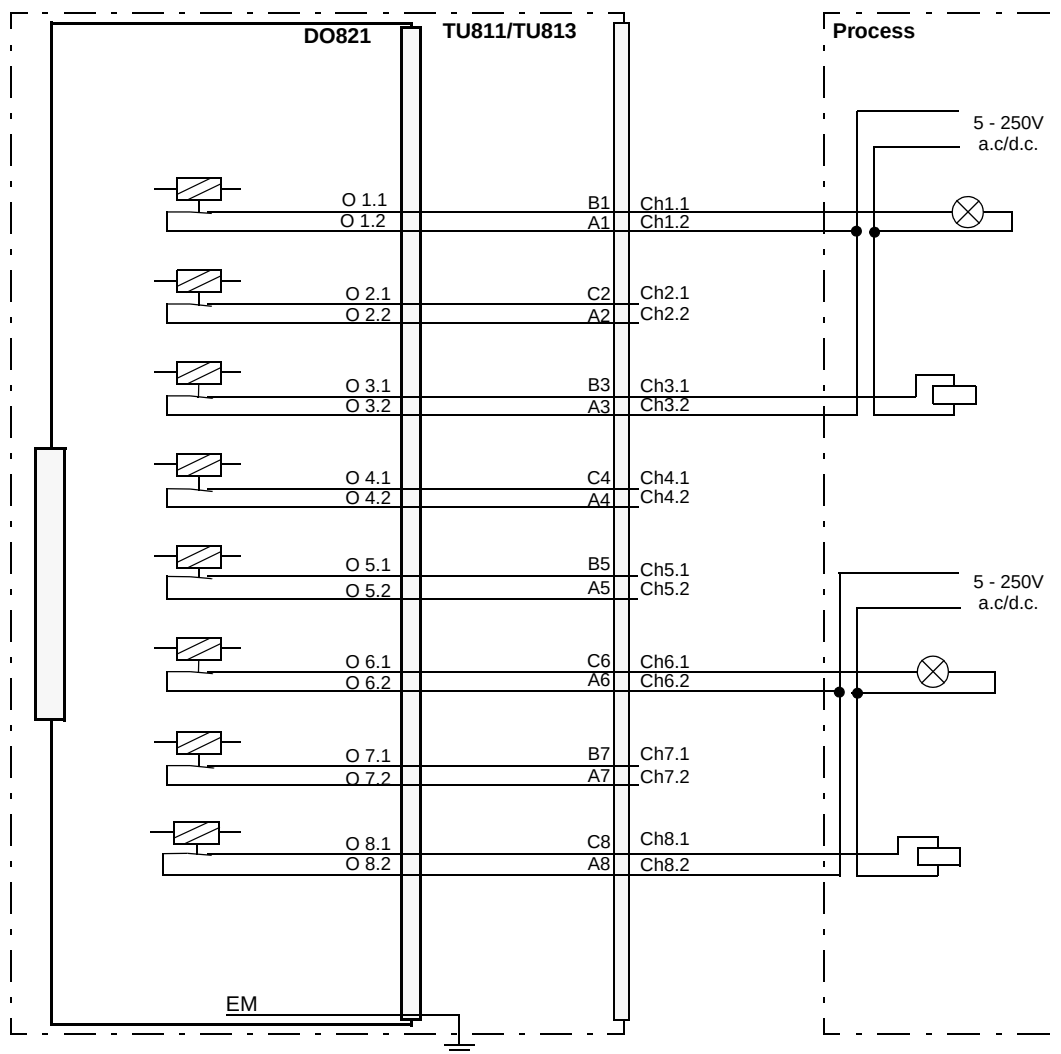
Figure 165. DO821 with TU811 or TU813 Compact MTU Process Connections
