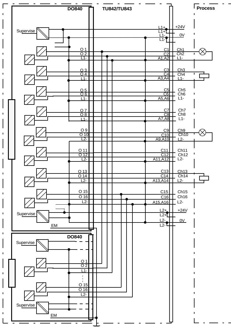
Figure 172. DO840 with TU842 or TU843 Redundant MTU Process Connections
