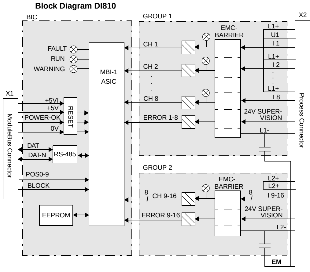
Figure 85. DI810 Block Diagram
