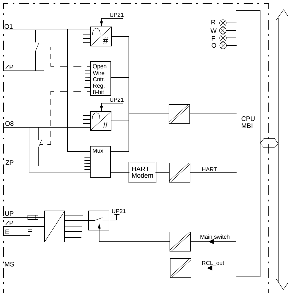
Figure 74. AO845/AO845A Block Diagram
