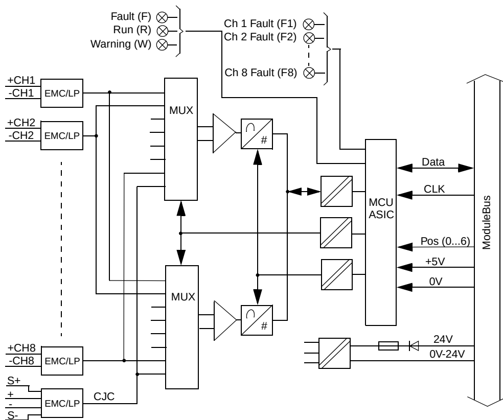
Figure 42. AI843 Block Diagram
