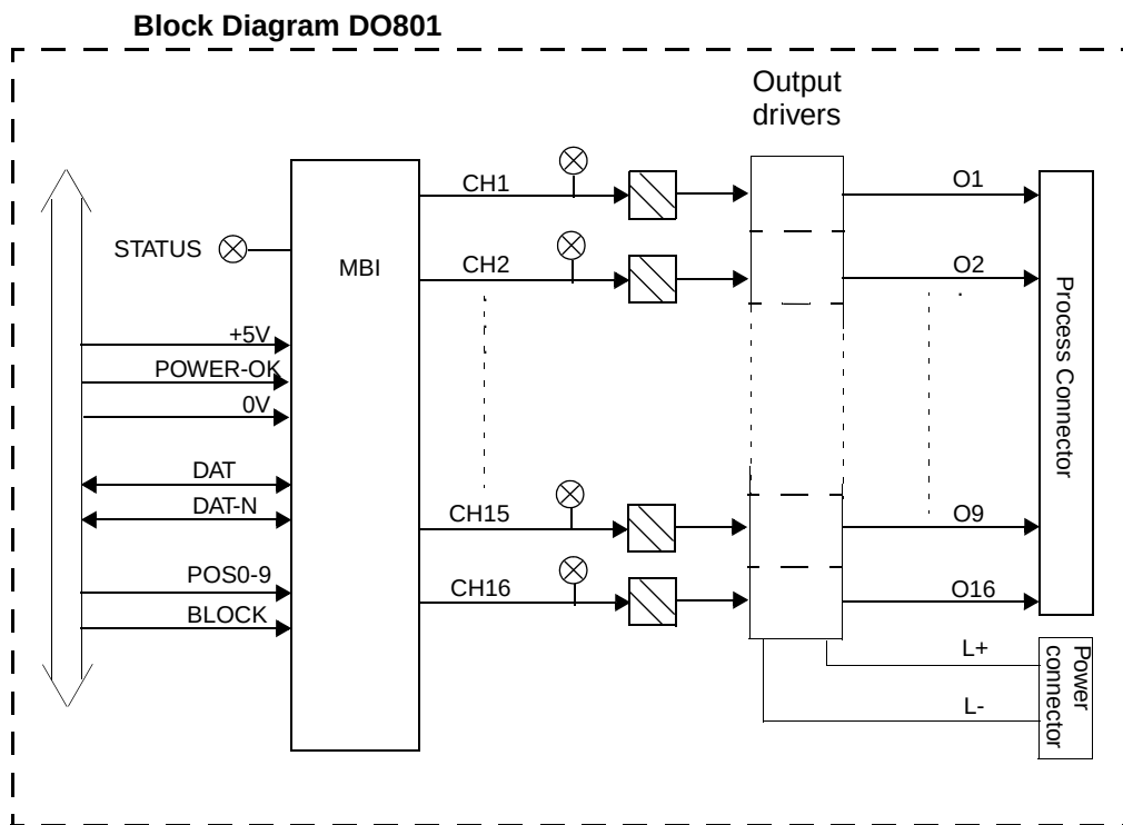
Figure 141. DO801 Block Diagram
