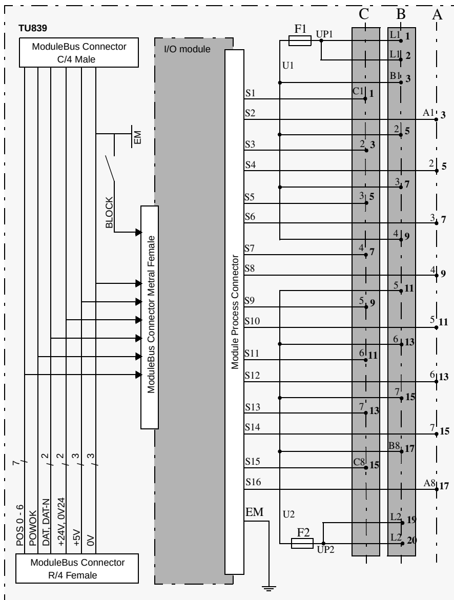
Figure 213. Block Diagram of TU839
