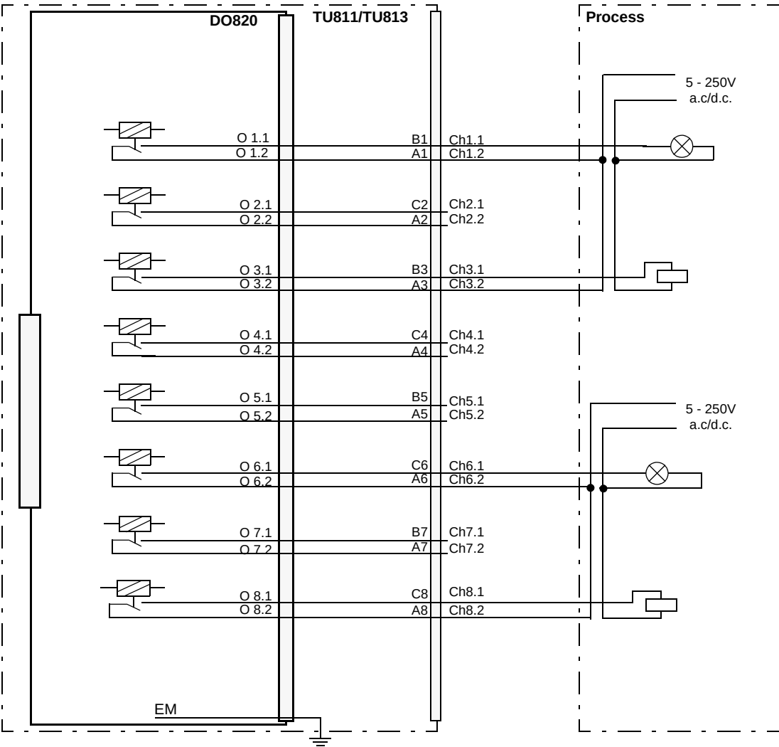
Figure 160. DO820 with TU811 or TU813 Compact MTU Process Connections
