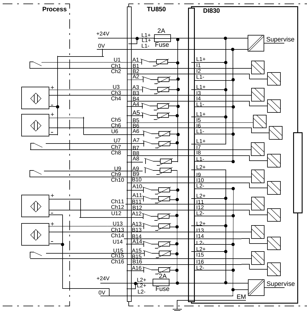
Figure 119. DI830 with TU850 Extended MTU Process Connection.
