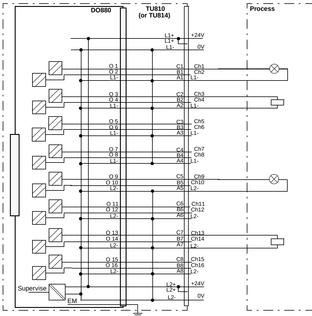
Figure 176. DO880 with TU810 or TU814 Compact MTU Process Connections
