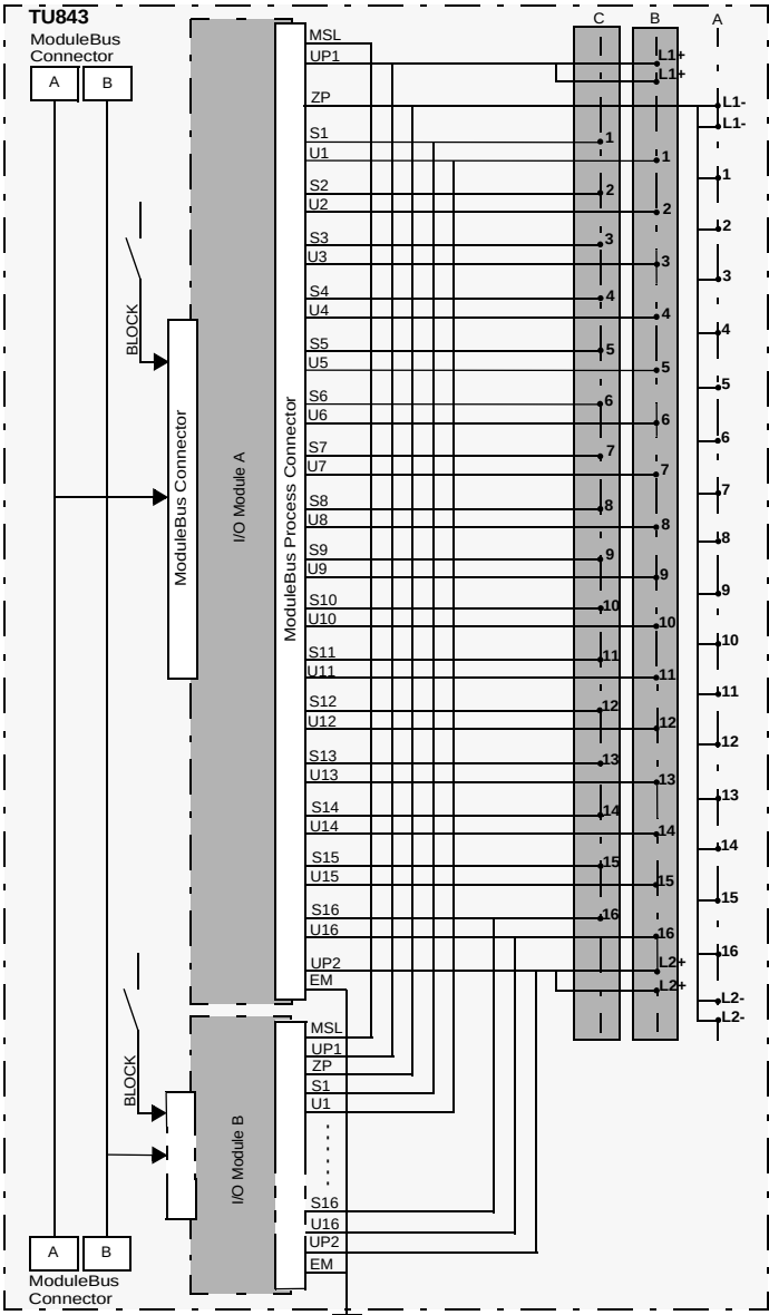
Block Diagram TU843
