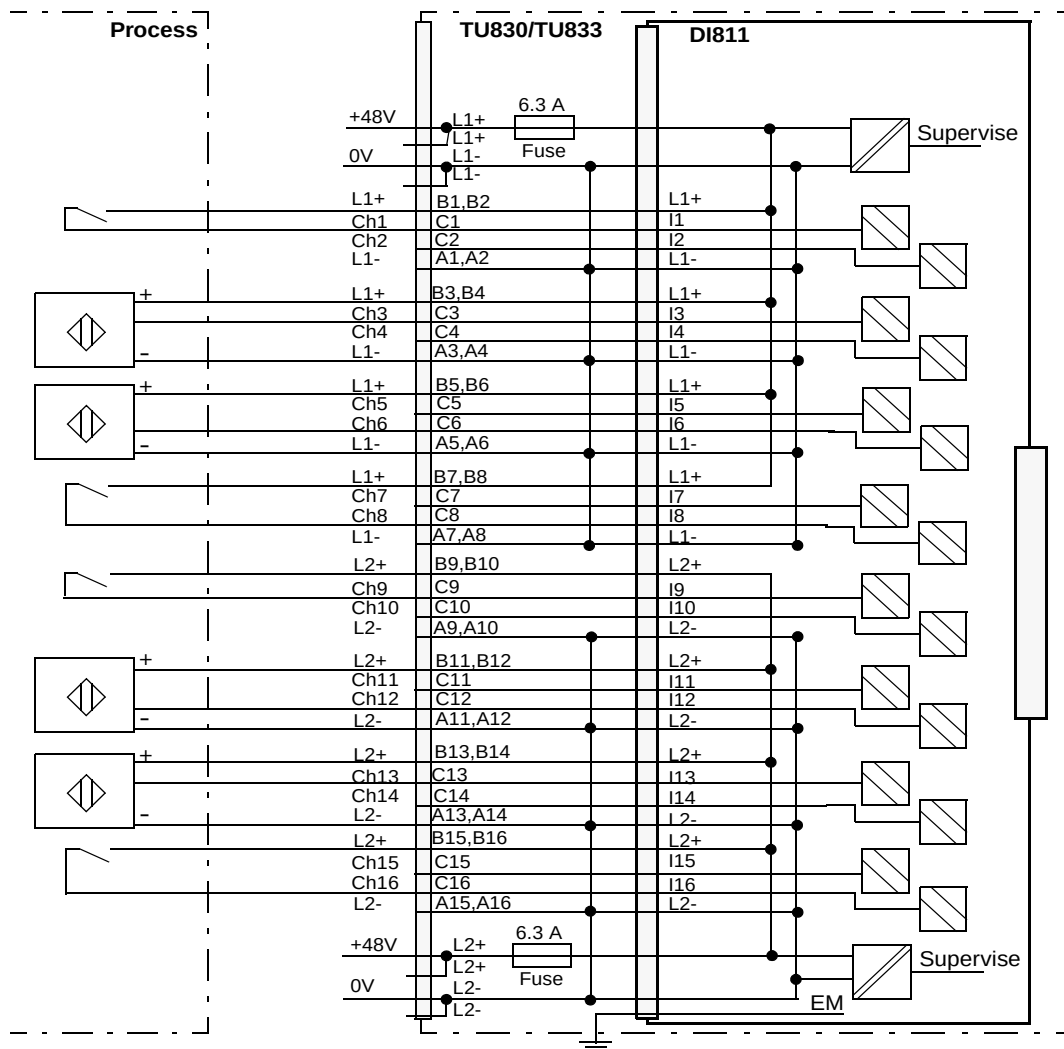
Figure 92. DI811 with TU830 Extended MTU Process Connections
