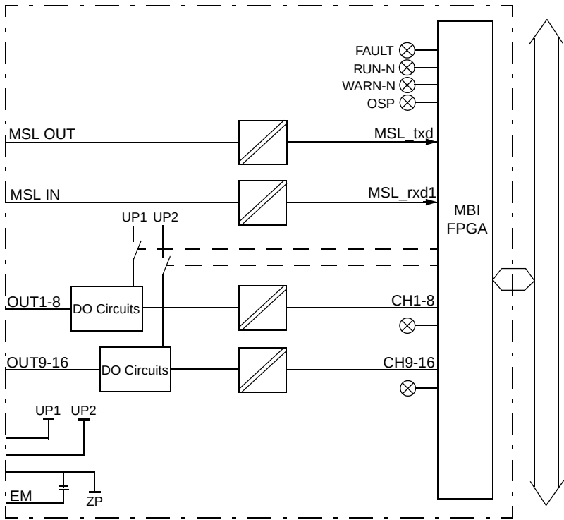
Figure 168. Block Diagram D0840
