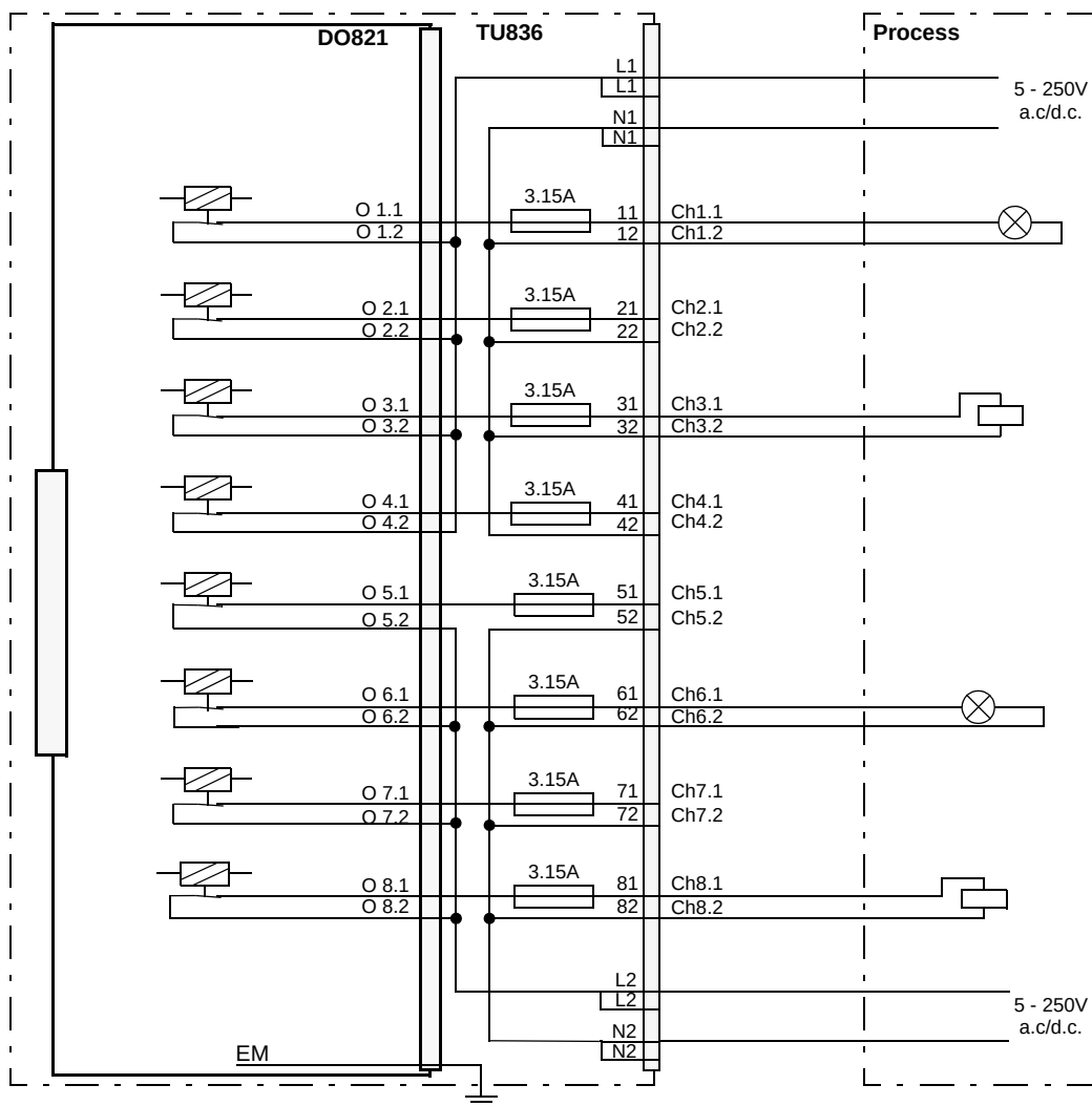
Figure 166. DO821 with TU836 Extended MTU Process Connections
