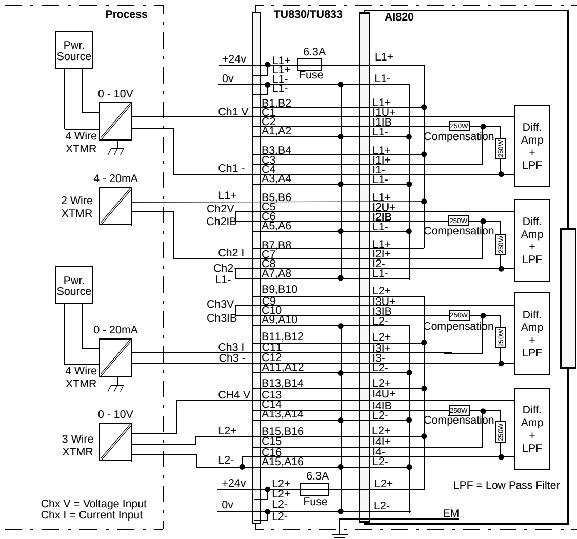
Figure 26. AI820 with TU830 Extended MTU Process Connections
