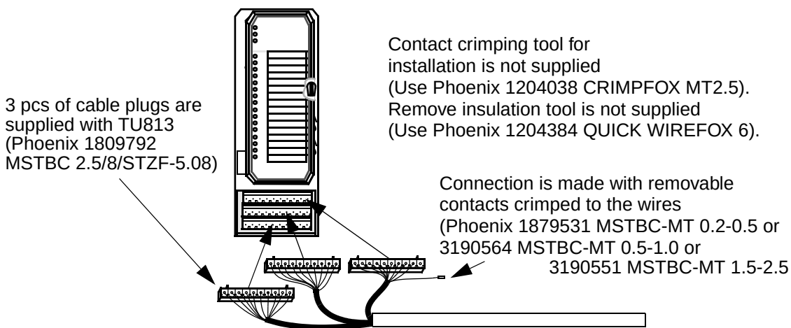
Figure 201. Connections to TU813
