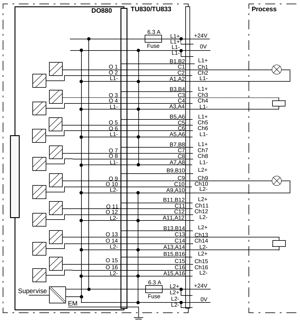
Figure 175. DO880 with TU830/TU833 Extended MTU Process Connections
