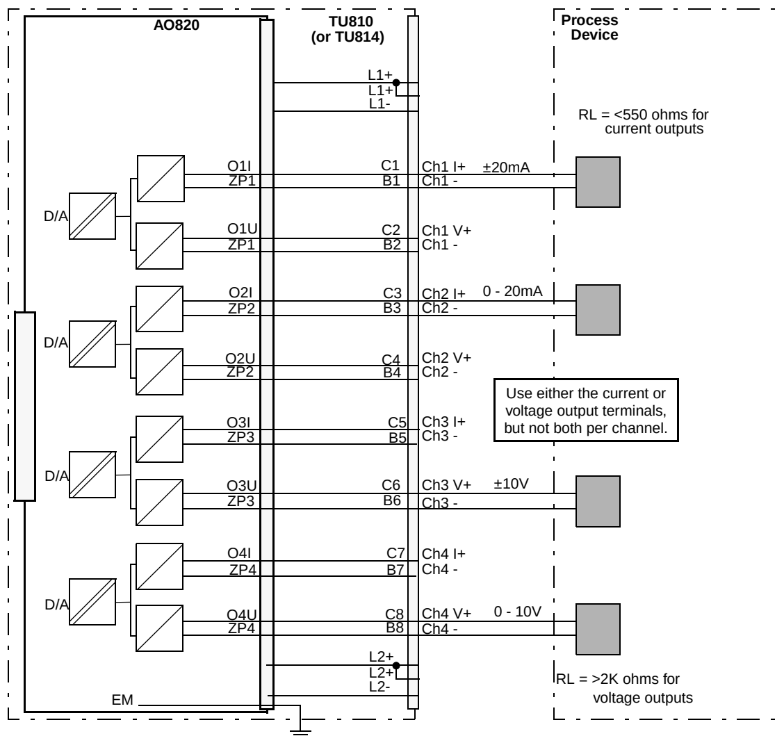
Figure 72. AO820 with TU810 or TU814 Compact MTU Process Connections
