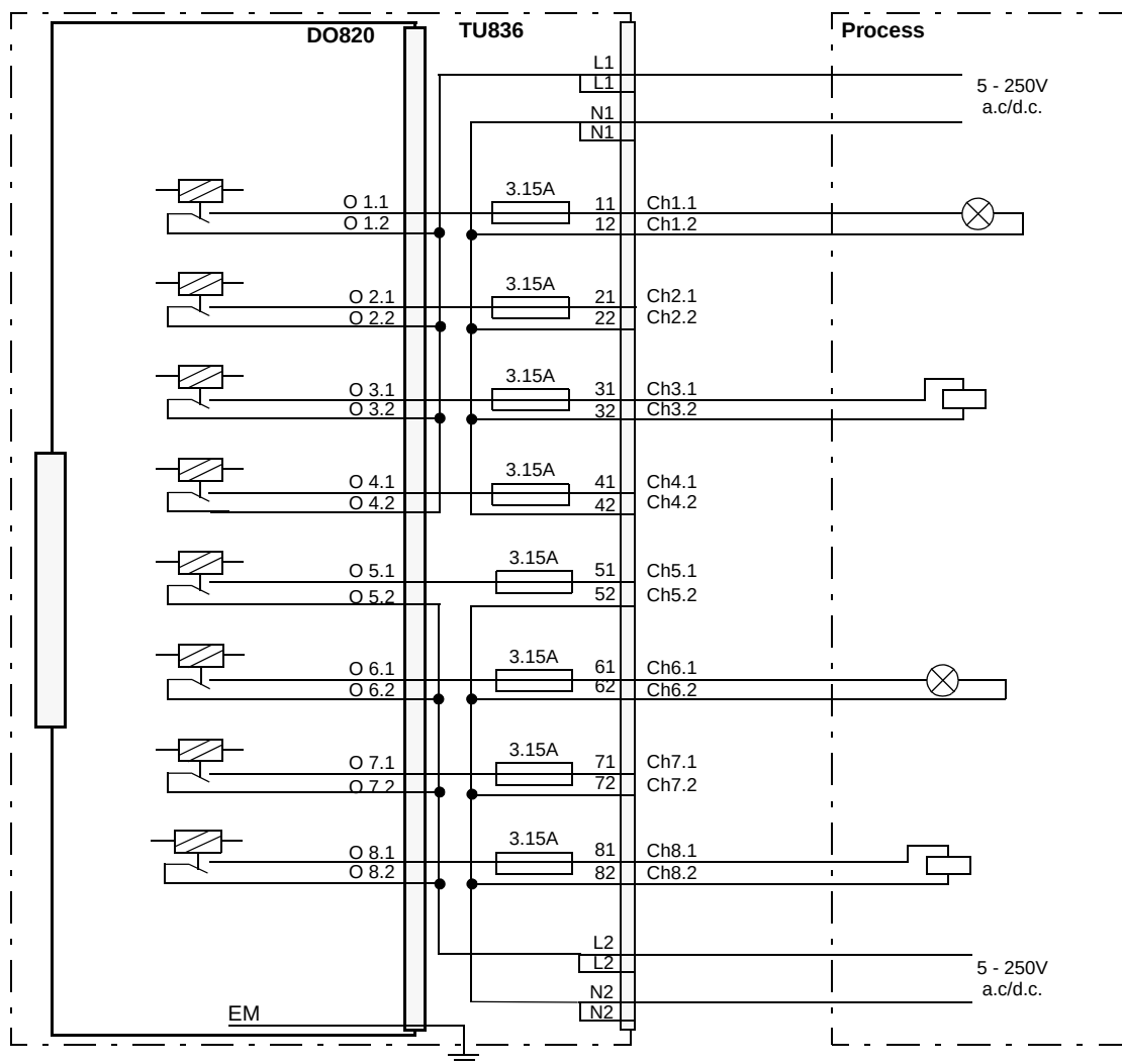
Figure 161. DO820 with TU836 Extended MTU Process Connections
