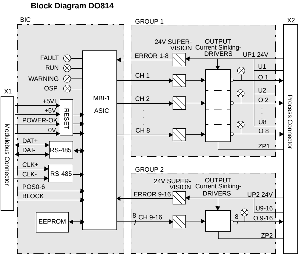
Figure 149. DO814 Block Diagram
