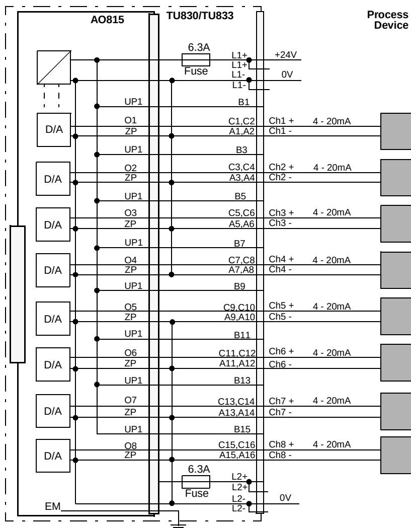
Figure 67. AO815 with TU830/TU833 Extended MTU Process Connections
