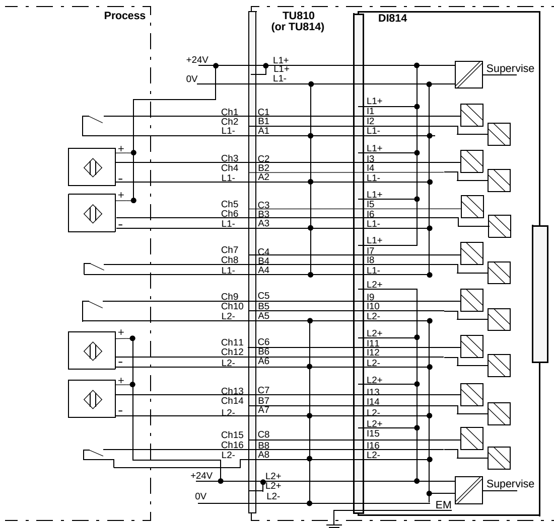
Figure 100. DI814 with TU810 or TU814 Compact MTU Process Connections
