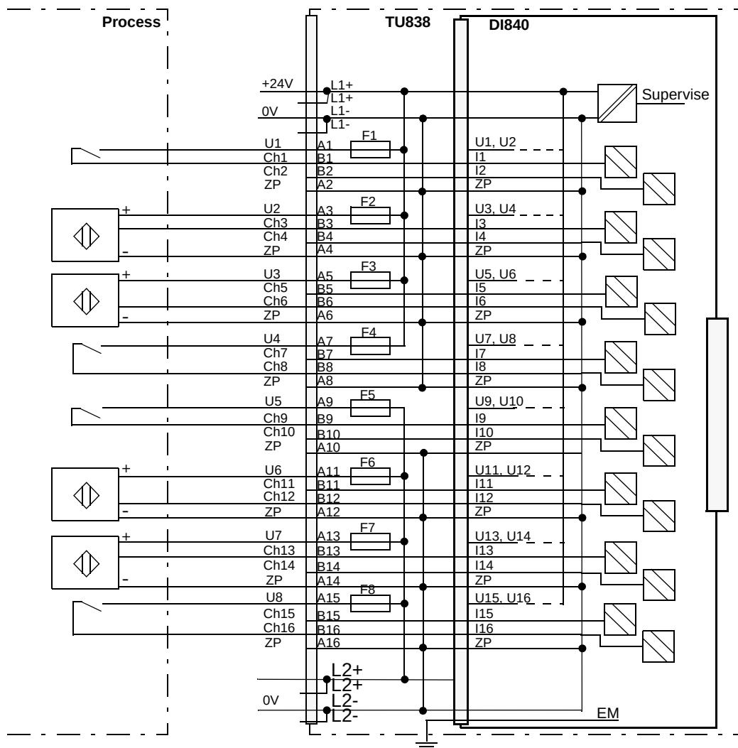
Figure 128. DI840 with TU838 Extended MTU Process Connections
