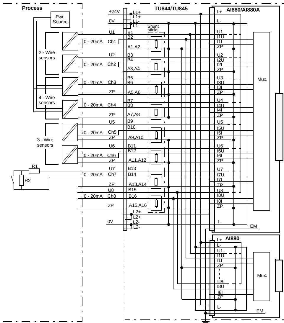
Figure 57. AI880/AI880A with TU844 or TU845 Redundant MTU Process Connections
