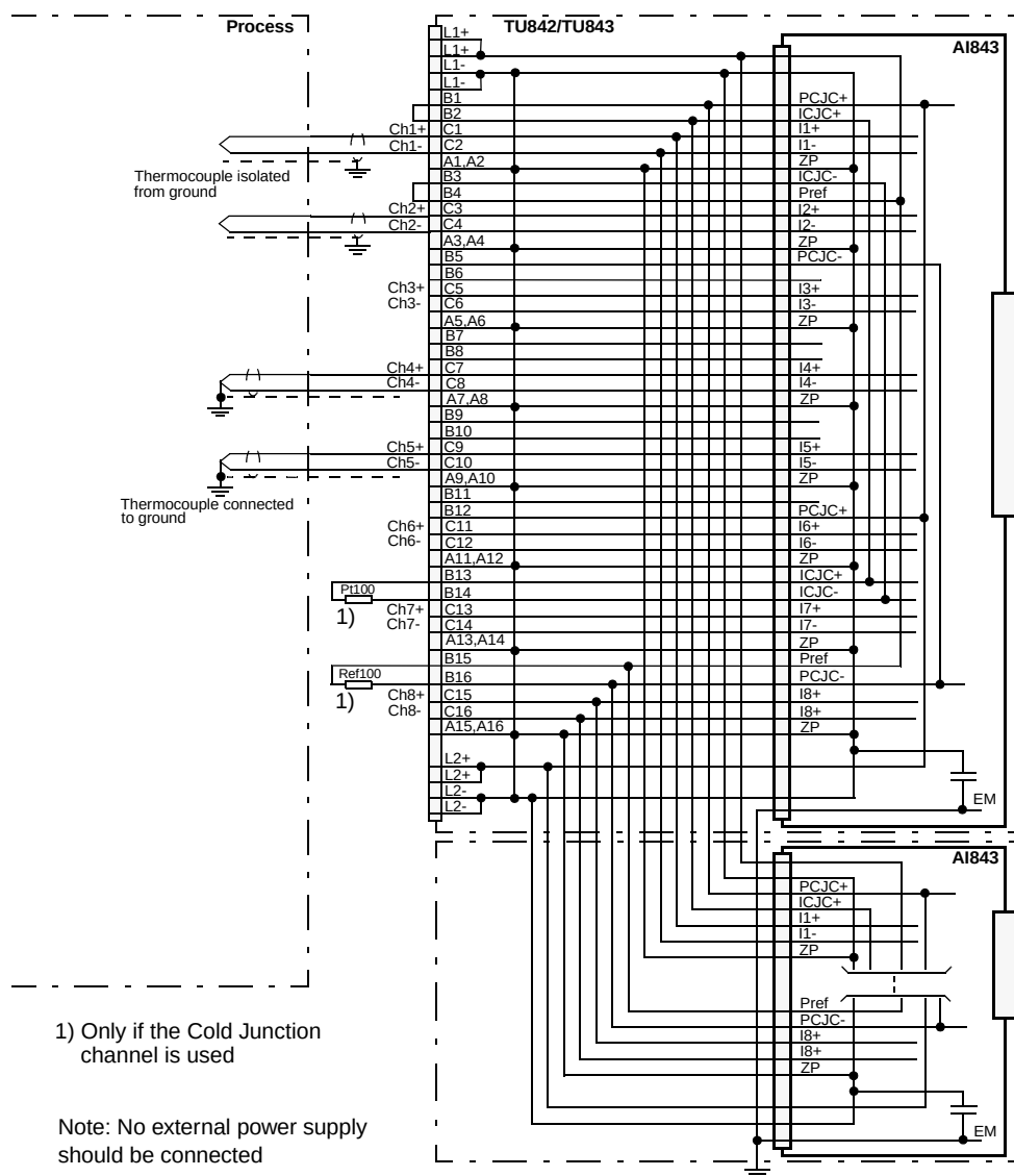
Figure 45. AI843 with TU842 or TU843 Extended MTU Process Connections
