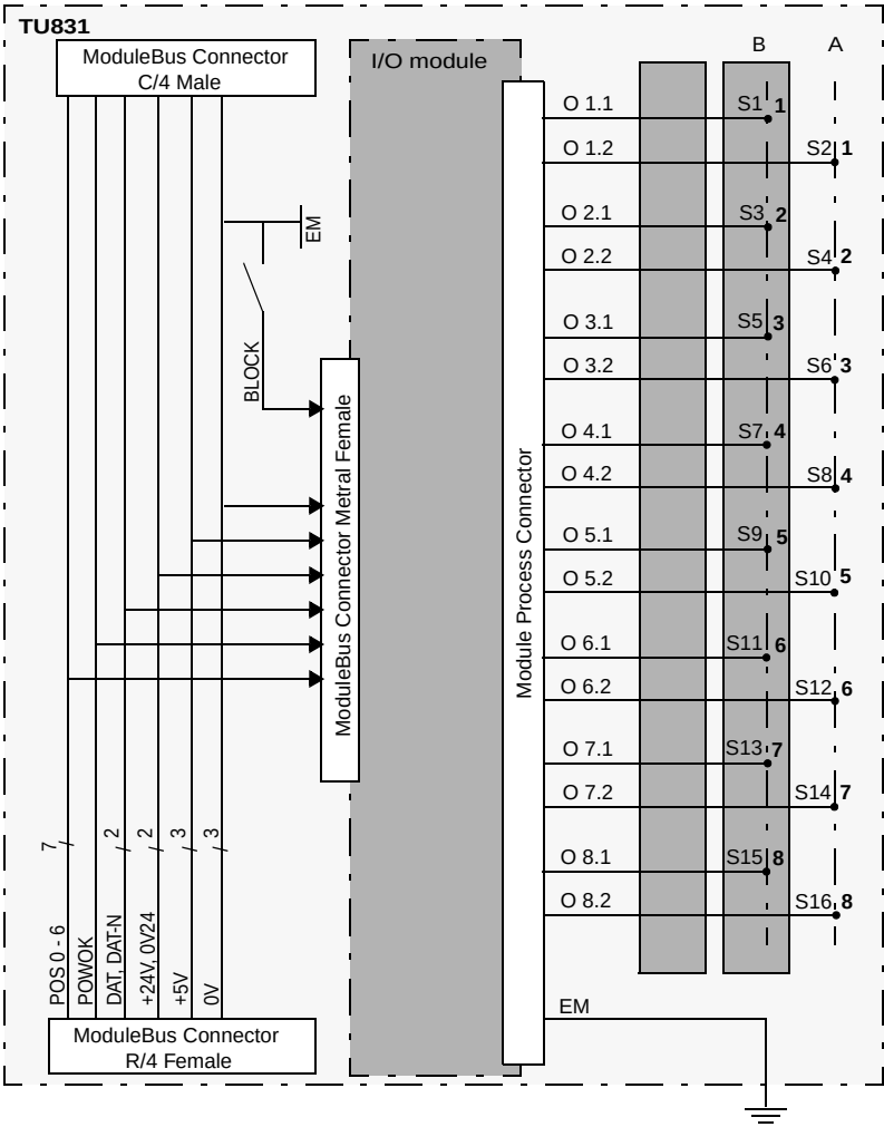
Figure 206. TU831/TU831V1 Block Diagram
