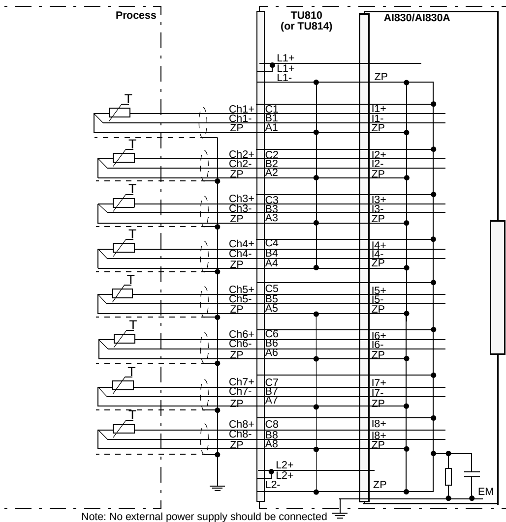
Figure 35. AI830/AI830A with TU810 or TU814 Compact MTU Process Connections
