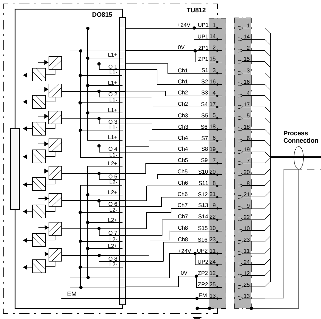
Figure 156. DO815 with TU812 Compact MTU Process Connections
