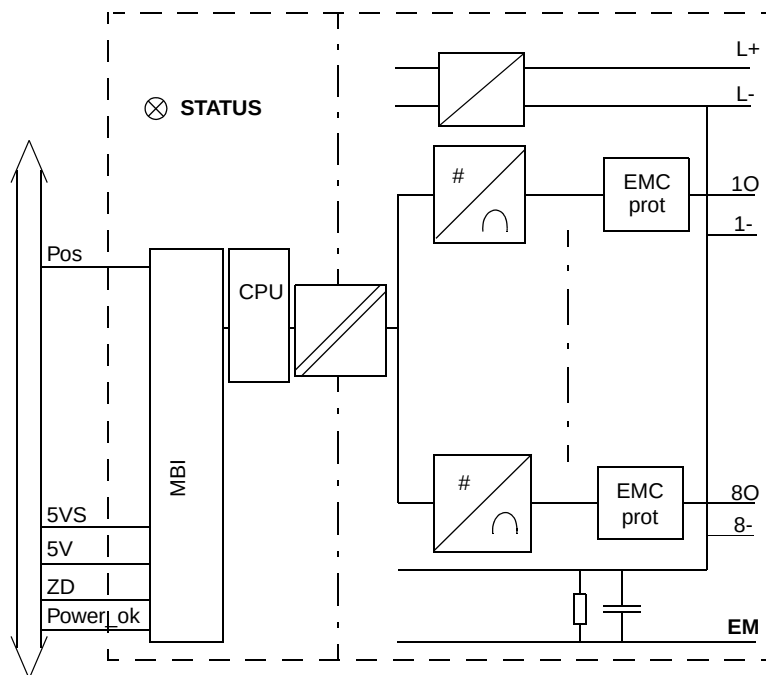
Figure 60. AO801 Block Diagram
