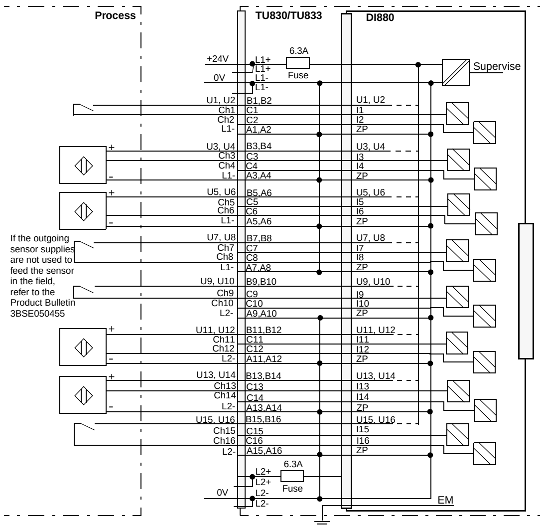
Figure 133. DI880 with TU830 Extended MTU Process Connections
