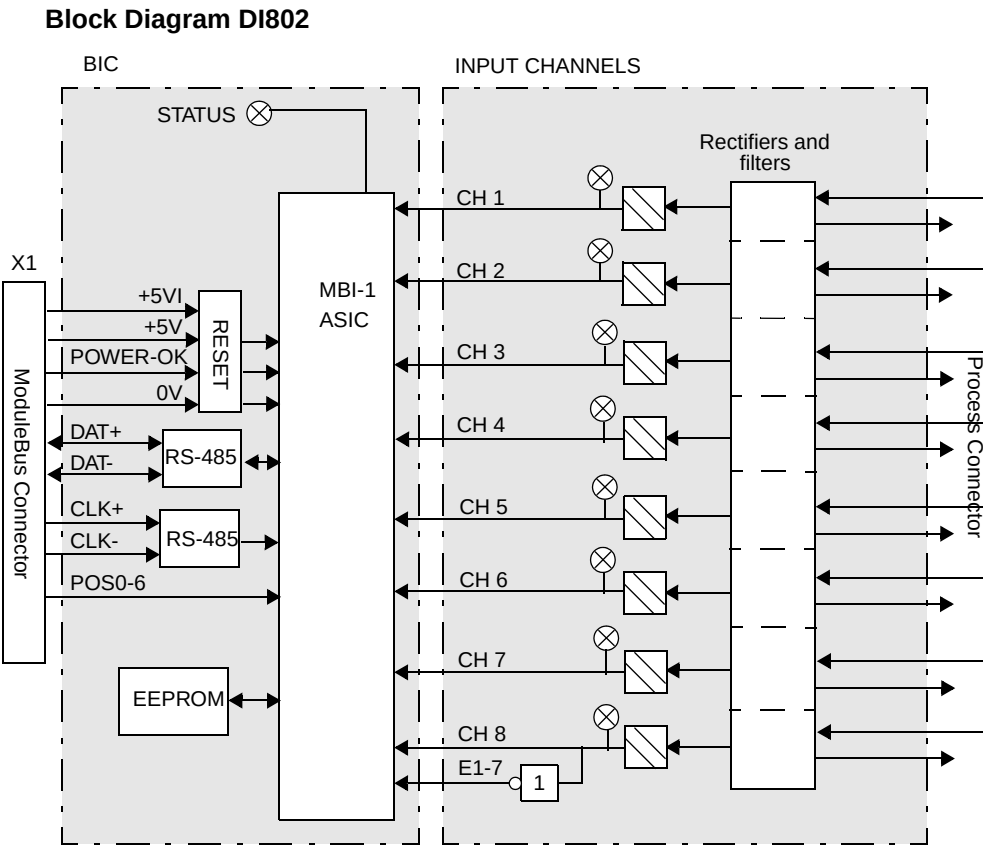
Figure 81. DI802 Block Diagram
