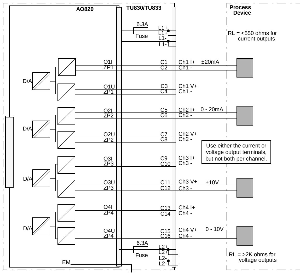
Figure 71. AO820 with TU830 Extended MTU Process Connections
