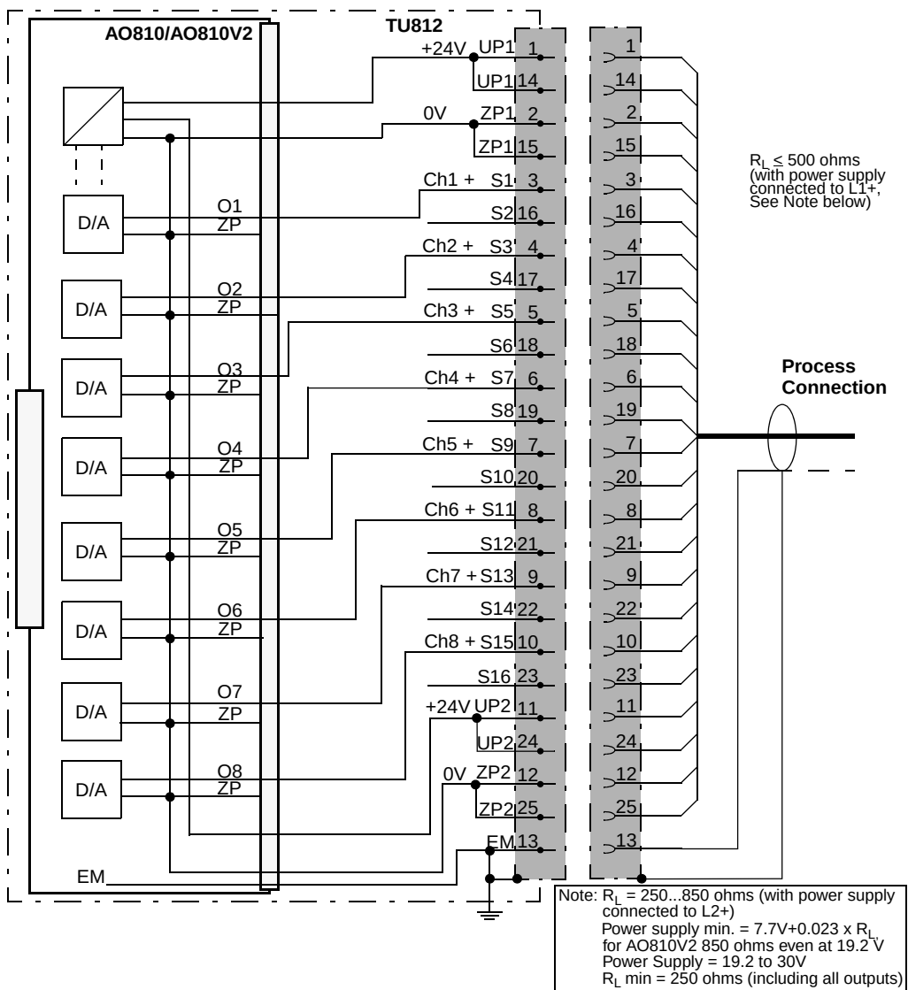
Figure 65. AO810/AO810V2 with TU812 Compact MTU Process Connections
