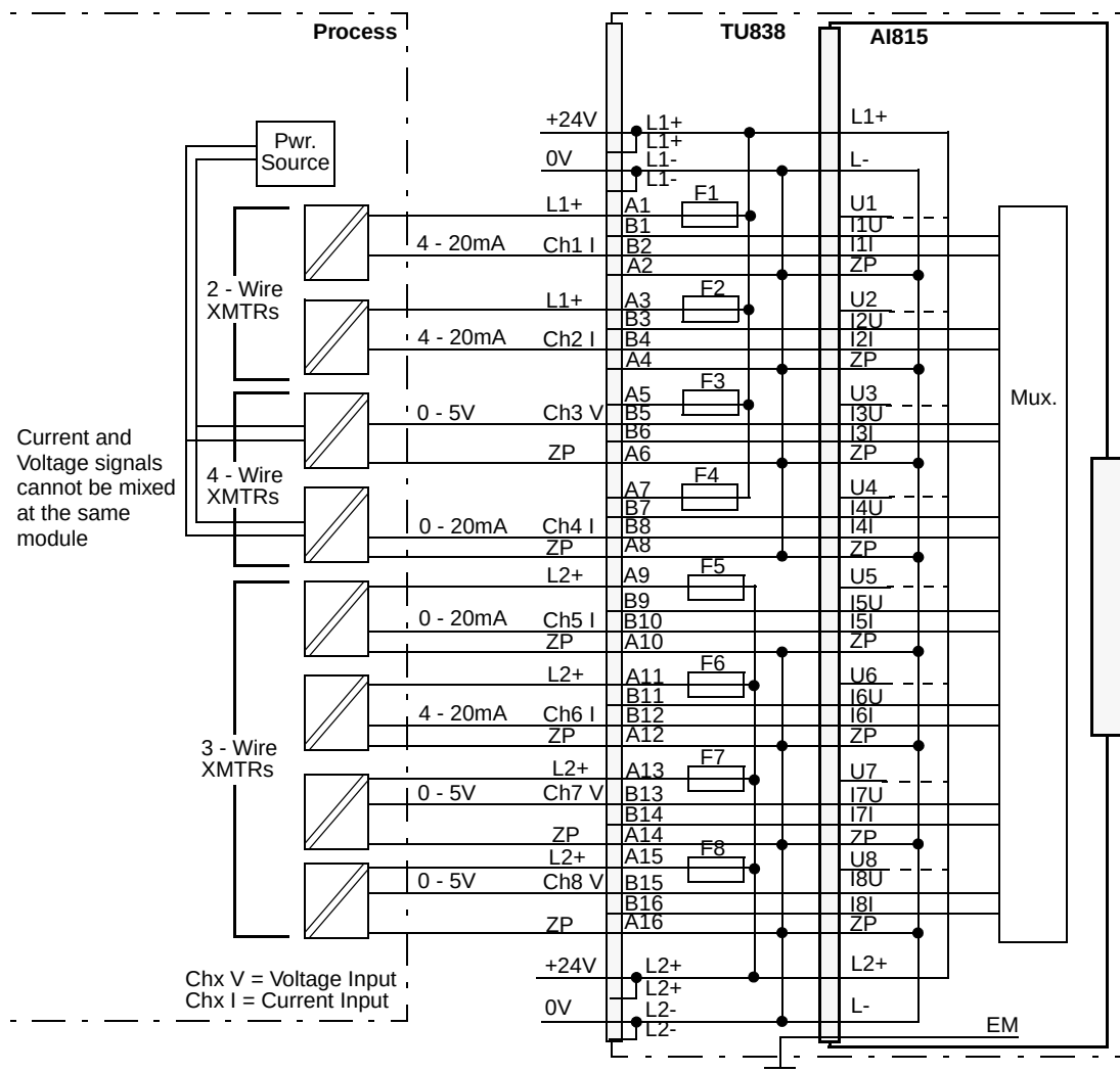
Figure 22. AI815 with TU838 Extended MTU Process Connections
