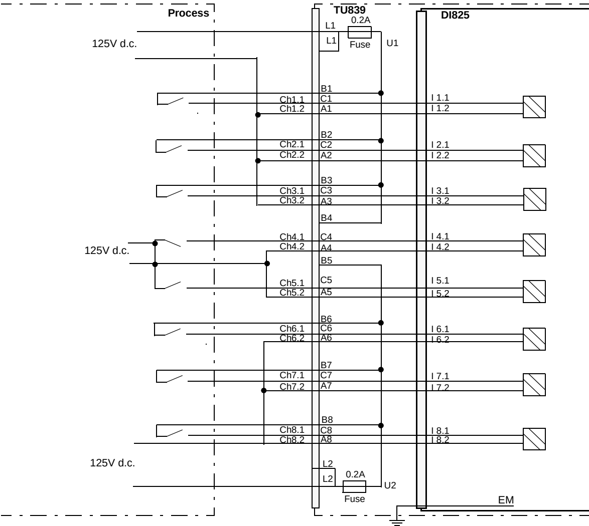
Figure 113. DI825 with TU839 Extended MTU Process Connections
