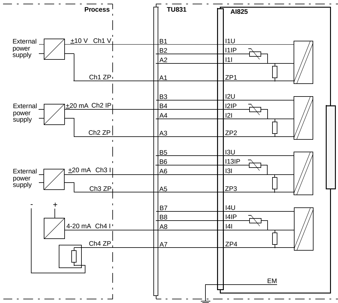
Figure 31. AI825 with TU831 Extended MTU Process Connections
