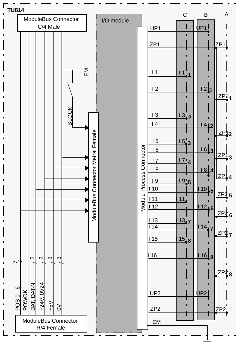
Figure 204. TU814/TU814V1 Block Diagram
