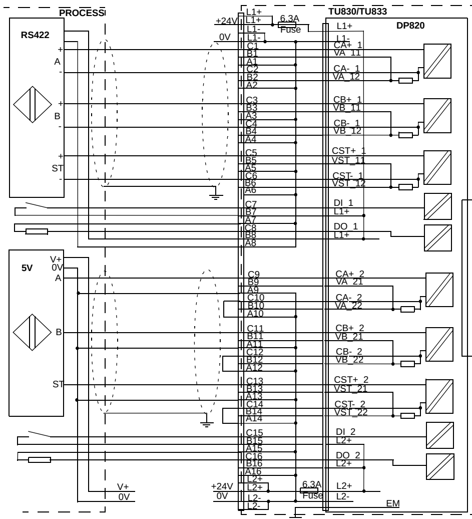
Figure 189. DP820 with TU830 MTU Process Connections and with Transducer Connections
