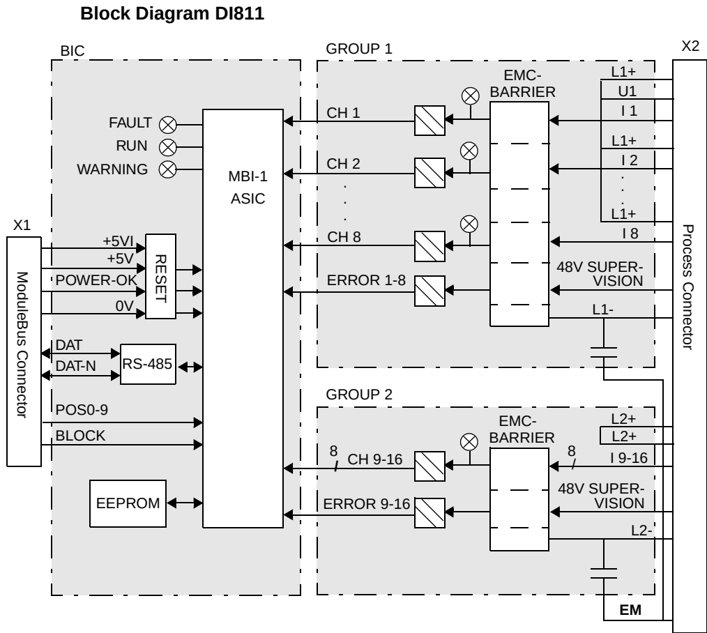
Figure 91. DI811 Block Diagram
