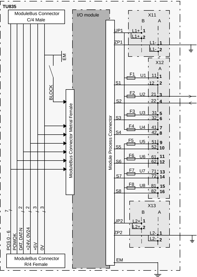
Figure 209. TU835/TU835V1 Block Diagram
