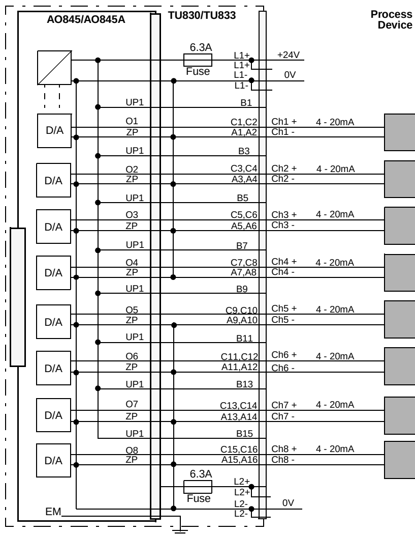
Figure 75. AO845/AO845A with TU830 Extended MTU Process Connections
