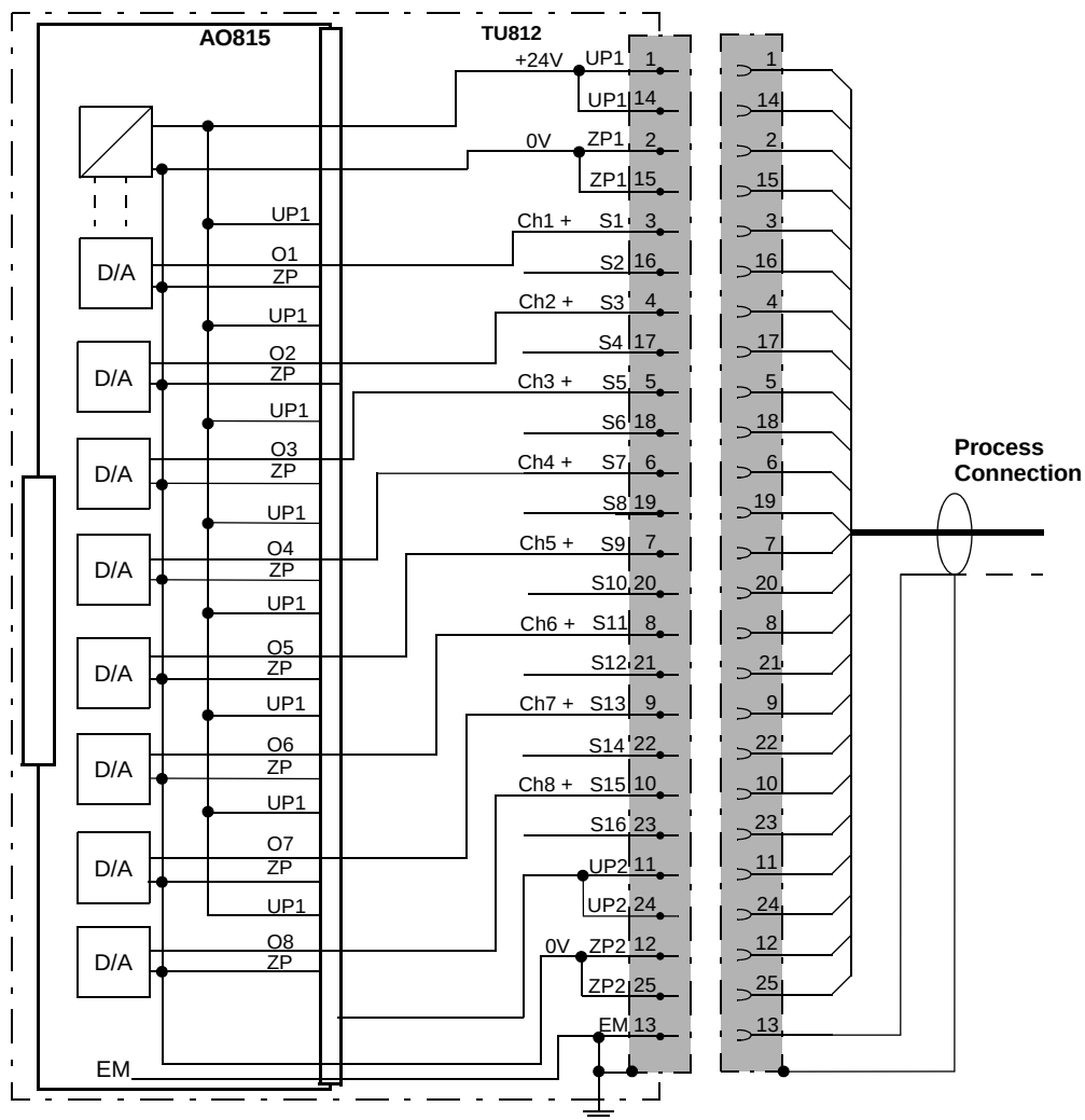
Figure 69. AO815 with TU812 Compact MTU Process Connections
