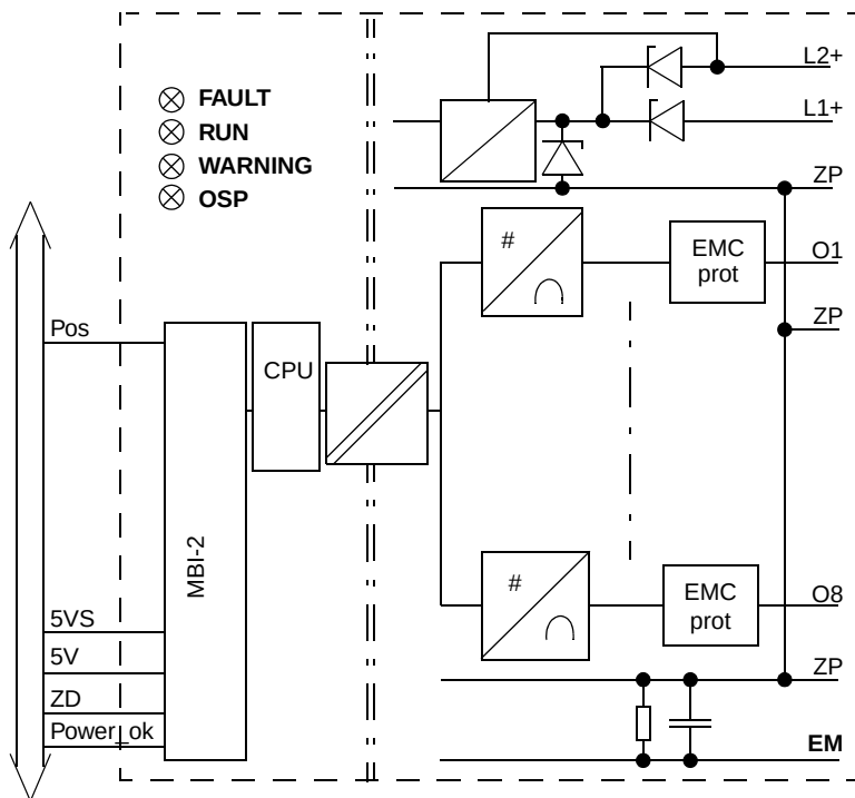
Figure 62. AO810/AO810V2 Block Diagram
