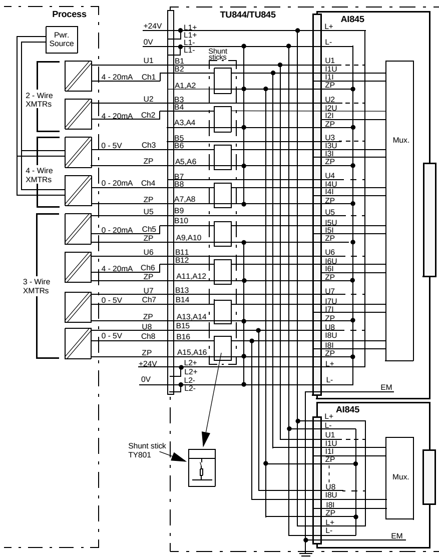
Figure 52. AI845 with TU844 or TU845 Redundant MTU Process Connections
