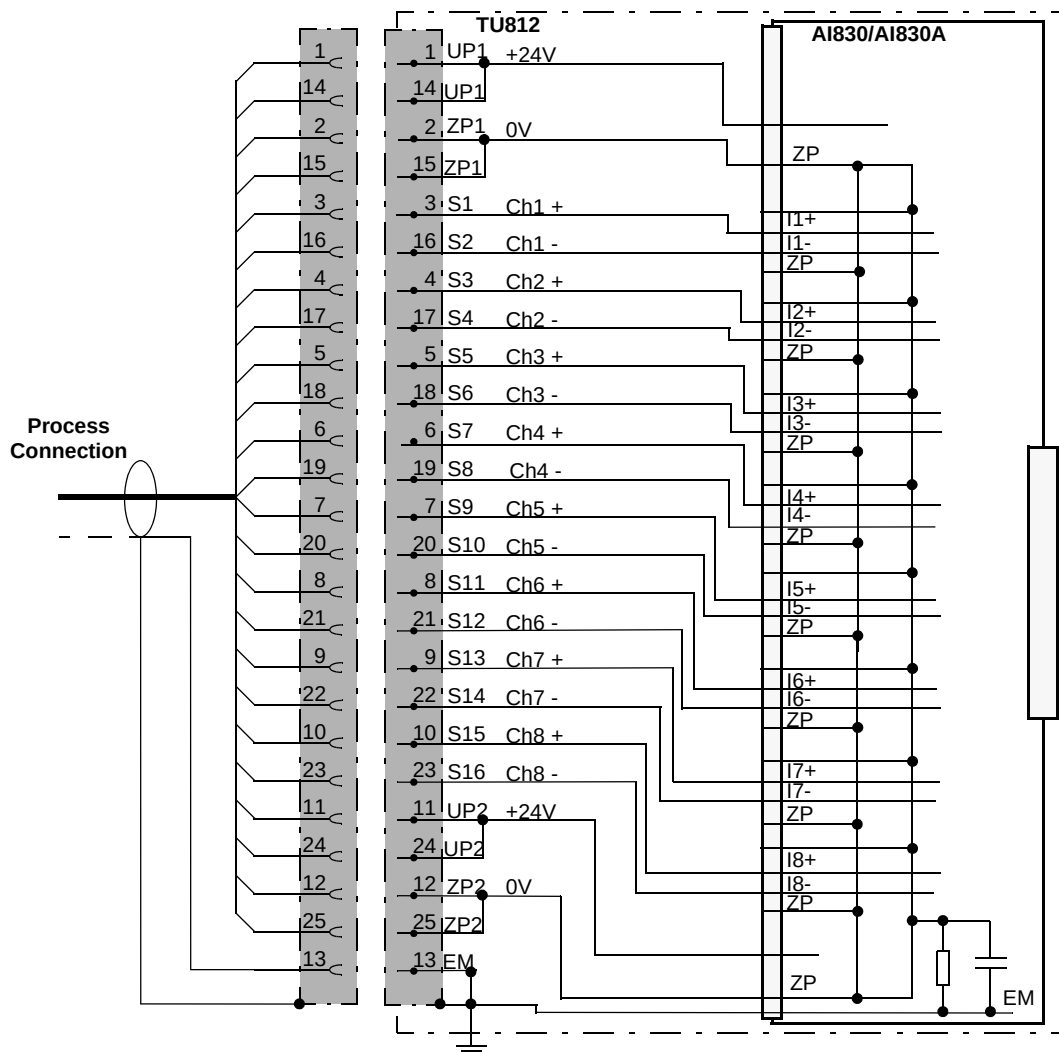
Figure 36. AI830/AI830A with TU812 Compact MTU Process Connections
