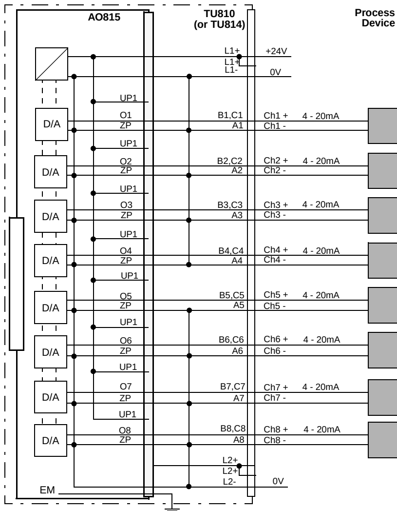
Figure 68. AO815 with TU810 or TU814 Compact MTU Process Connections
