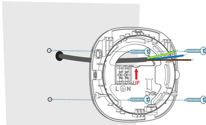
Support mural
