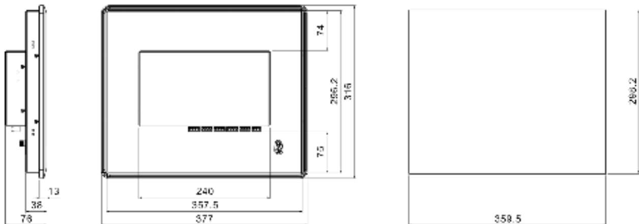
Fig.17 – Case Dimensions and Panel Cutout
