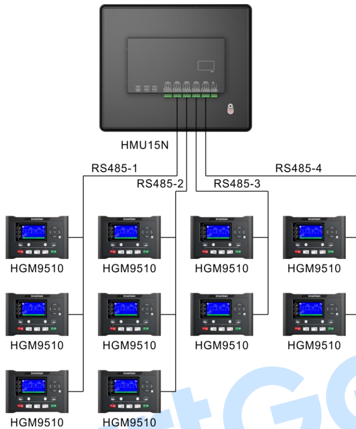
Fig.15 – Typical Application Diagram 1
