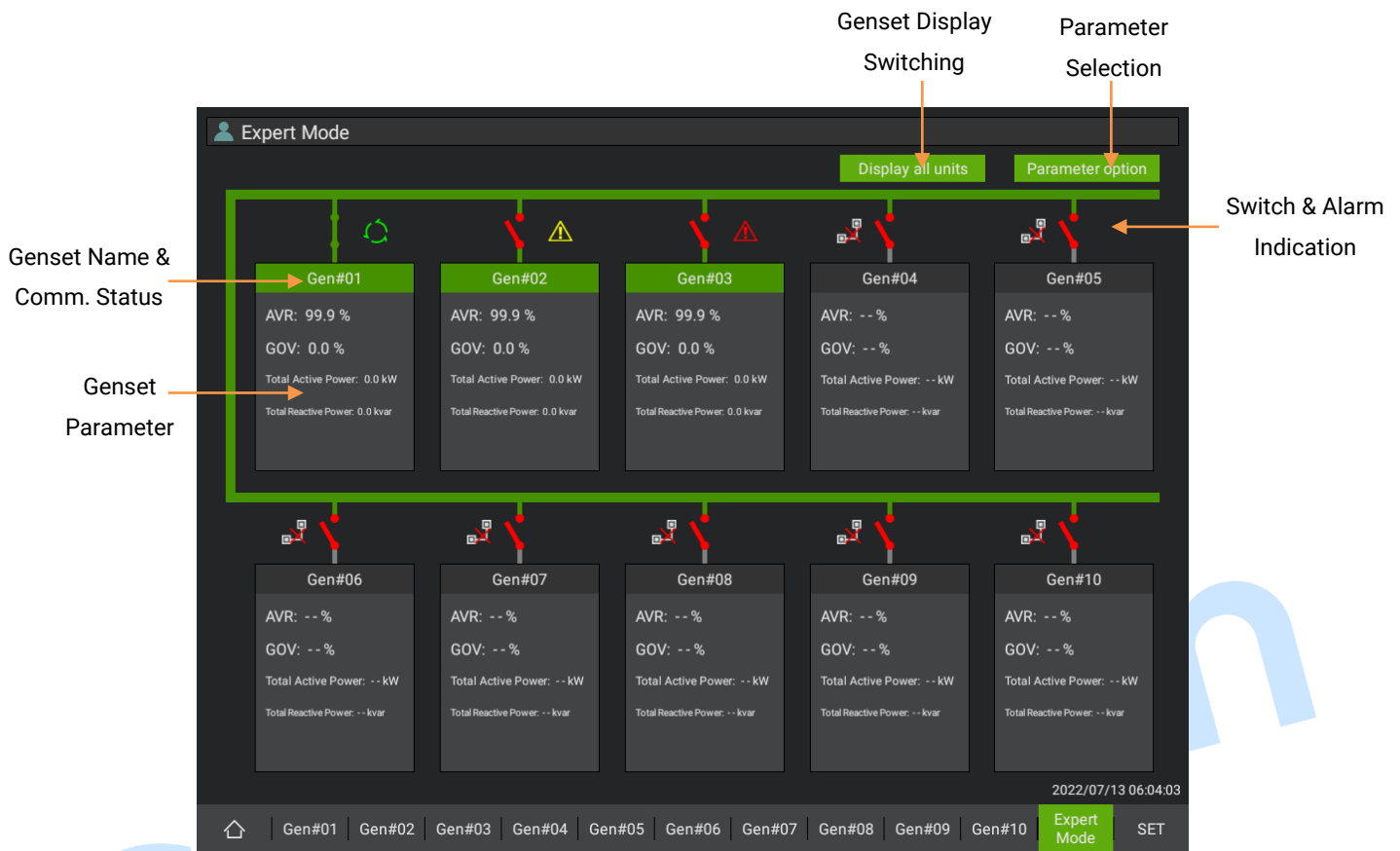
Fig.6 – Expert Mode Interface
