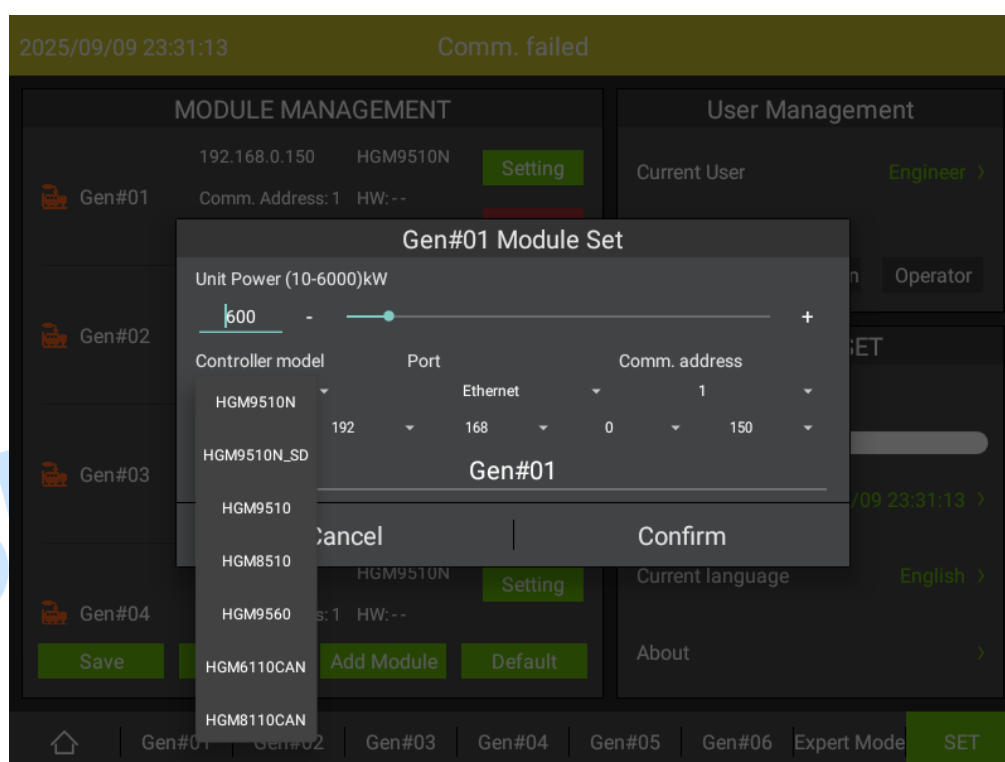
Fig.10 – Model Setting
