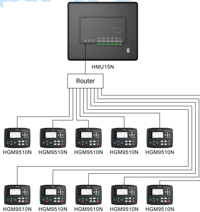
Fig.16 – Typical Application Diagram 2
