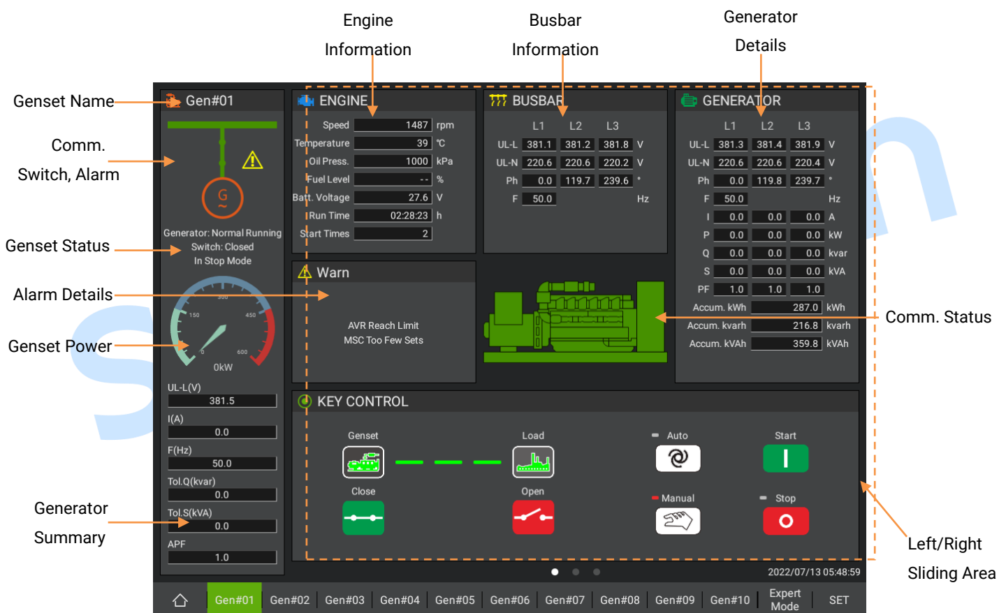
Fig.3 – Genset Details Interface
