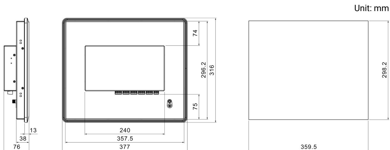
Fig.17 – Case Dimensions and Panel Cutout
