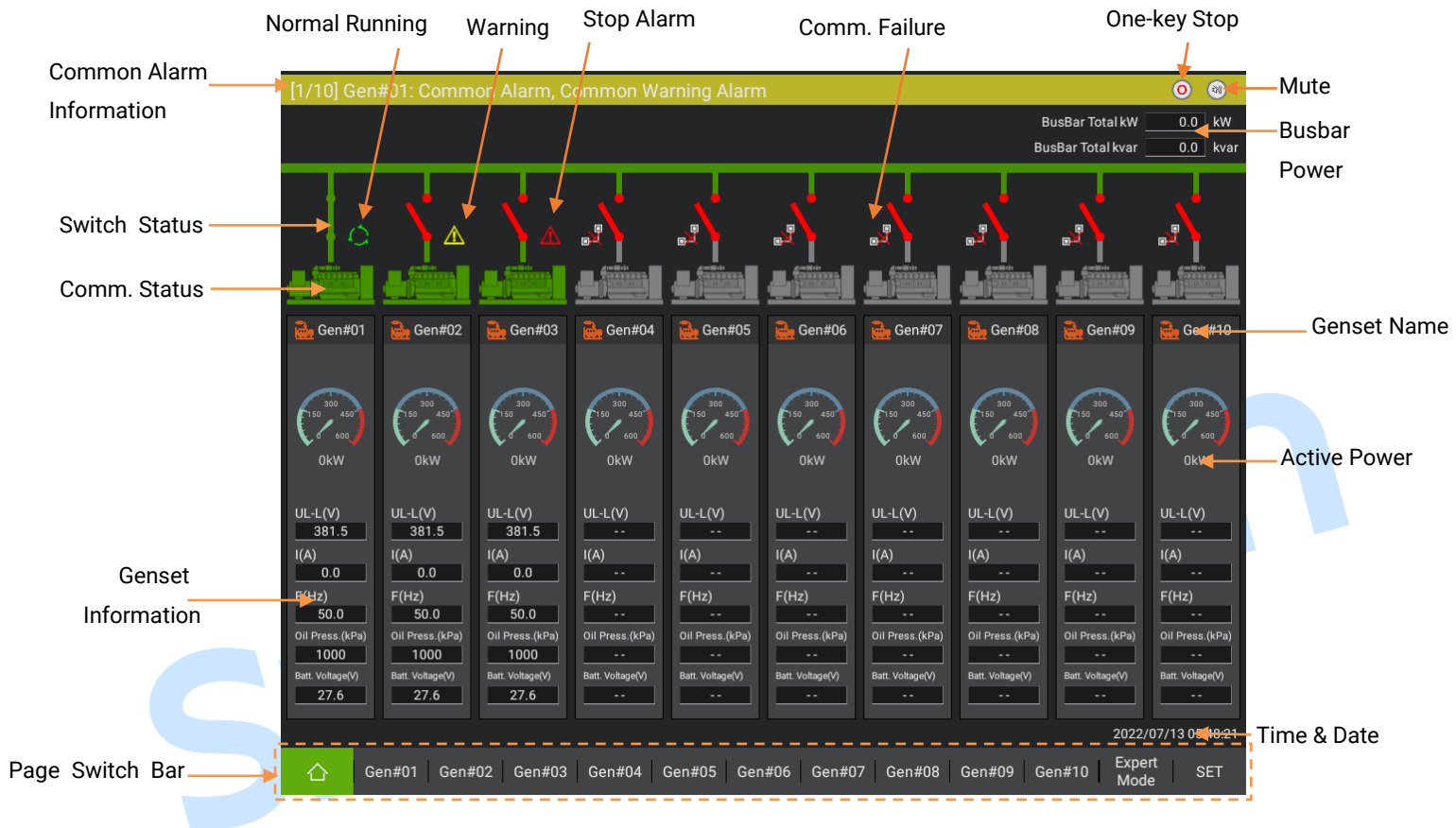
Fig.2 – Homepage Interface
