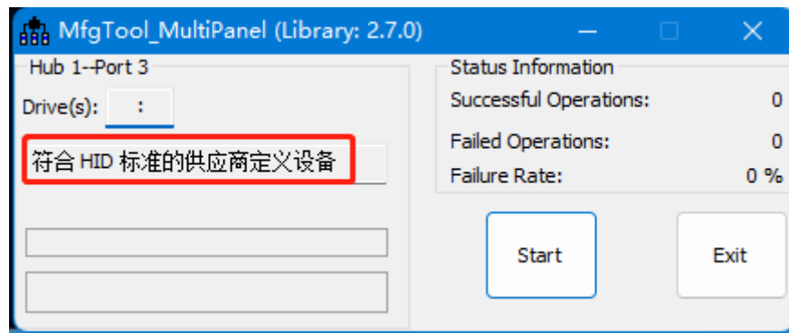
Fig.13 – Flash Mode
