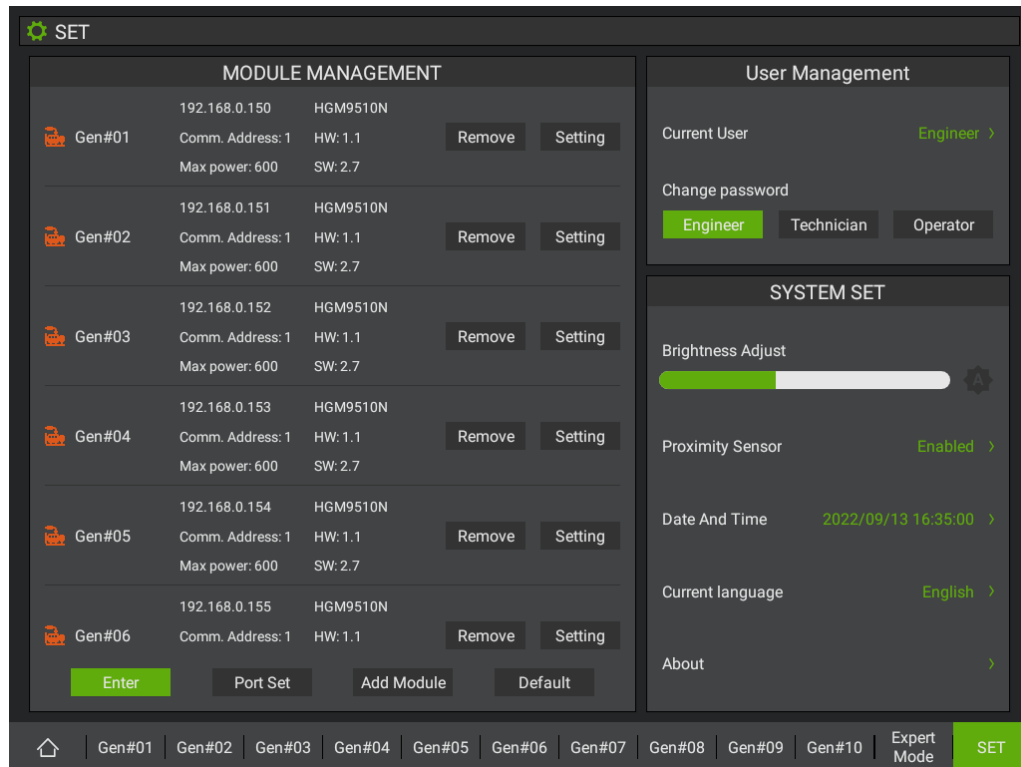
Fig.8 – Setting Interface
