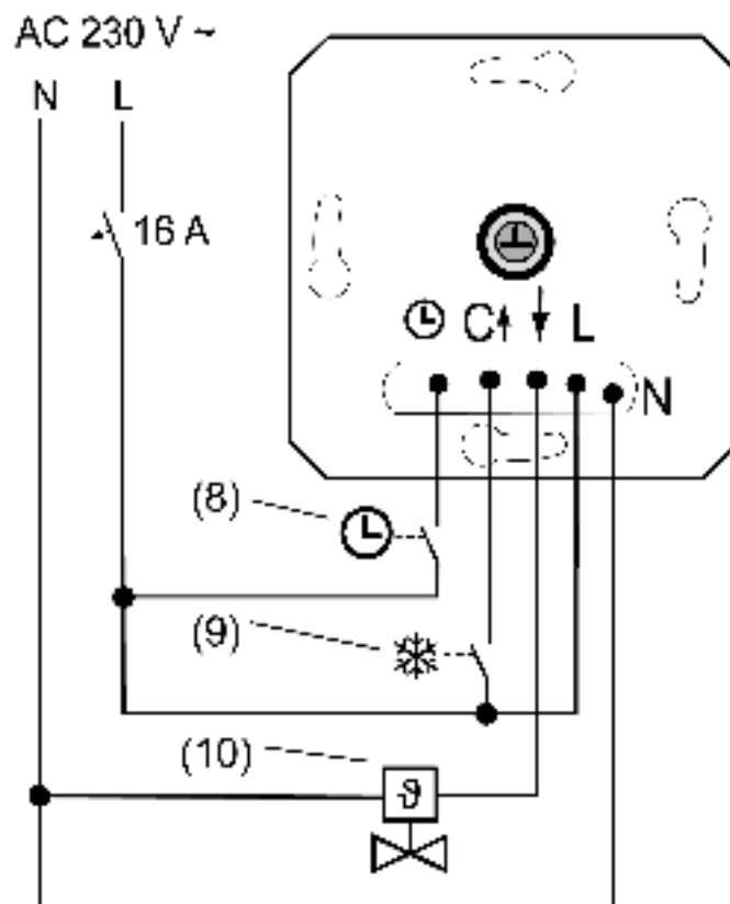
Figure 2: Connection example of the insert
