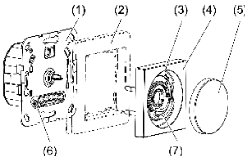
Figure 1: Device components
