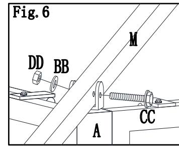
Fig.6 Attach the assembled slanting beam bottomend (M) to plate top of post(A), by using bolt(CC),washer (BB) and nut(DD).
