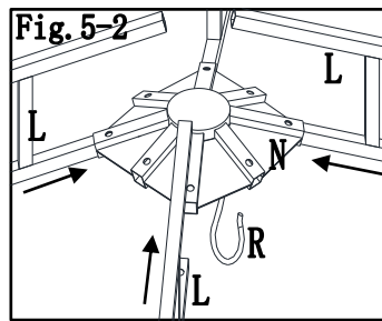
Fig.5-2: Insert slanting beam upper end(L) into large top connector(N),then attach hook(R) to top connector(N).
