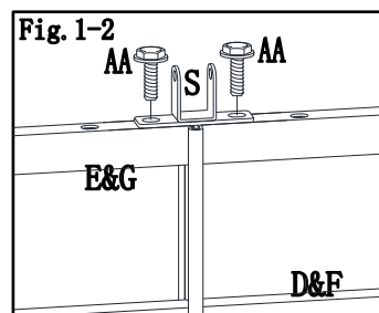
Fig.1-2: Fix middle beam connector(S) to screen, by using bolt(AA).
