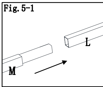
Fig.5- 1:Insert slanting bottom tube(M) into slanting beam(L).
