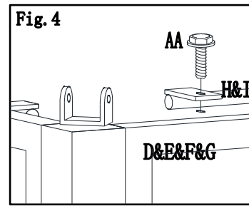
Fig.4: Attach long netting rod(H) to long screen, short netting rod(I) to short screen, by using bolt(AA).
